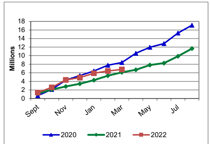
Figure 4: Assessed Penalties
