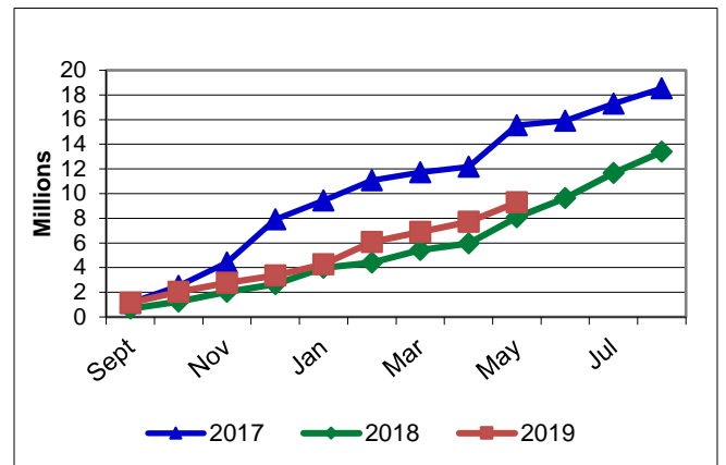
Figure 4: Assessed Penalties
