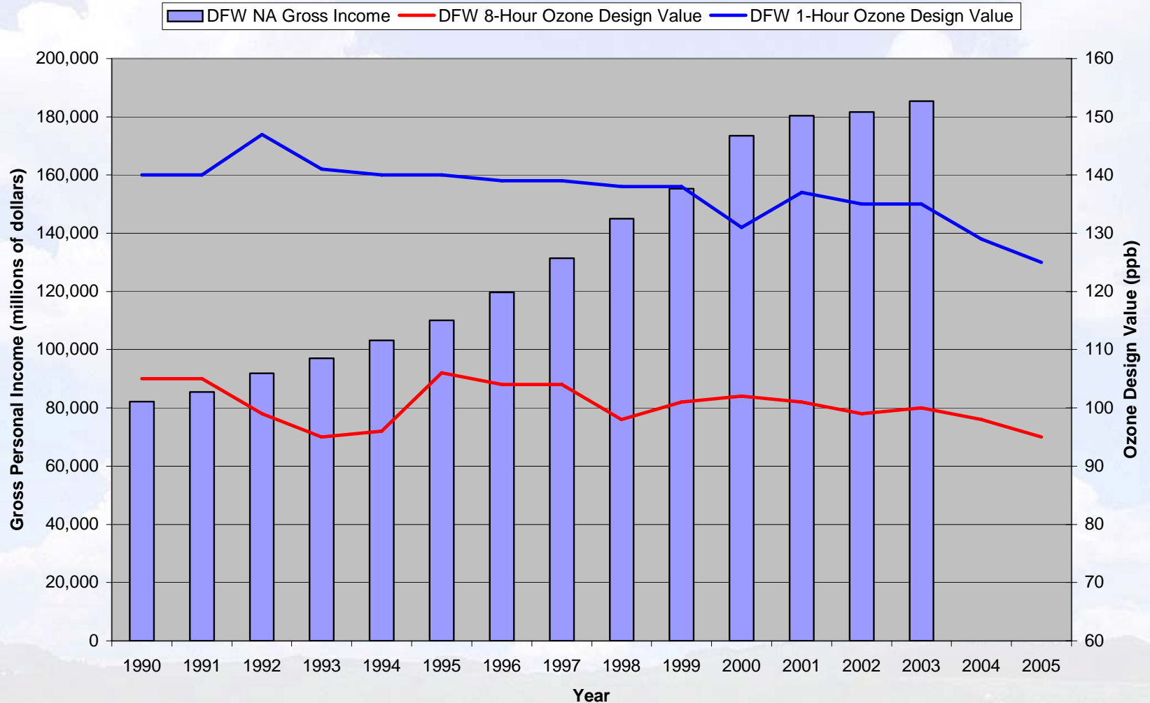
DFW NA Gross Personal Income Versus Ozone Design Values
