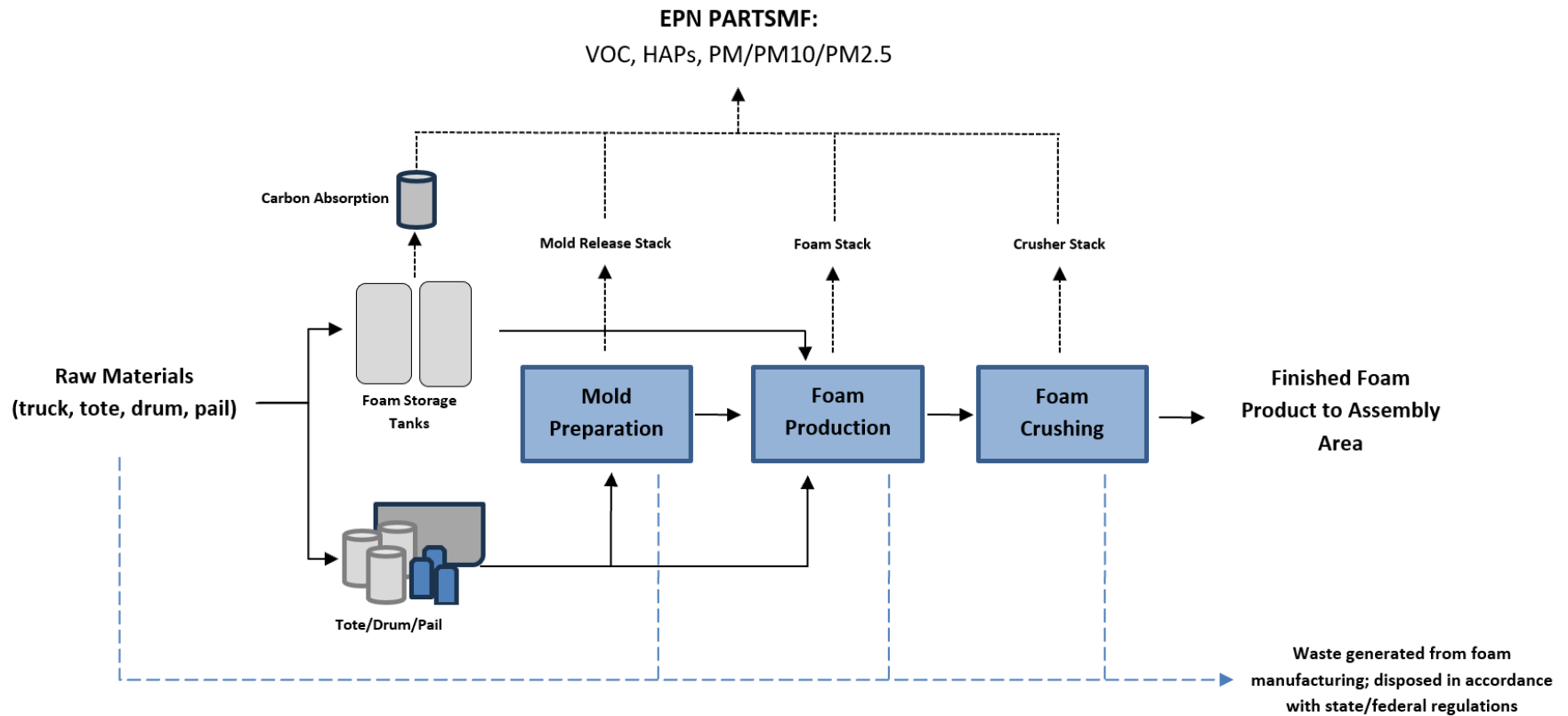
FIGURE 3: FOAM MANUFACTURING
