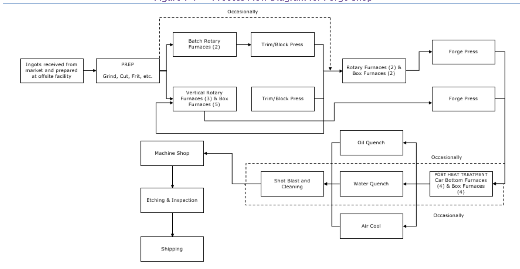
Figure 1-4 Process Flow Diagram for Forge Shop
