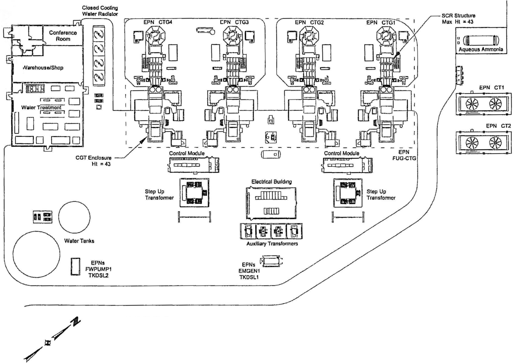
Figure 3-2 PLOT PLAN Leon Creek Plant San Antonio, Texas
