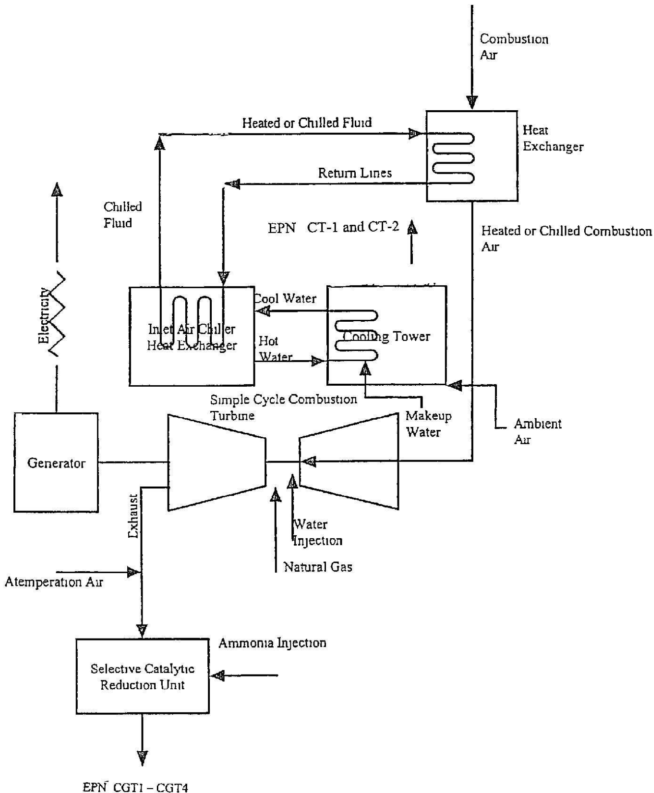
Figure 4-1 PROCESS FLOW DIAGRAM Leon Creek Plant San Antonio, Texas
