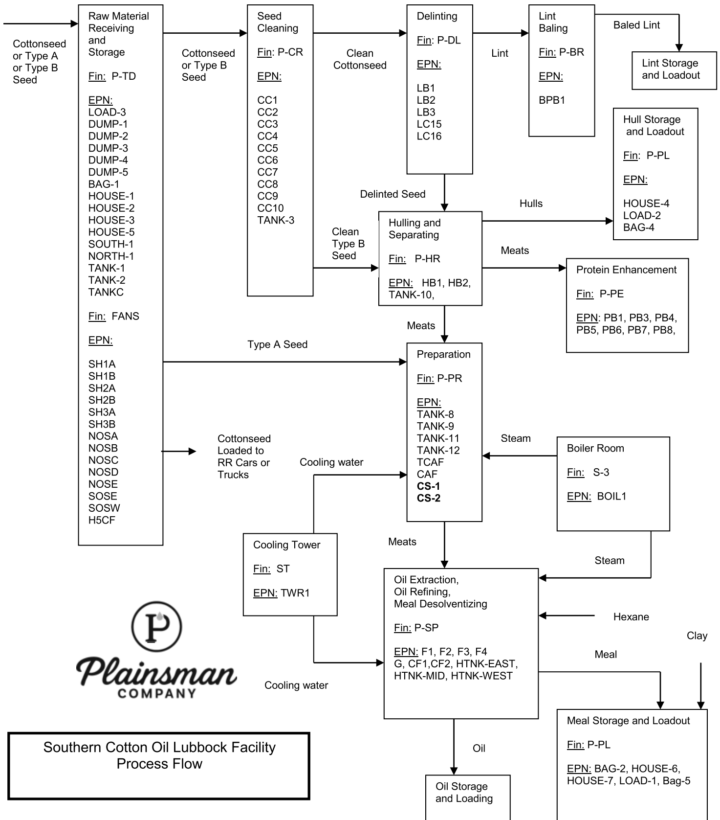
Figure 3-1. Process Flow Diagram
