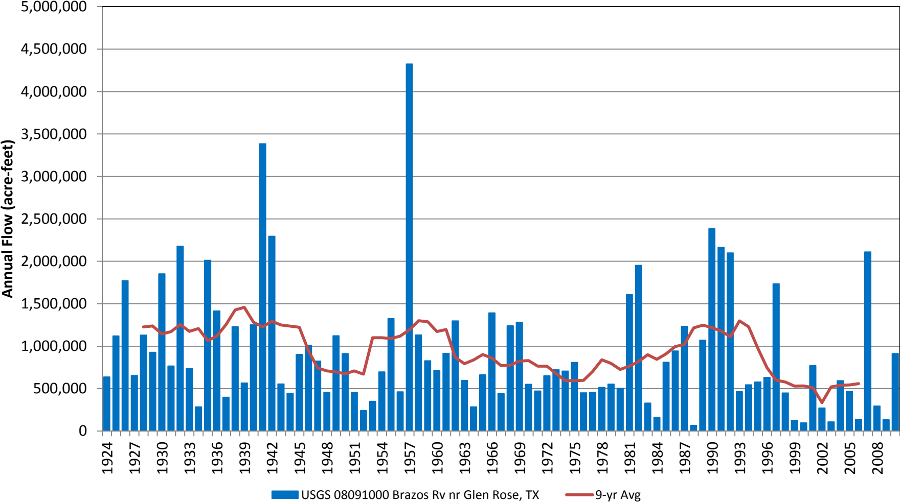
USGS 08091000 Brazos Rv nr Glen Rose, TX Annual Flow (acre-feet)
