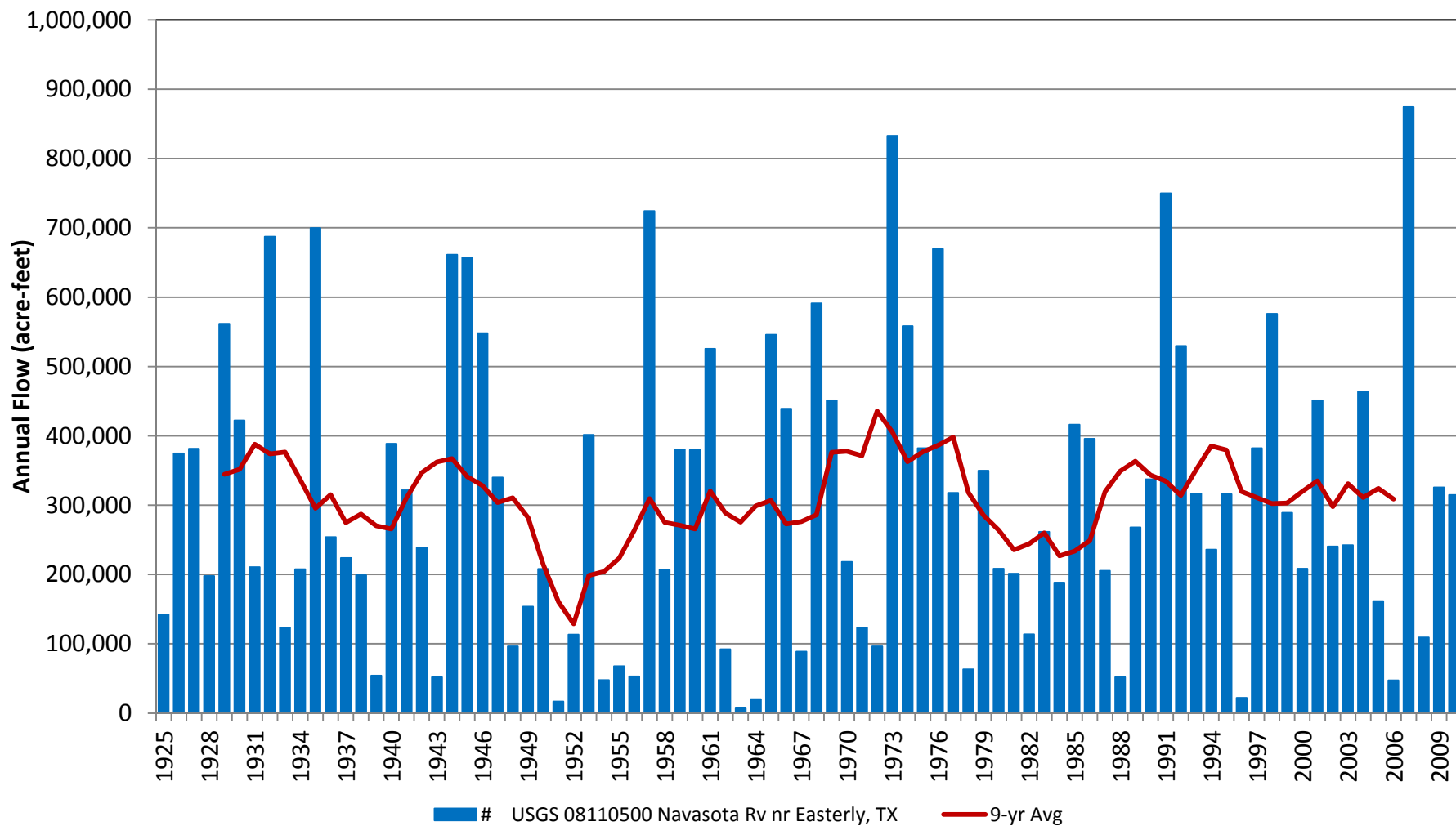
USGS 08110500 Navasota Rv nr Easterly, TX Annual Flow (acre-feet per year)
