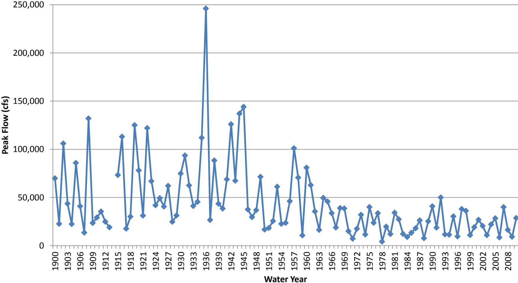
USGS 08096500 Brazos Rv at Waco, TX Peak Flows
