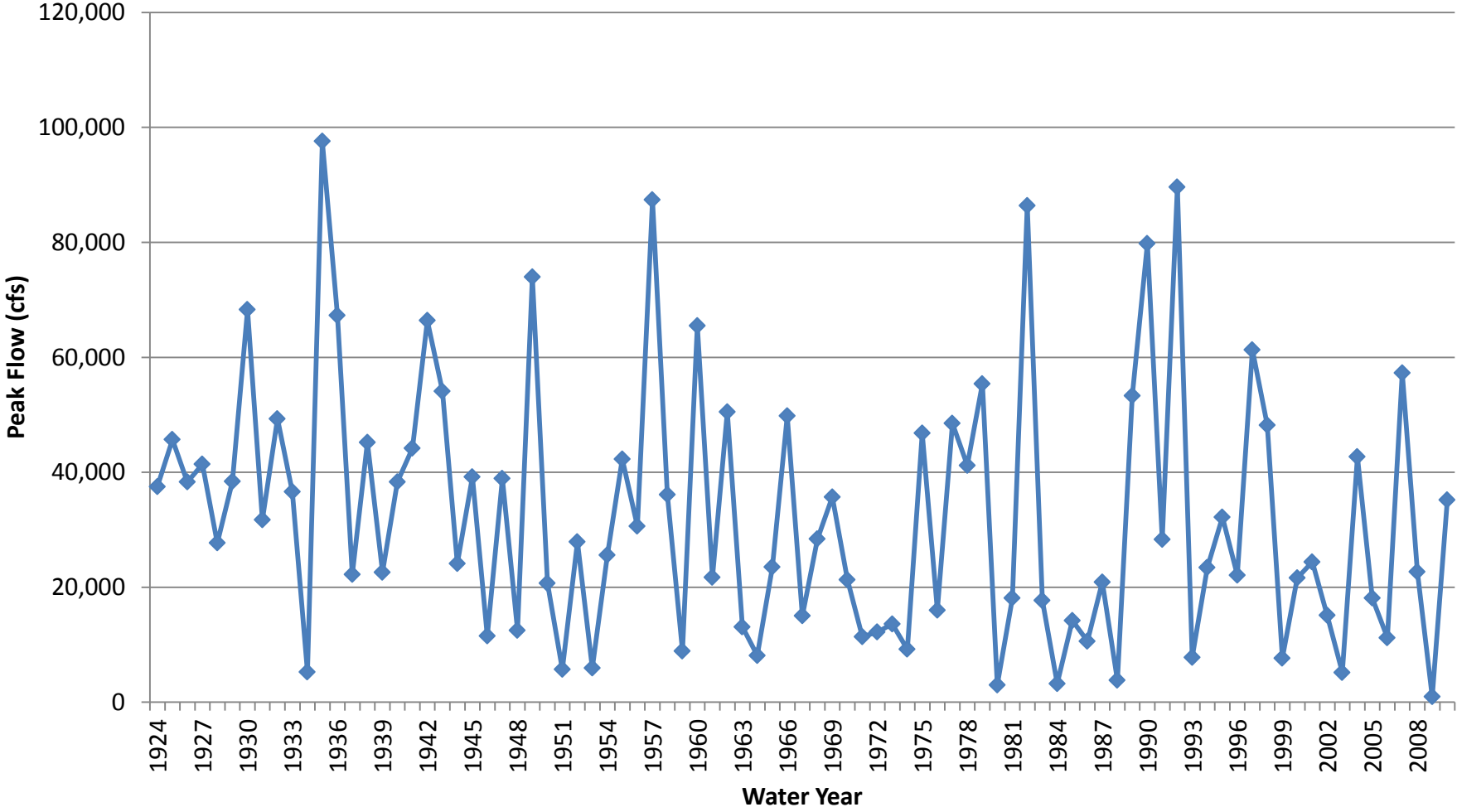
USGS 08091000 Brazos Rv nr Glen Rose, TX Peak Flows
