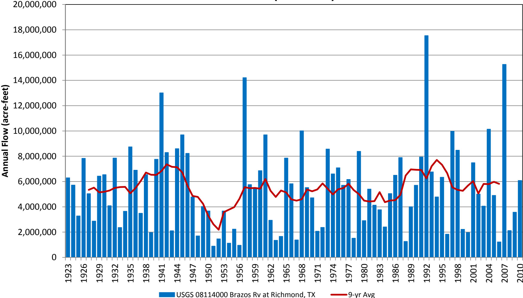
USGS 08114000 Brazos Rv at Richmond, TX Annual Flow (acre-feet)
