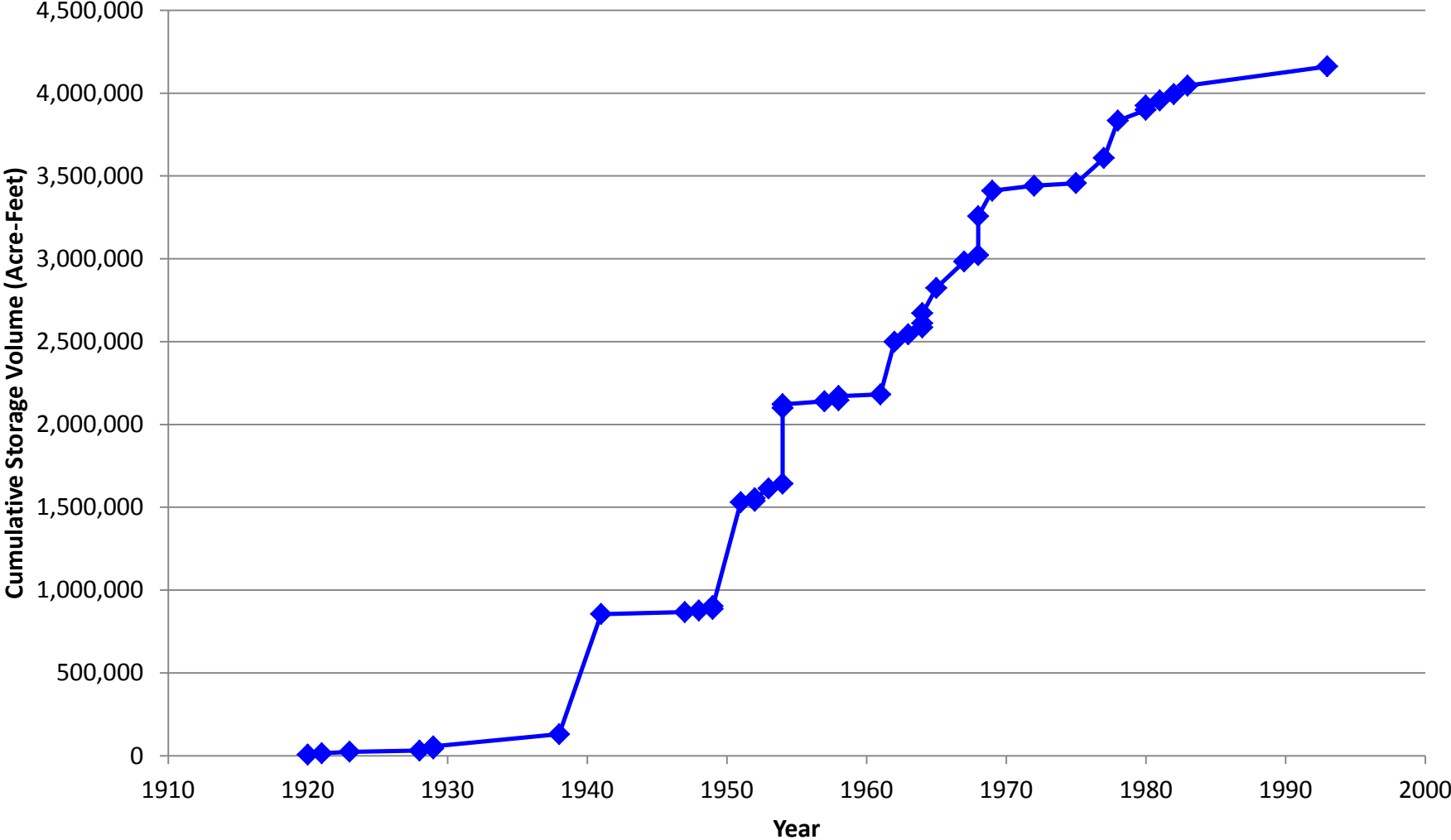
Cumulative Amount of Reservoir Storage Volume in the Brazos Basin
