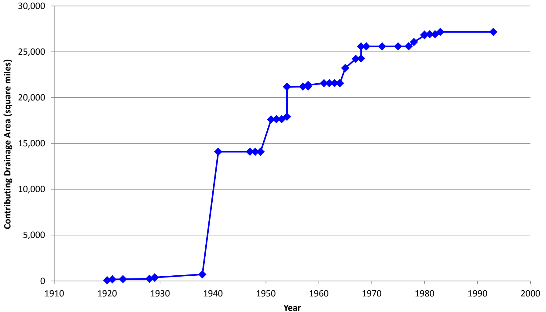
Cumulative Amount of Contributing Drainage Area in the Brazos Basin
