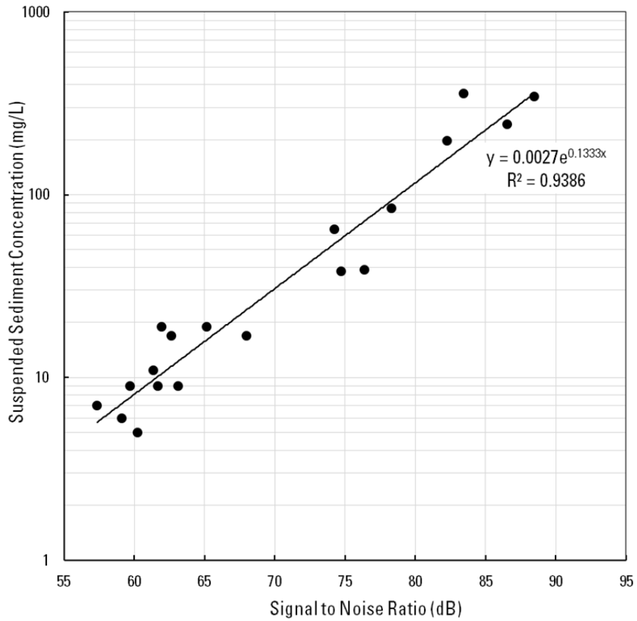
Figure 8. Preliminary regression of suspended sediment concentration on acoustic backscatter data.
