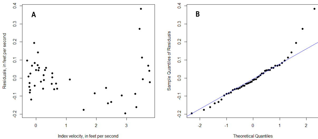
Figure 5. Plots of (A) regression residuals with index velocity and (B) and Quantile-Quantile probability for residuals.
