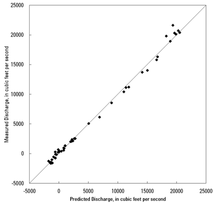
Figure 6. Plot showing measured discharge versus predicted discharge and 1:1 line.
