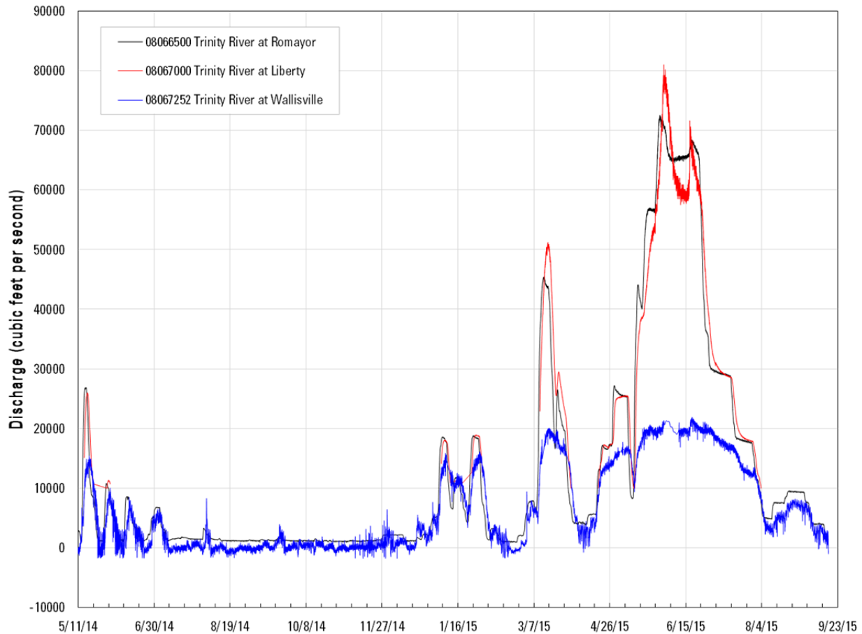
Figure 7. Hydrographs of stations 08066500 Trinity River at Romayor, Tex., 08067000 Trinity River at Liberty, Tex., and 08067252 Trinity River at Wallisville, Tex. from May 2014 to September 2015.
