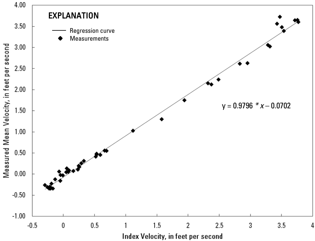
Figure 4. Linear index velocity rating.
