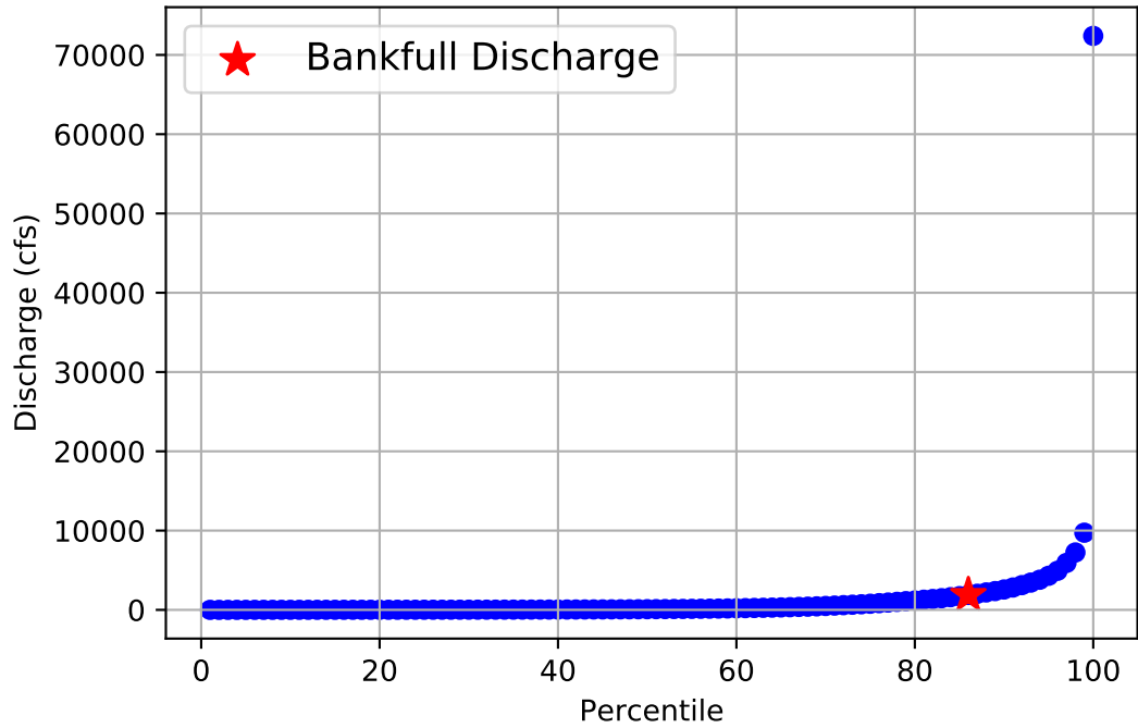
Flow Frequency Distribution for USGS Gage 08018500 from 1939 to 2020
