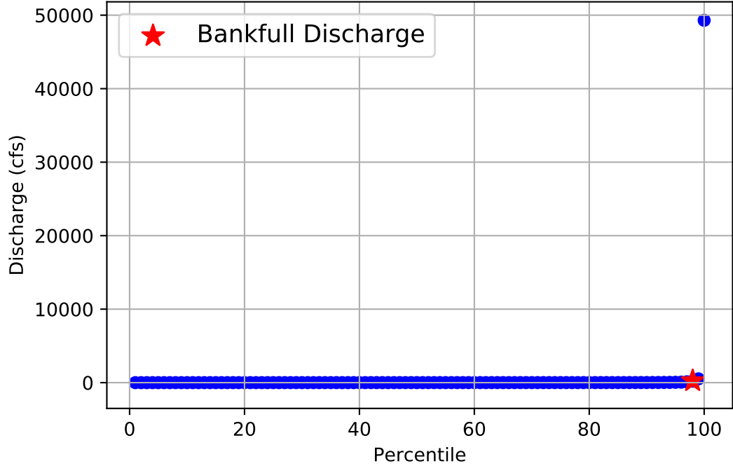
Flow Frequency Distribution for USGS Gage 08189700 from 1964 to 2020
