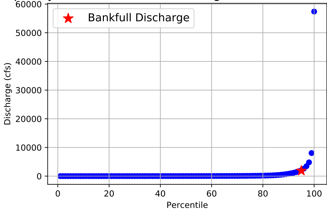
Flow Frequency Distribution for USGS Gage 08110500 from 1924 to 2020
