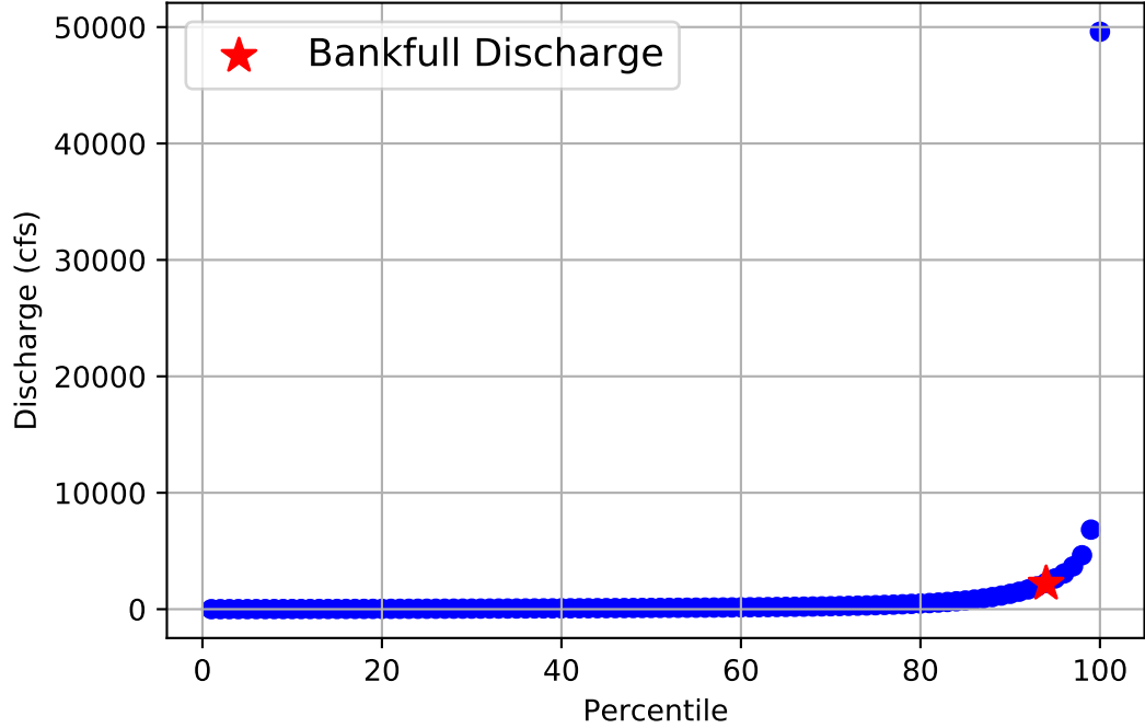
Flow Frequency Distribution for USGS Gage 08117500 from 1954 to 2020
