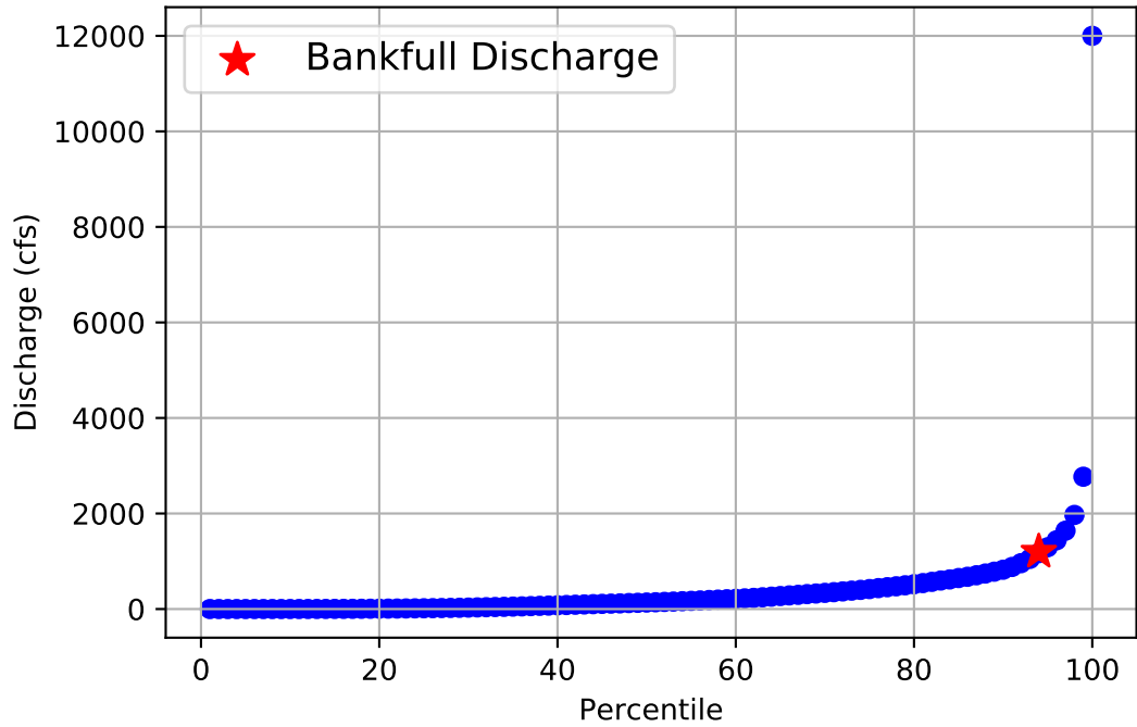
Flow Frequency Distribution for USGS Gage 07346045 from 1968 to 2020
