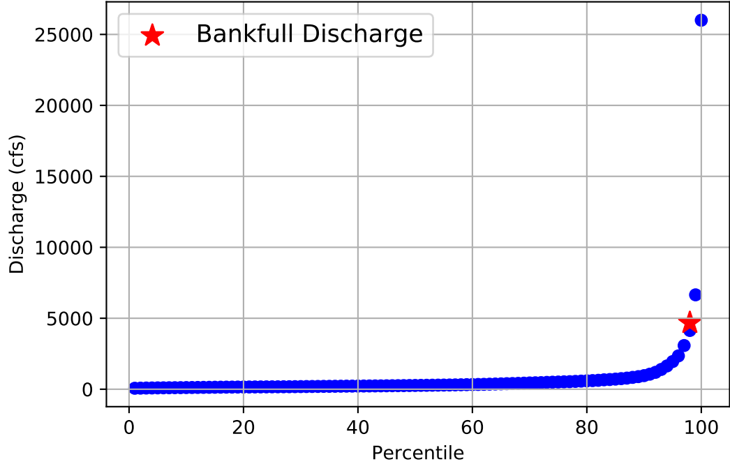
Flow Frequency Distribution for USGS Gage 08183200 from 2006 to 2020
