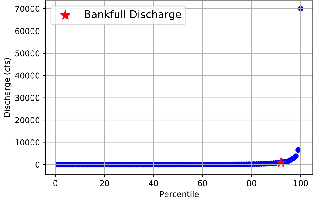
Flow Frequency Distribution for USGS Gage 08194500 from 1942 to 2020
