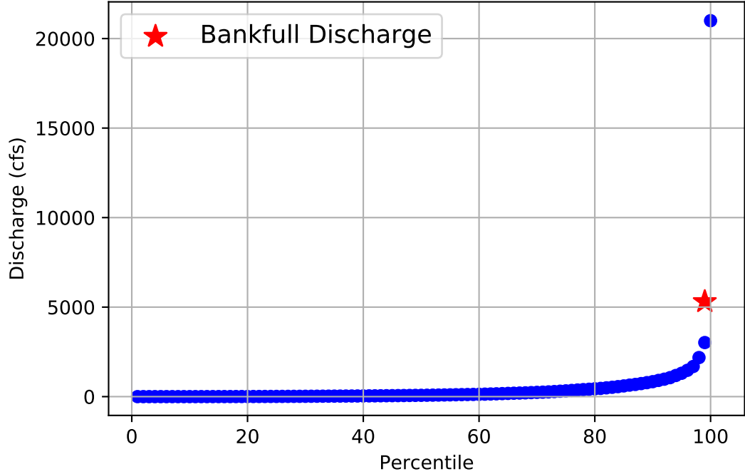
Flow Frequency Distribution for USGS Gage 07346050 from 1962 to 2020
