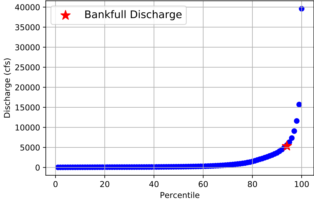
Flow Frequency Distribution for USGS Gage 08019200 from 1997 to 2020
