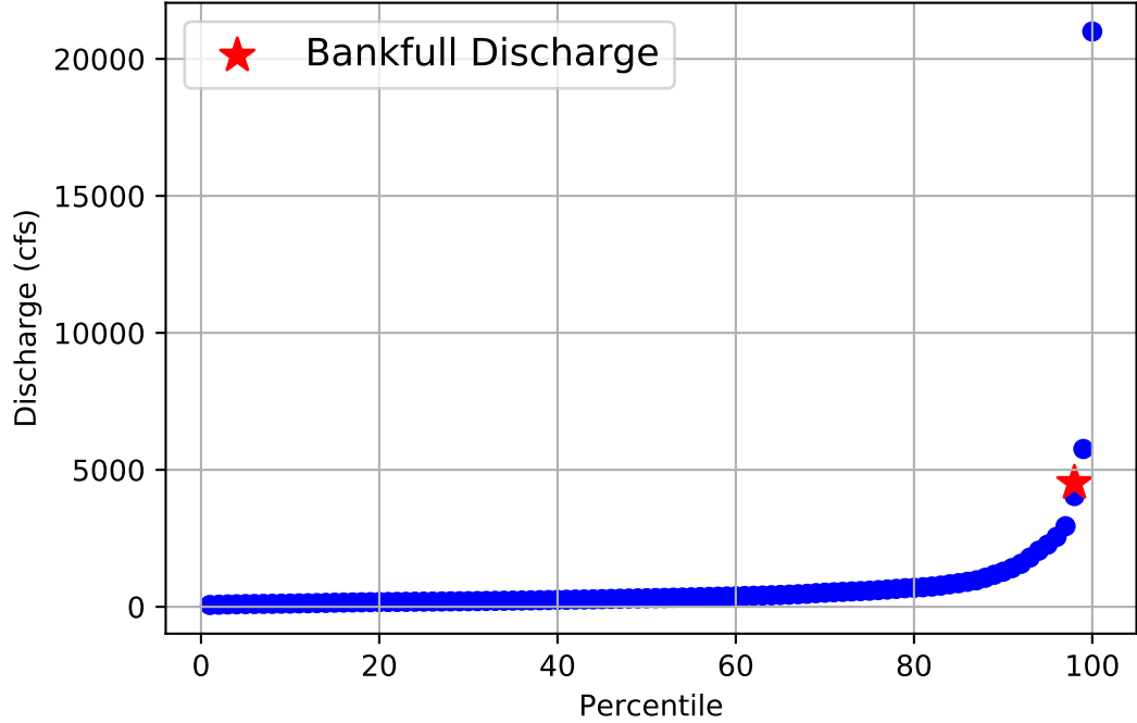
Flow Frequency Distribution for USGS Gage 08188060 from 2011 to 2020
