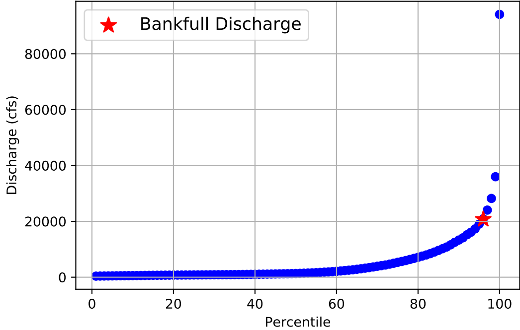
Flow Frequency Distribution for USGS Gage 08062700 from 1964 to 2020
