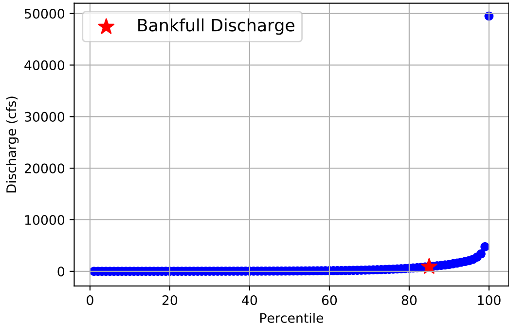
Flow Frequency Distribution for USGS Gage 08041700 from 1967 to 2020
