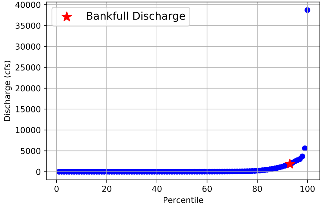
Flow Frequency Distribution for USGS Gage 07342500 from 1942 to 2020
