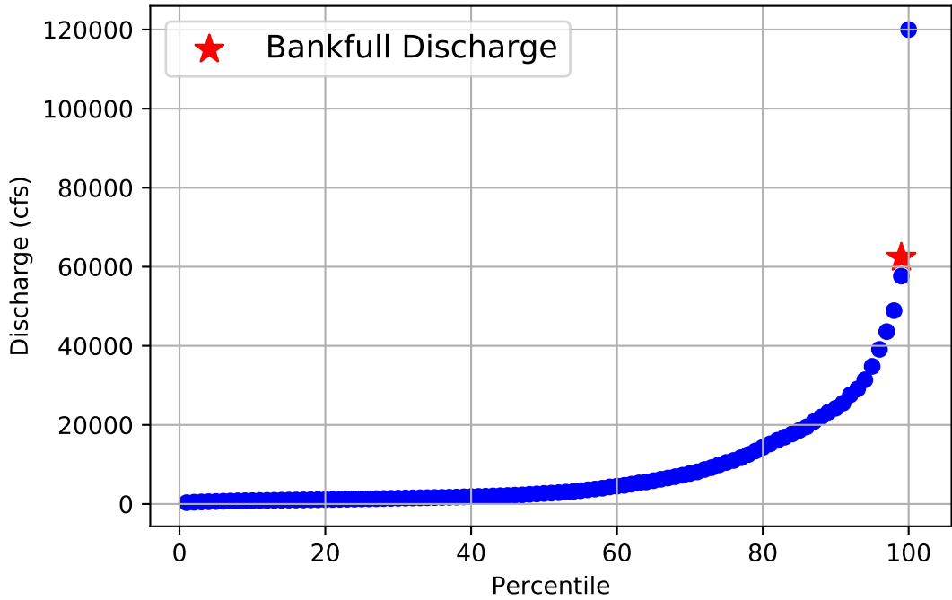
Flow Frequency Distribution for USGS Gage 08066250 from 1965 to 2020
