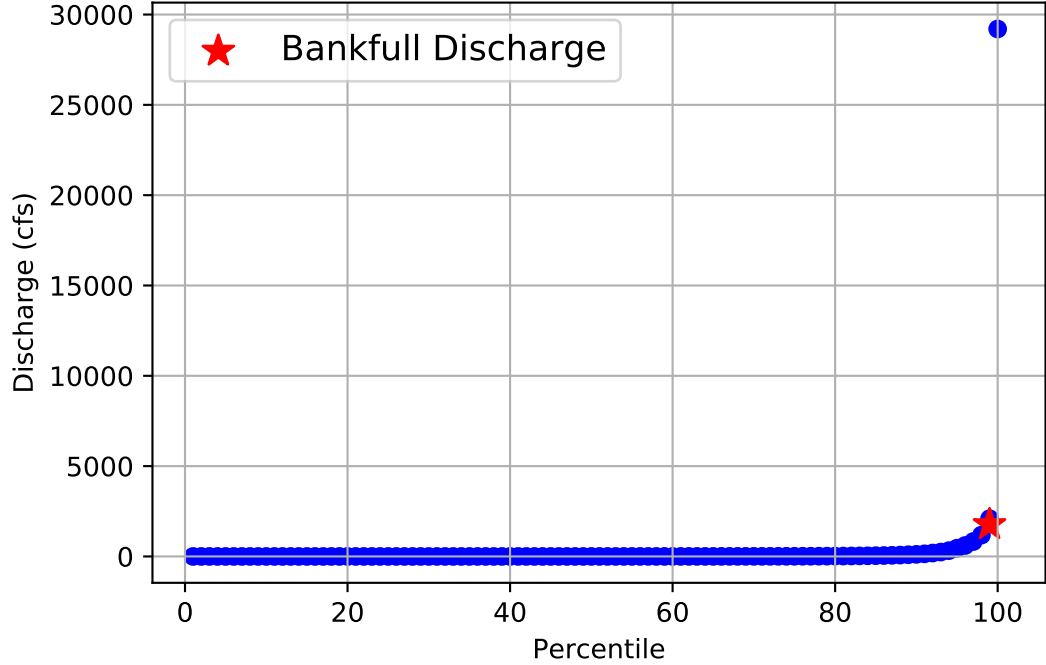
Flow Frequency Distribution for USGS Gage 08042800 from 1956 to 2020
