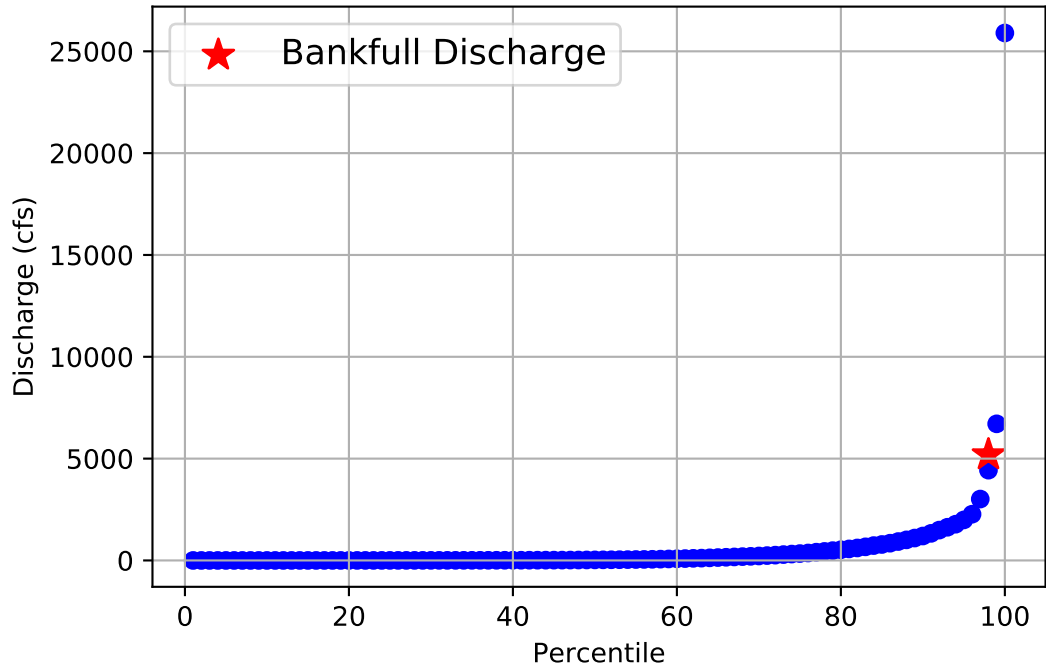
Flow Frequency Distribution for USGS Gage 08064100 from 1983 to 2020
