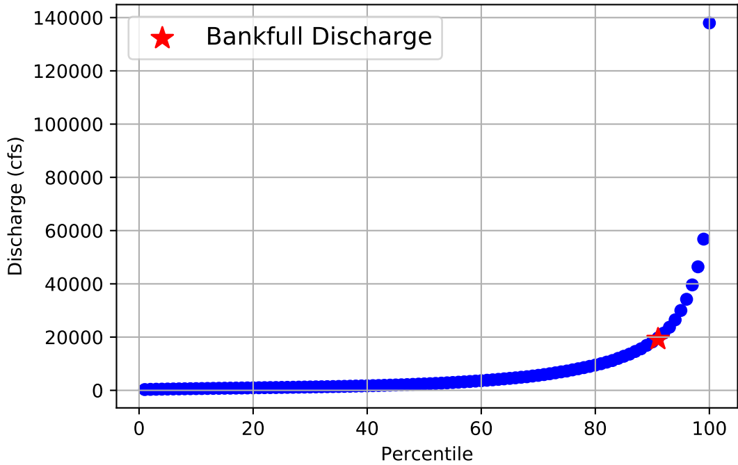
Flow Frequency Distribution for USGS Gage 08111500 from 1938 to 2020
