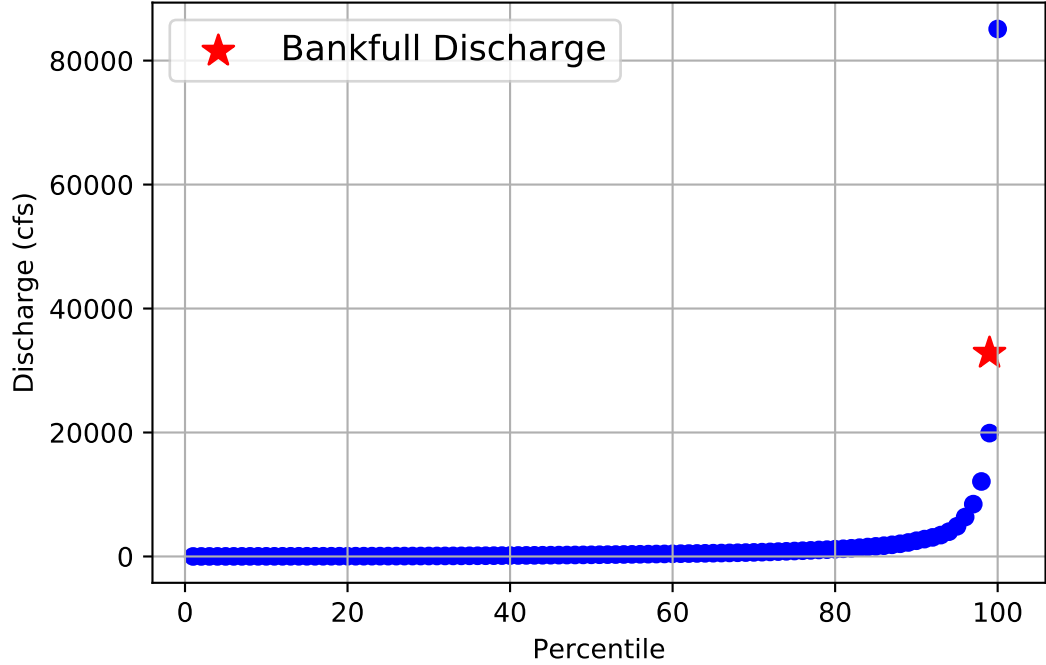
Flow Frequency Distribution for USGS Gage 08091000 from 1923 to 2020
