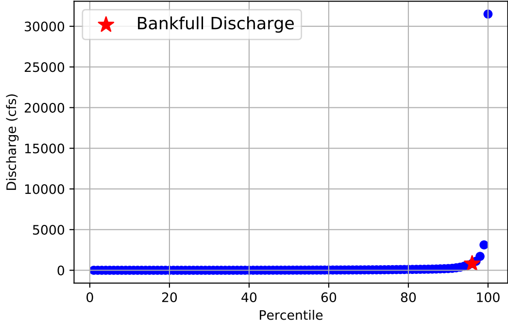
Flow Frequency Distribution for USGS Gage 08206600 from 1978 to 2020
