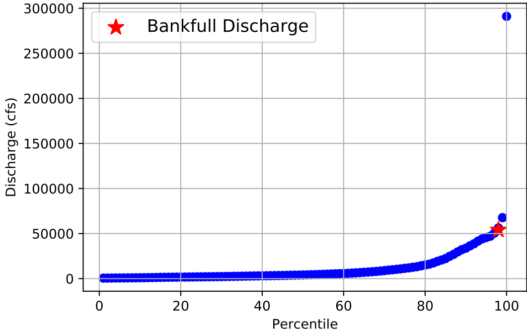
Flow Frequency Distribution for USGS Gage 07336820 from 2004 to 2020
