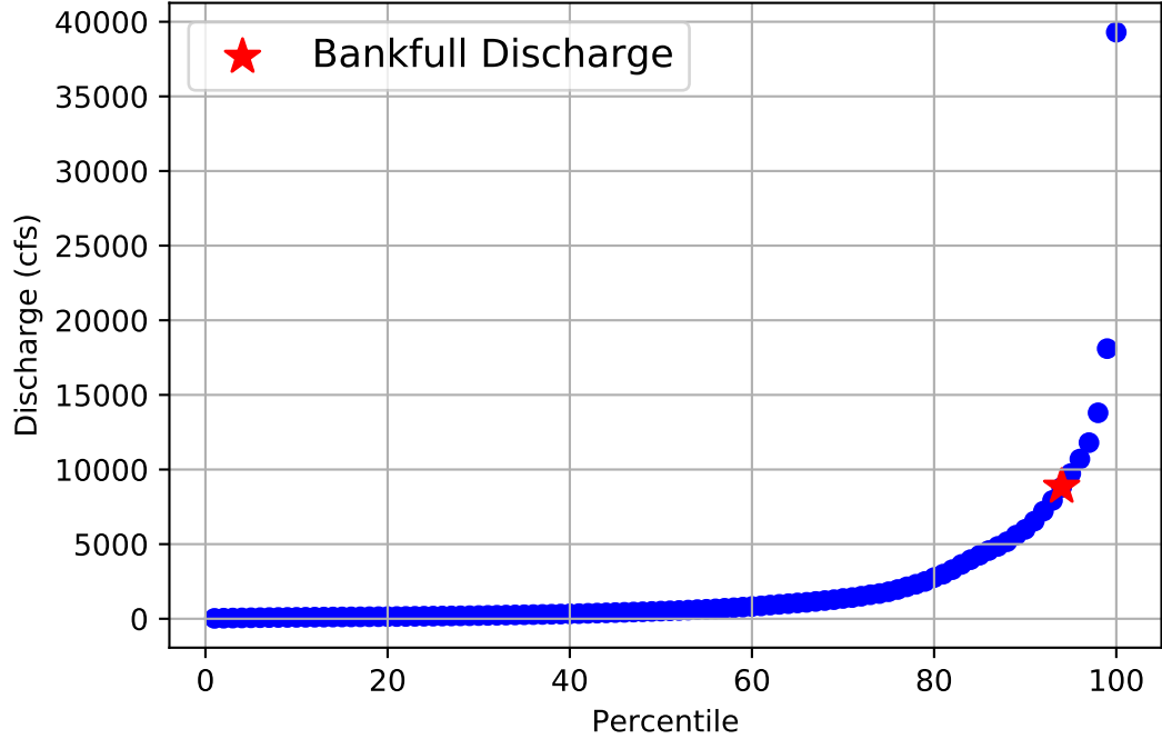
Flow Frequency Distribution for USGS Gage 08020900 from 1995 to 2020
