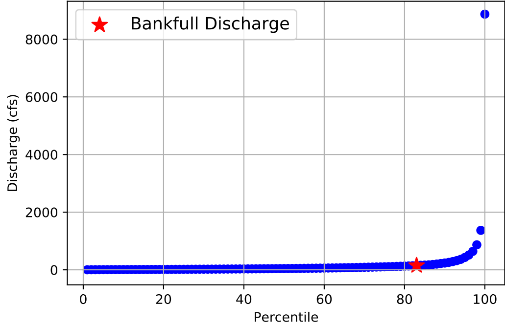
Flow Frequency Distribution for USGS Gage 08033900 from 1964 to 2020
