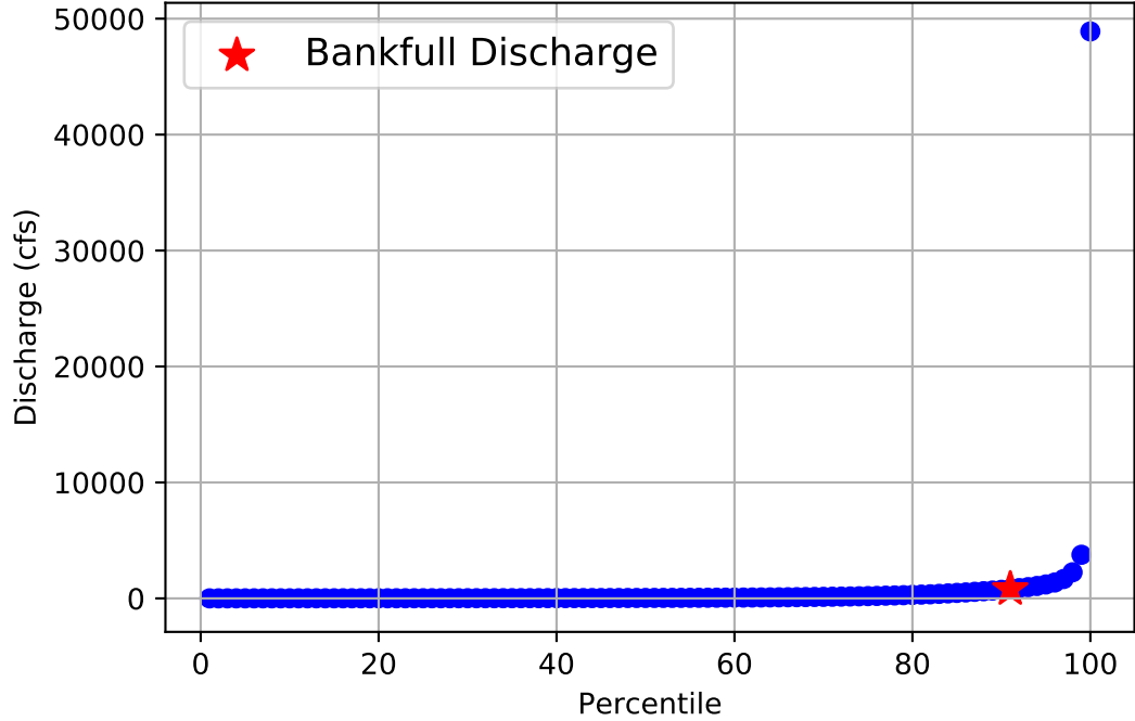
Flow Frequency Distribution for USGS Gage 07344500 from 1943 to 2020
