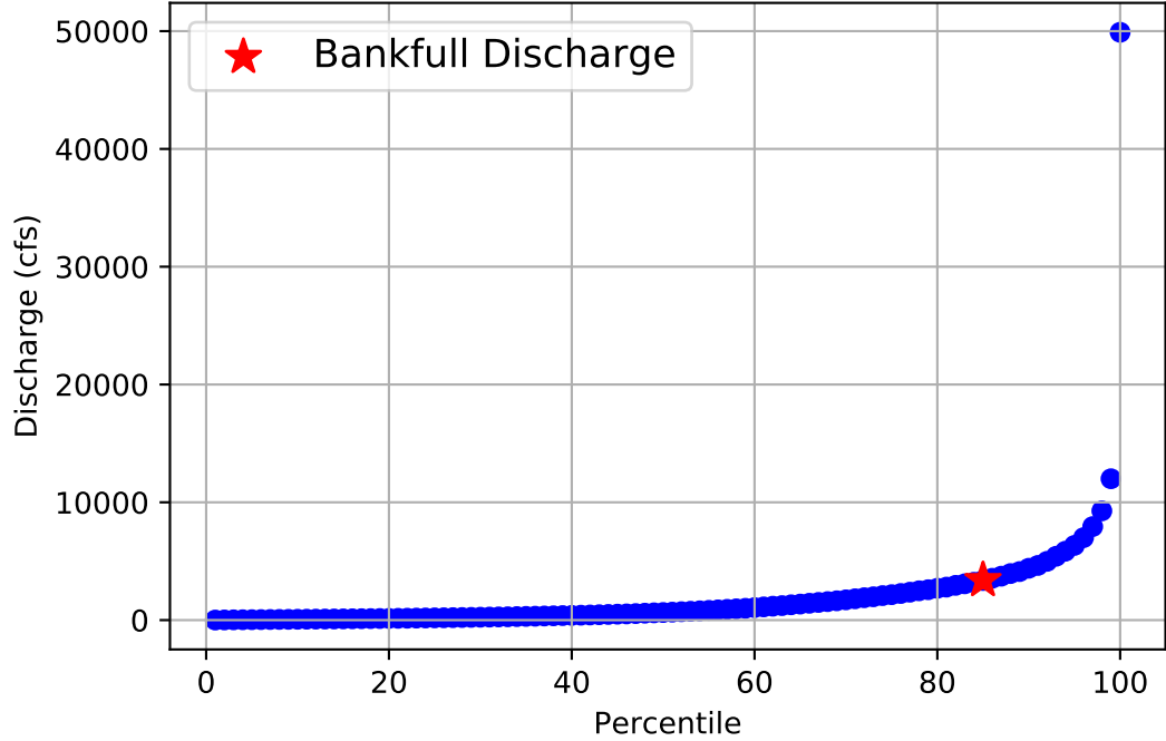
Flow Frequency Distribution for USGS Gage 08033000 from 1923 to 2020
