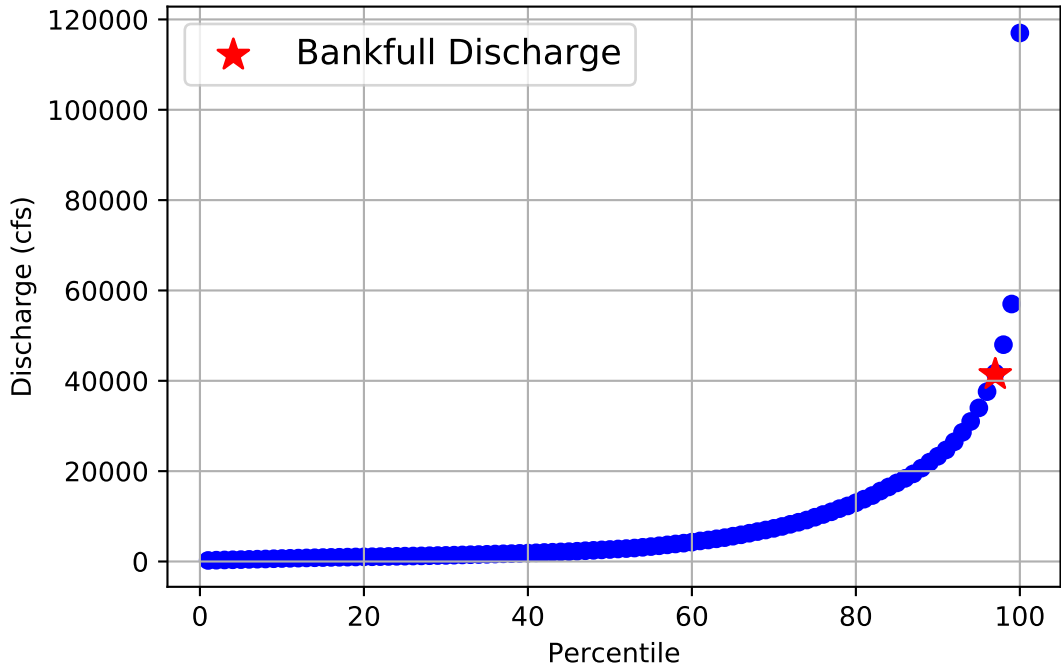
Flow Frequency Distribution for USGS Gage 08066500 from 1924 to 2020
