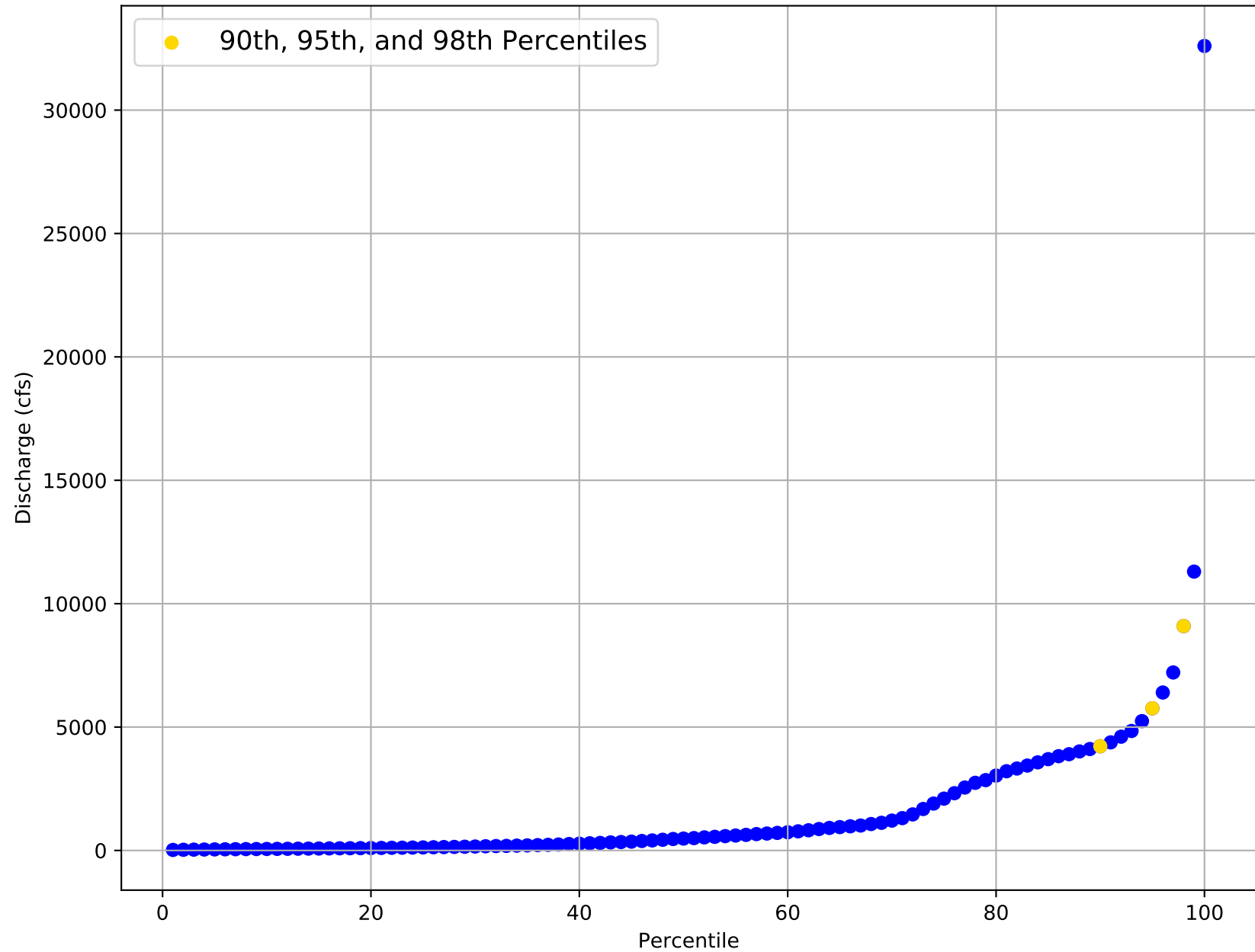
Flow Frequency Distribution for USGS Gage 07346080 from 2006 to 2019
