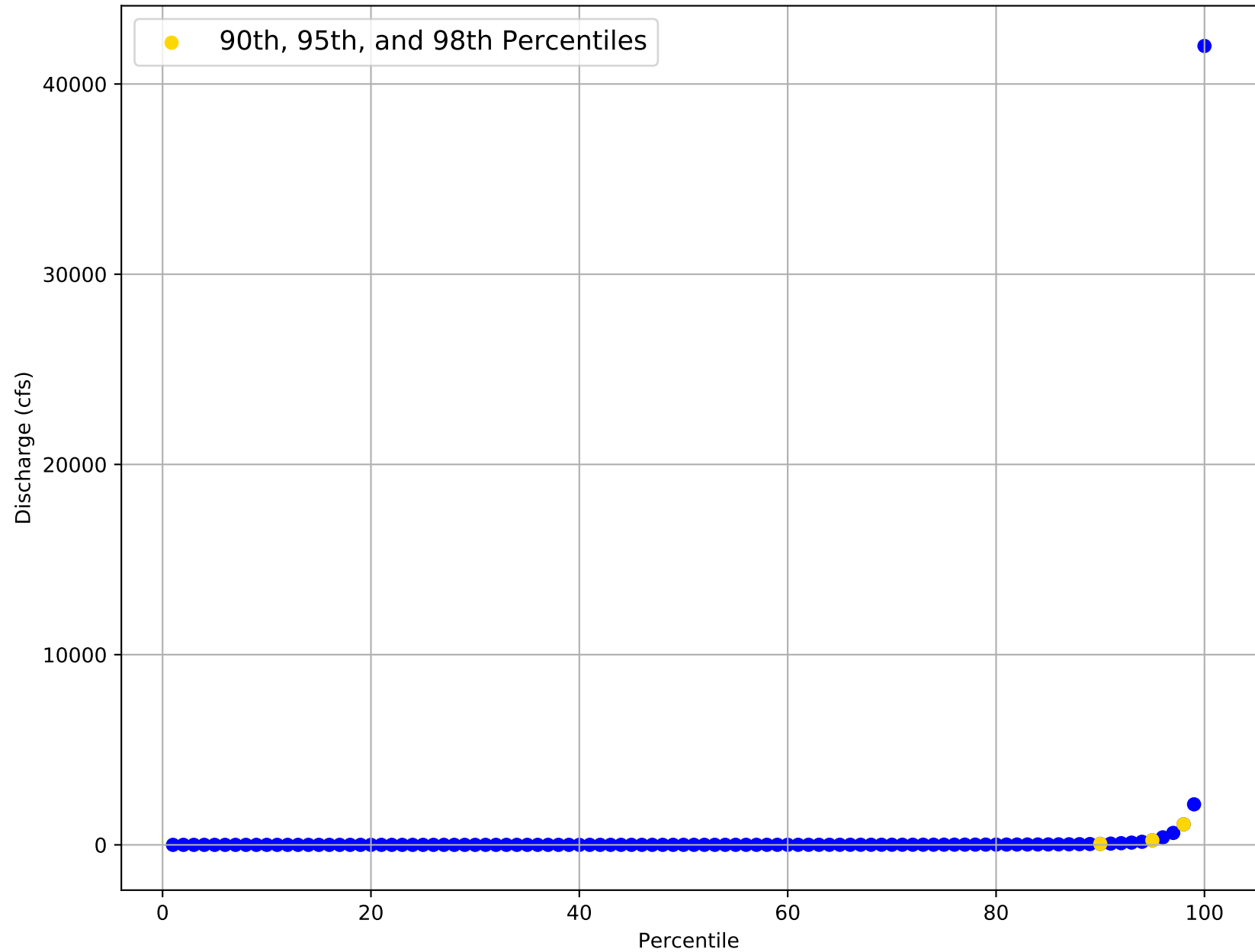
Flow Frequency Distribution for USGS Gage 08064700 from 1968 to 2020
