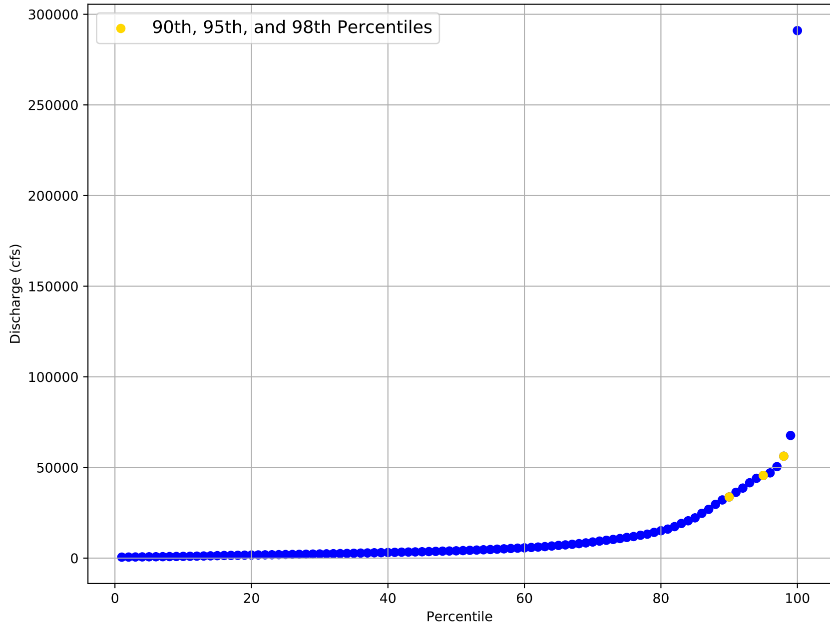
Flow Frequency Distribution for USGS Gage 07336820 from 2004 to 2020
