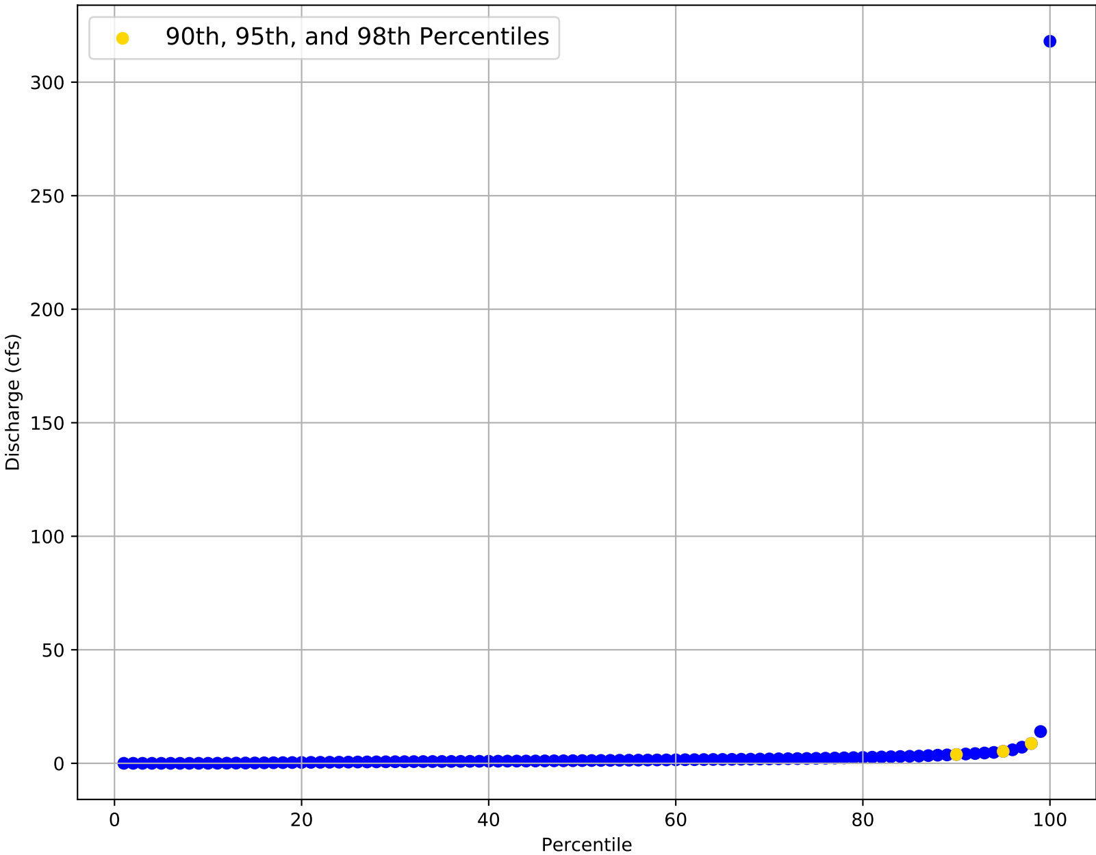
Flow Frequency Distribution for USGS Gage 07299890 from 1997 to 2020
