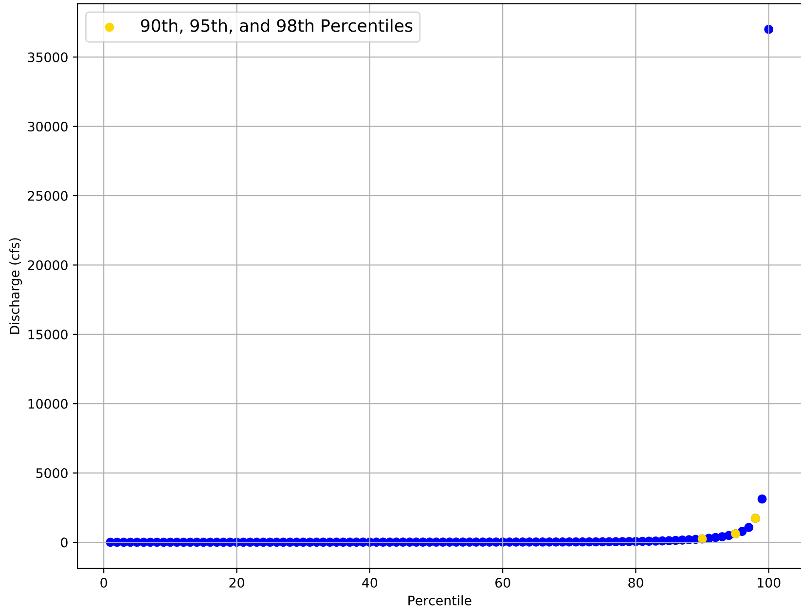
Flow Frequency Distribution for USGS Gage 08143600 from 1967 to 2020
