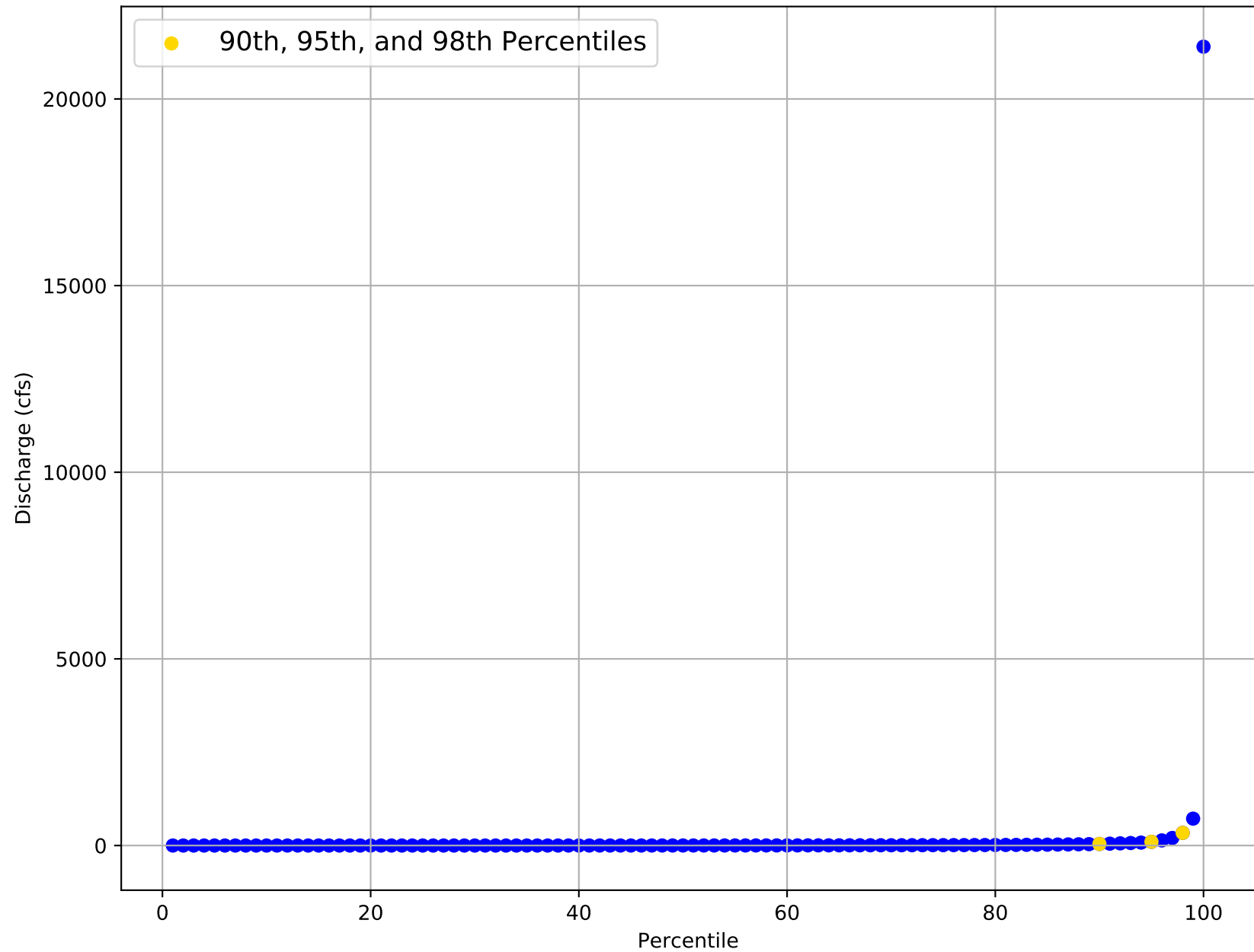
Flow Frequency Distribution for USGS Gage 08127000 from 1932 to 2020
