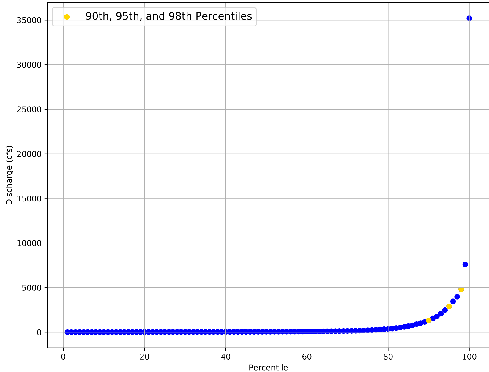
Flow Frequency Distribution for USGS Gage 08048543 from 1976 to 2020
