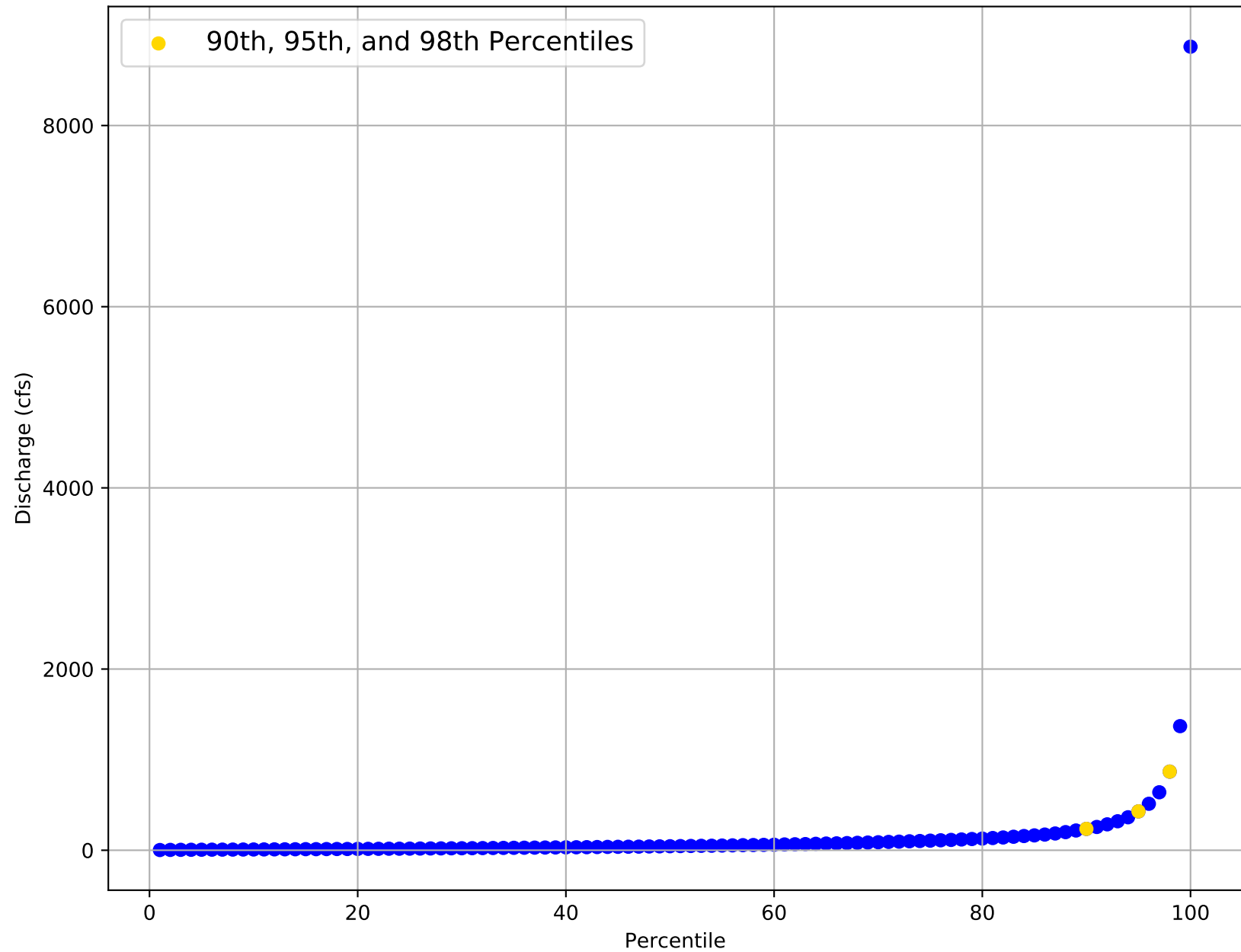
Flow Frequency Distribution for USGS Gage 08033900 from 1964 to 2020
