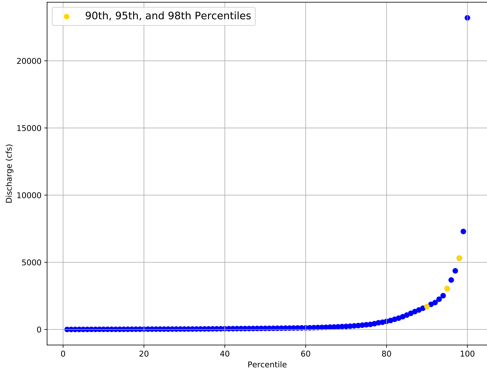
Flow Frequency Distribution for USGS Gage 08111010 from 1977 to 1985
