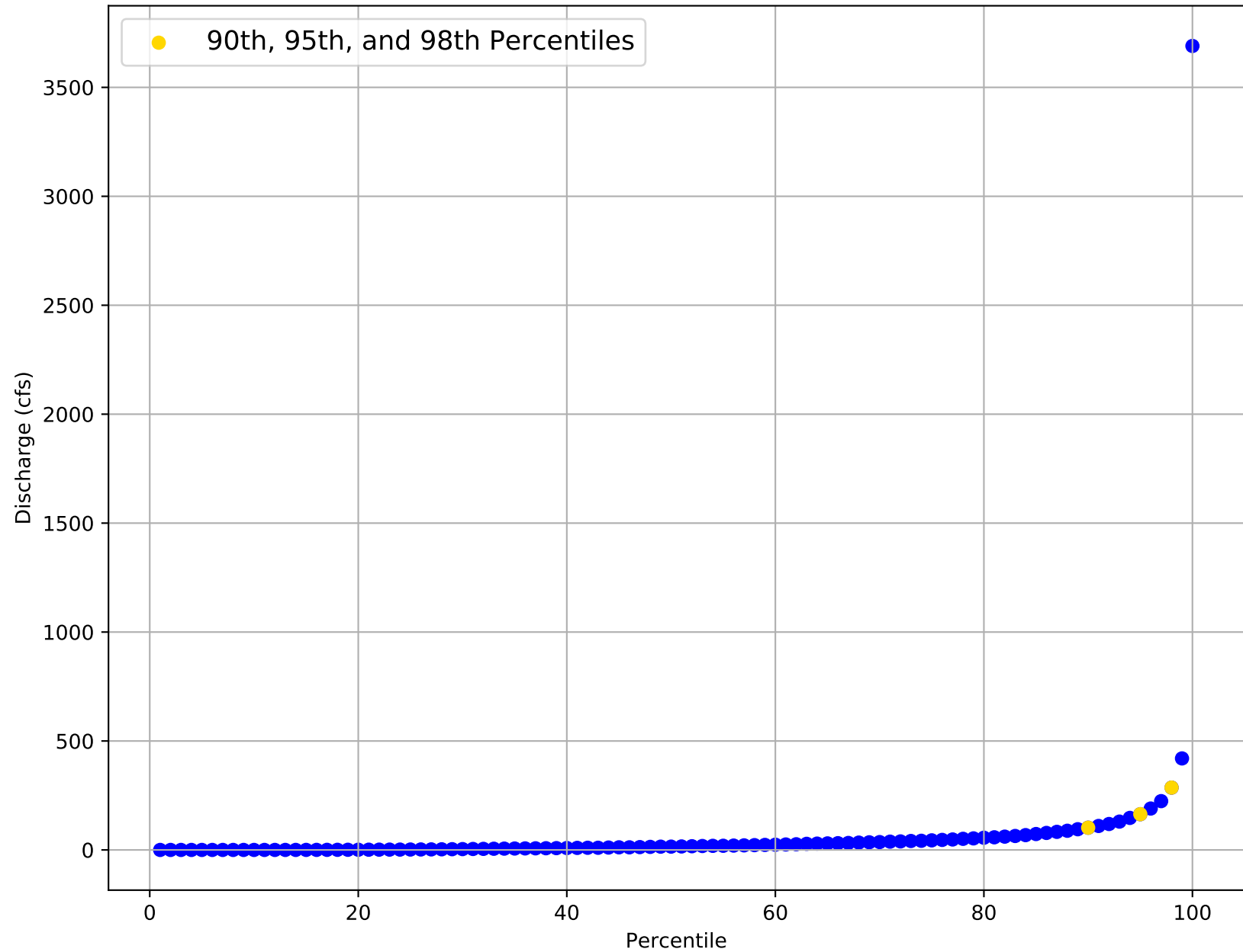
Flow Frequency Distribution for USGS Gage 07346140 from 1964 to 1991
