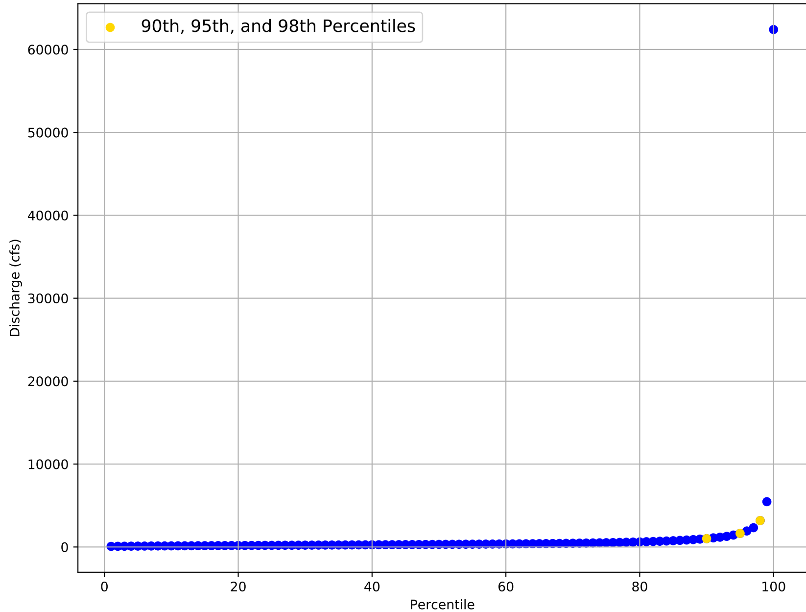
Flow Frequency Distribution for USGS Gage 08181800 from 1962 to 2020
