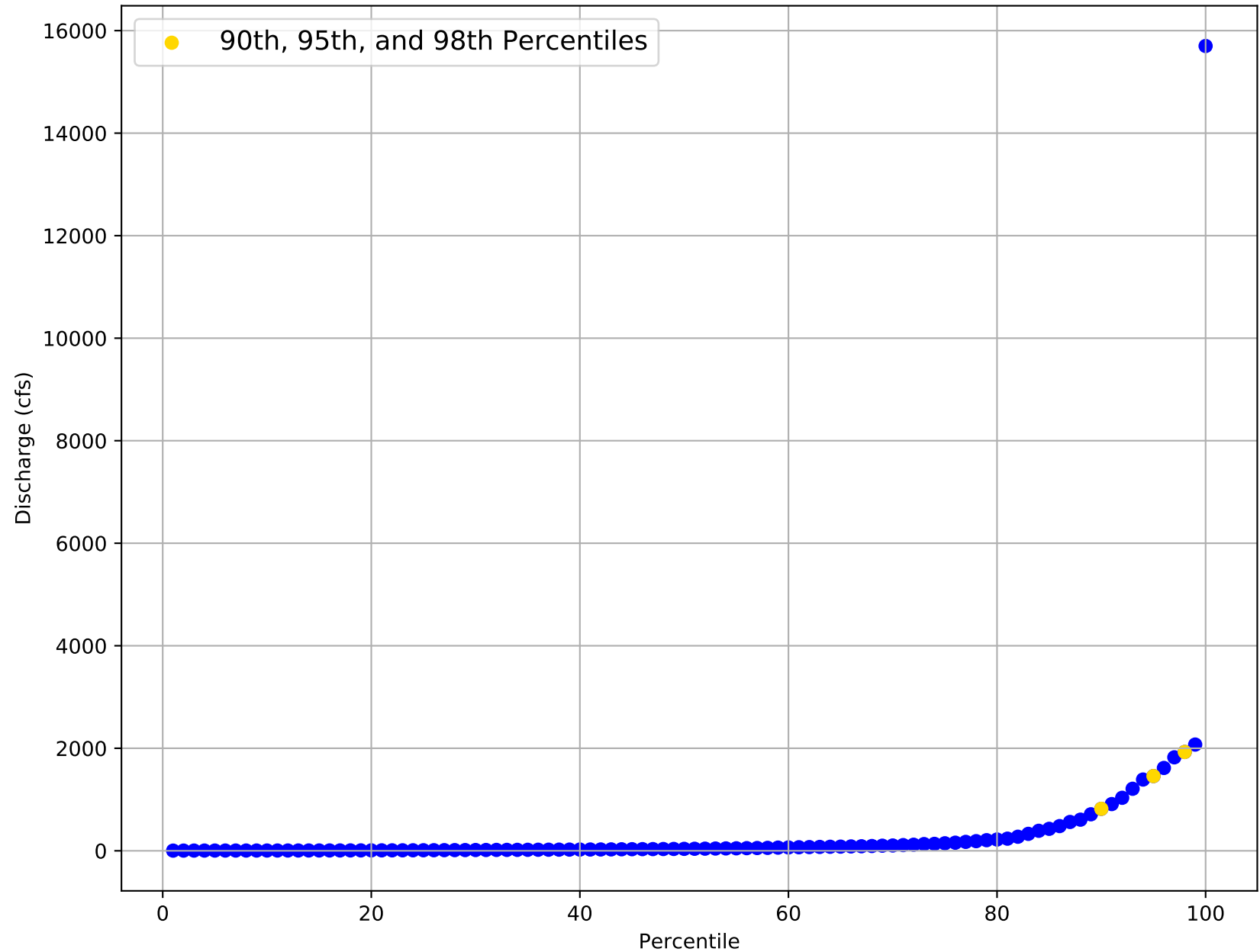
Flow Frequency Distribution for USGS Gage 08067900 from 2002 to 2005
