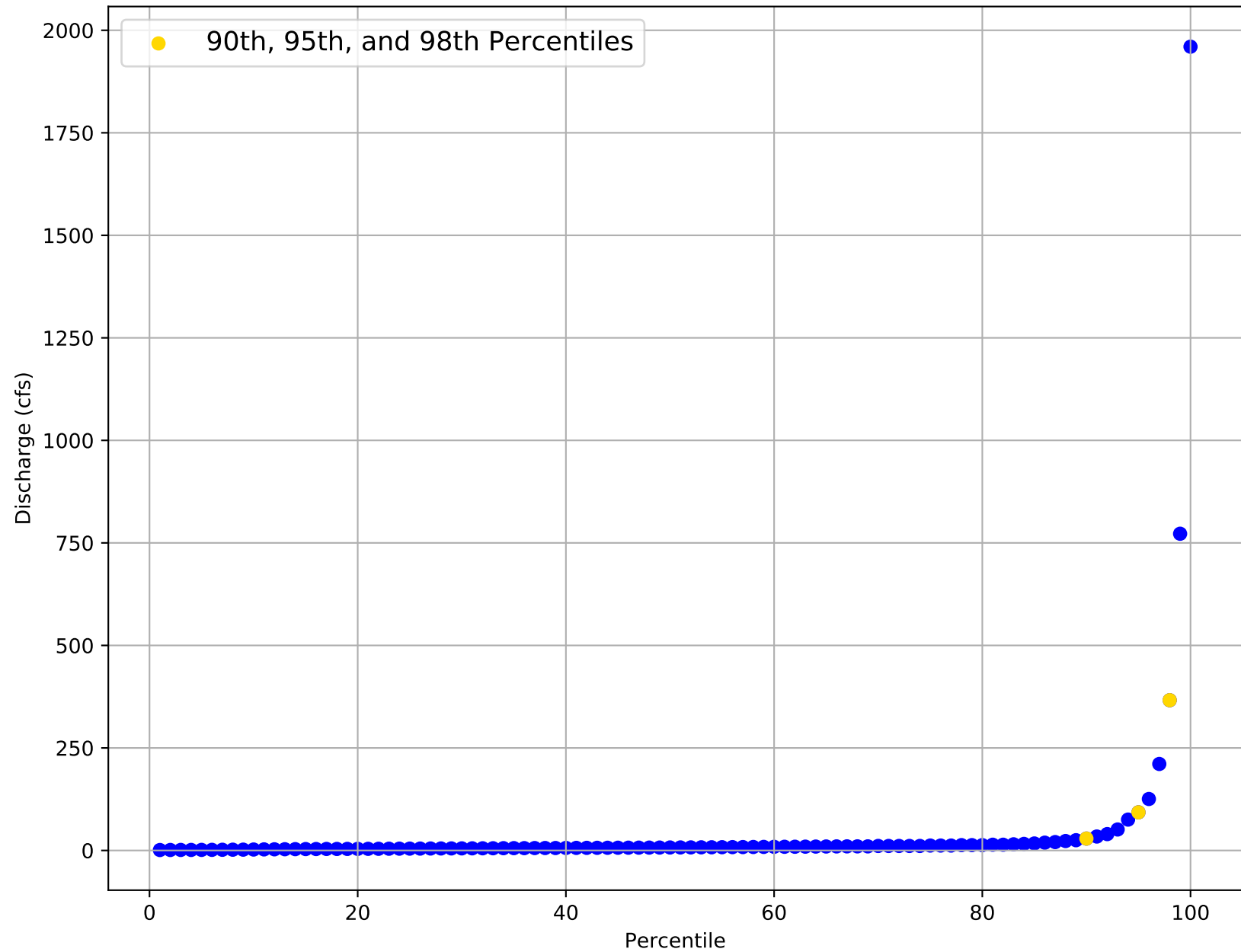
Flow Frequency Distribution for USGS Gage 07312130 from 1996 to 2002
