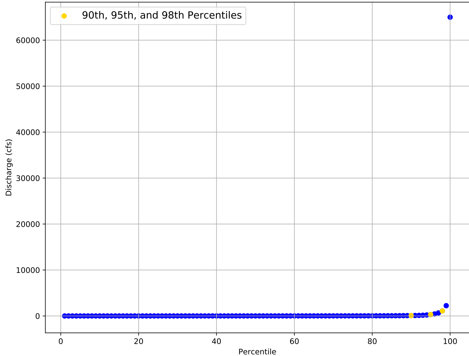
Flow Frequency Distribution for USGS Gage 08208000 from 1932 to 2020
