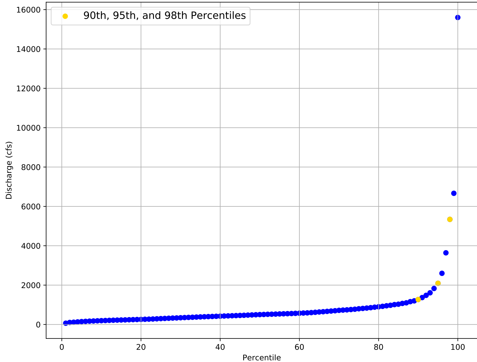
Flow Frequency Distribution for USGS Gage 08169792 from 2005 to 2020
