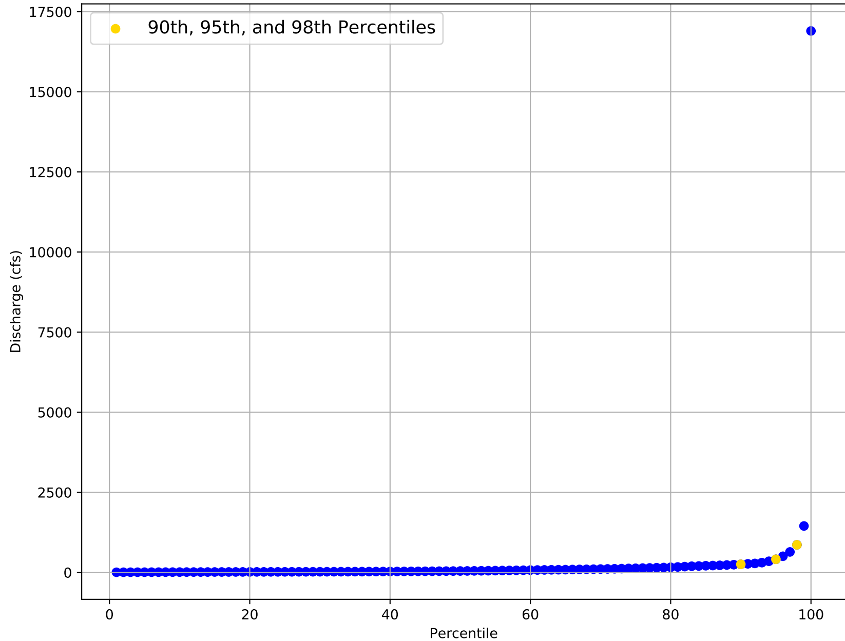
Flow Frequency Distribution for USGS Gage 08178565 from 1986 to 2020
