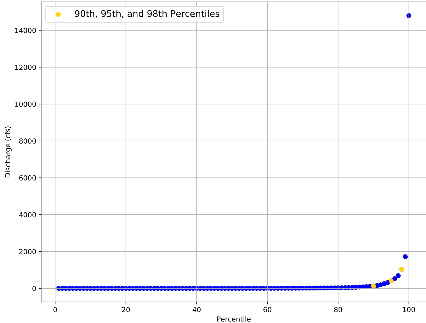
Flow Frequency Distribution for USGS Gage 07336800 from 1962 to 1977
