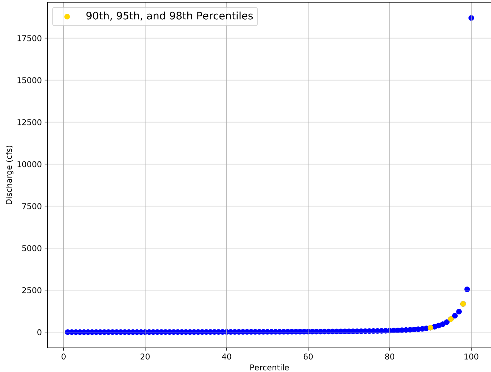
Flow Frequency Distribution for USGS Gage 08164503 from 1977 to 2020
