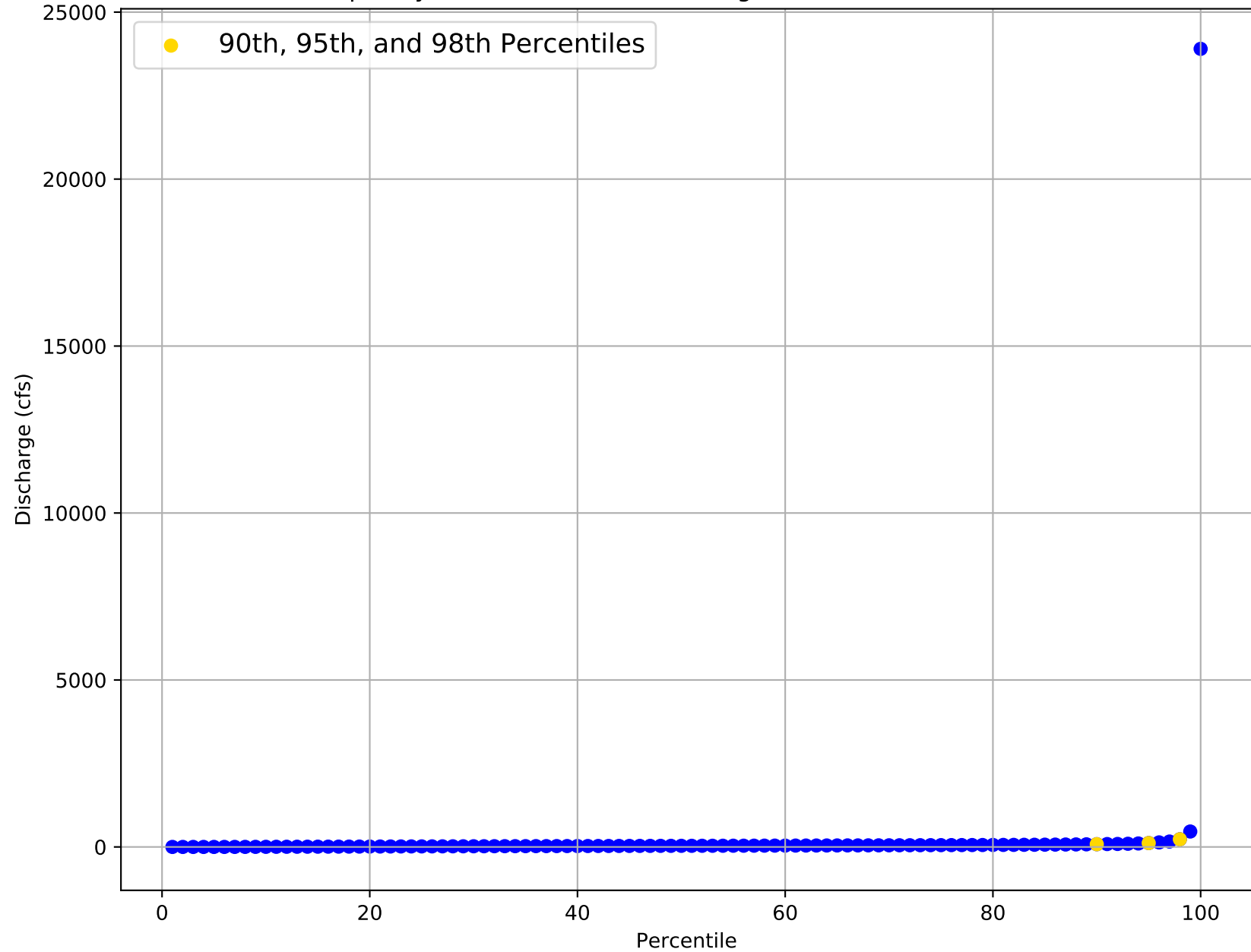
Flow Frequency Distribution for USGS Gage 08144600 from 1979 to 2012
