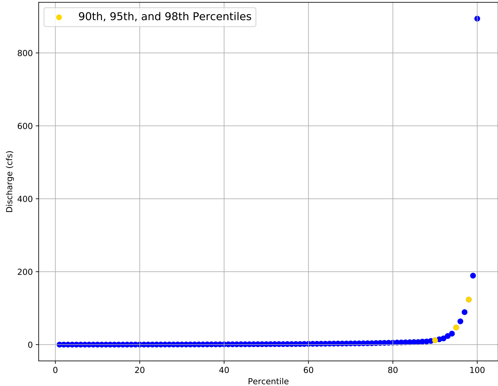
Flow Frequency Distribution for USGS Gage 08063003 from 1982 to 1984
