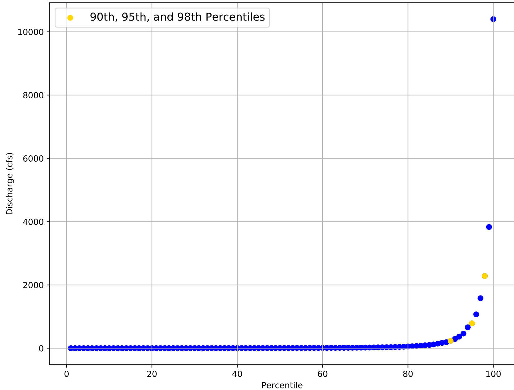
Flow Frequency Distribution for USGS Gage 08062895 from 2009 to 2020
