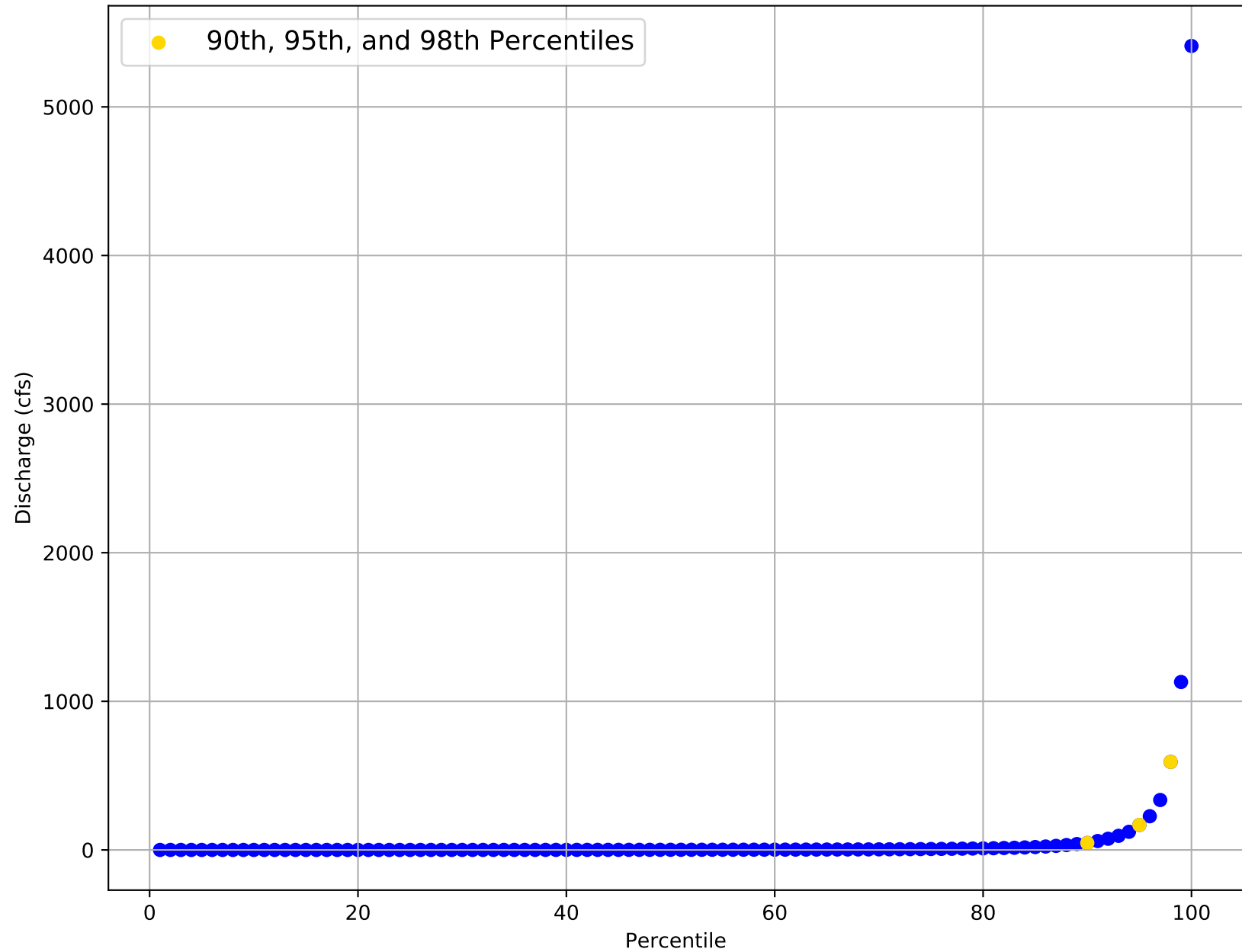
Flow Frequency Distribution for USGS Gage 08164504 from 1996 to 2020
