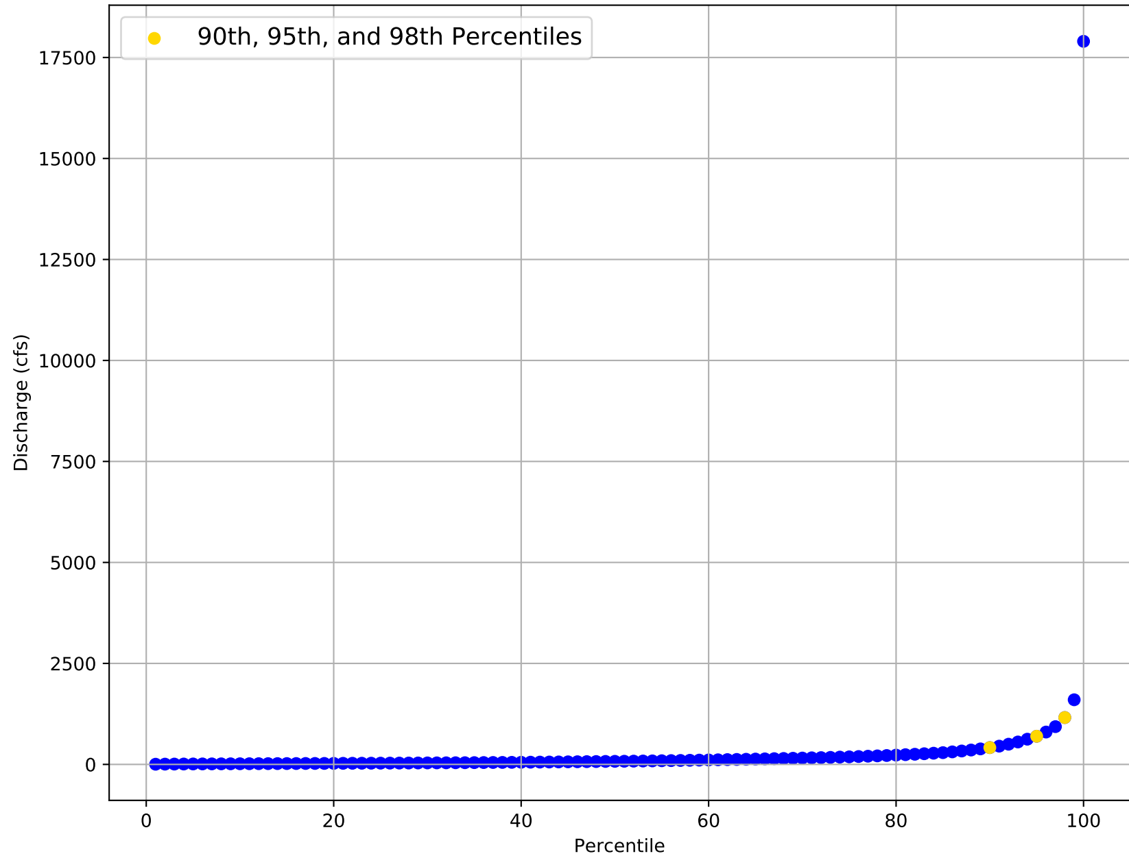
Flow Frequency Distribution for USGS Gage 08019500 from 1939 to 2020
