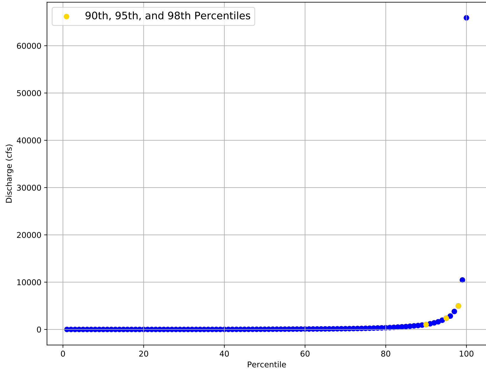
Flow Frequency Distribution for USGS Gage 08194600 from 1965 to 1977
