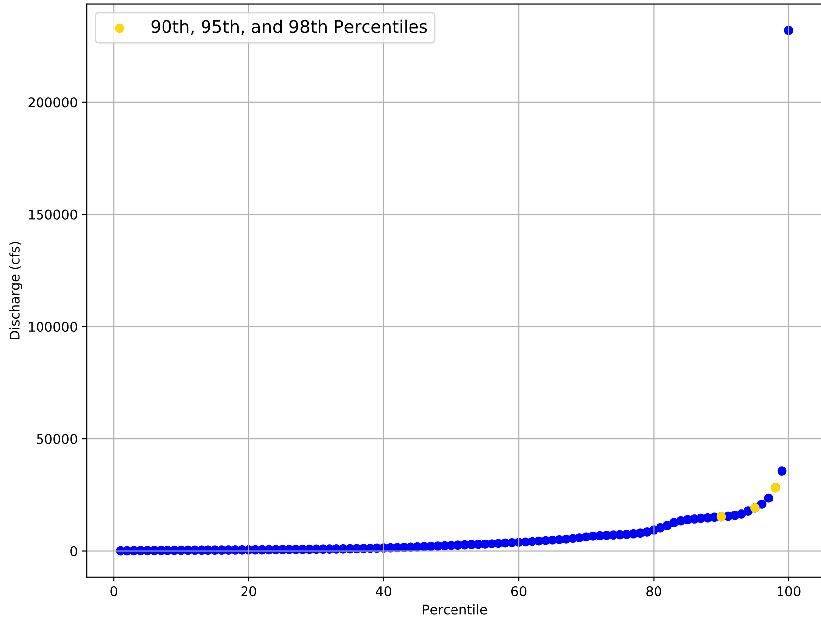
Flow Frequency Distribution for USGS Gage 08026000 from 1955 to 2020
