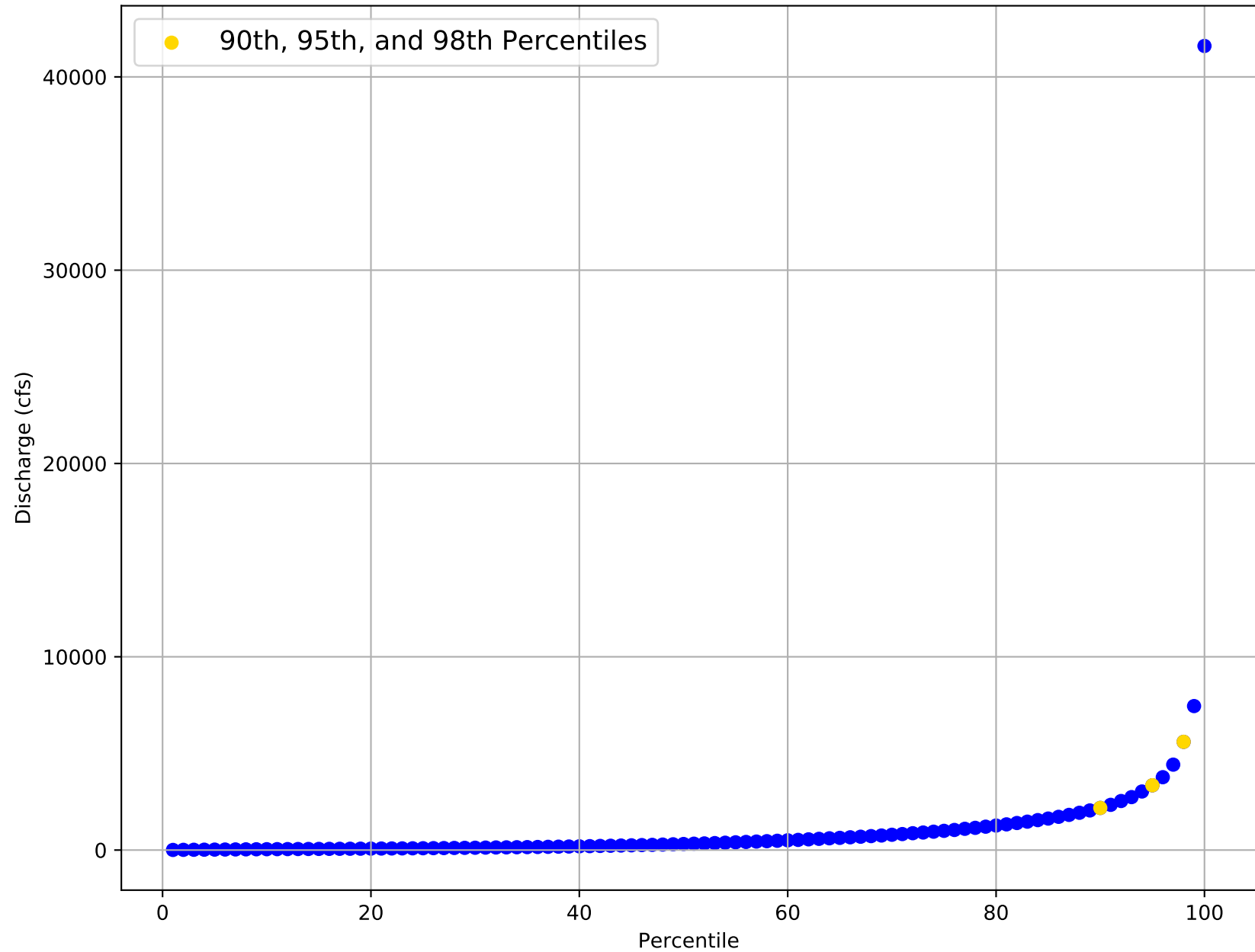
Flow Frequency Distribution for USGS Gage 08036500 from 1940 to 2020
