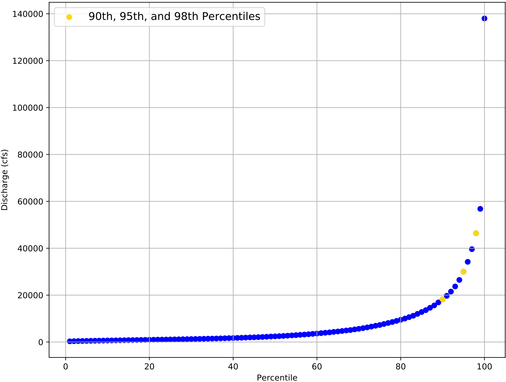
Flow Frequency Distribution for USGS Gage 08111500 from 1938 to 2020
