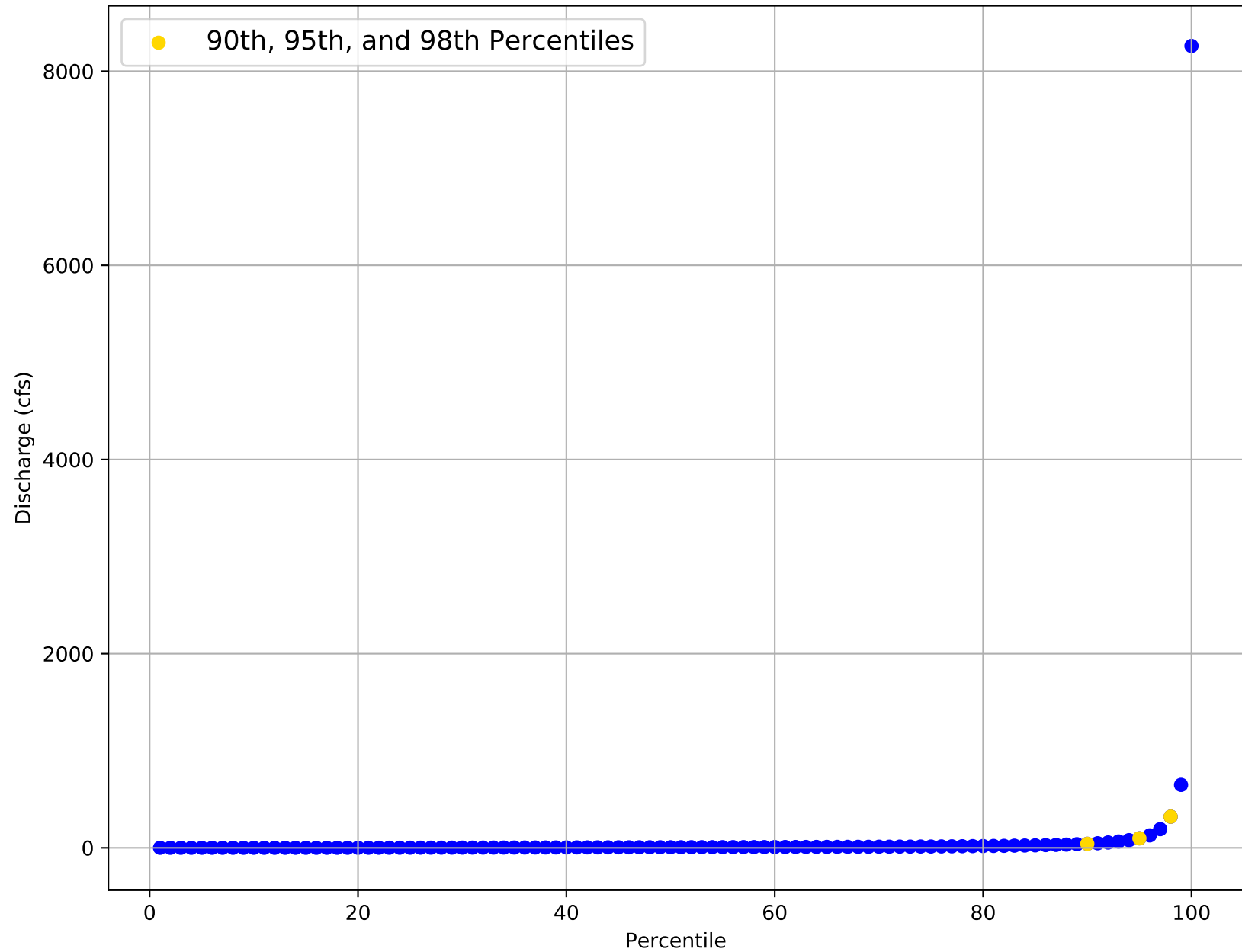
Flow Frequency Distribution for USGS Gage 07311800 from 1959 to 2020
