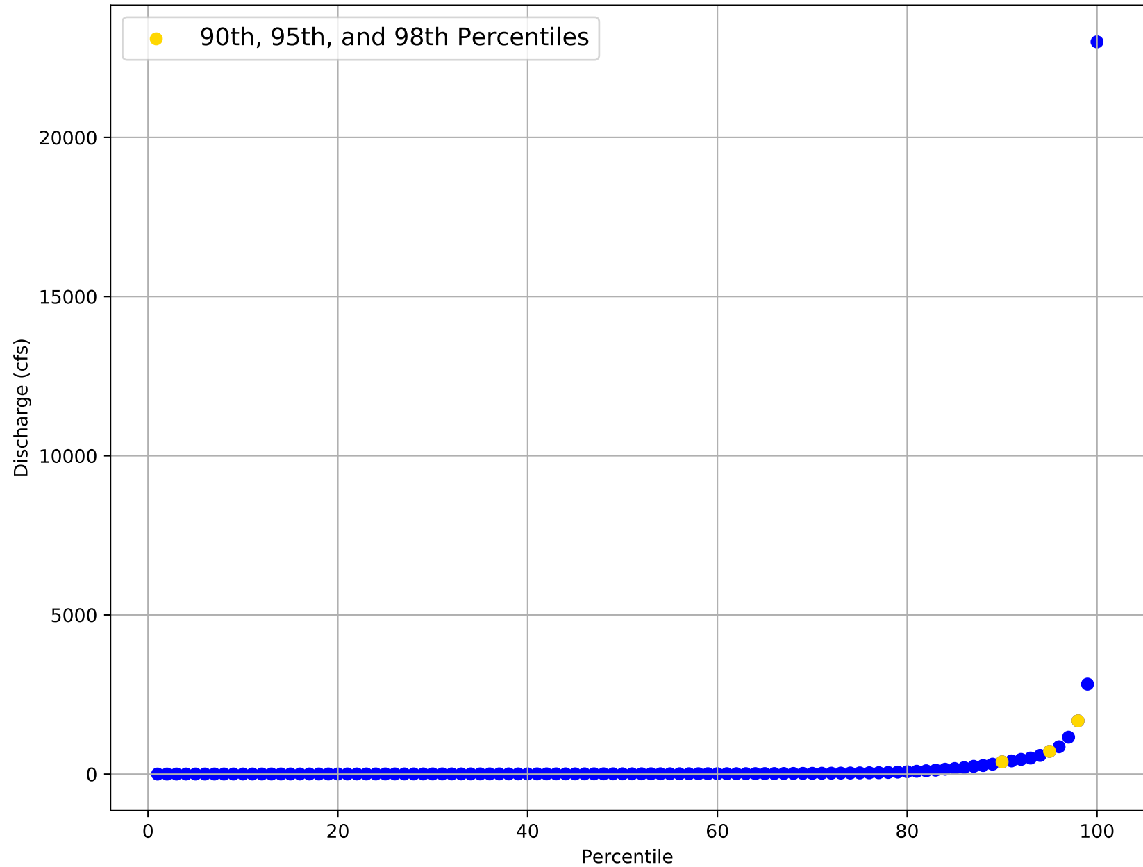
Flow Frequency Distribution for USGS Gage 07344493 from 2004 to 2020
