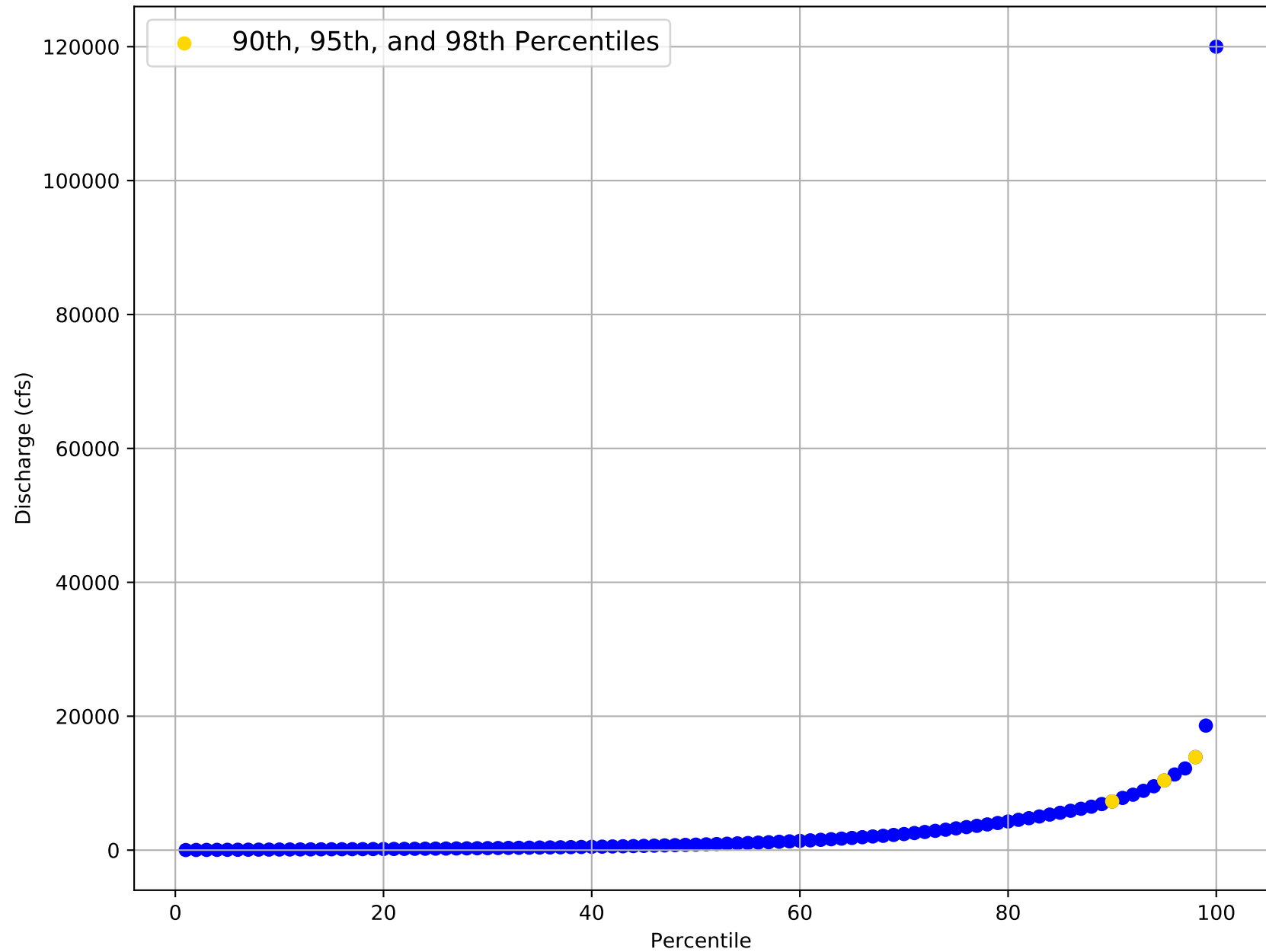
Flow Frequency Distribution for USGS Gage 08022040 from 1938 to 2020
