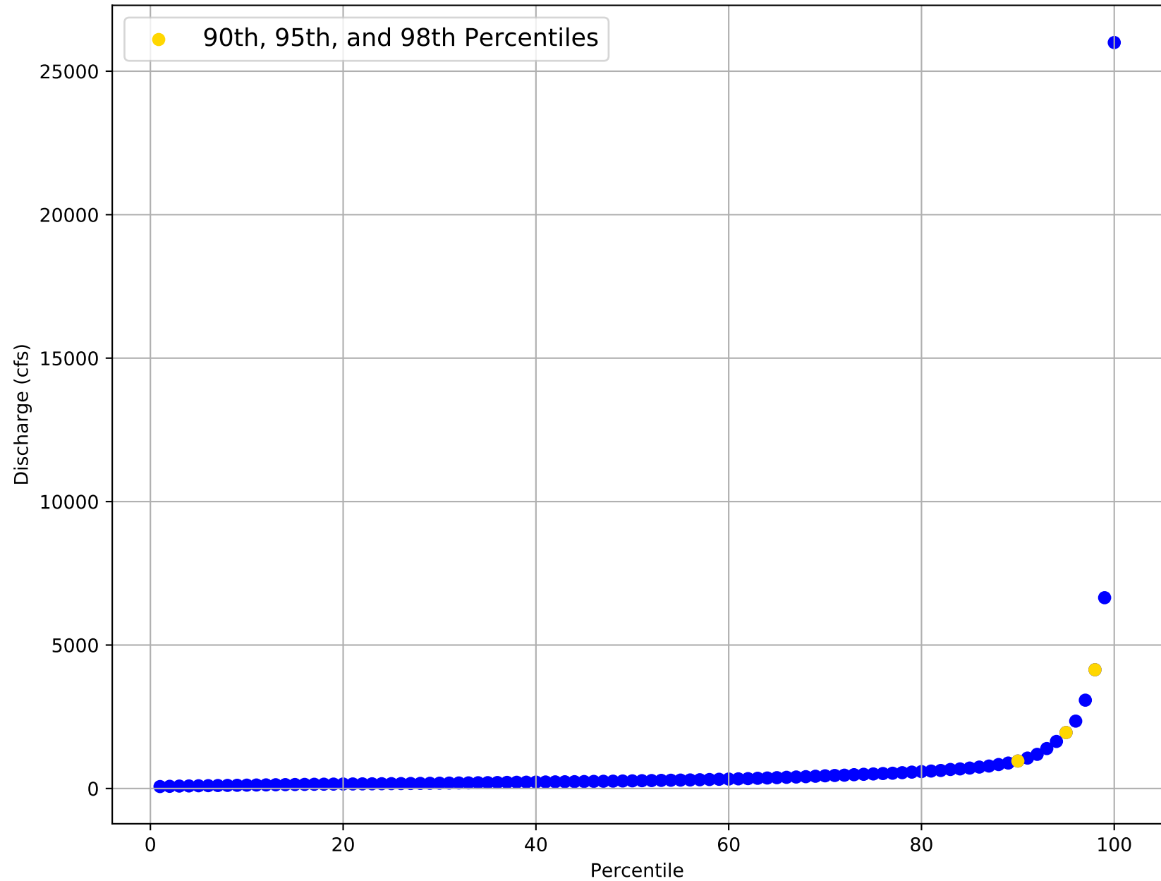
Flow Frequency Distribution for USGS Gage 08183200 from 2006 to 2020
