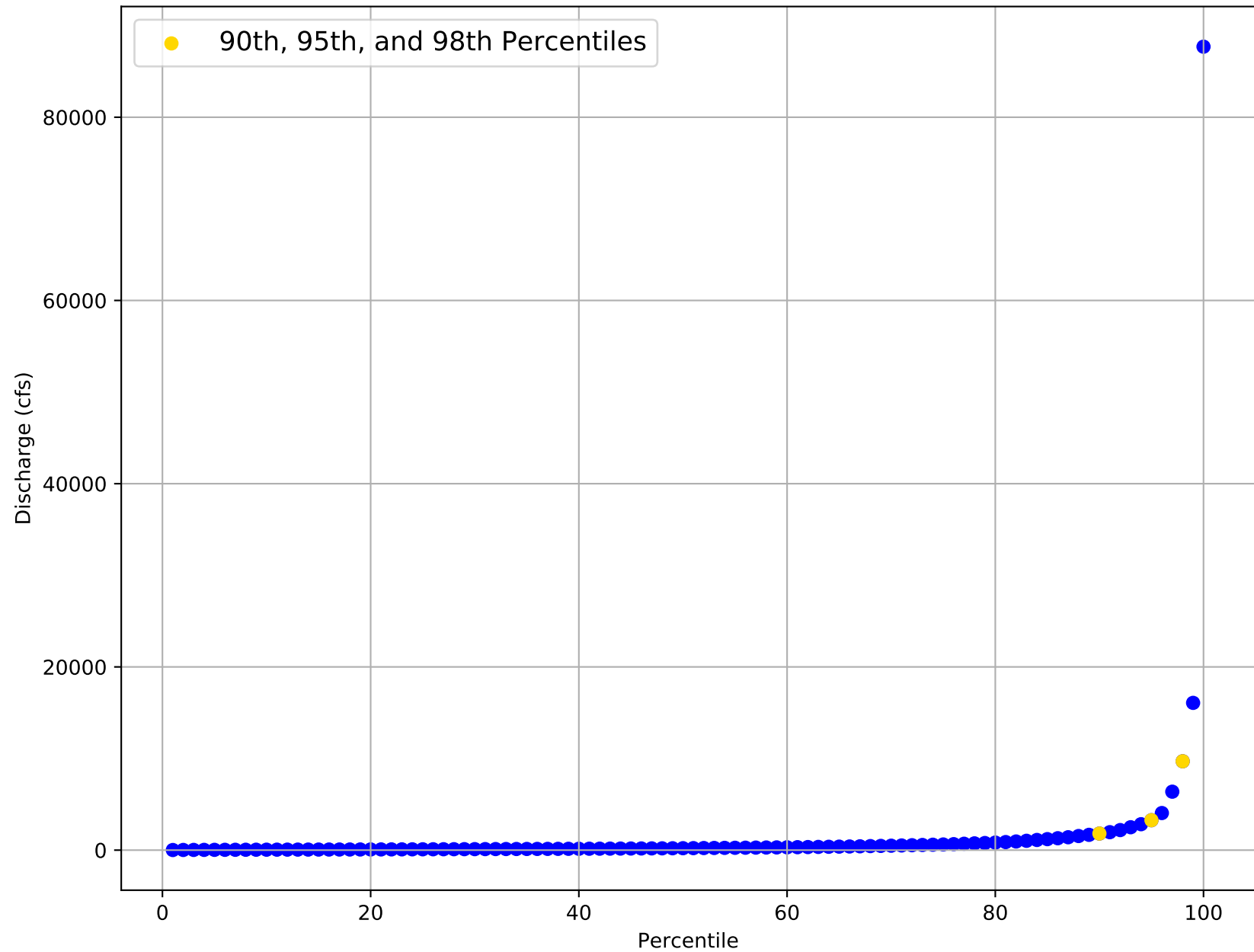
Flow Frequency Distribution for USGS Gage 08090800 from 1968 to 2020
