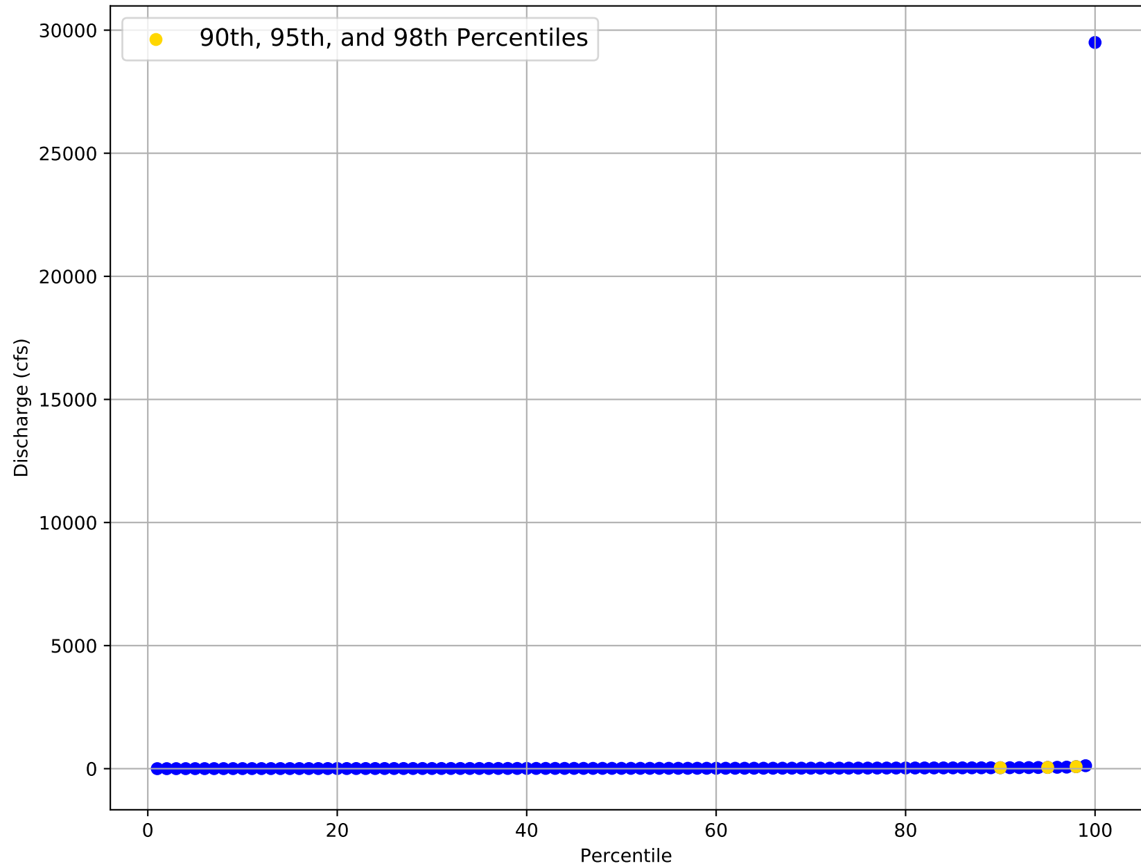
Flow Frequency Distribution for USGS Gage 08128000 from 1930 to 2020
