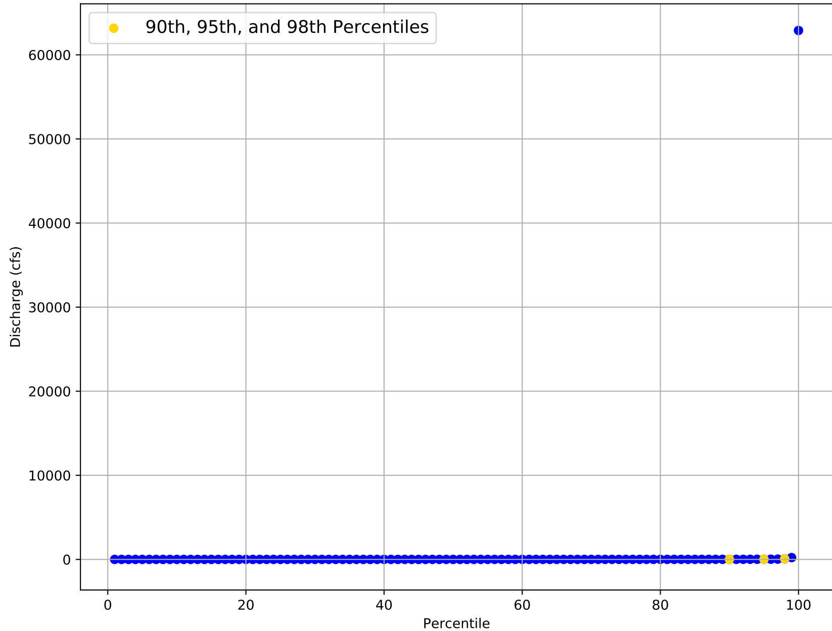
Flow Frequency Distribution for USGS Gage 08134000 from 1924 to 2020
