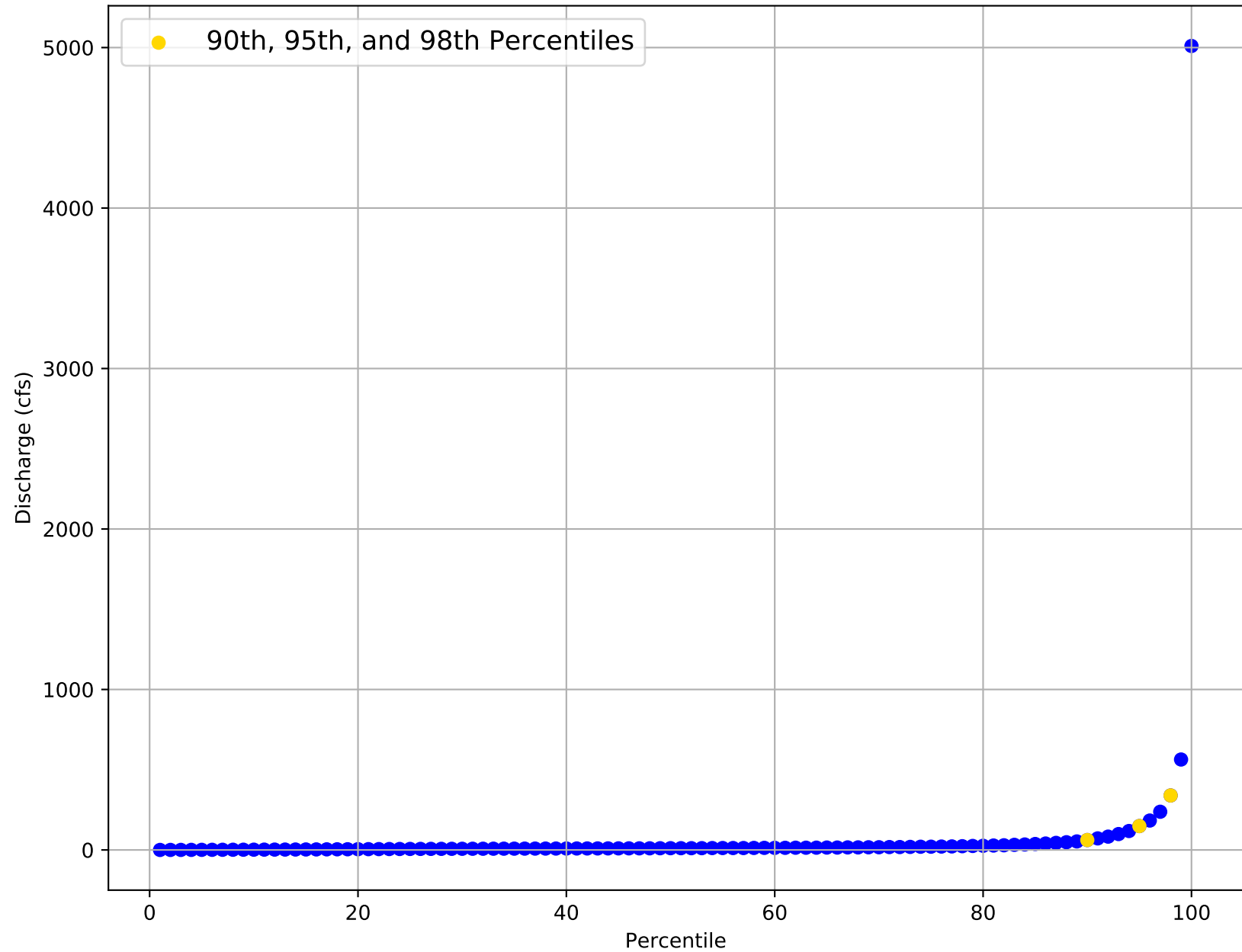
Flow Frequency Distribution for USGS Gage 08076500 from 1952 to 2020
