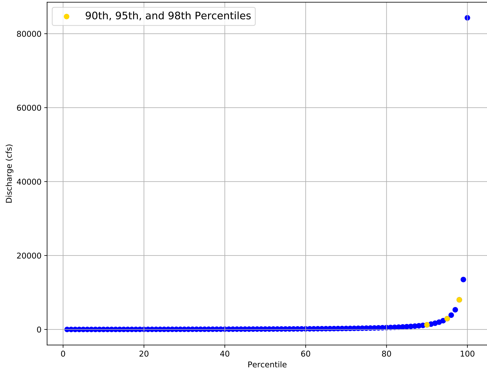
Flow Frequency Distribution for USGS Gage 08088000 from 1938 to 2020
