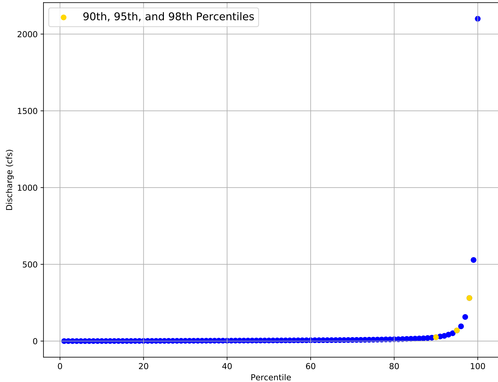
Flow Frequency Distribution for USGS Gage 07344482 from 1974 to 1991
