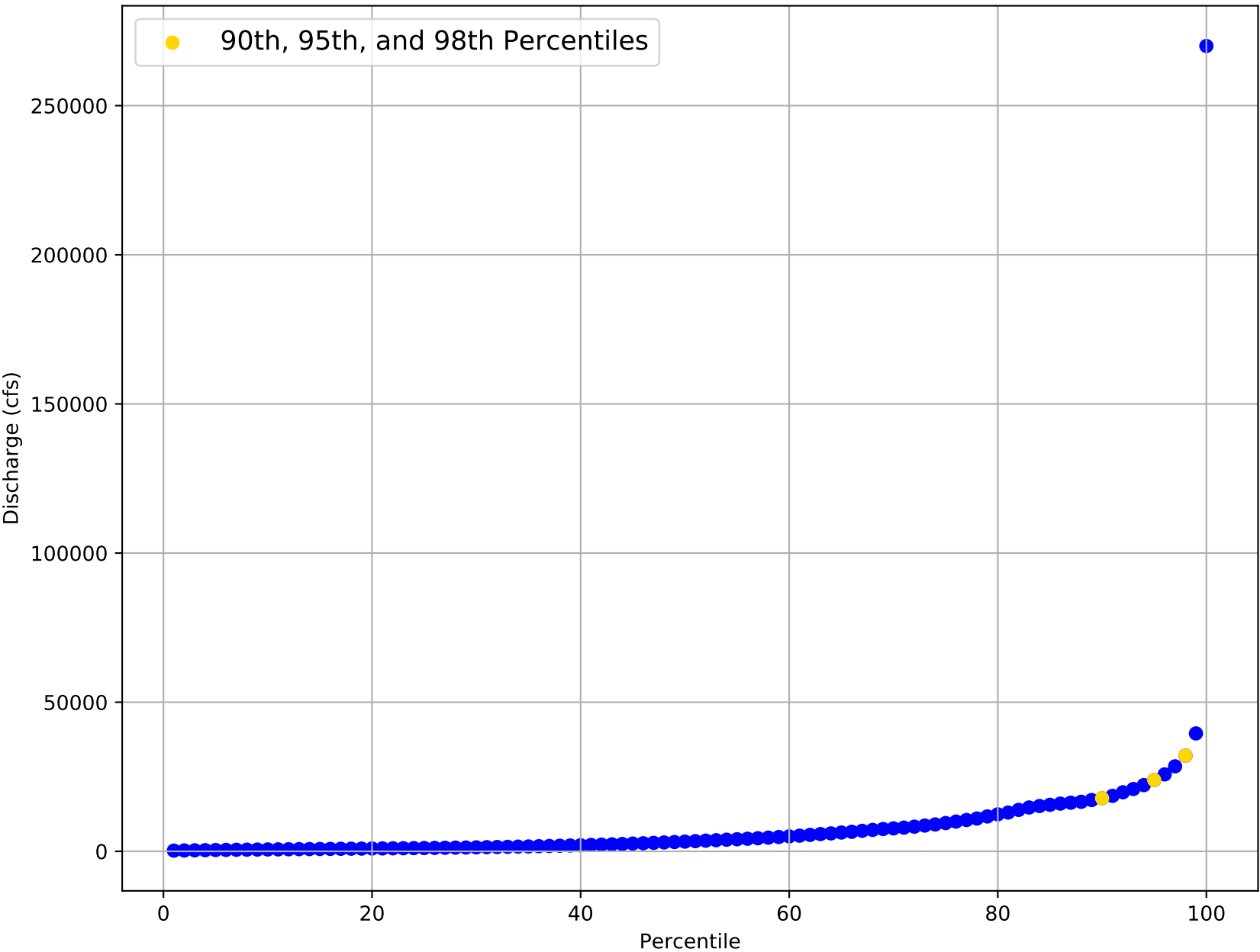
Flow Frequency Distribution for USGS Gage 08028500 from 1923 to 2020
