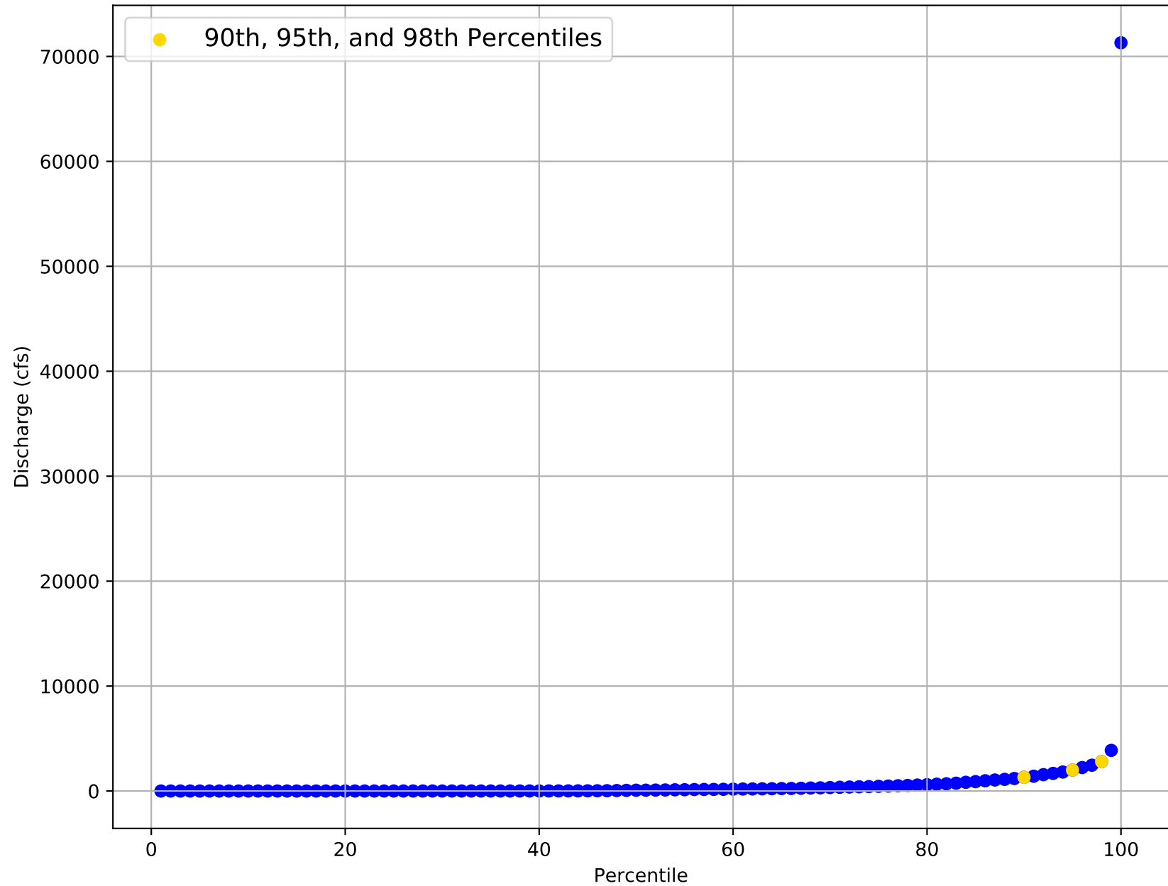
Flow Frequency Distribution for USGS Gage 08067650 from 1973 to 2020
