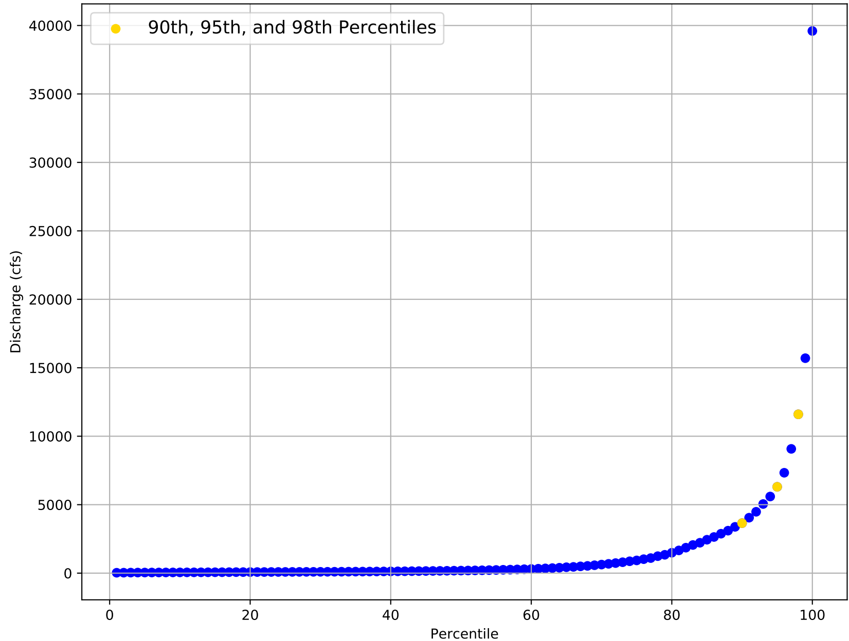
Flow Frequency Distribution for USGS Gage 08019200 from 1997 to 2020
