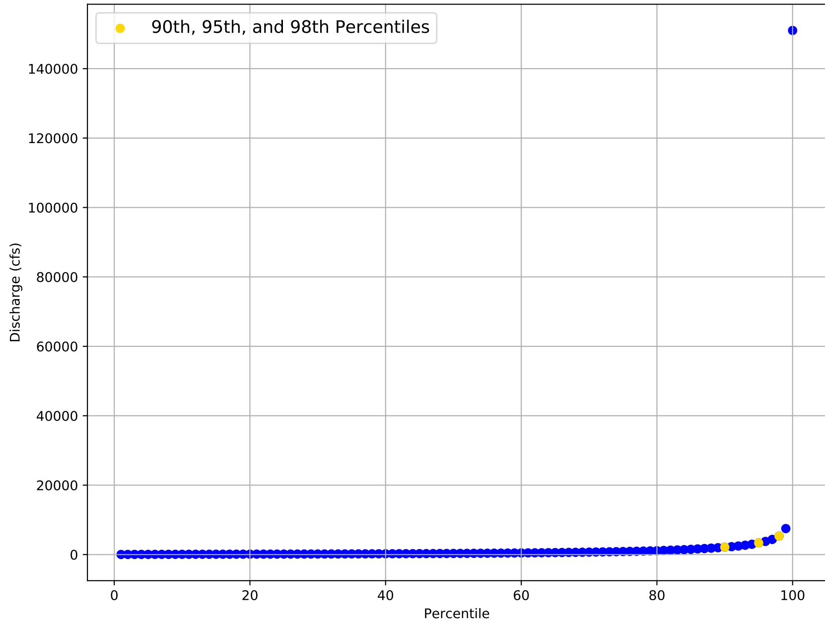
Flow Frequency Distribution for USGS Gage 08041500 from 1924 to 2020
