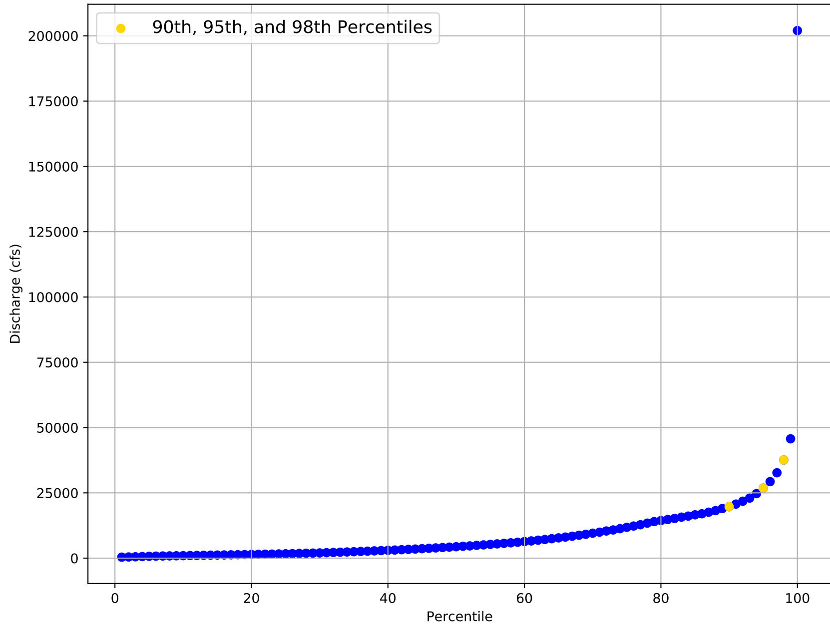
Flow Frequency Distribution for USGS Gage 08030500 from 1924 to 2020
