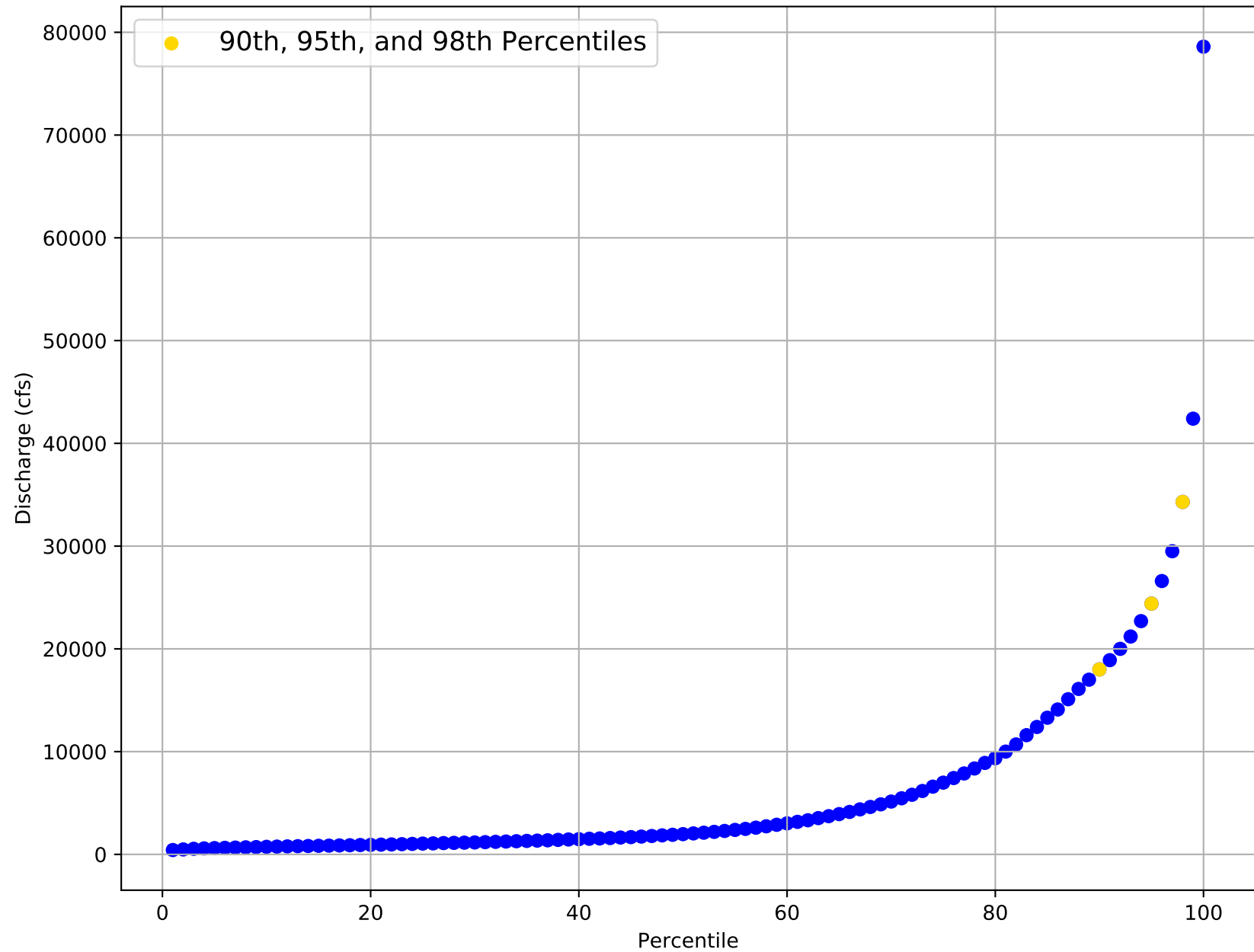
Flow Frequency Distribution for USGS Gage 08065350 from 1964 to 2020
