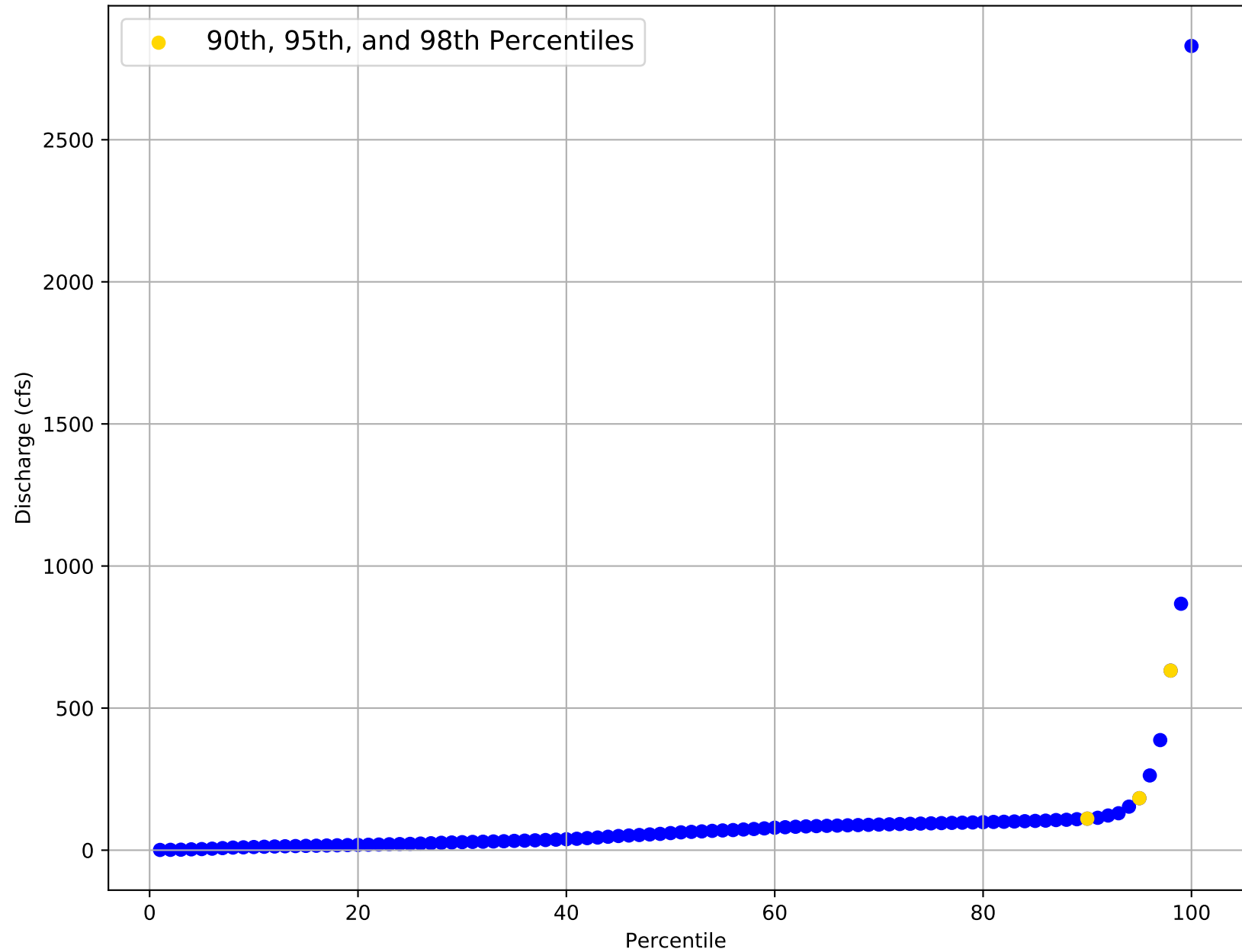
Flow Frequency Distribution for USGS Gage 08052745 from 2004 to 2020
