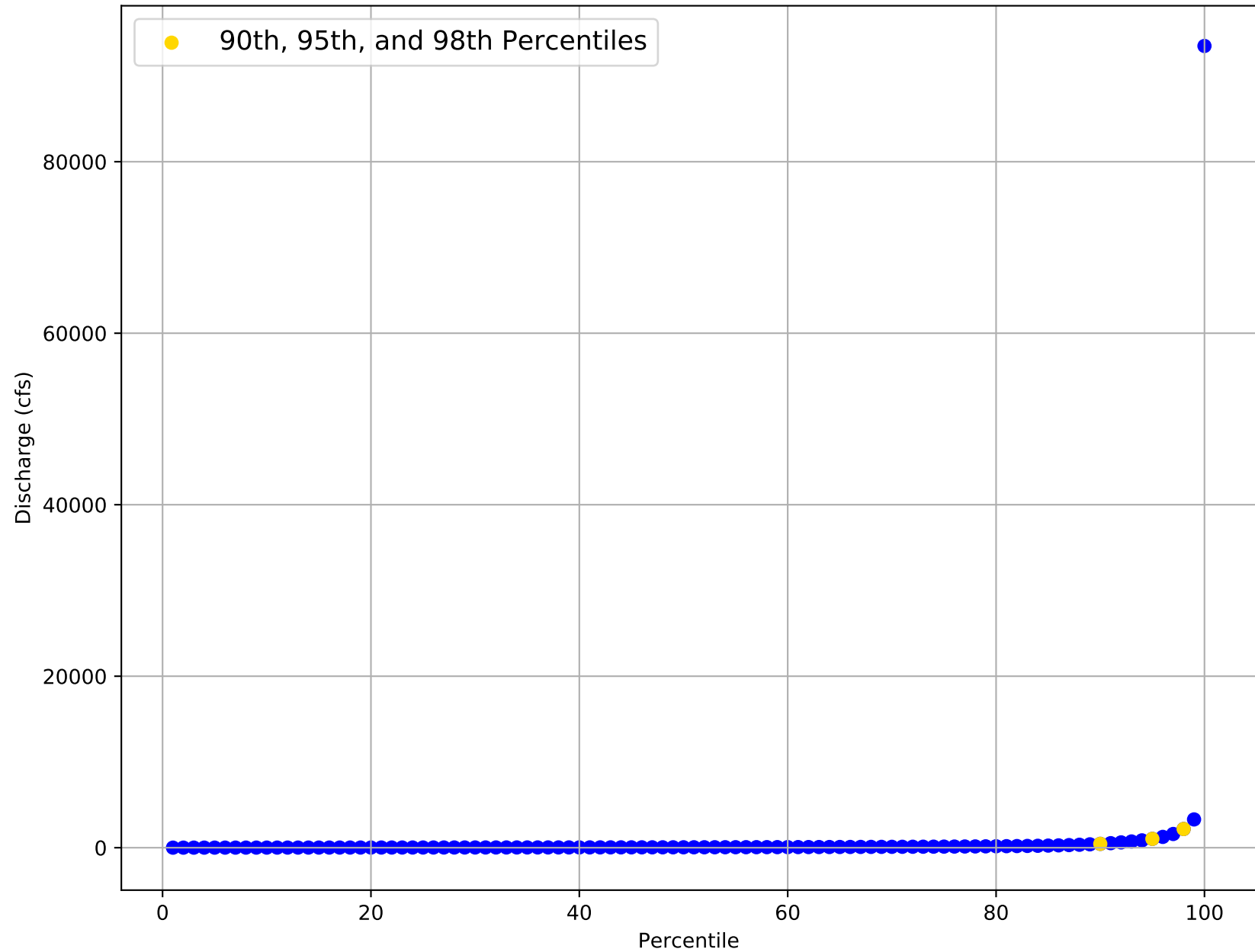
Flow Frequency Distribution for USGS Gage 08070000 from 1939 to 2020
