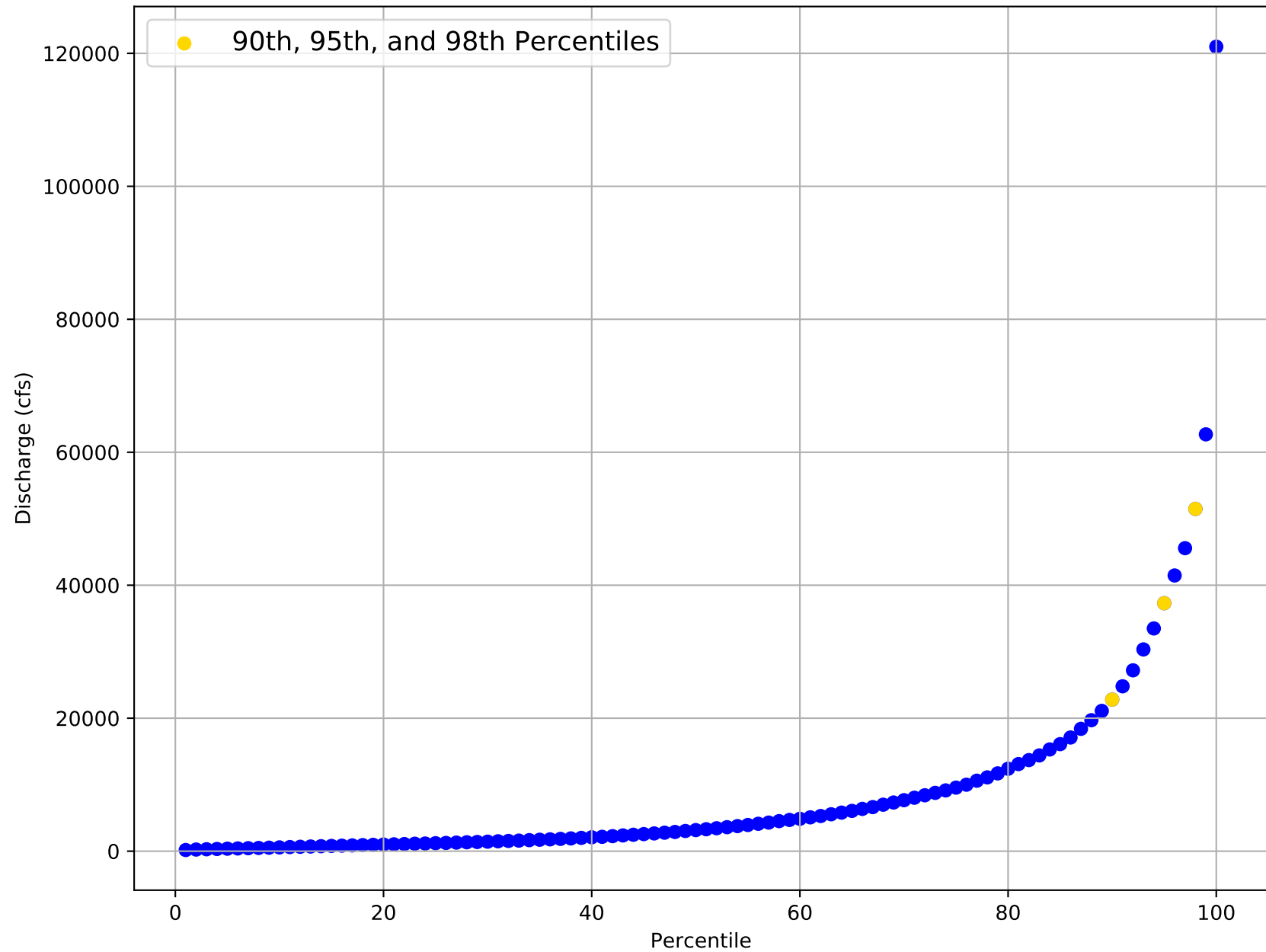
Flow Frequency Distribution for USGS Gage 08116650 from 1967 to 2020
