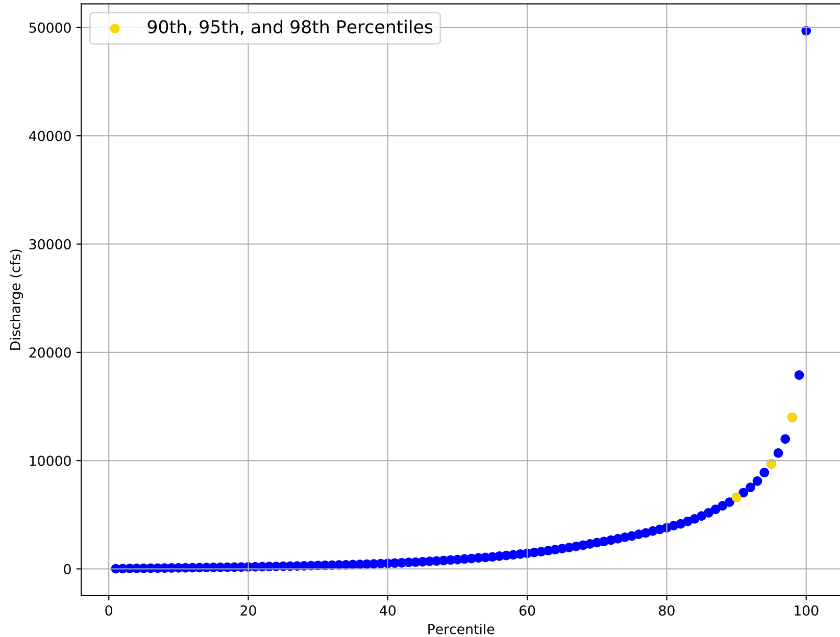
Flow Frequency Distribution for USGS Gage 08033500 from 1903 to 2020
