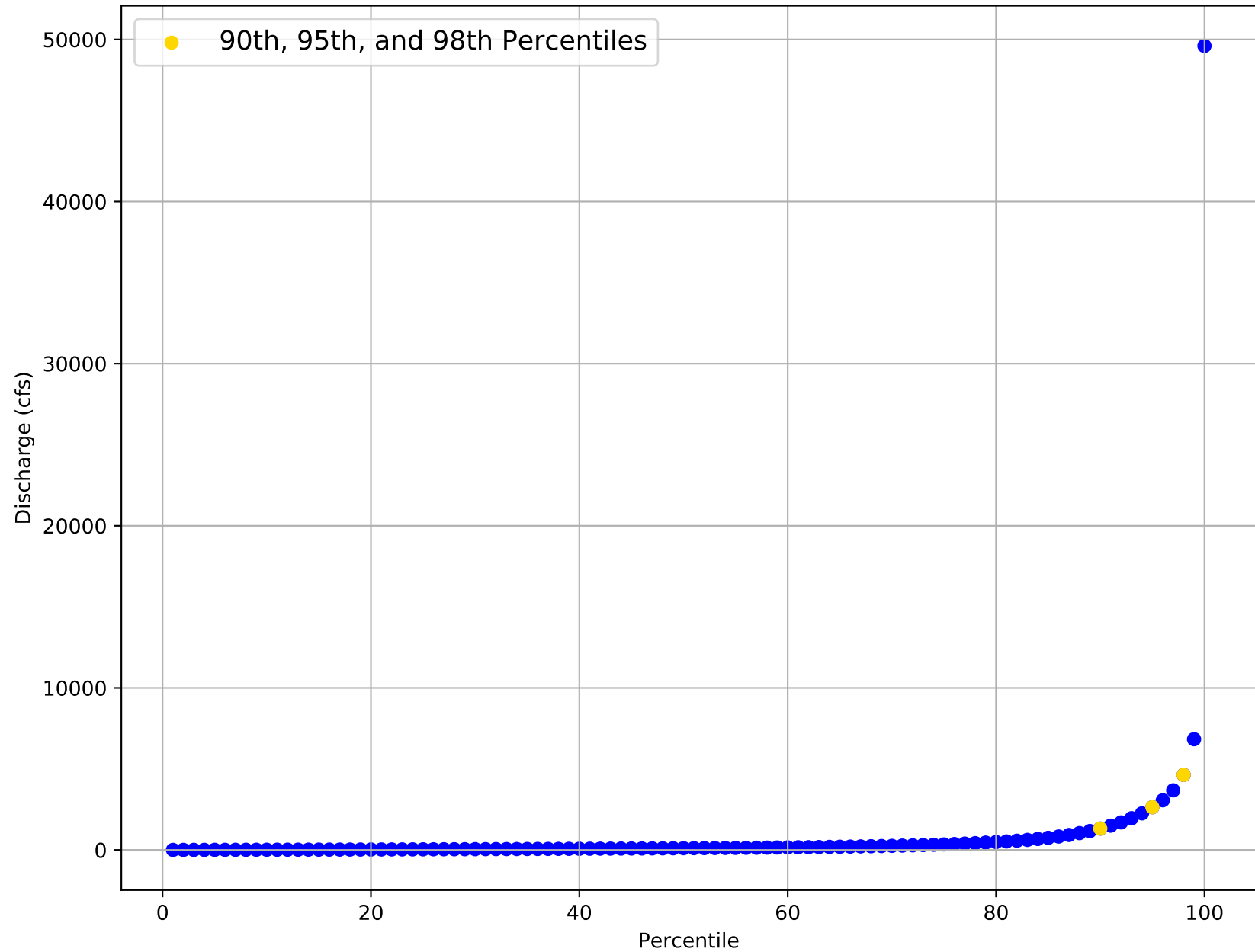
Flow Frequency Distribution for USGS Gage 08117500 from 1954 to 2020
