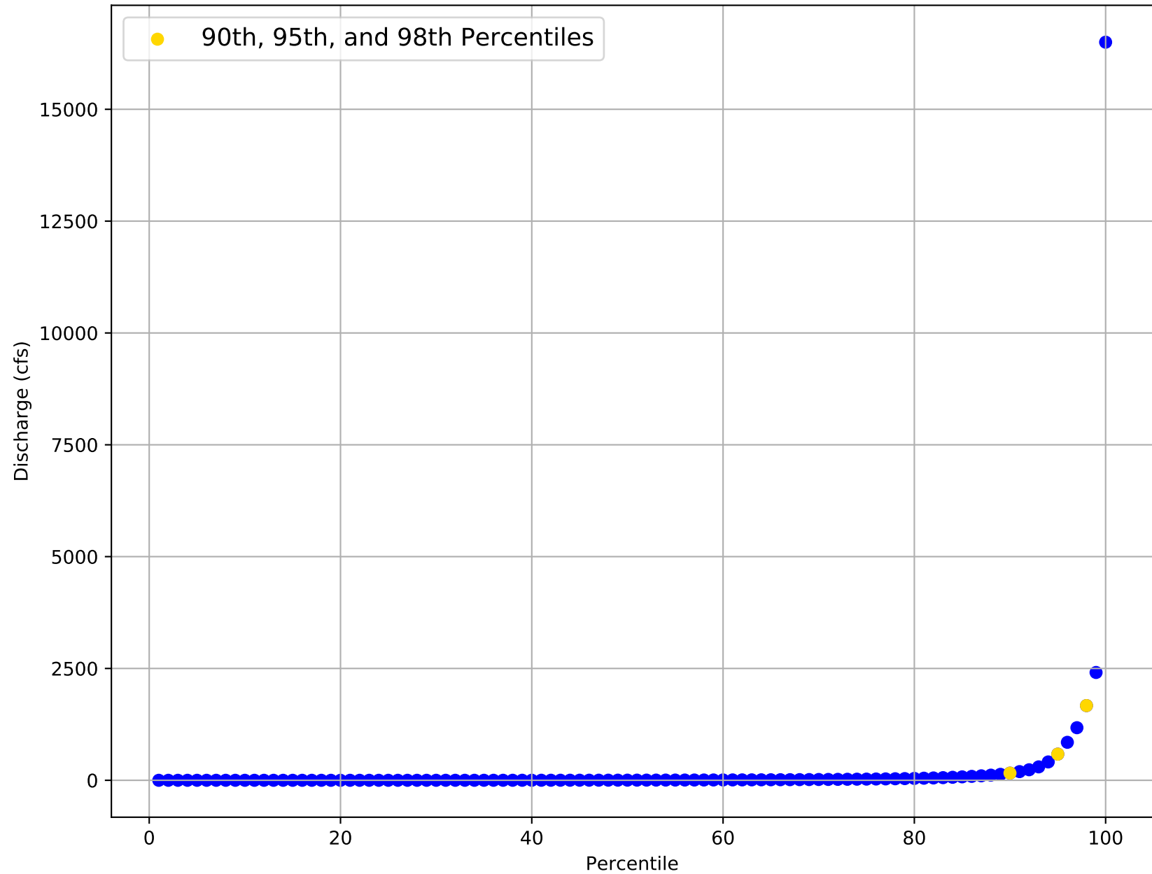
Flow Frequency Distribution for USGS Gage 08062800 from 1963 to 2020
