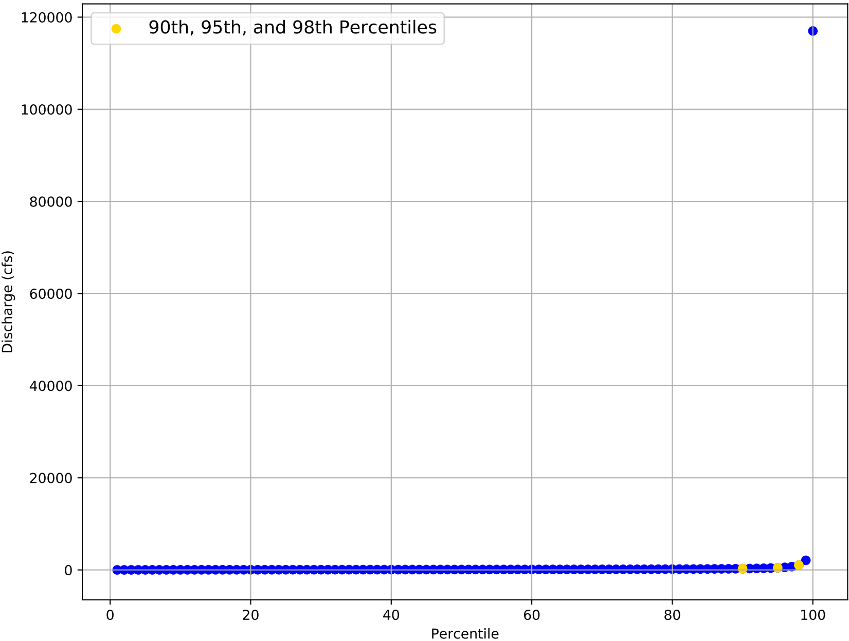
Flow Frequency Distribution for USGS Gage 08146000 from 1915 to 2020
