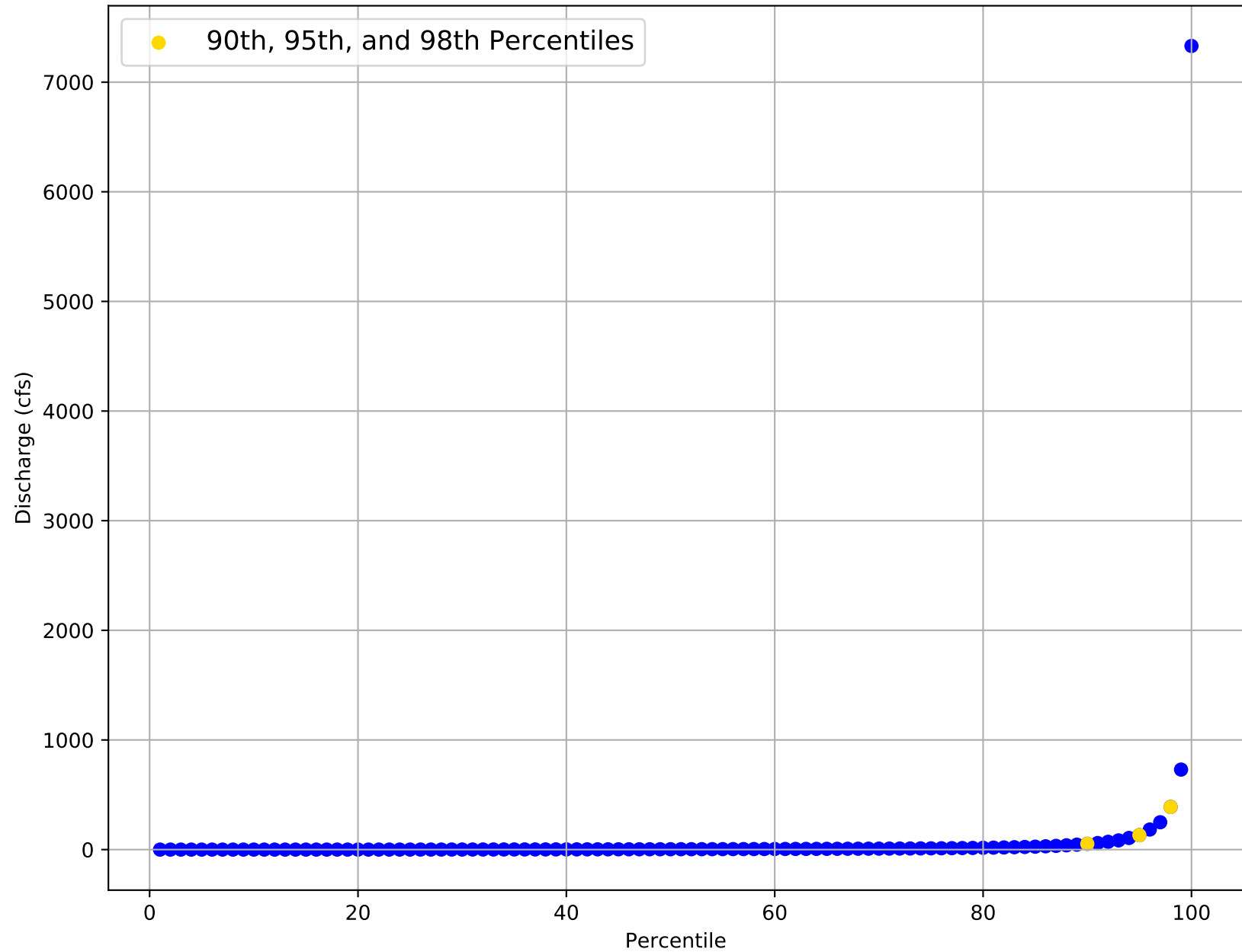
Flow Frequency Distribution for USGS Gage 08048970 from 1989 to 2020
