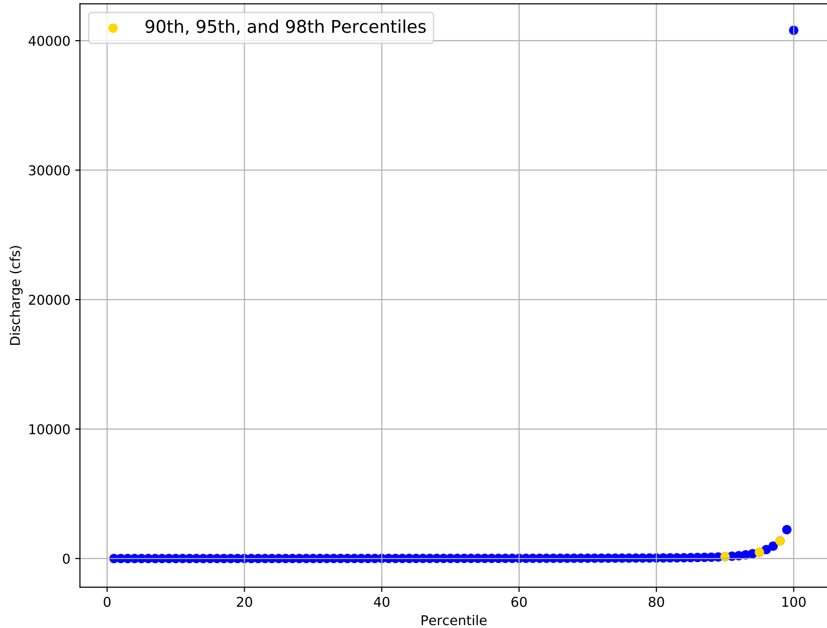
Flow Frequency Distribution for USGS Gage 08068275 from 1999 to 2020
