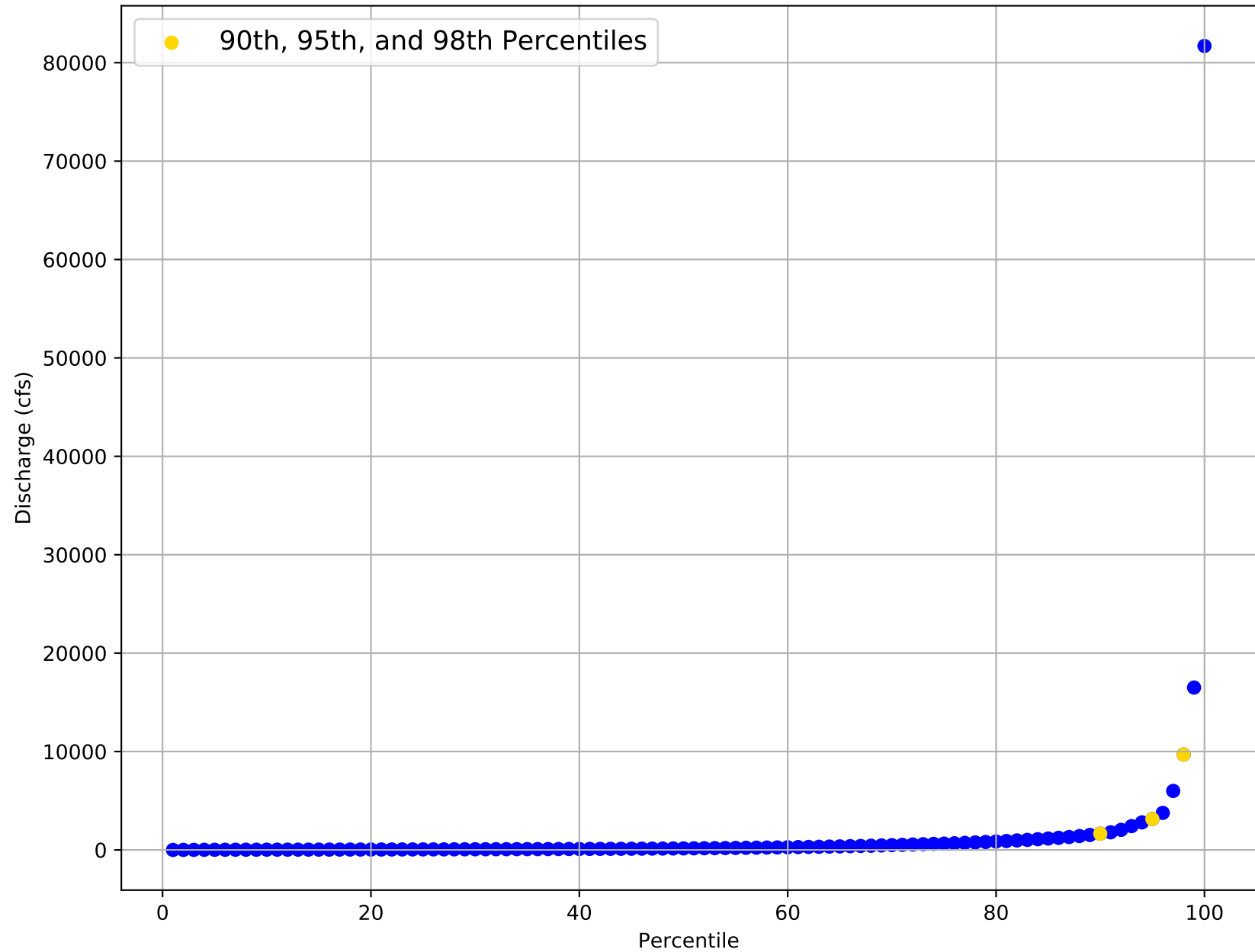
Flow Frequency Distribution for USGS Gage 08089000 from 1924 to 2020
