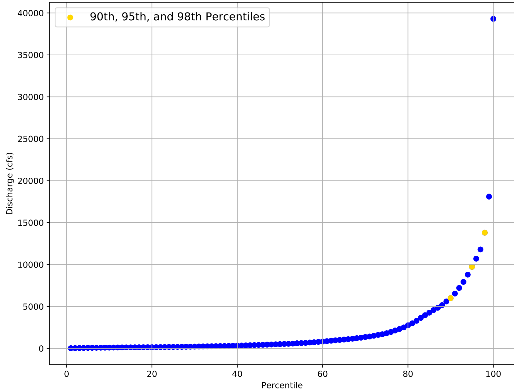
Flow Frequency Distribution for USGS Gage 08020900 from 1995 to 2020
