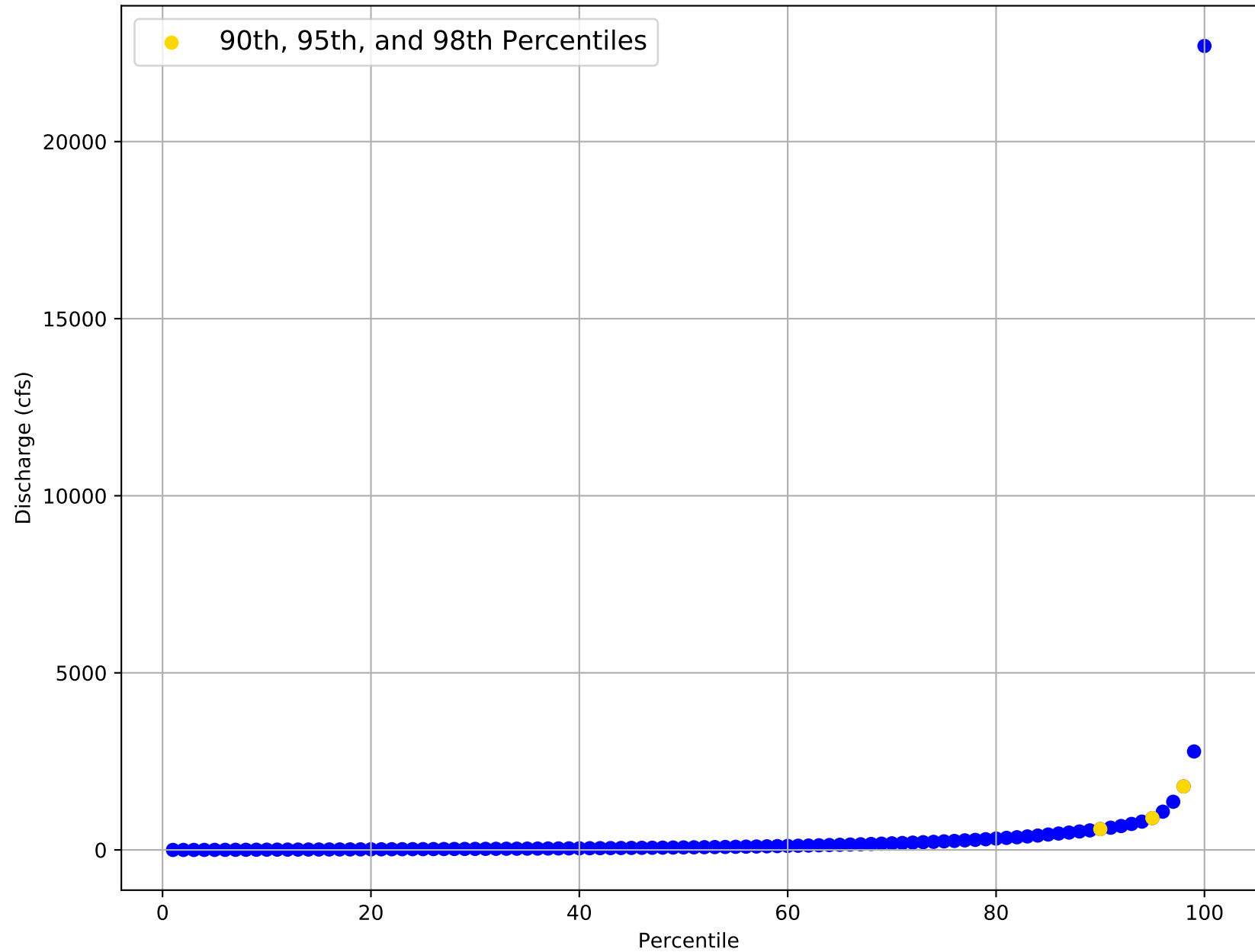
Flow Frequency Distribution for USGS Gage 08034500 from 1939 to 2020
