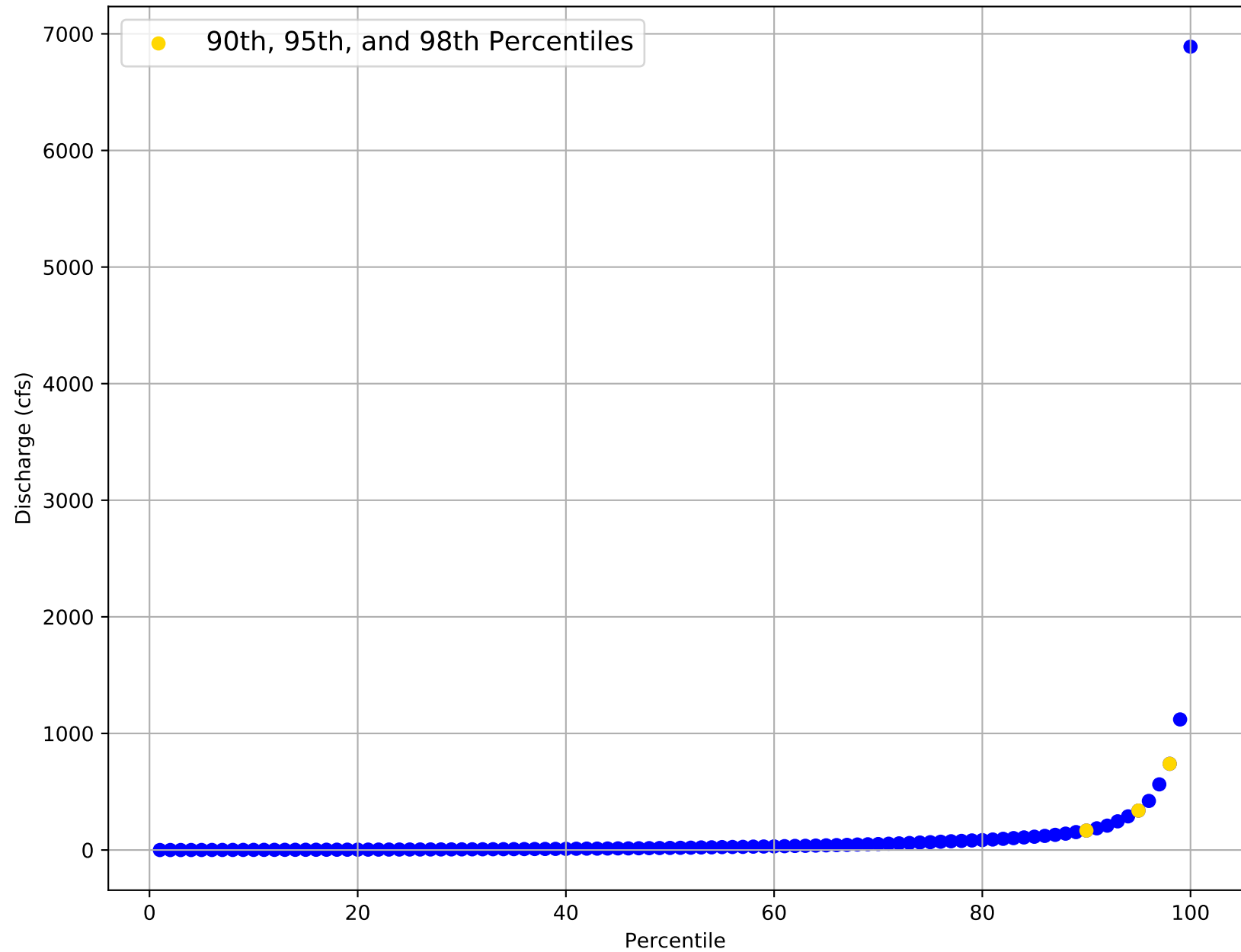
Flow Frequency Distribution for USGS Gage 08039100 from 1959 to 1985
