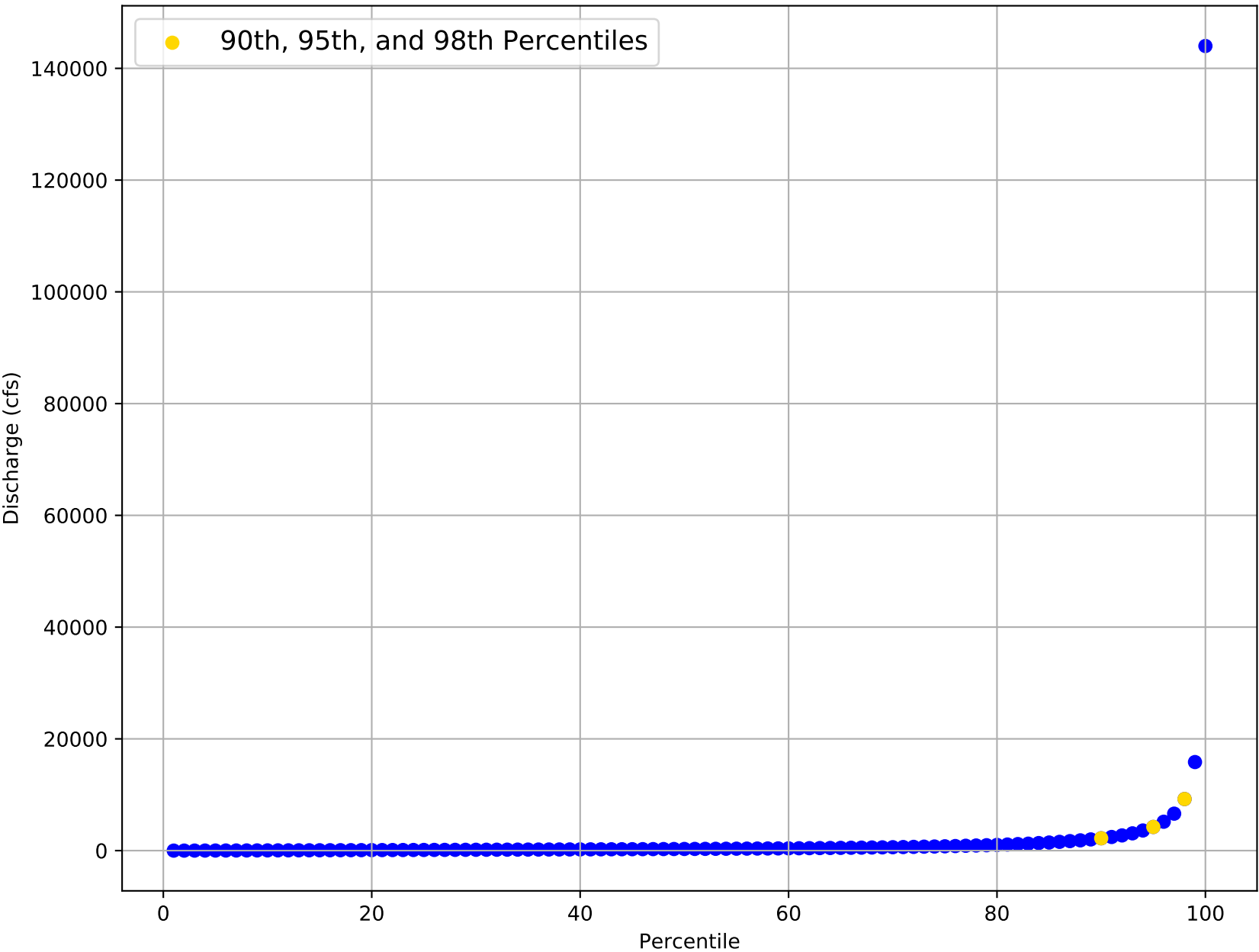
Flow Frequency Distribution for USGS Gage 07308500 from 1924 to 2020
