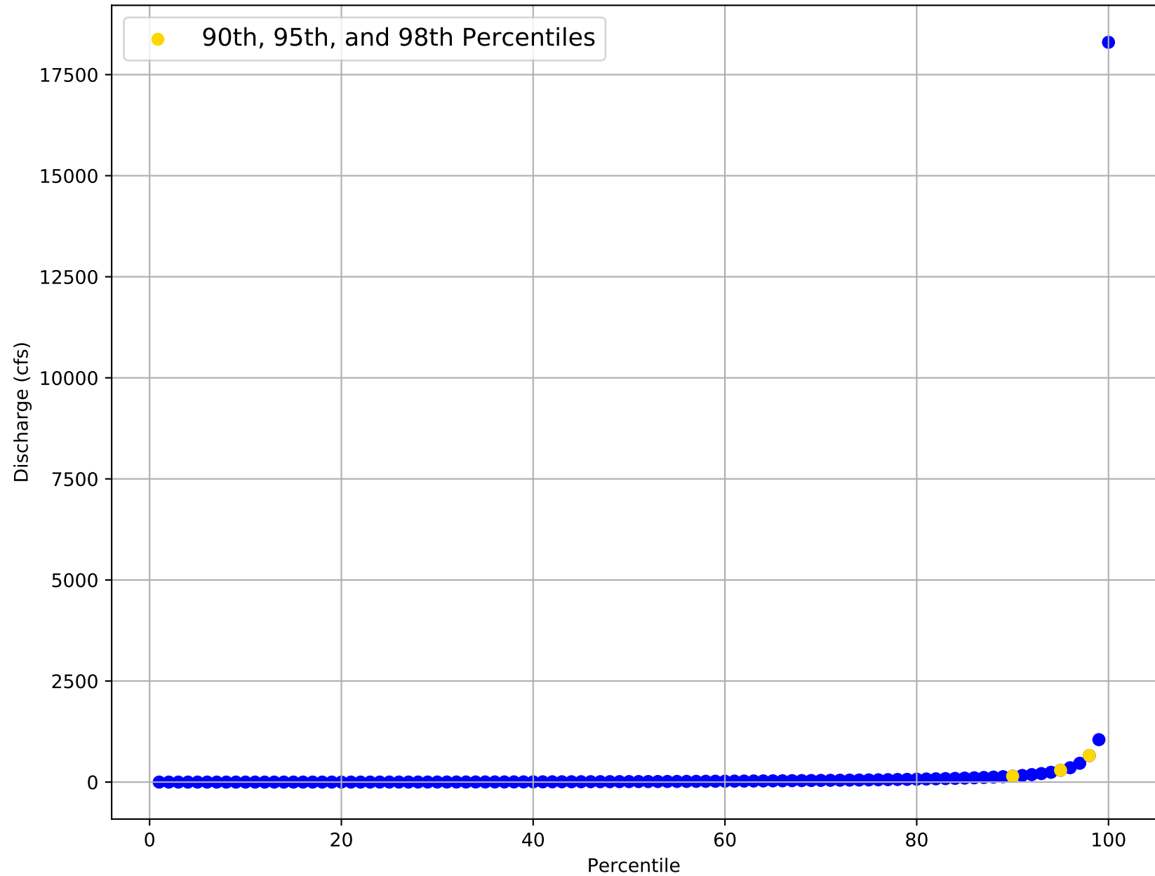
Flow Frequency Distribution for USGS Gage 07345000 from 1943 to 1977
