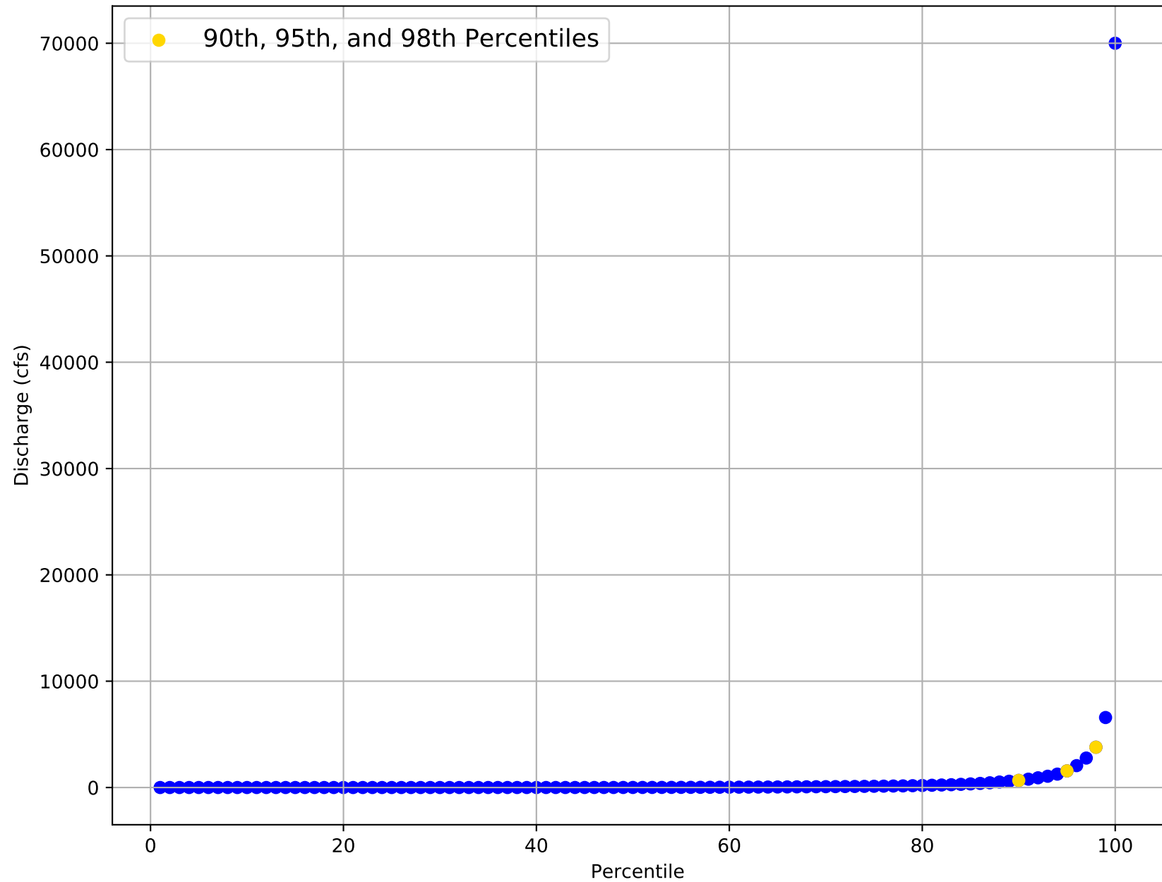
Flow Frequency Distribution for USGS Gage 08194500 from 1942 to 2020
