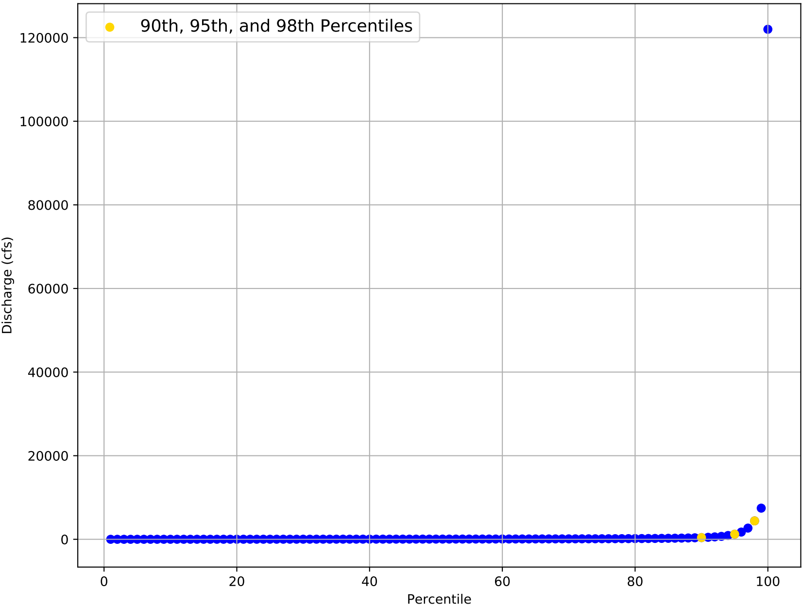
Flow Frequency Distribution for USGS Gage 08164000 from 1938 to 2020
