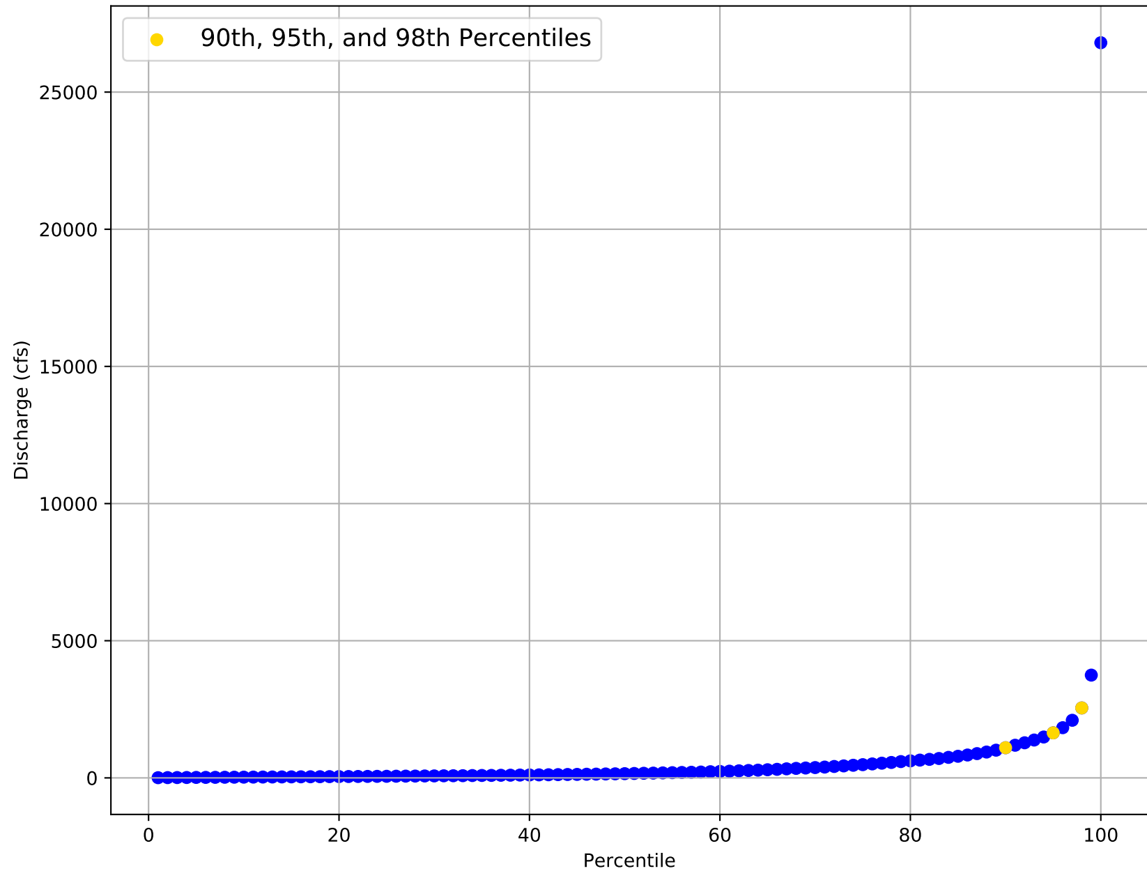
Flow Frequency Distribution for USGS Gage 08038000 from 1924 to 1985
