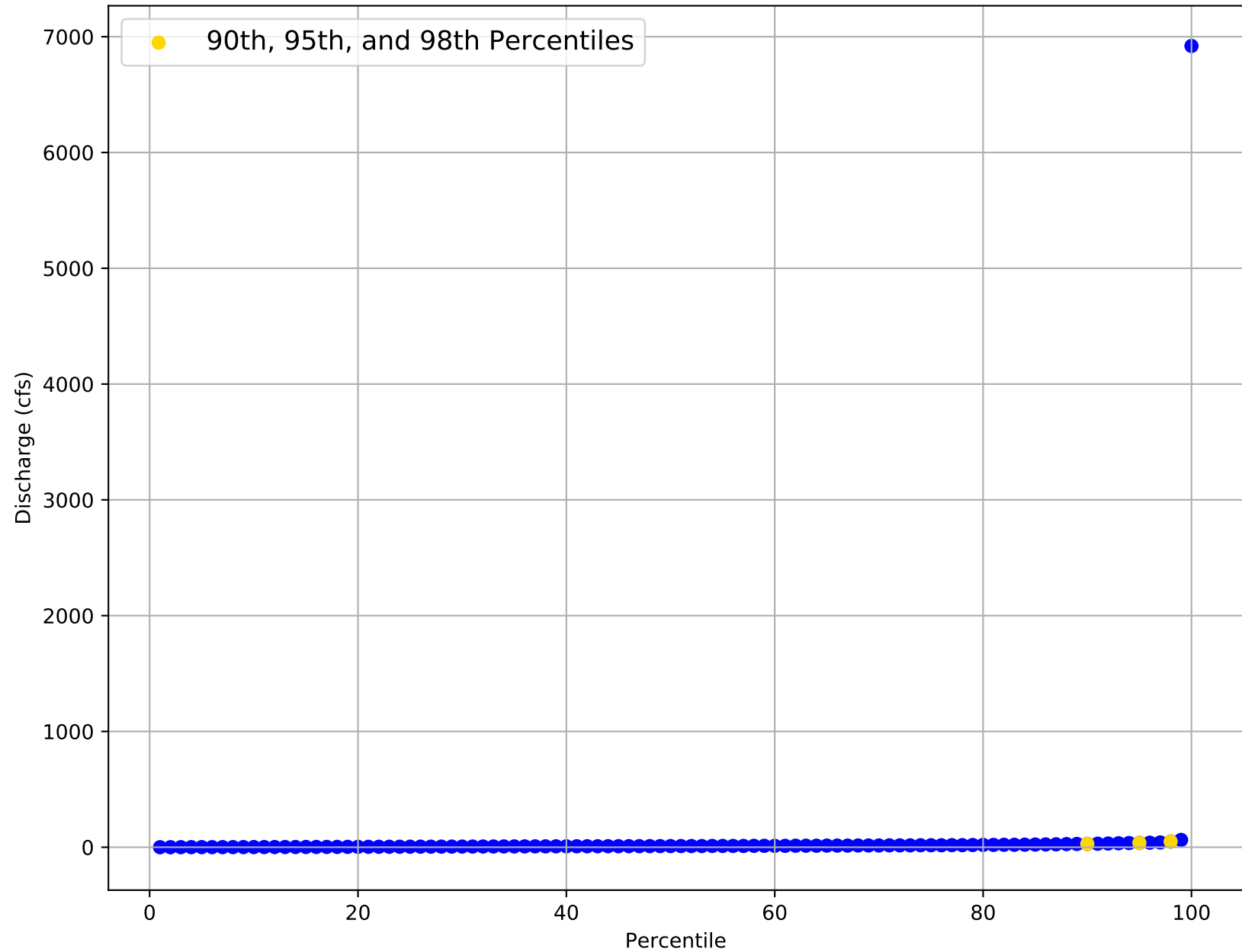
Flow Frequency Distribution for USGS Gage 08130500 from 1960 to 2018
