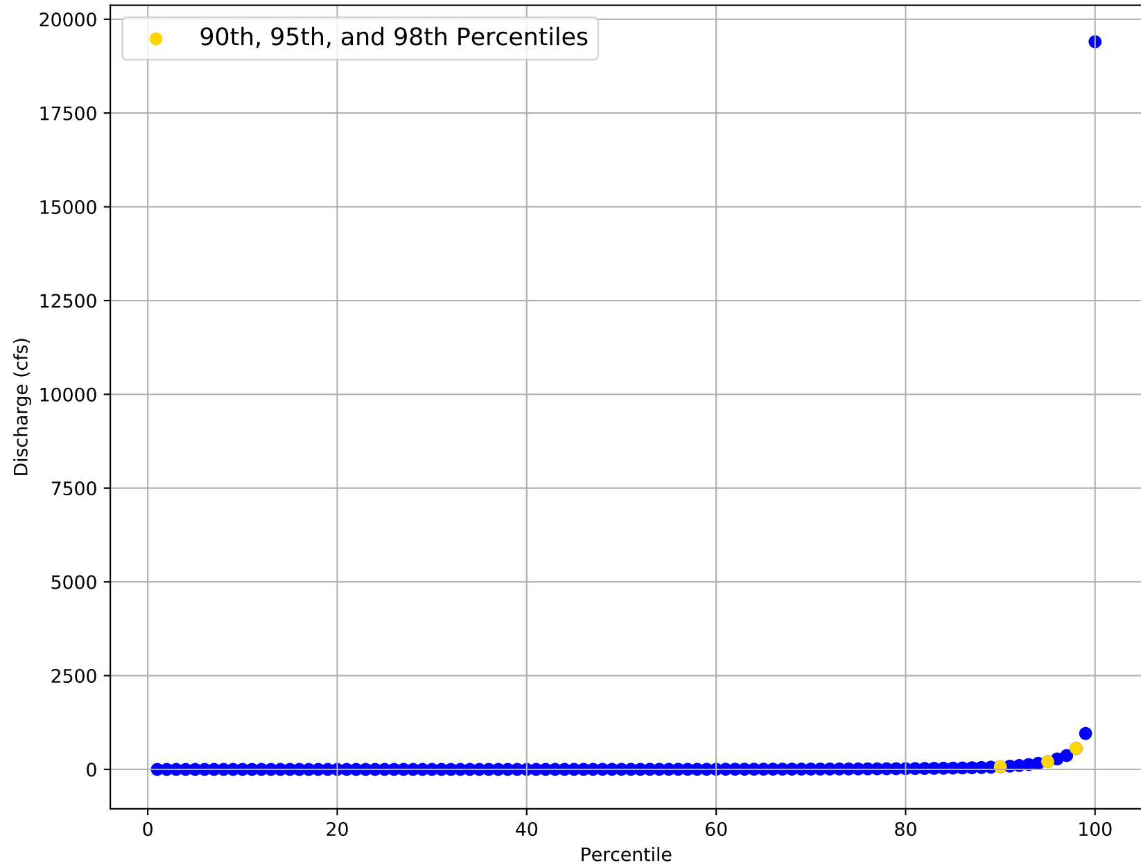
Flow Frequency Distribution for USGS Gage 08172400 from 1959 to 2020
