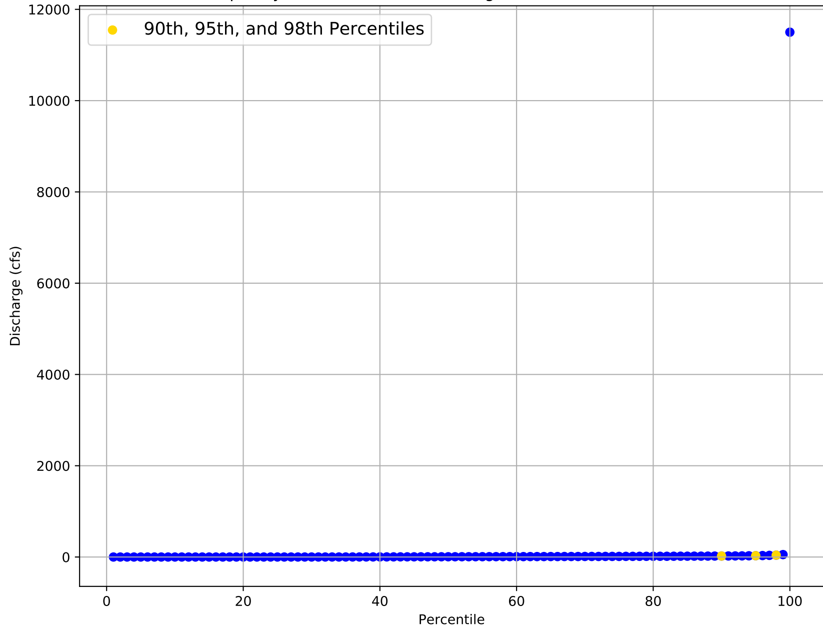
Flow Frequency Distribution for USGS Gage 08129300 from 1960 to 1995
