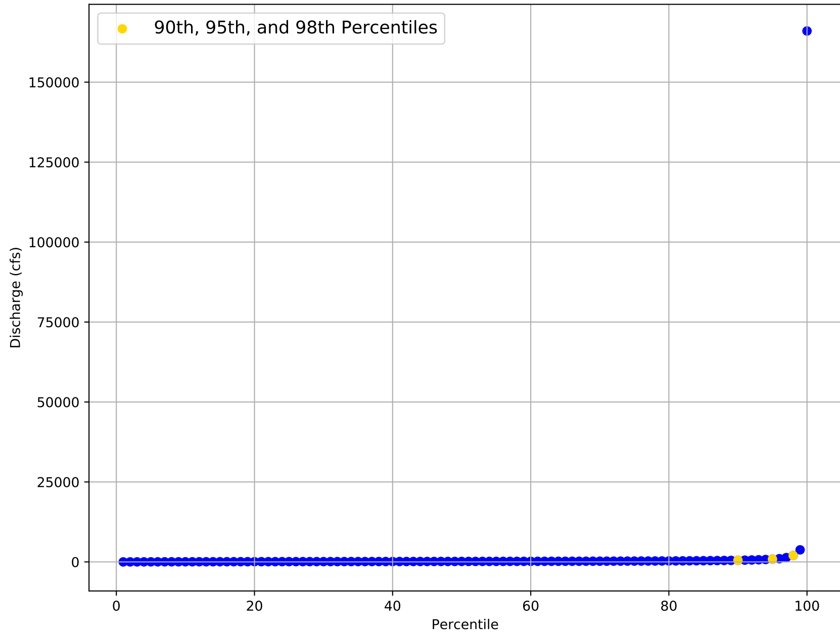
Flow Frequency Distribution for USGS Gage 08151500 from 1939 to 2020
