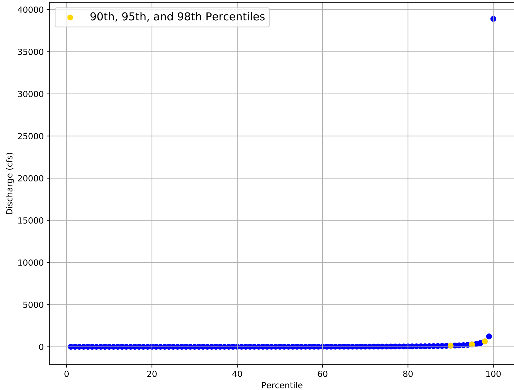
Flow Frequency Distribution for USGS Gage 08159000 from 1924 to 2020
