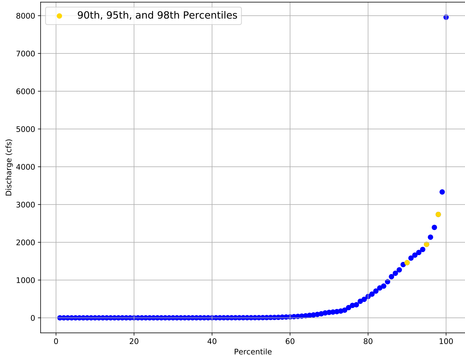
Flow Frequency Distribution for USGS Gage 08051130 from 1985 to 1993
