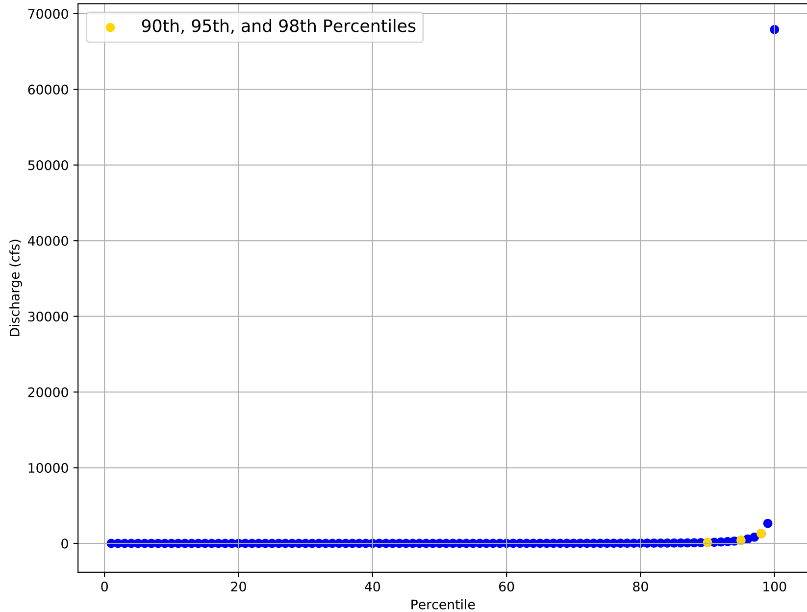
Flow Frequency Distribution for USGS Gage 08175000 from 1930 to 2020
