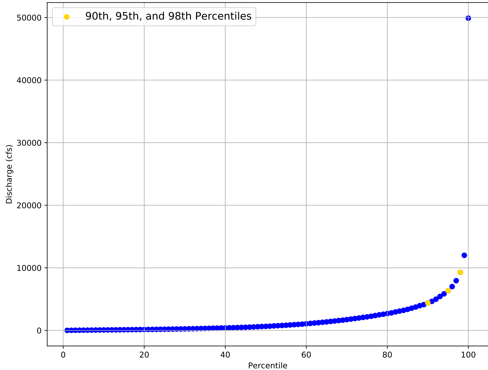
Flow Frequency Distribution for USGS Gage 08033000 from 1923 to 2020
