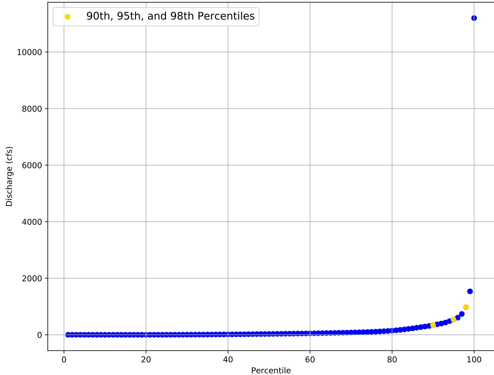
Flow Frequency Distribution for USGS Gage 08031200 from 1962 to 1989
