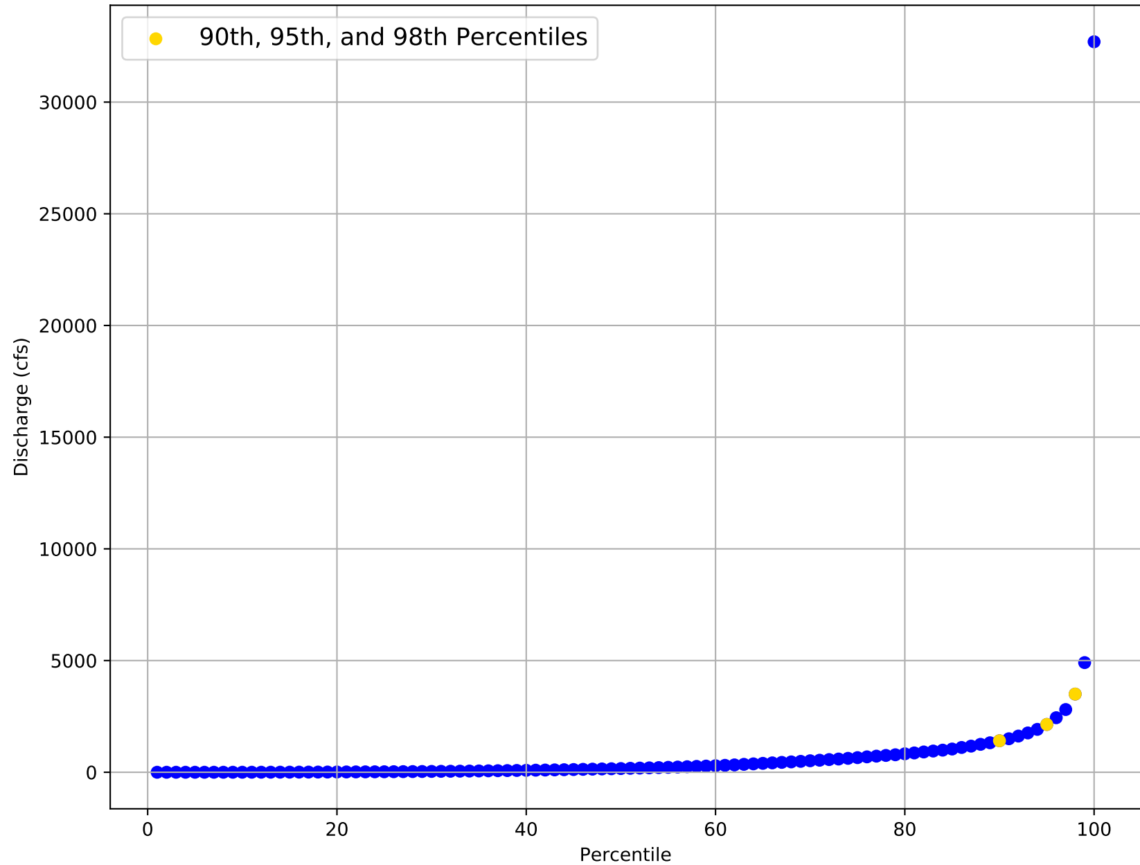
Flow Frequency Distribution for USGS Gage 07346070 from 1946 to 2020
