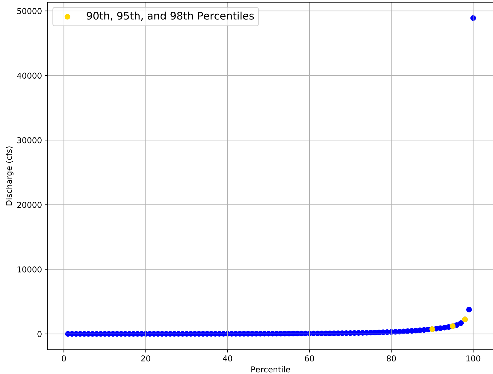
Flow Frequency Distribution for USGS Gage 07344500 from 1943 to 2020
