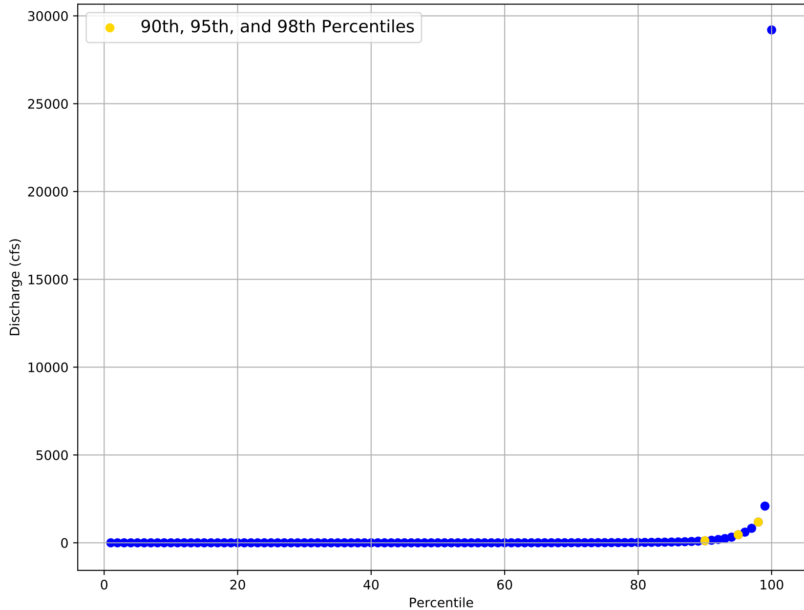
Flow Frequency Distribution for USGS Gage 08042800 from 1956 to 2020
