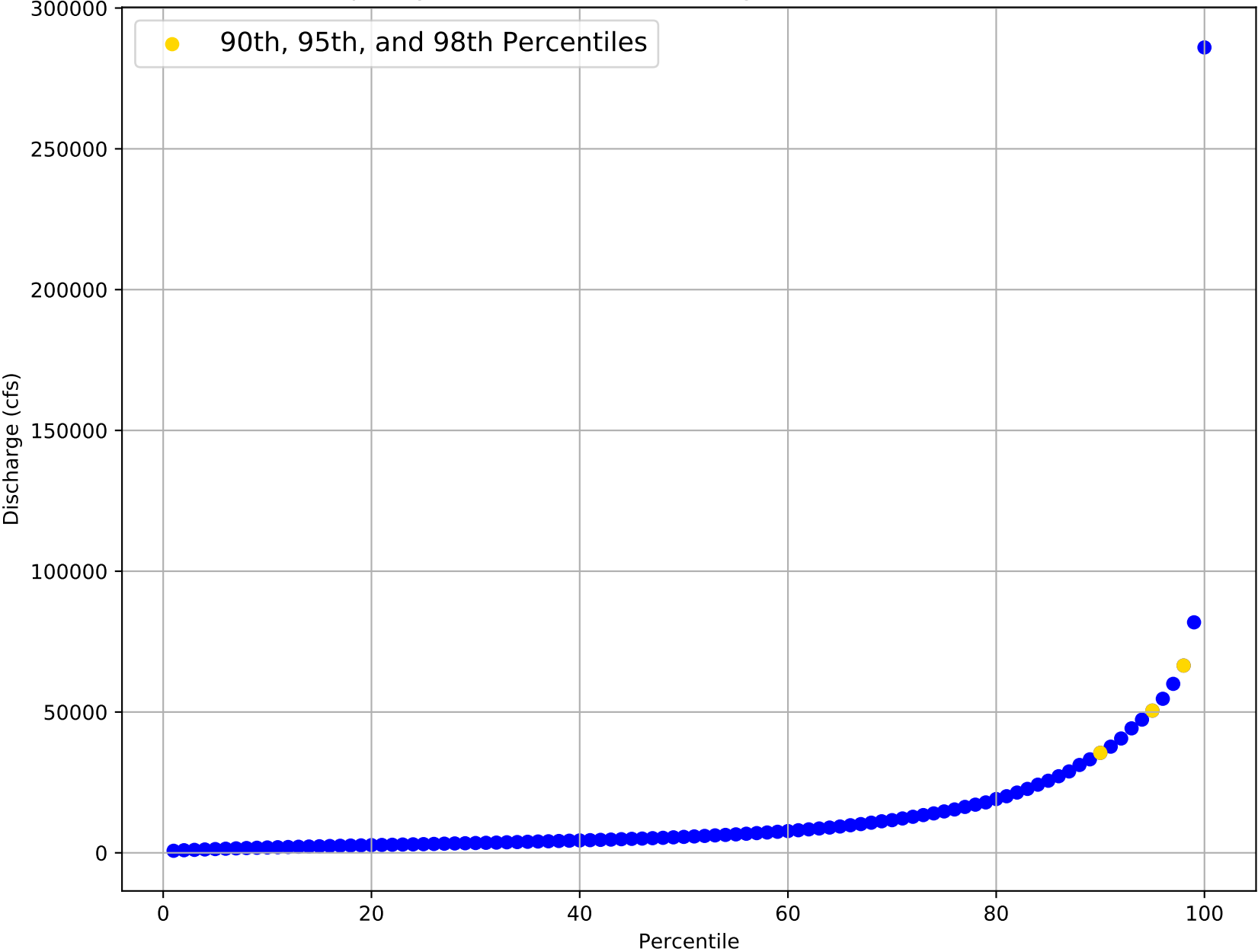
Flow Frequency Distribution for USGS Gage 07337000 from 1936 to 2020
