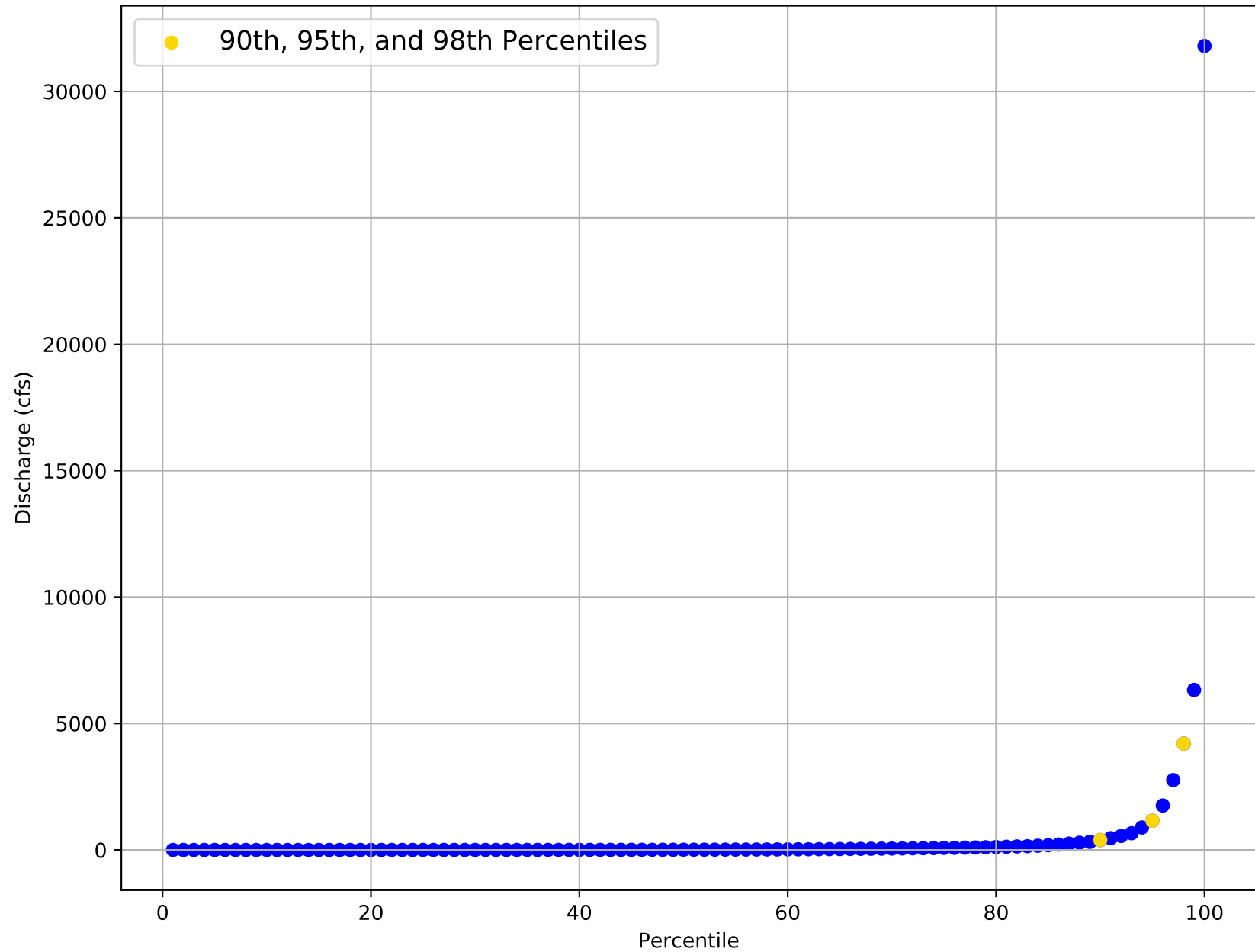
Flow Frequency Distribution for USGS Gage 07332622 from 2009 to 2020
