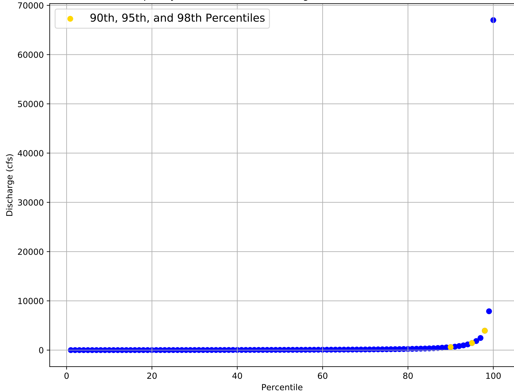
Flow Frequency Distribution for USGS Gage 08138000 from 1923 to 2011
