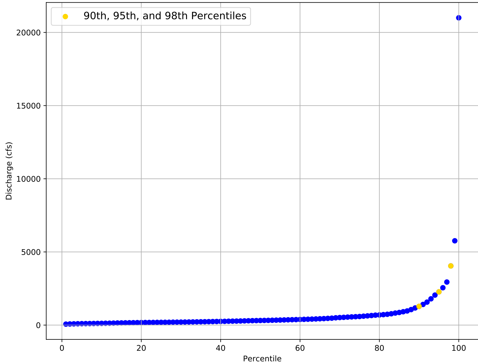
Flow Frequency Distribution for USGS Gage 08188060 from 2011 to 2020
