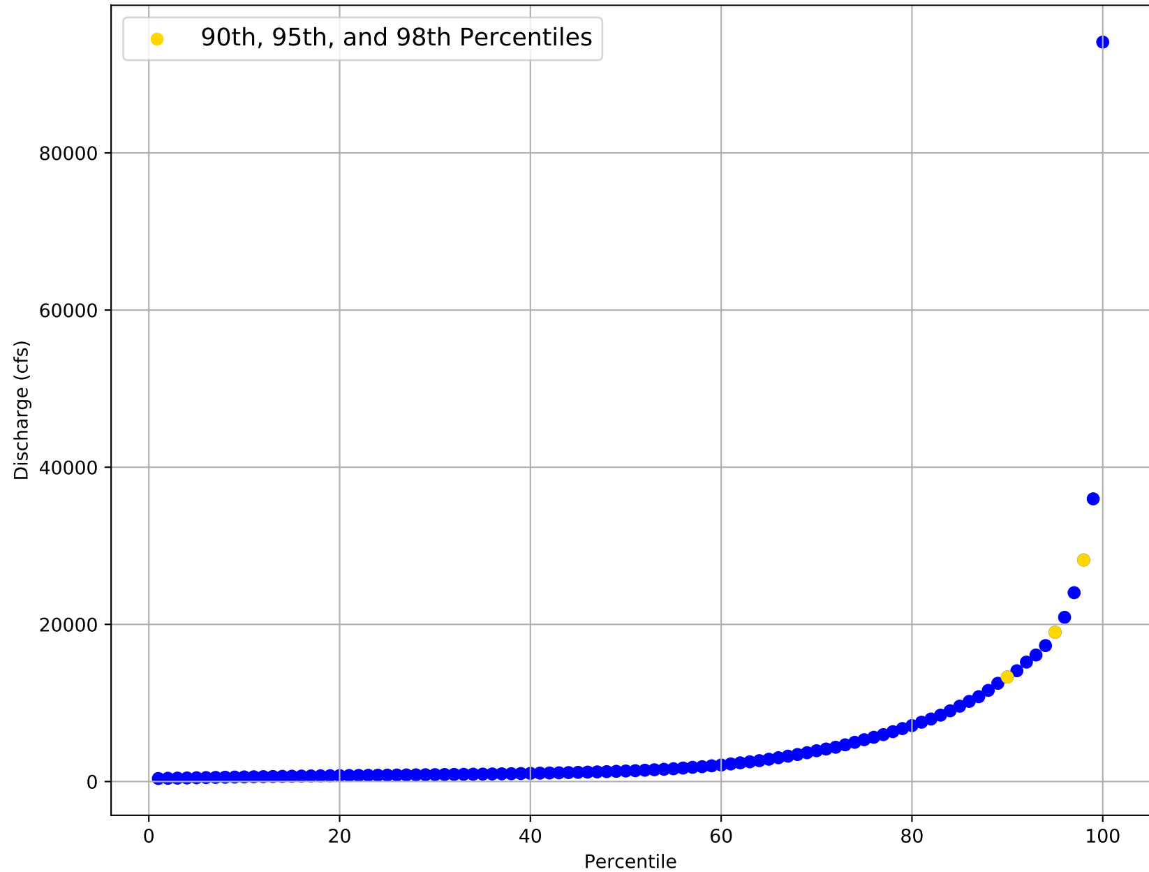
Flow Frequency Distribution for USGS Gage 08062700 from 1964 to 2020
