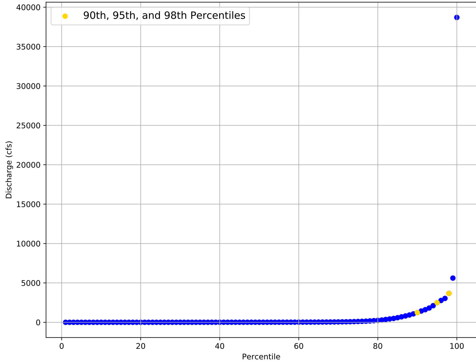
Flow Frequency Distribution for USGS Gage 07342500 from 1942 to 2020
