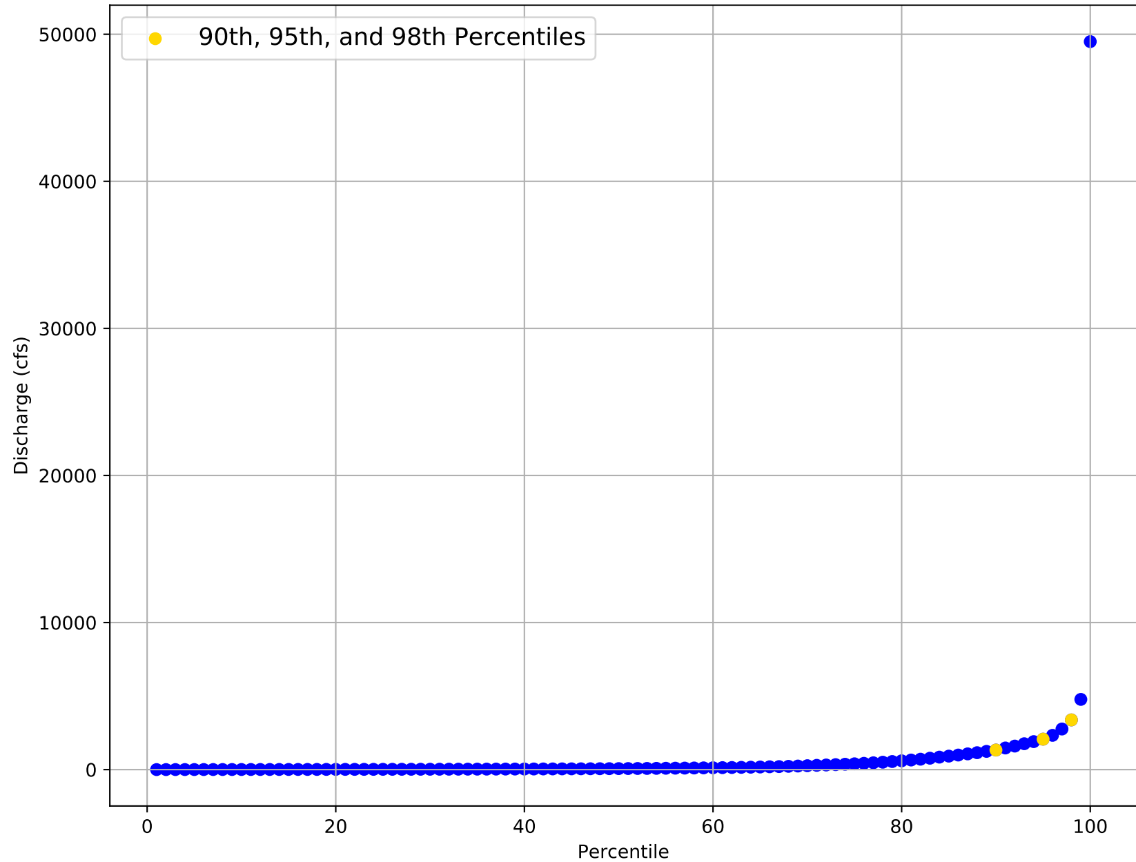
Flow Frequency Distribution for USGS Gage 08041700 from 1967 to 2020
