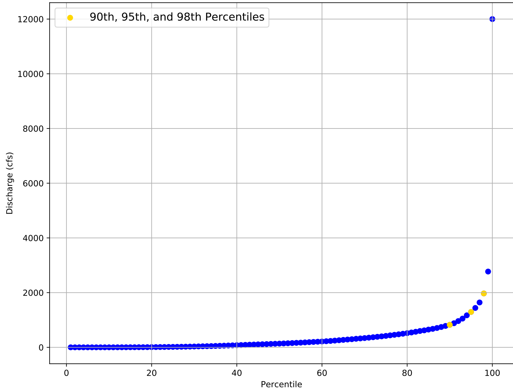
Flow Frequency Distribution for USGS Gage 07346045 from 1968 to 2020
