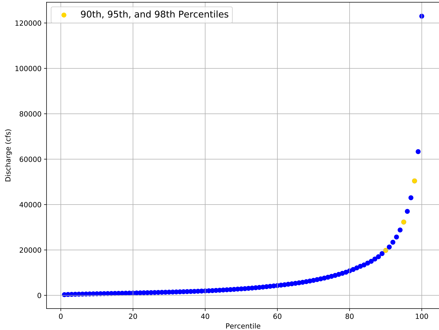
Flow Frequency Distribution for USGS Gage 08114000 from 1903 to 2020
