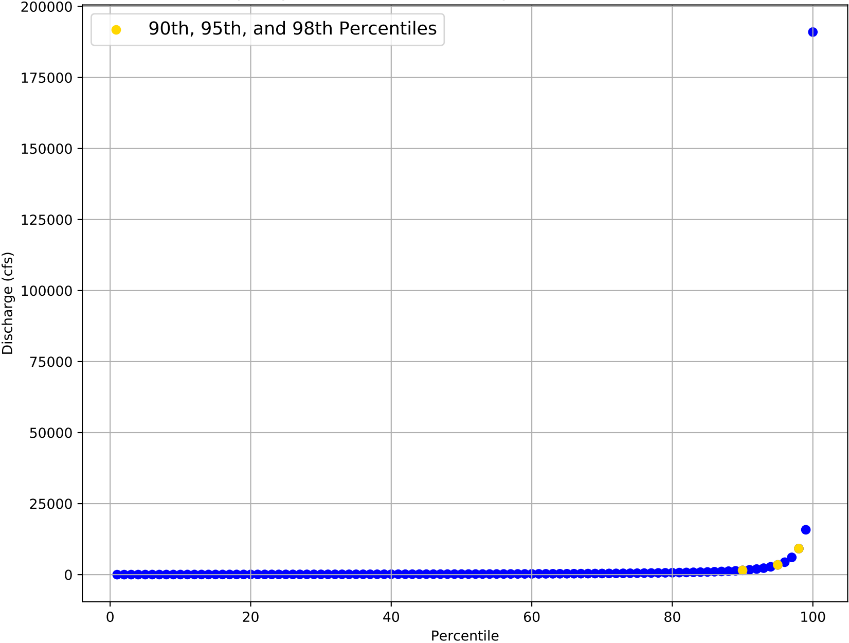
Flow Frequency Distribution for USGS Gage 08147000 from 1915 to 2020
