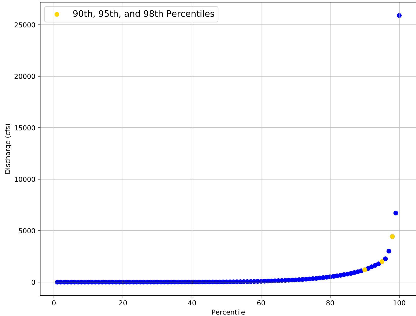
Flow Frequency Distribution for USGS Gage 08064100 from 1983 to 2020
