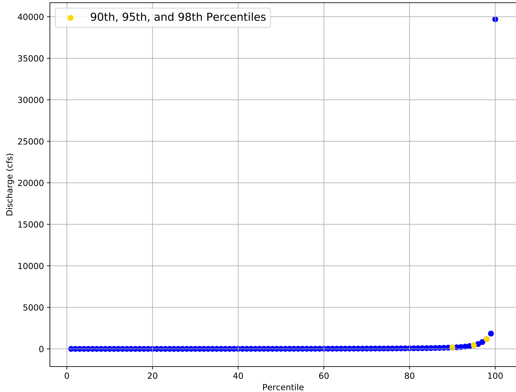
Flow Frequency Distribution for USGS Gage 08051500 from 1949 to 2020
