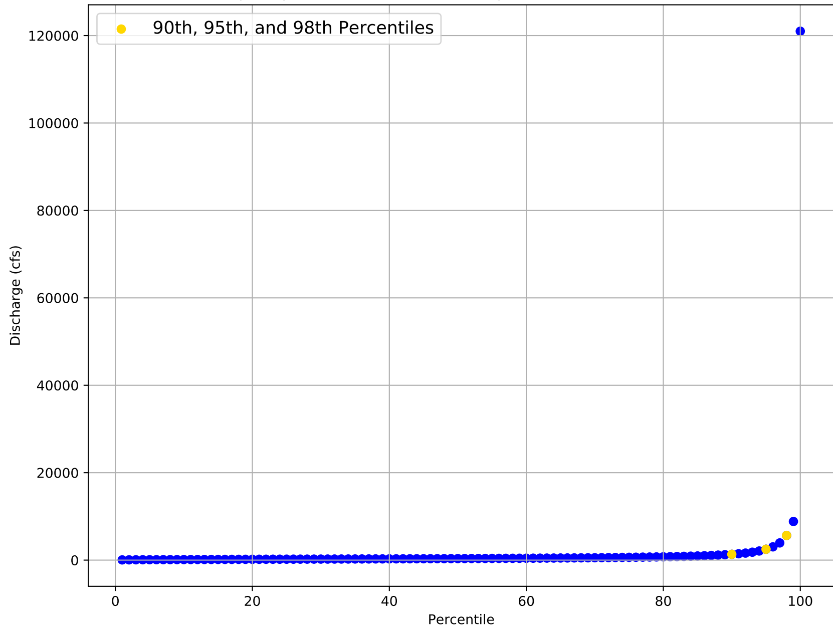
Flow Frequency Distribution for USGS Gage 08188500 from 1924 to 2020
