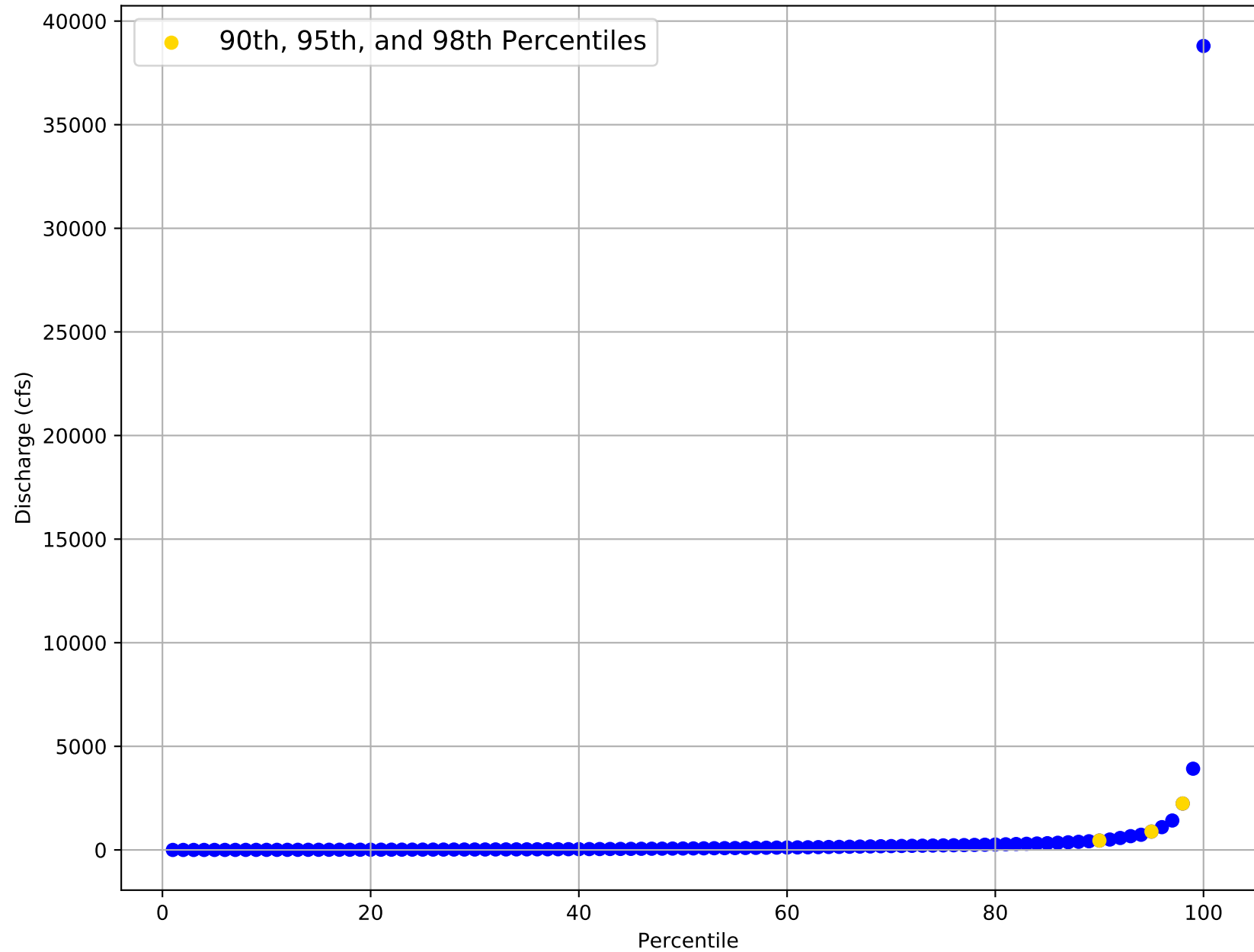
Flow Frequency Distribution for USGS Gage 08044500 from 1947 to 2020
