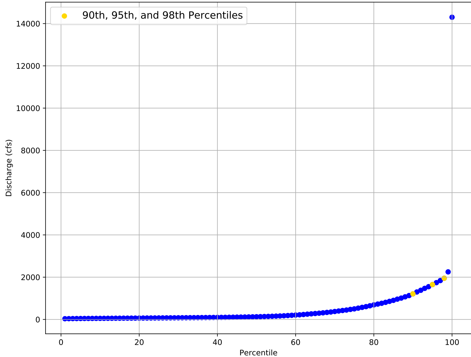
Flow Frequency Distribution for USGS Gage 08073600 from 1971 to 2020
