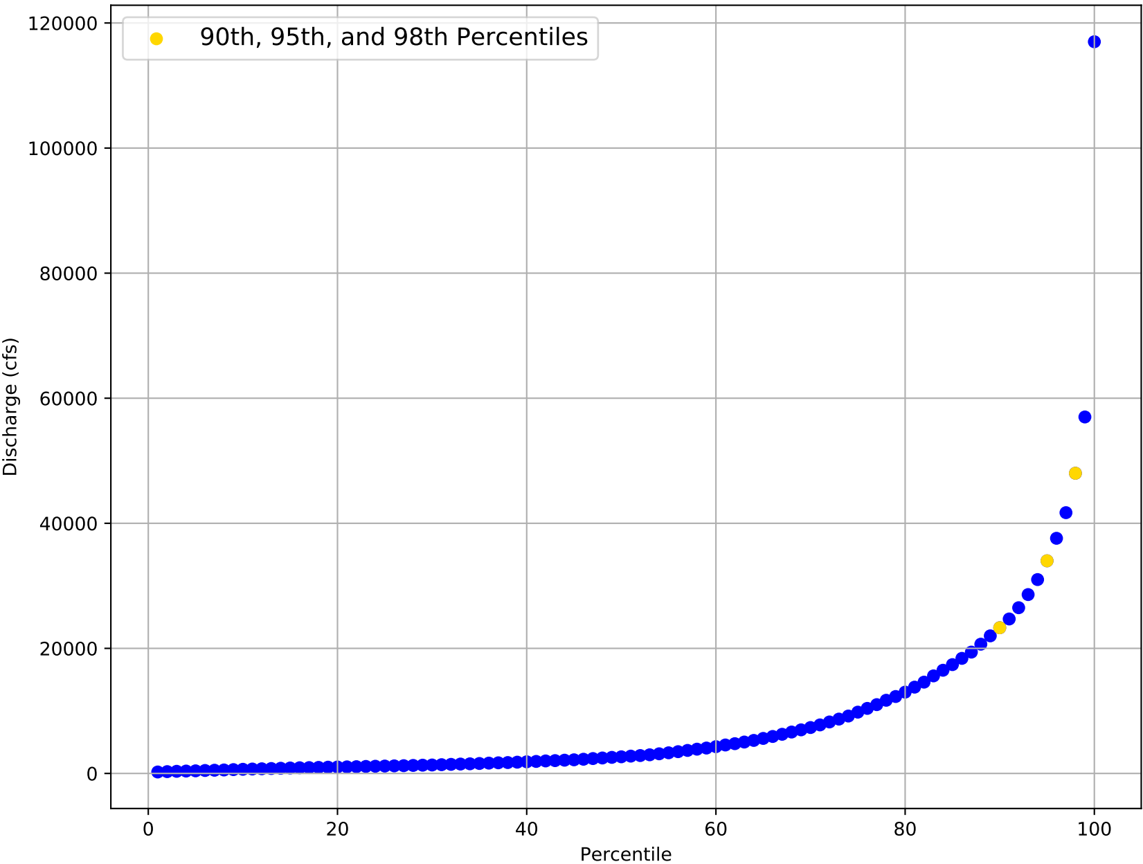
Flow Frequency Distribution for USGS Gage 08066500 from 1924 to 2020
