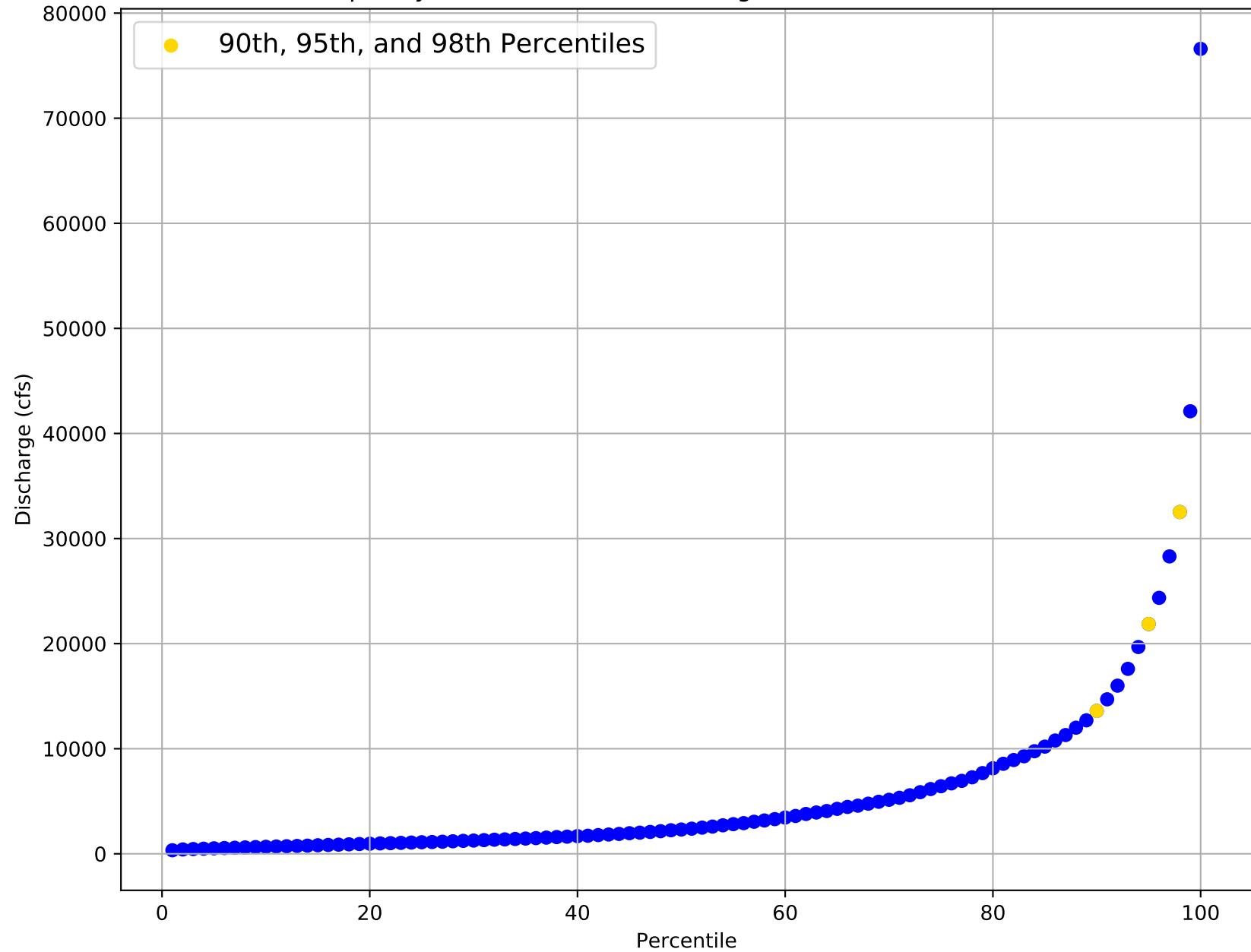
Flow Frequency Distribution for USGS Gage 08110200 from 1965 to 1987
