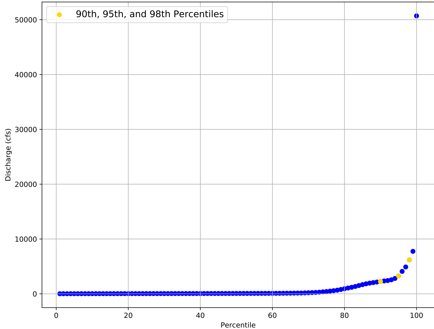
Flow Frequency Distribution for USGS Gage 08061750 from 1973 to 2020
