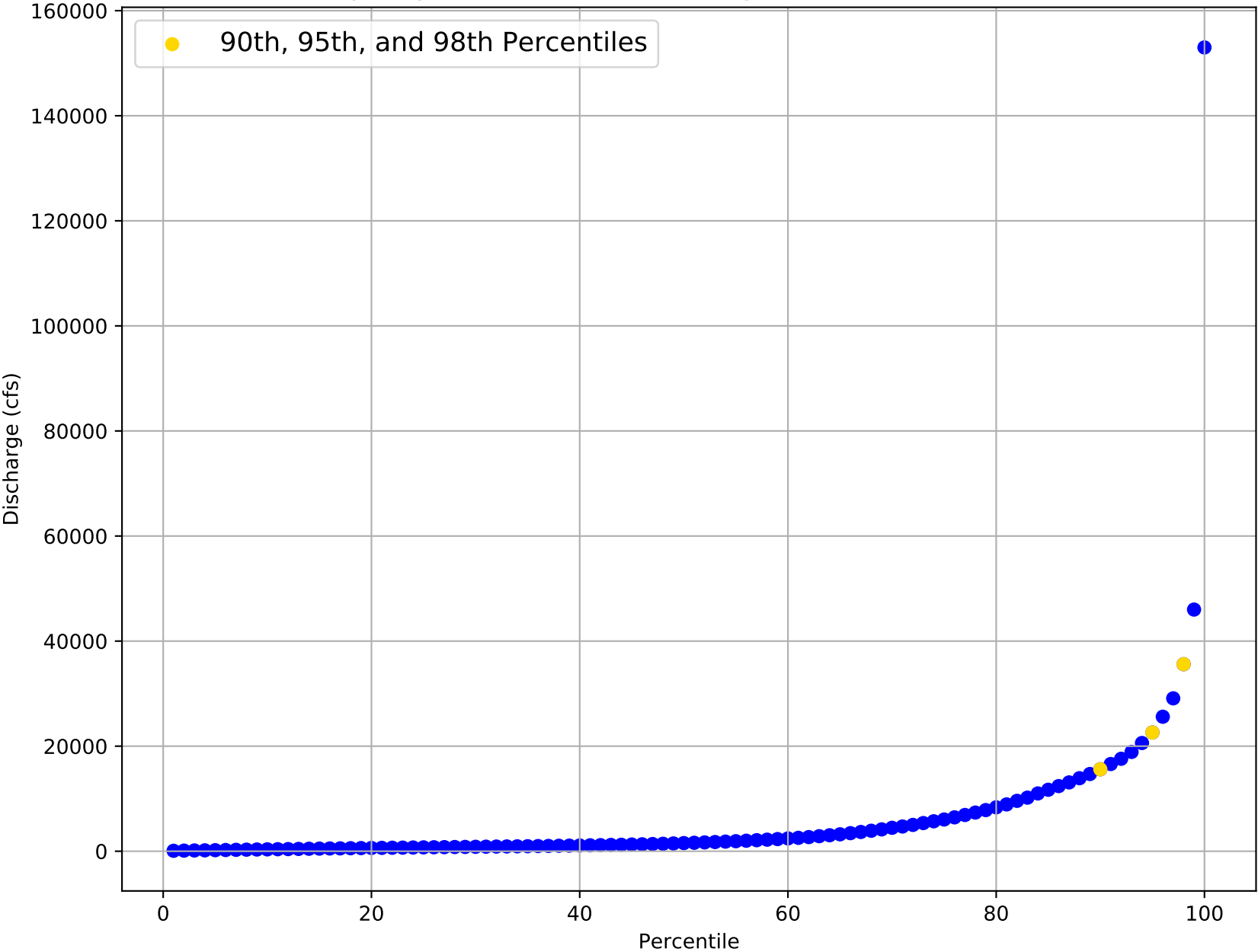
Flow Frequency Distribution for USGS Gage 08065000 from 1923 to 2020
