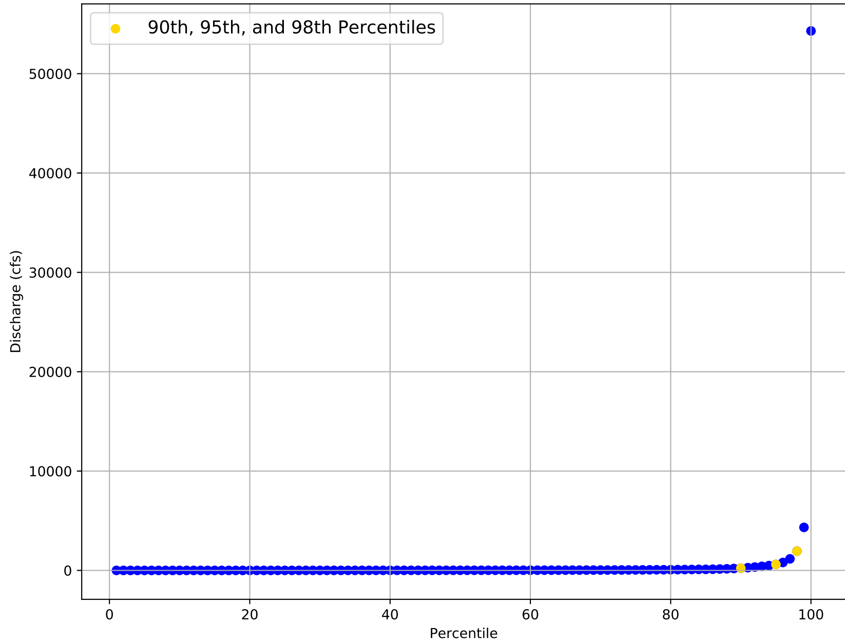
Flow Frequency Distribution for USGS Gage 08126380 from 1907 to 2020
