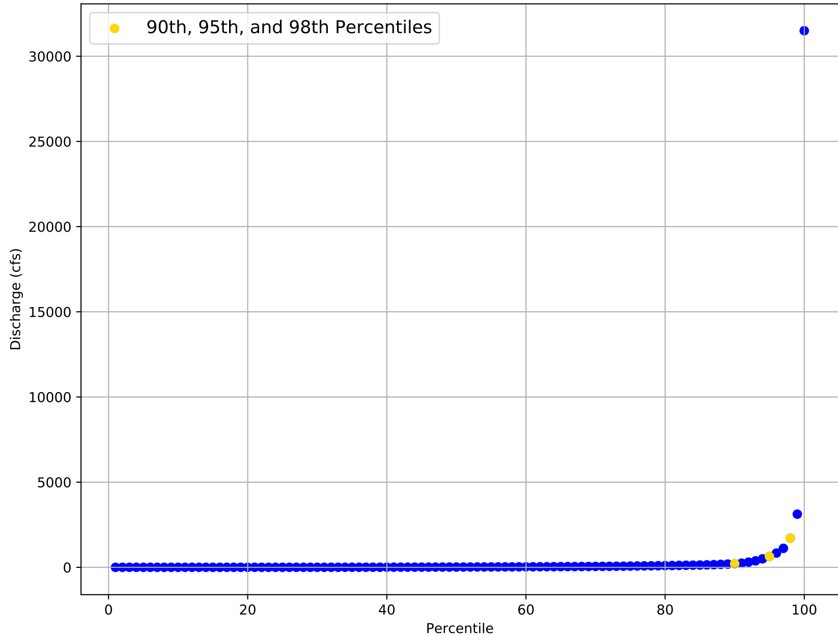
Flow Frequency Distribution for USGS Gage 08206600 from 1978 to 2020
