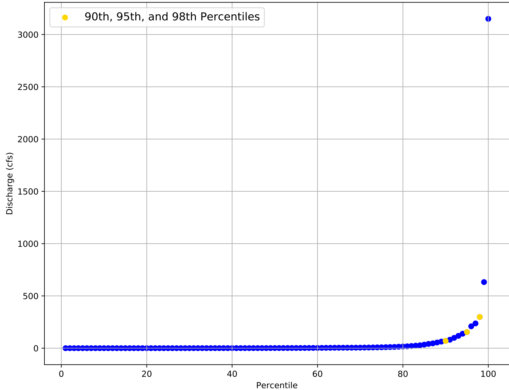
Flow Frequency Distribution for USGS Gage 08062980 from 1982 to 1984
