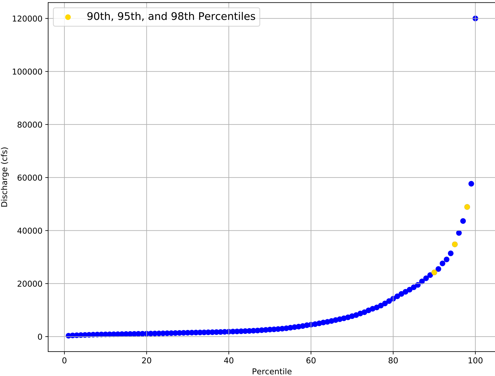
Flow Frequency Distribution for USGS Gage 08066250 from 1965 to 2020
