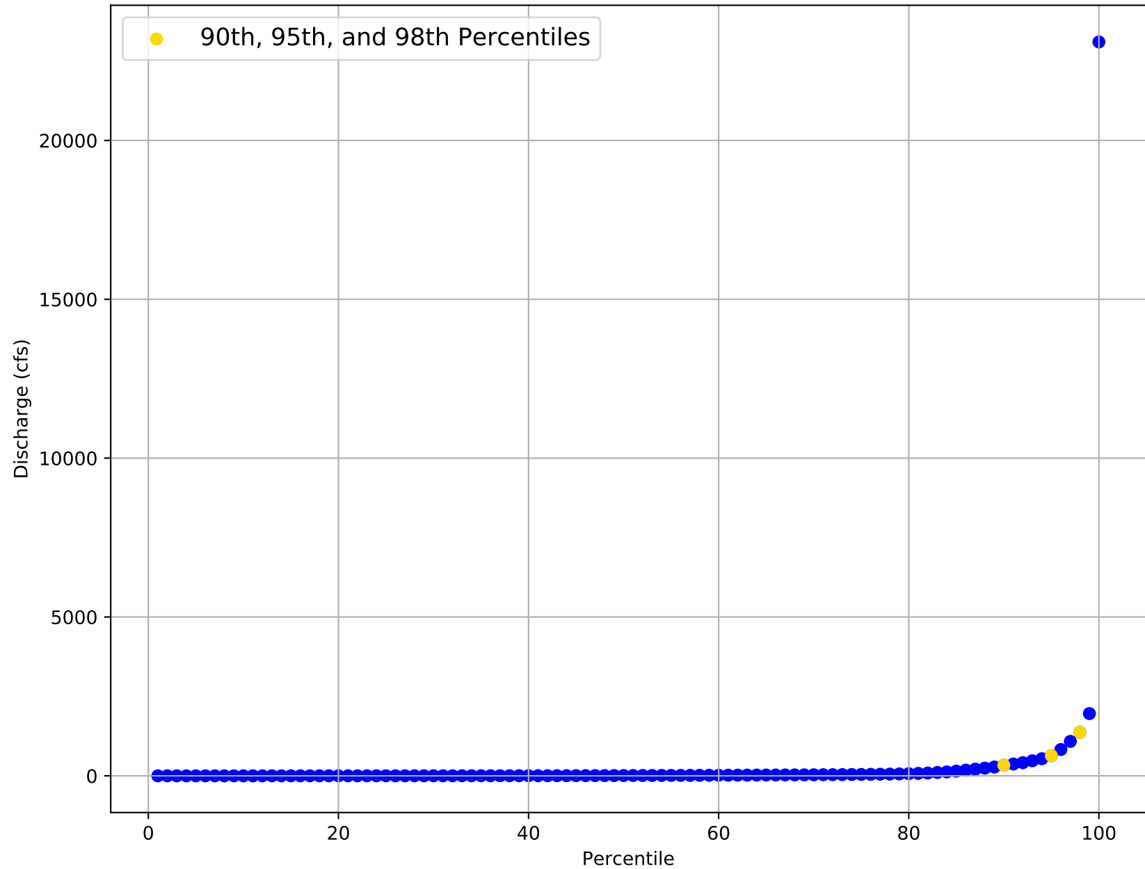
Flow Frequency Distribution for USGS Gage 08099500 from 1939 to 2020
