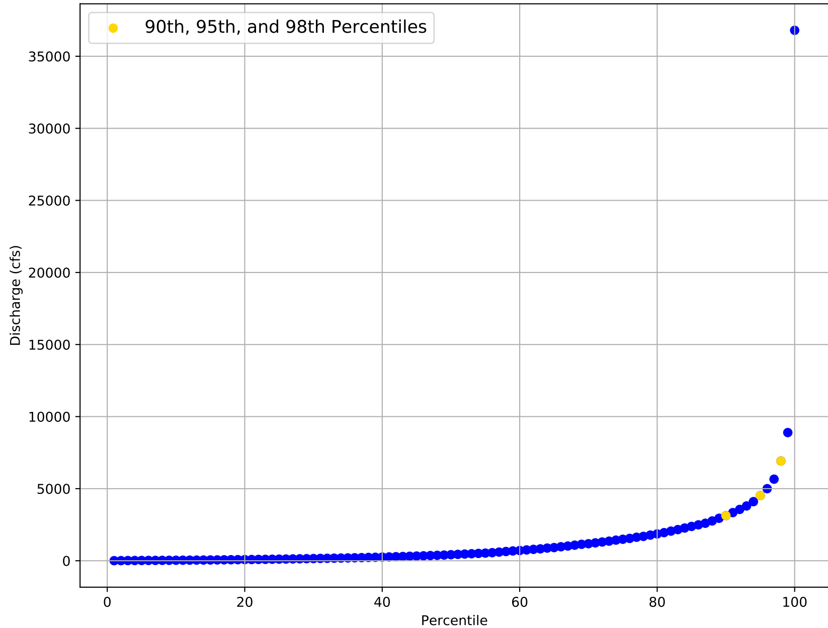
Flow Frequency Distribution for USGS Gage 08037000 from 1923 to 1979
