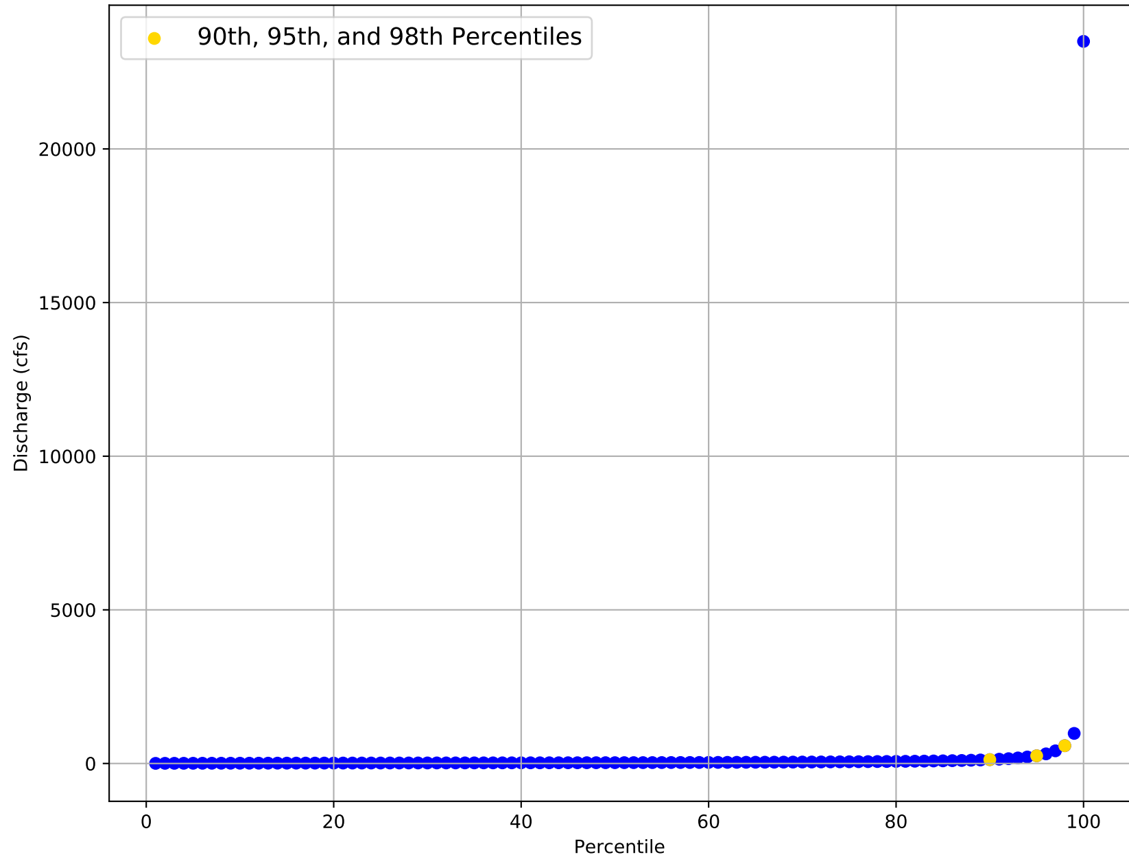
Flow Frequency Distribution for USGS Gage 08071000 from 1943 to 2020
