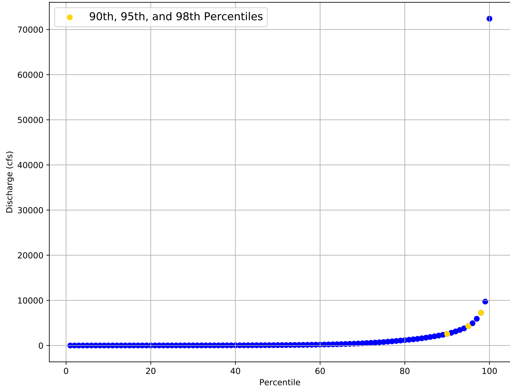
Flow Frequency Distribution for USGS Gage 08018500 from 1939 to 2020
