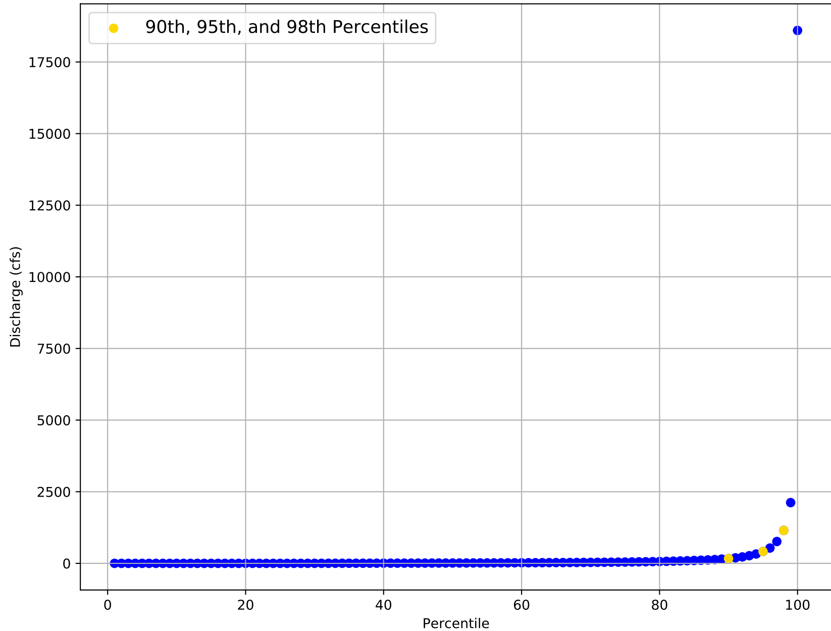
Flow Frequency Distribution for USGS Gage 08053500 from 1949 to 2020
