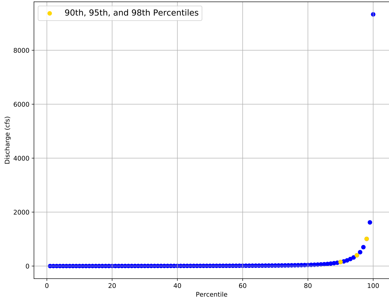
Flow Frequency Distribution for USGS Gage 08067500 from 1971 to 2020
