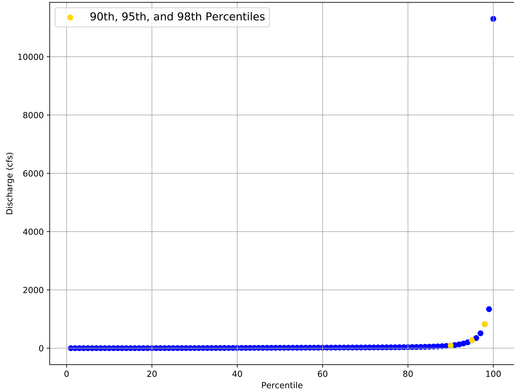
Flow Frequency Distribution for USGS Gage 08109800 from 1962 to 2020
