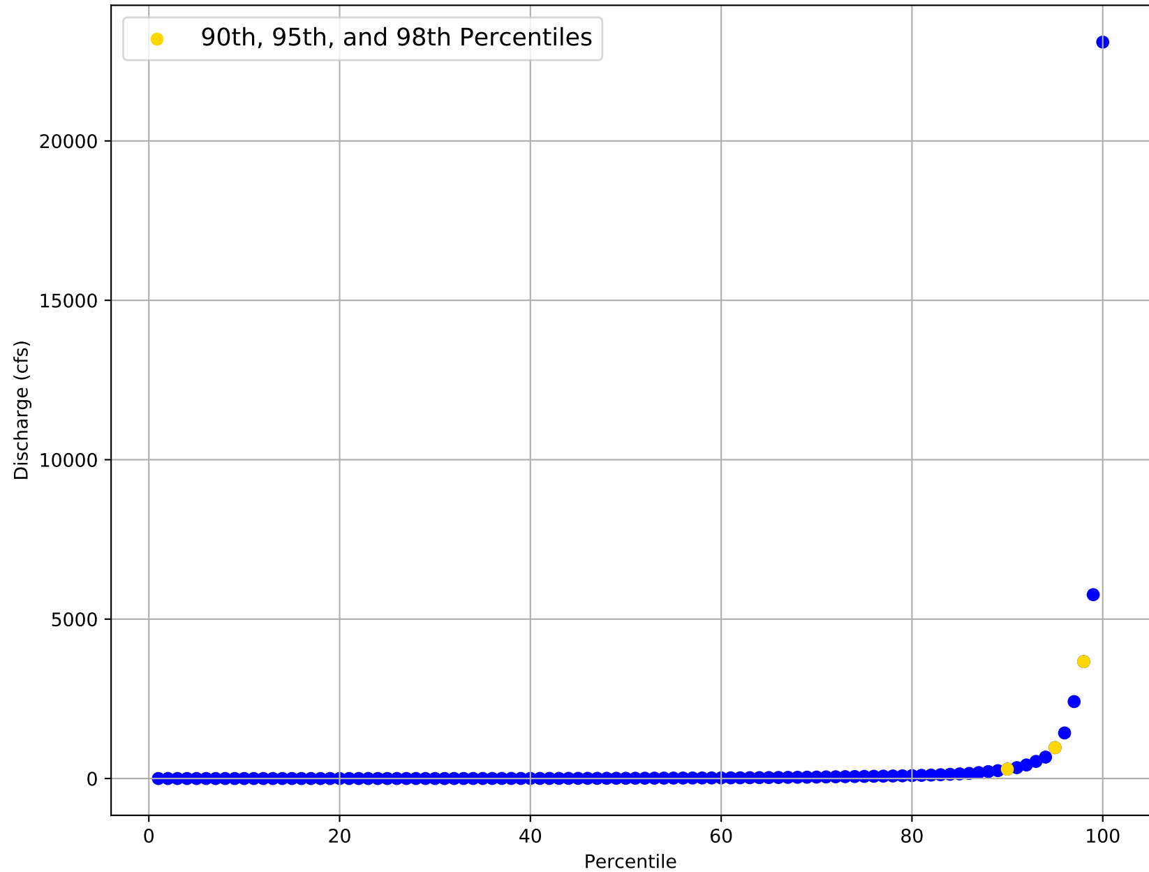
Flow Frequency Distribution for USGS Gage 07332620 from 2006 to 2019
