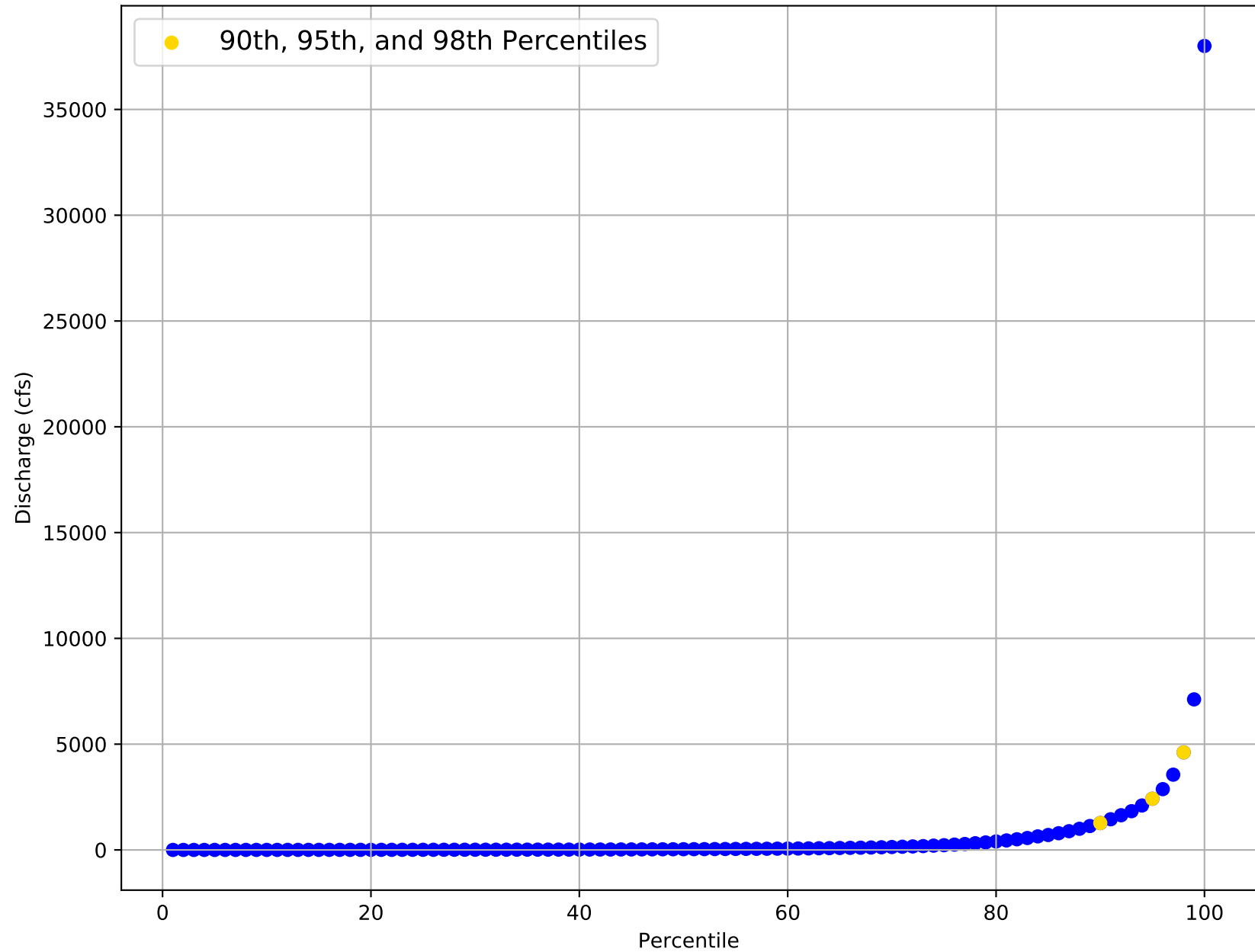
Flow Frequency Distribution for USGS Gage 07343500 from 1949 to 2020
