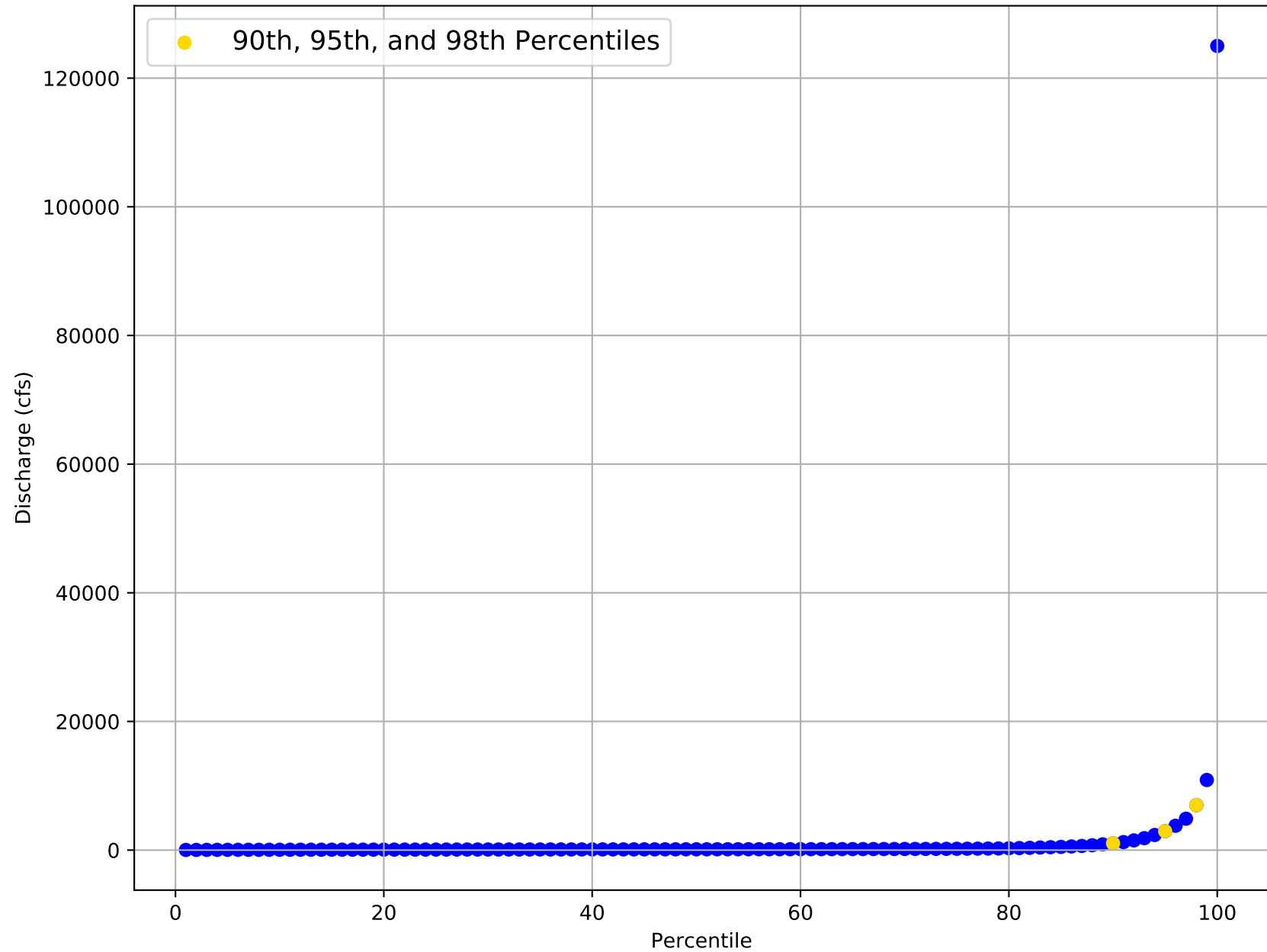
Flow Frequency Distribution for USGS Gage 08211000 from 1939 to 2020
