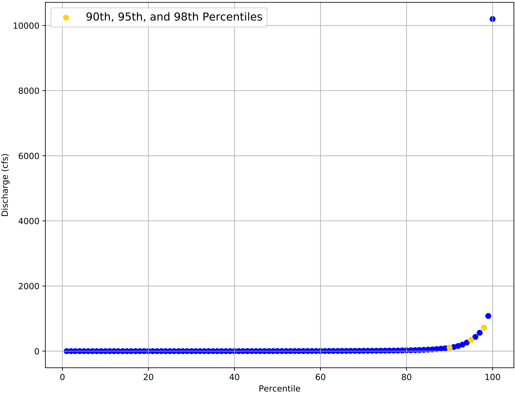
Flow Frequency Distribution for USGS Gage 08068720 from 1975 to 2020
