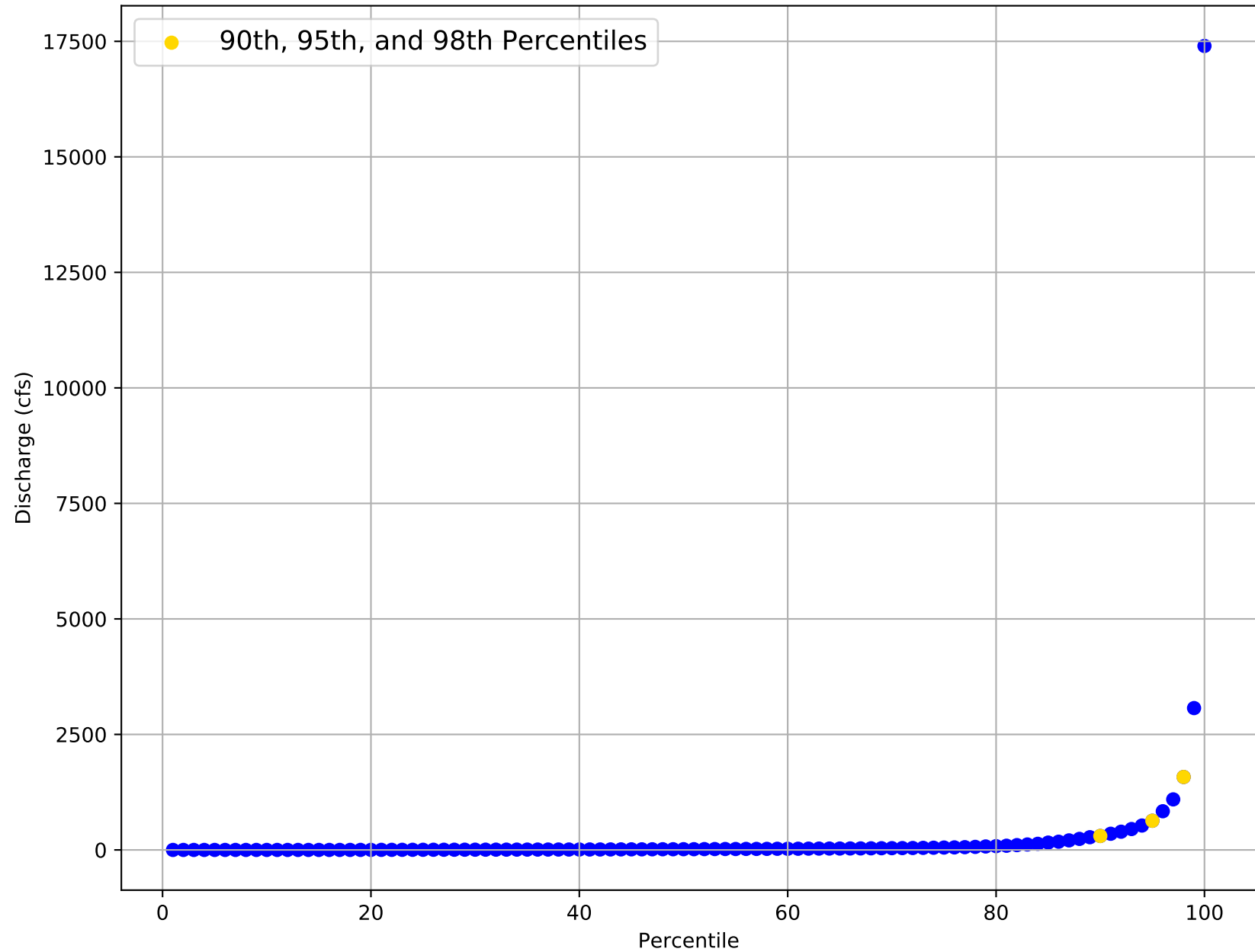
Flow Frequency Distribution for USGS Gage 07227470 from 1968 to 1977
