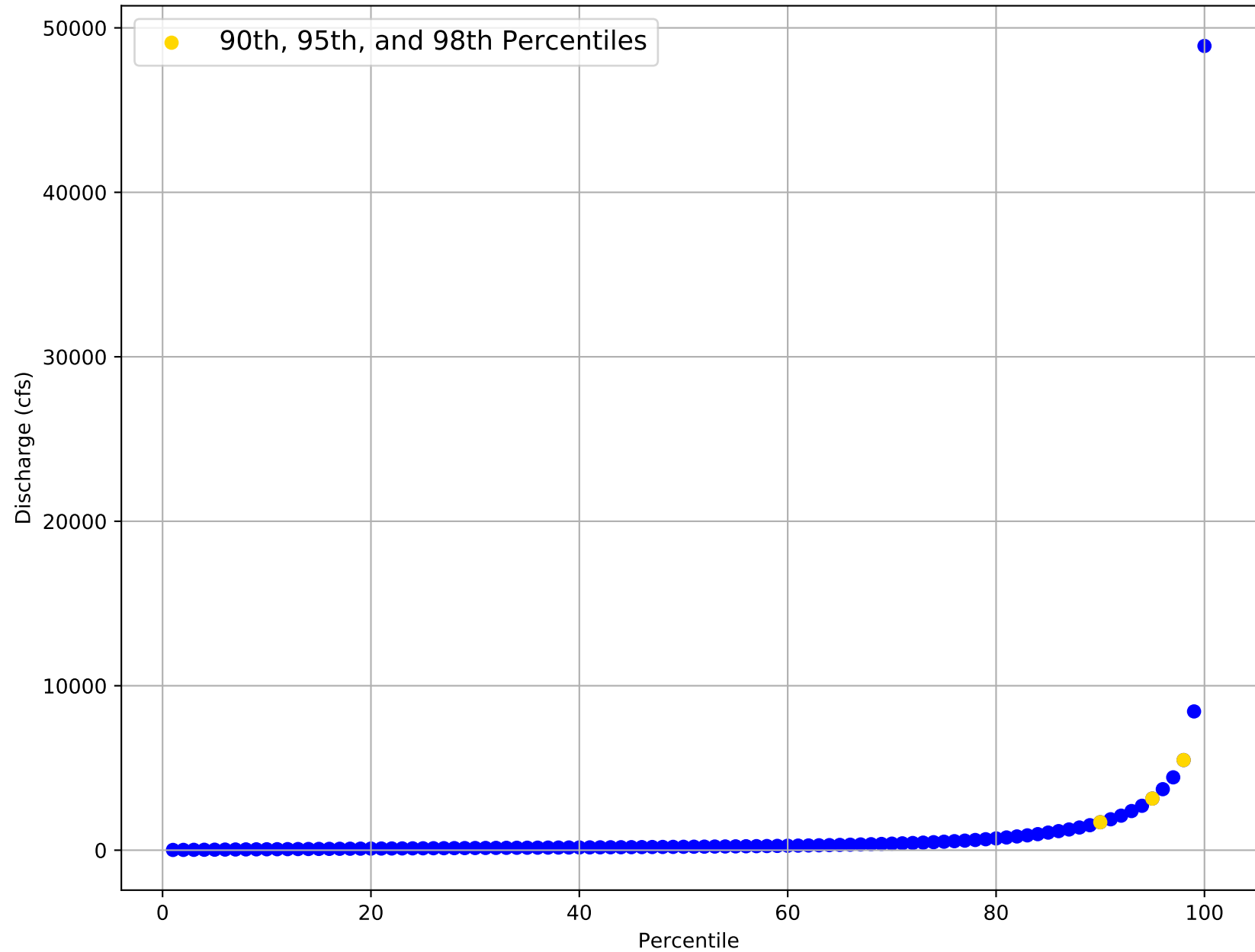
Flow Frequency Distribution for USGS Gage 08049500 from 1925 to 2020
