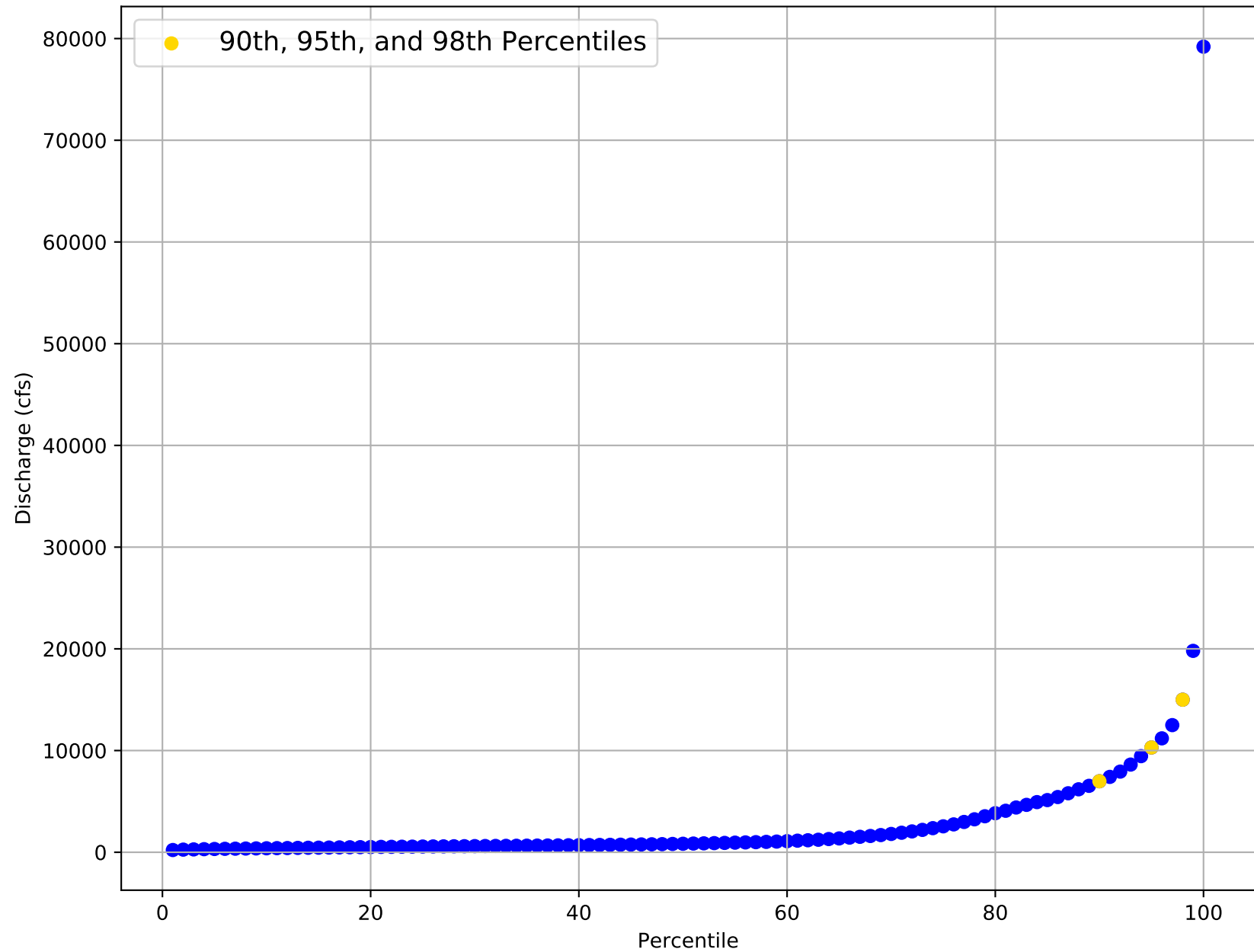
Flow Frequency Distribution for USGS Gage 08057410 from 1956 to 2020
