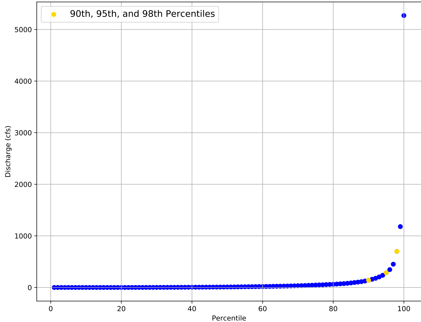
Flow Frequency Distribution for USGS Gage 08059500 from 1949 to 1975
