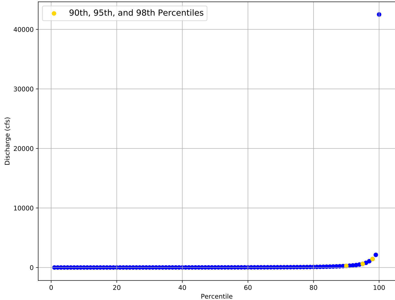
Flow Frequency Distribution for USGS Gage 08047500 from 1924 to 2020
