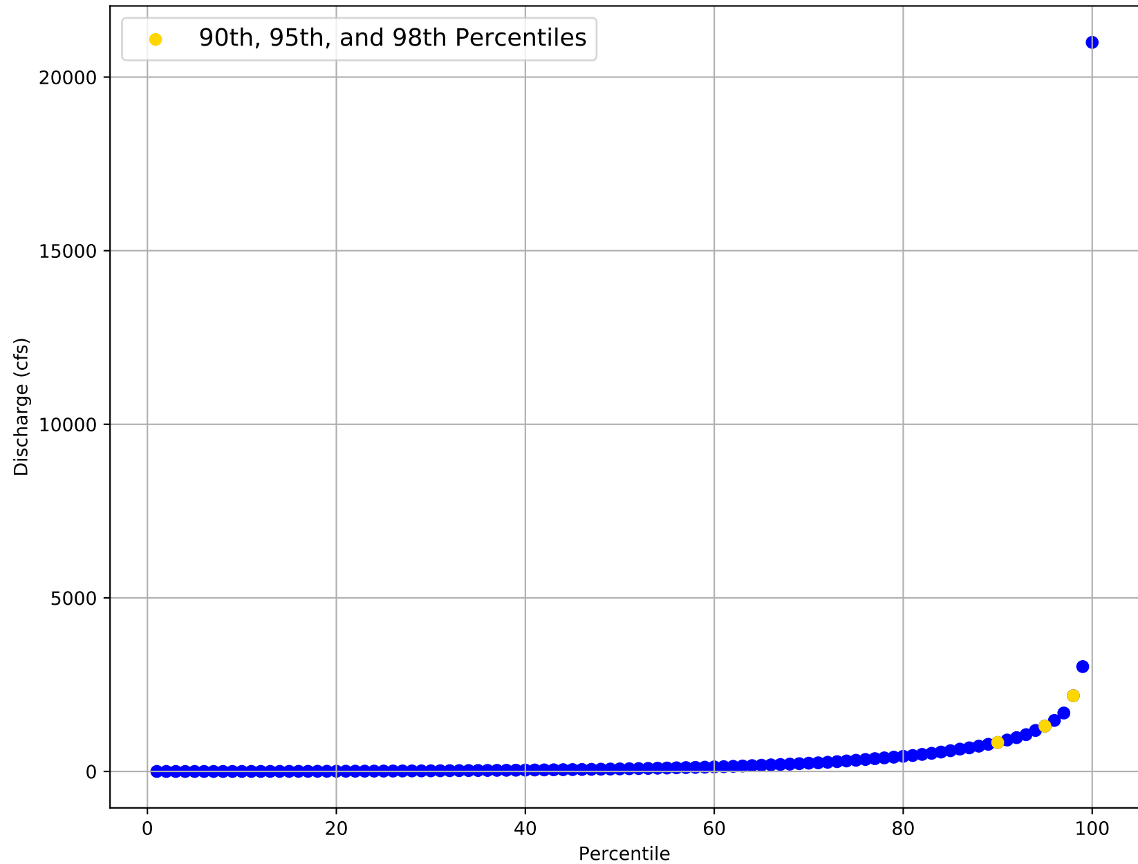
Flow Frequency Distribution for USGS Gage 07346050 from 1962 to 2020
