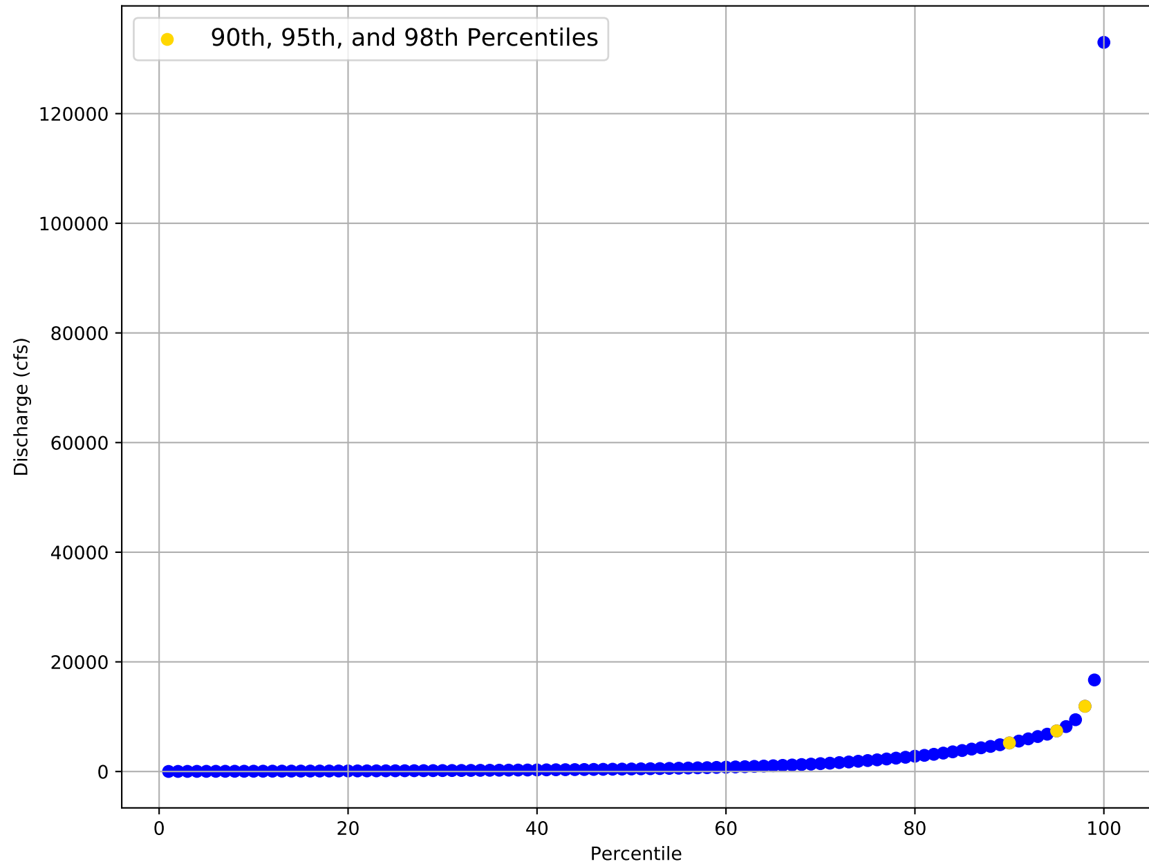
Flow Frequency Distribution for USGS Gage 08020000 from 1932 to 2020
