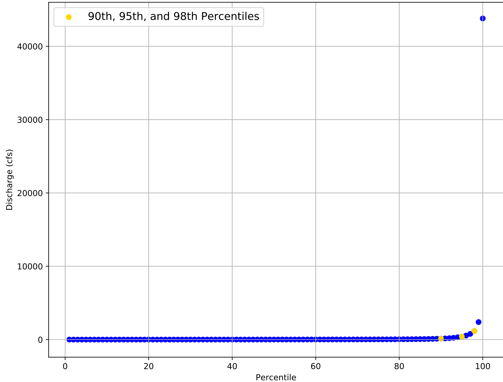
Flow Frequency Distribution for USGS Gage 08173000 from 1930 to 2020
