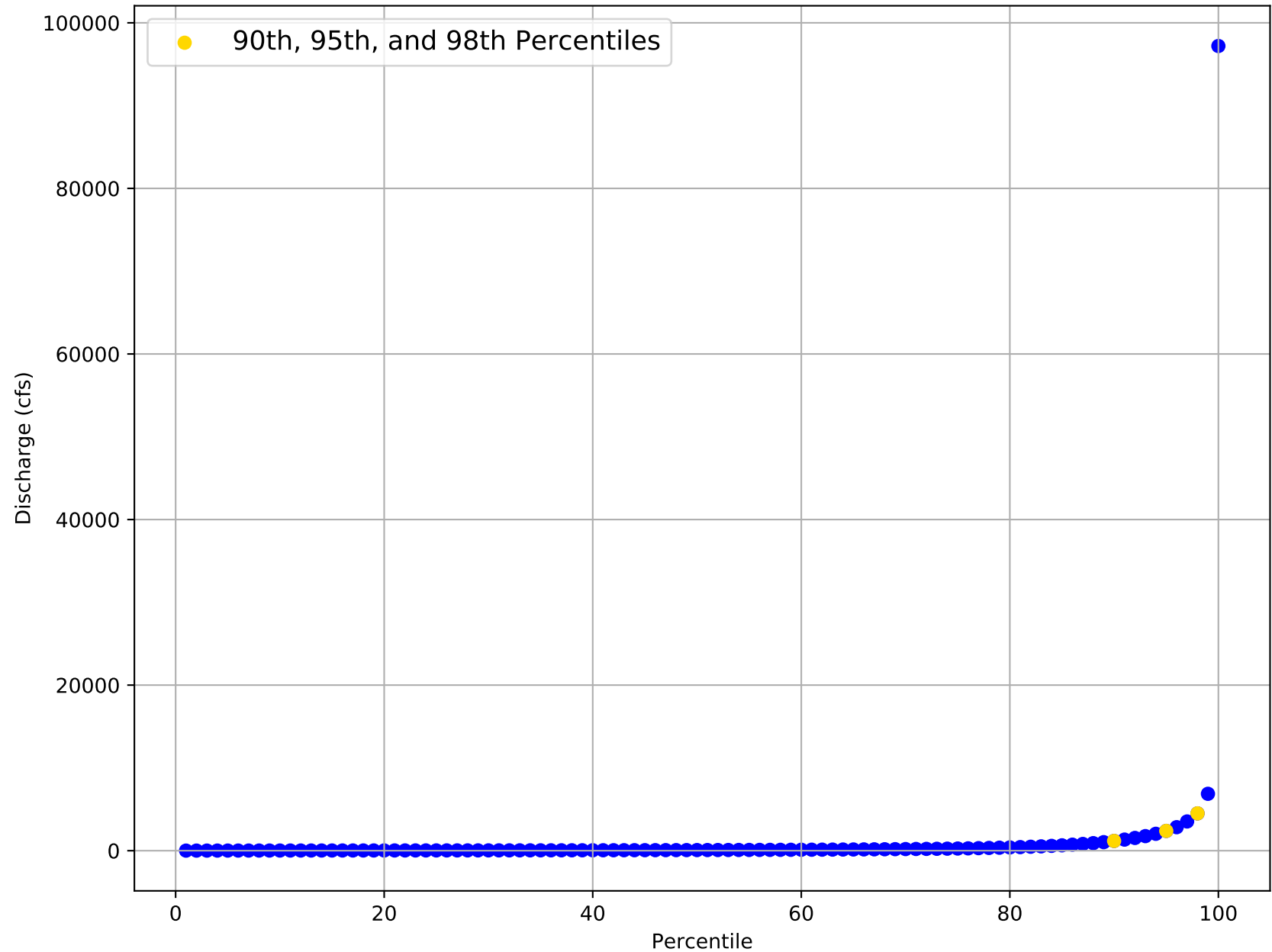
Flow Frequency Distribution for USGS Gage 08068000 from 1924 to 2020
