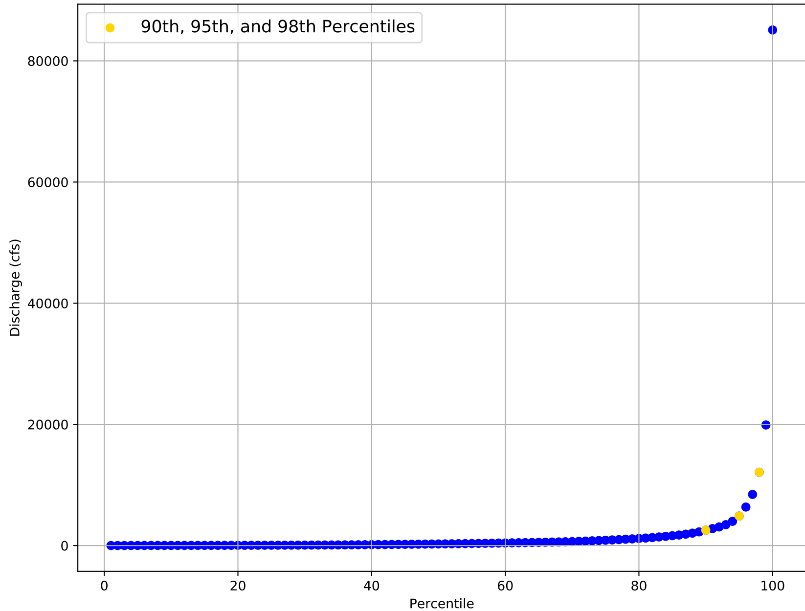
Flow Frequency Distribution for USGS Gage 08091000 from 1923 to 2020
