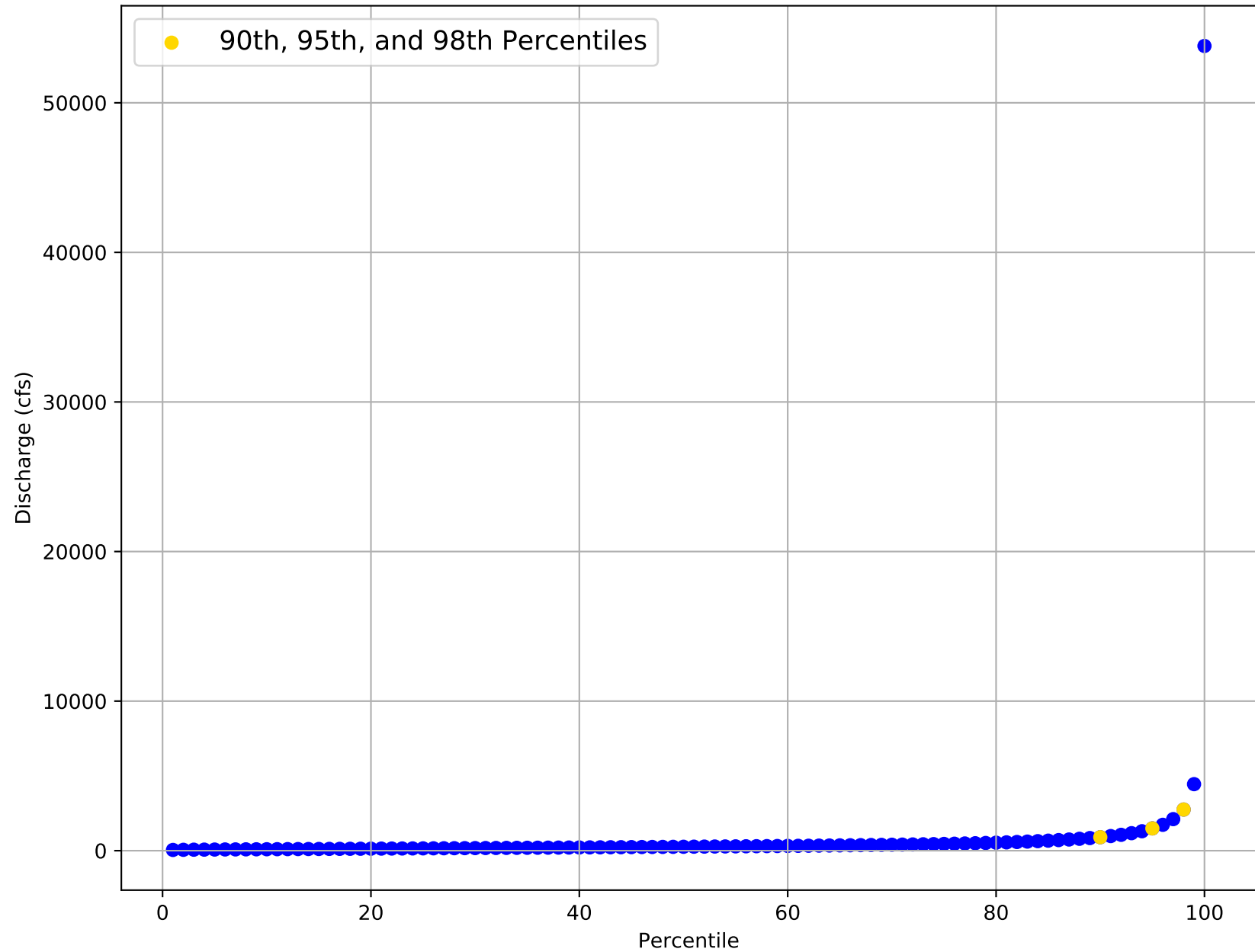
Flow Frequency Distribution for USGS Gage 08183500 from 1925 to 2020
