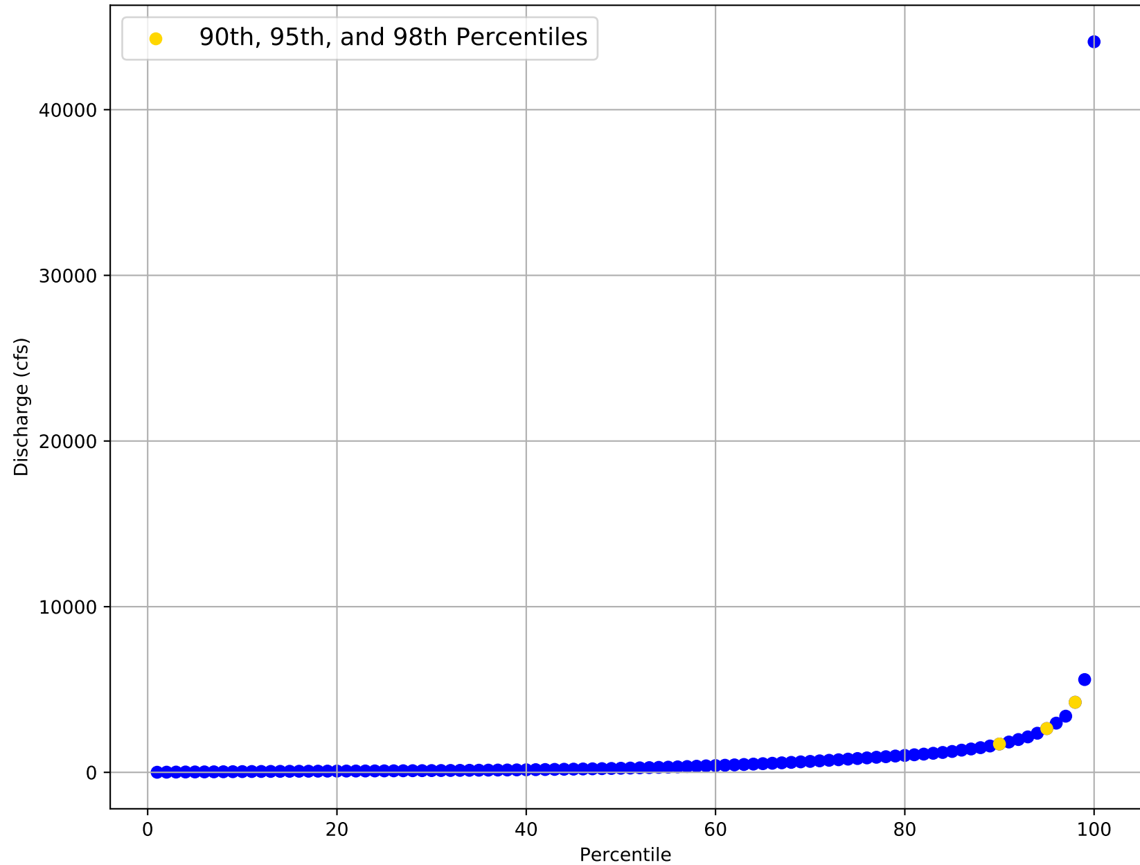
Flow Frequency Distribution for USGS Gage 08032000 from 1939 to 2020
