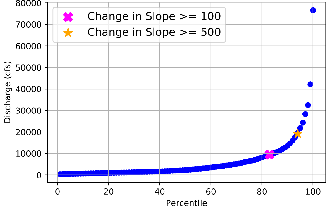
Flow Frequency Distribution for USGS Gage 08110200 from 1965 to 1987
