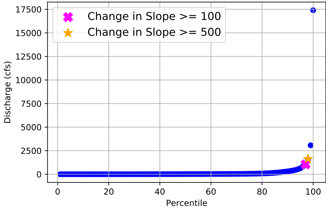
Flow Frequency Distribution for USGS Gage 07227470 from 1968 to 1977
