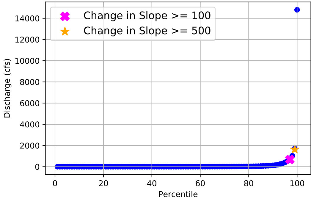
Flow Frequency Distribution for USGS Gage 07336800 from 1962 to 1977
