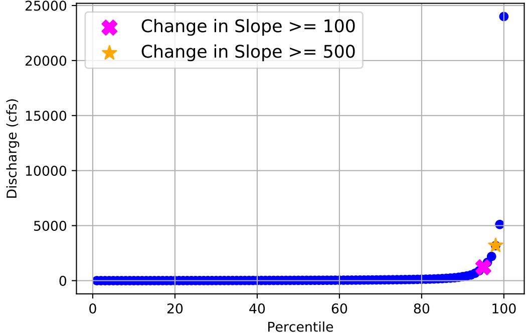
Flow Frequency Distribution for USGS Gage 08164390 from 1996 to 2020
