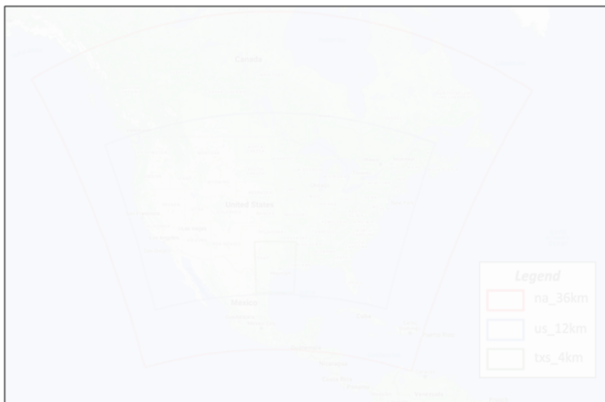
Figure 3-4: CAMx Domains
