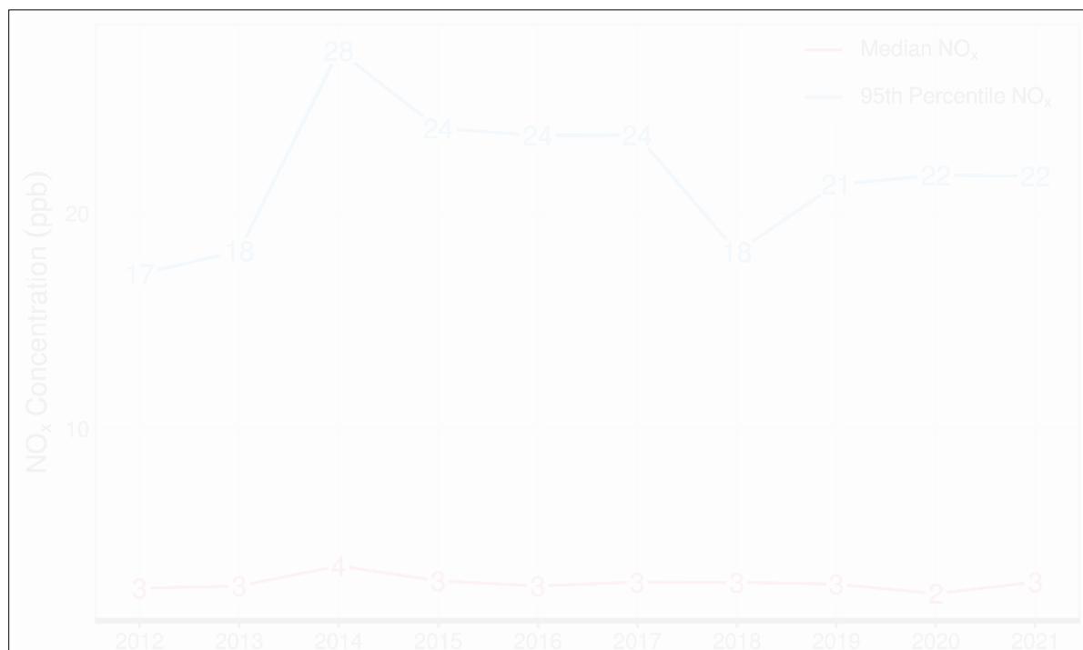
Figure 5-5: Ozone Season \text{NO}_x Trends in Bexar County 2015 Ozone NAAQS Nonattainment Area
