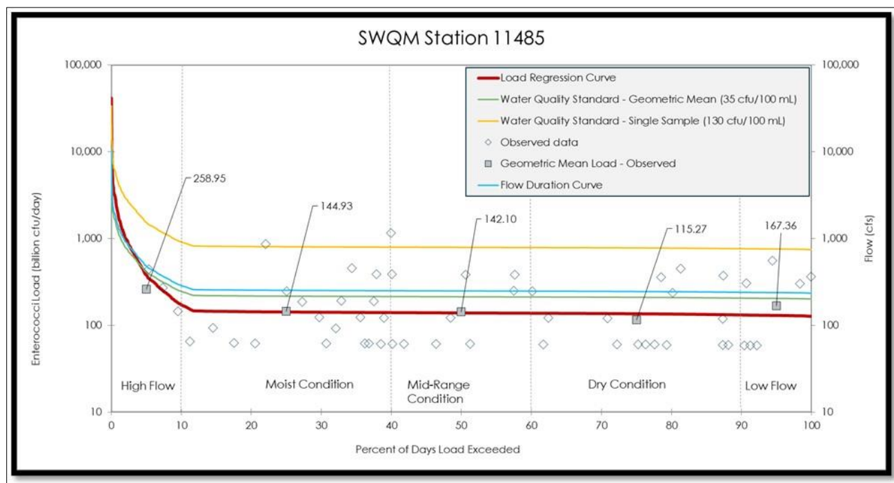
Figure 16. Modified LDC for TCEQ SWQM Station 11485 in Oyster Creek Tidal (AU 1109_01)
