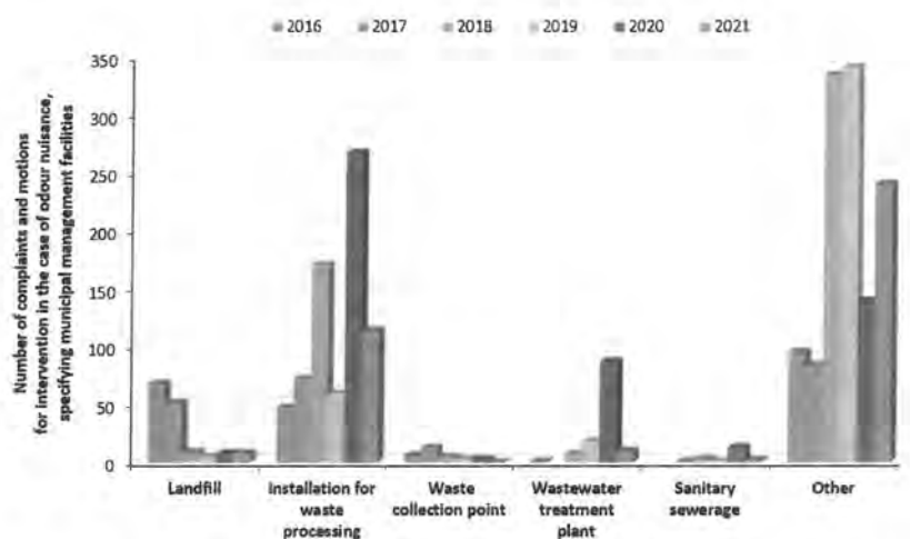
Figure 6. Number of notifications between 2016 and 2021 for odour nuisance of municipal management facilities (own elaboration based on [55]).
