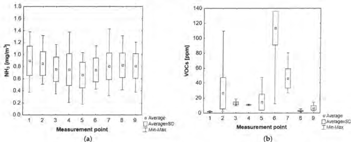
Figure 10. Concentration values at different measurement points of WWTP 1: for (a) ammonia; (b) volatile organic compounds (own elaboration based on [60]). 1—entrance to the wastewater treatment plant, 2—expansion chamber, 3—mechanical treatment block, 4—measurement directly over the screen, 5—measurement directly over the grit chamber, 6—outlet from the biofilter, 7—biological treatment block, 8—sludge lagoon 1 (aeration off), 9—sludge lagoon 2 (aeration on).
