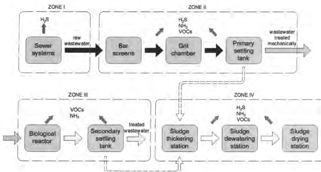
Figure 1. Emission zones at the WWTPs and types of hazardous substances to health emitted from them (own elaboration).
