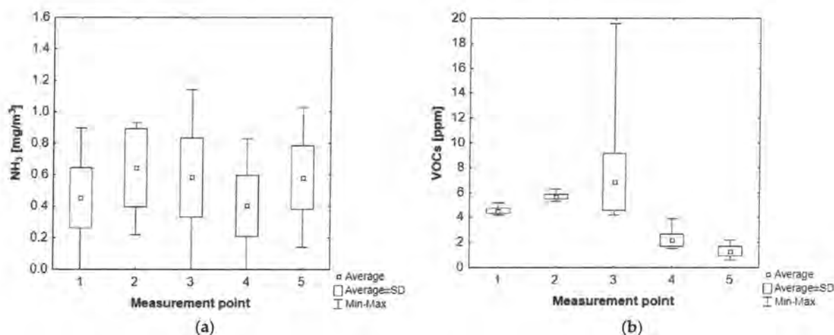
Figure 11. Concentration values at different measurement points of WWTP 2: for (a) ammonia; (b) volatile organic compounds (own elaboration based on [60]). 1—entrance to the wastewater treatment plant, 2—mechanical treatment block, 3—biological treatment block, 4—sludge lagoon (aeration on), 5—container with screenings.
