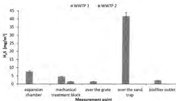
Figure 9. Concentration of hydrogen sulphide in WWTP 1 and WWTP 2 (Poland) at different measurement points (own elaboration based on [60]).
