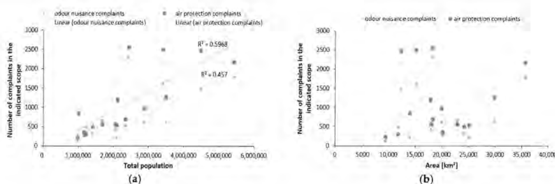
Figure 8. Number of complaints and applications handled in the field of air protection and odour nuisance in relation to: (a) total population of the voivodeship; (b) area of the voivodeship.
