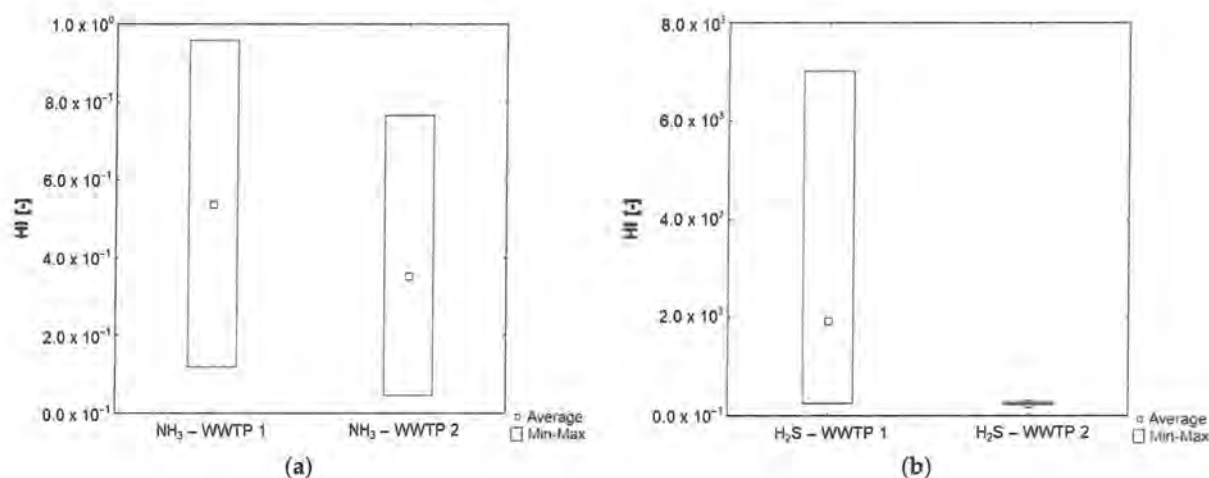
Figure 12. Ranges of hazard index (HI) parameter determined for ammonia (a) and hydrogen sulphide (b) (HI values were determined by the method proposed by [7], assuming that daily exposure time is 6 h/day, exposure frequency is 350 days/year, exposure duration is 35 years, average time is 25 years for non-carcinogenic risks. According to [71], the reference concentration for NH 3 and H 2 S was assumed 5.0 \times 10^{-1} mg/m 3 and 2.0 \times 10^{-3} mg/m 3 , respectively).
