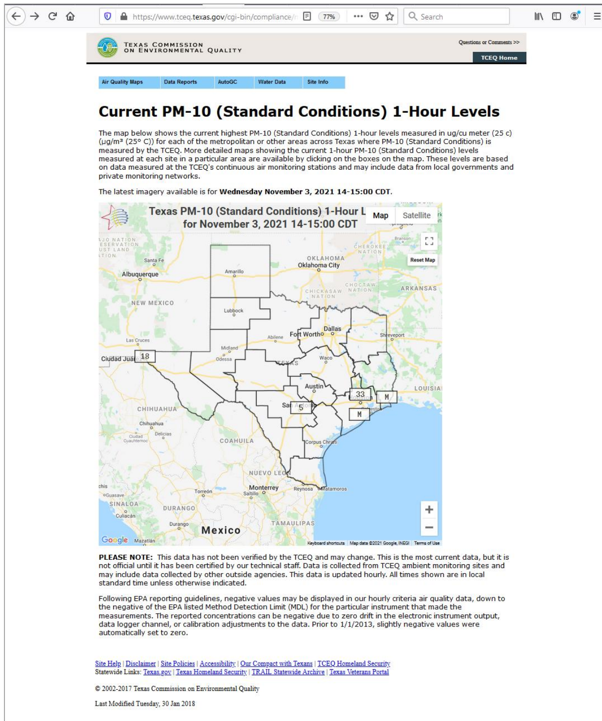
Figure E-3: Sample of the TCEQ Map of Current PM 10 Levels
