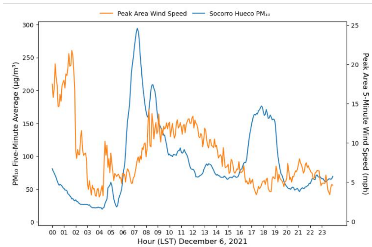
Figure D-4: Continuous Five-Minute PM 10 and Peak Area Five-Minute Sustained Wind Speed Measurements on December 6, 2021
