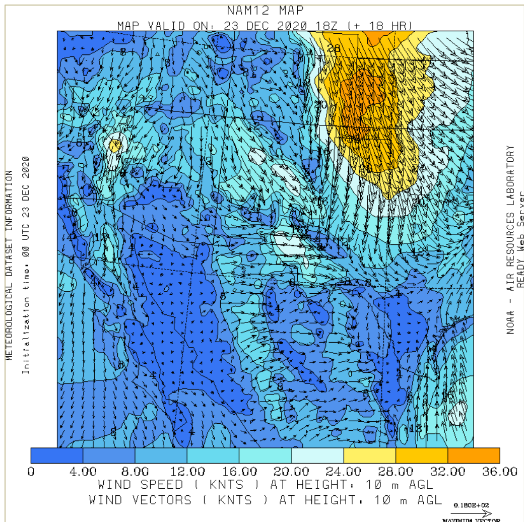
Figure B-19: NOAA ARL Model Wind Field in the Southeast United States at 13:00 CST on January 15, 2021
