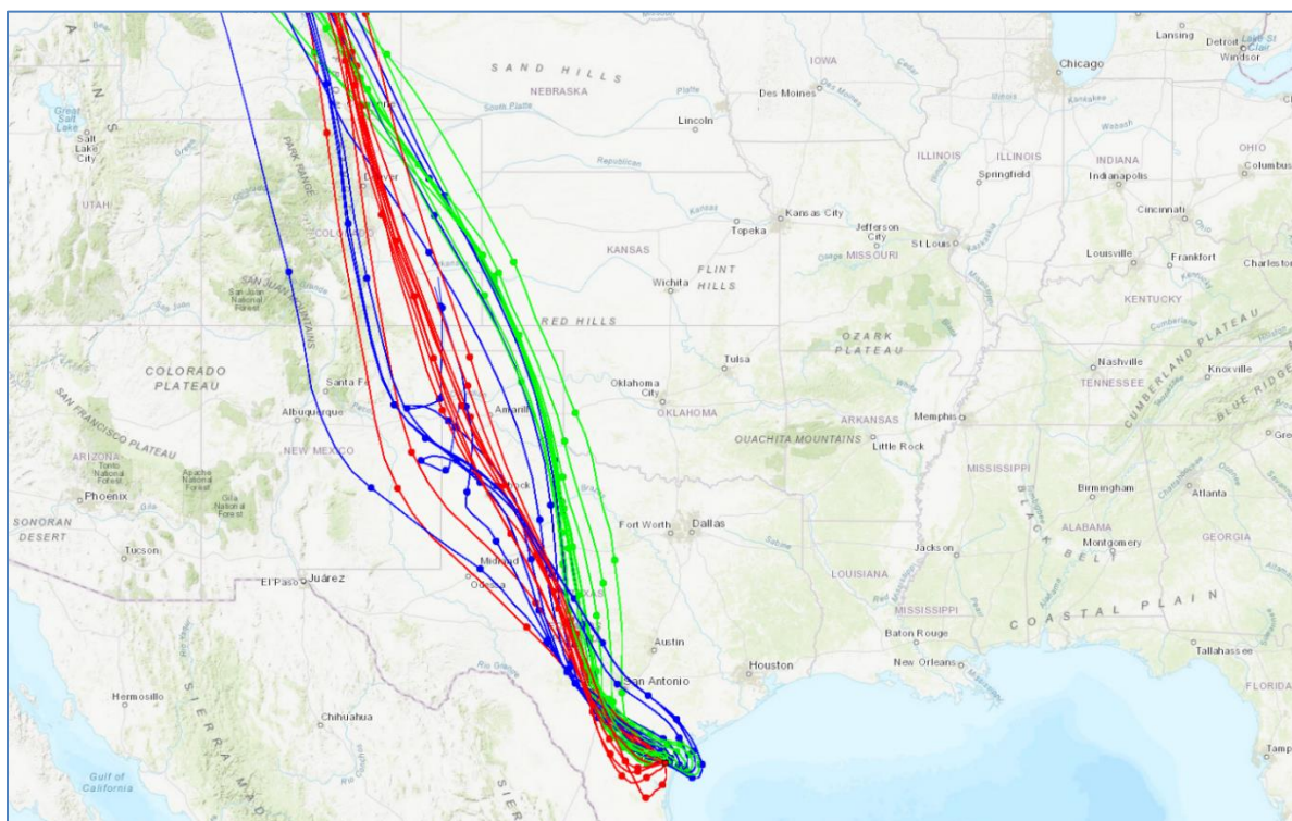
Figure B-5: HYSPLIT Backward Trajectories (Every 2 Hours on Jan. 16, 2021) at 10, 100, and 1000 m AGL at Dona Park
