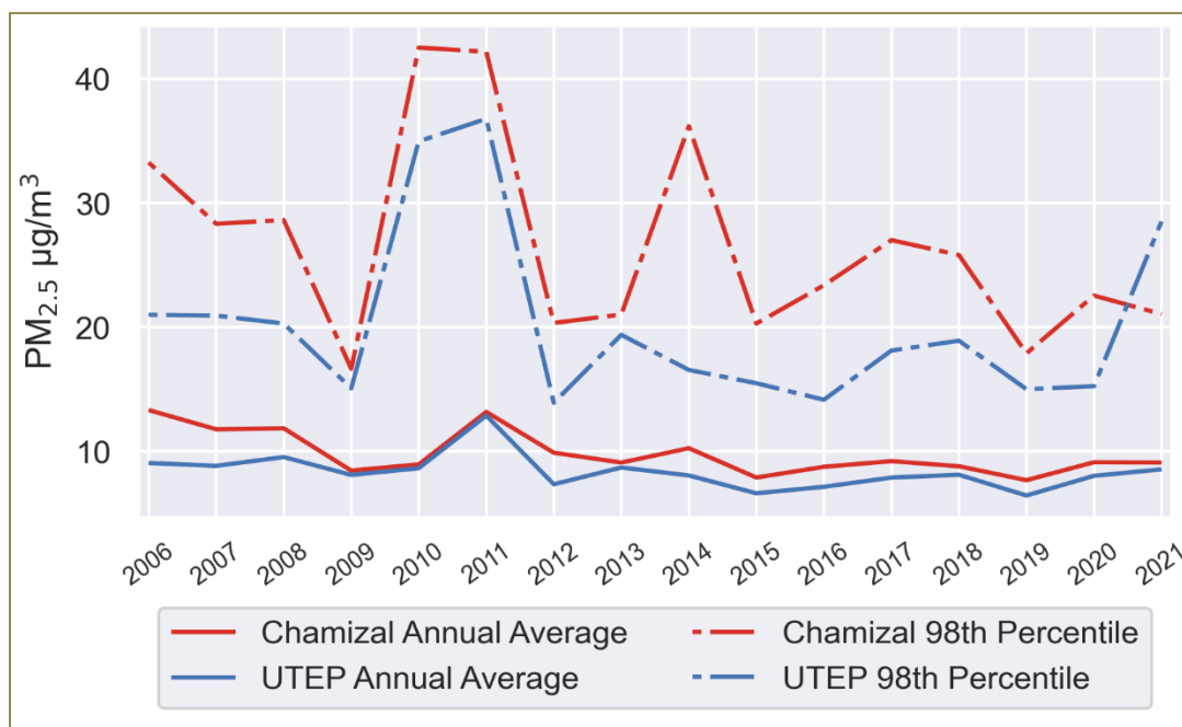
Figure 2-11: El Paso County PM 2.5 Annual Averages and Annual 98th Percentile of 24-hour Averages for Long-Term FRM Monitoring Sites, Including Exceptional Event Days
