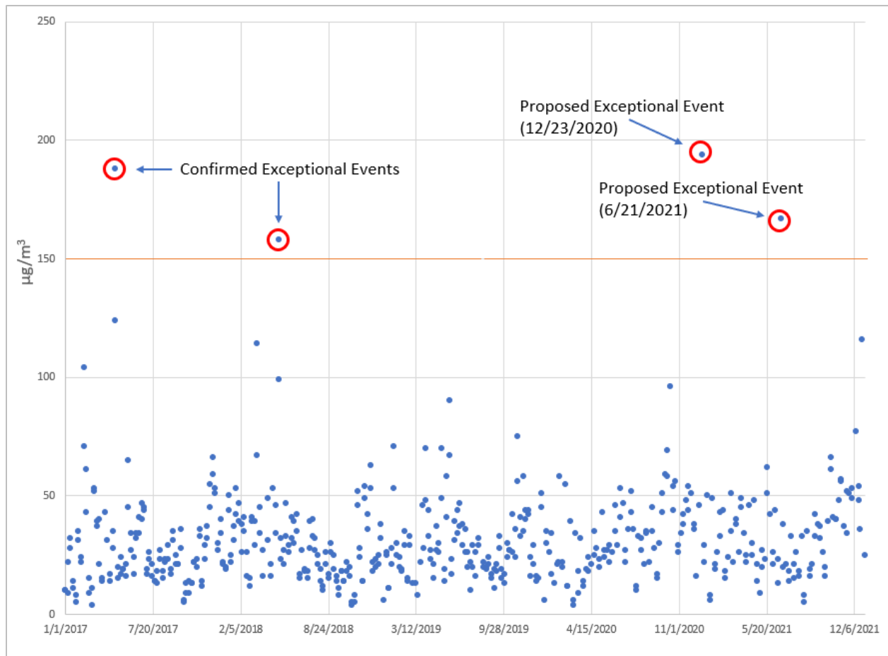
Figure 5-3: Socorro Hueco (C49) FRM PM 10 Daily Measurements from 2017 through 2021
