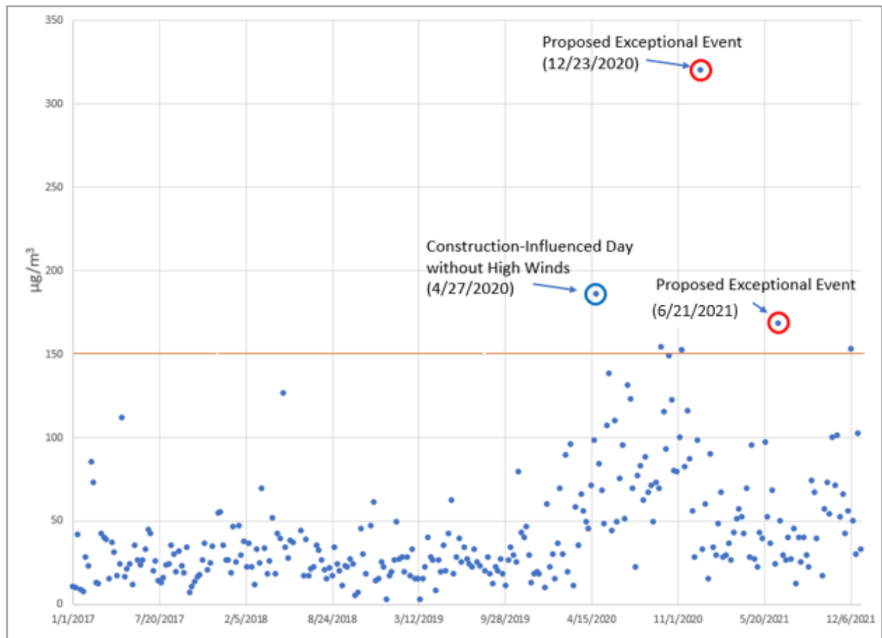
Figure 5-4: Riverside/El Paso Mimosa (C9996) FRM PM 10 Daily Measurements from 2017 through 2021
