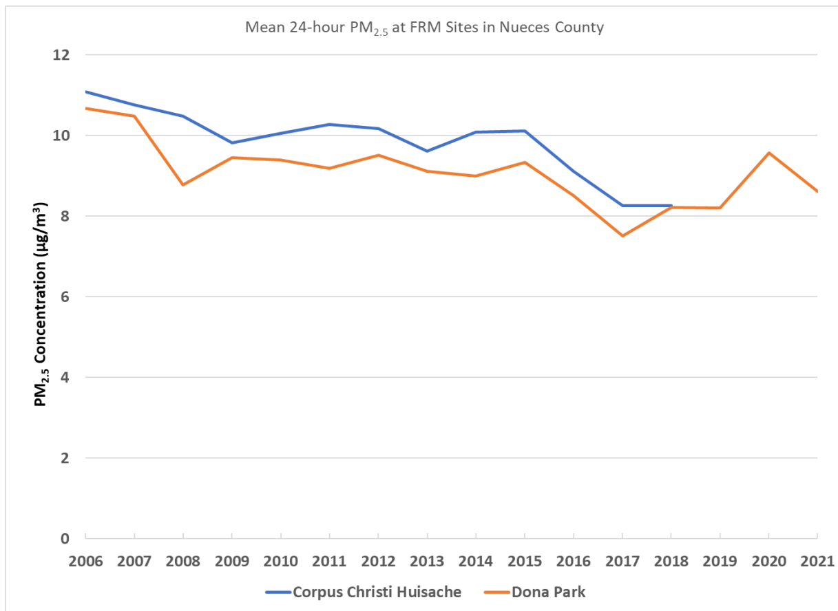
Figure 2-8: Nueces County PM 2.5 Annual 24-hour Averages for Long-Term FRM Monitoring Sites, Including Exceptional Event Days
