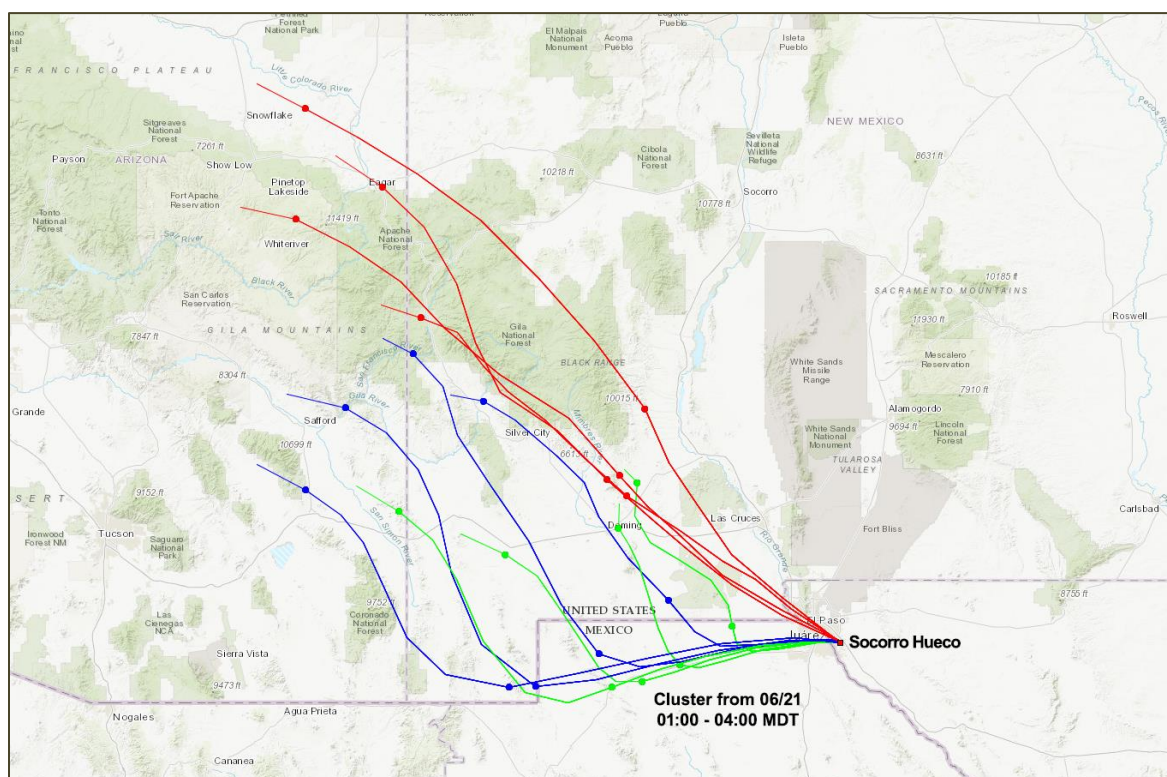
Figure C-3: HYSPLIT Backward Trajectories (June 21, 2021 from 01:00 through 04:00 MDT) at 10, 100, and 1,000 m AGL
