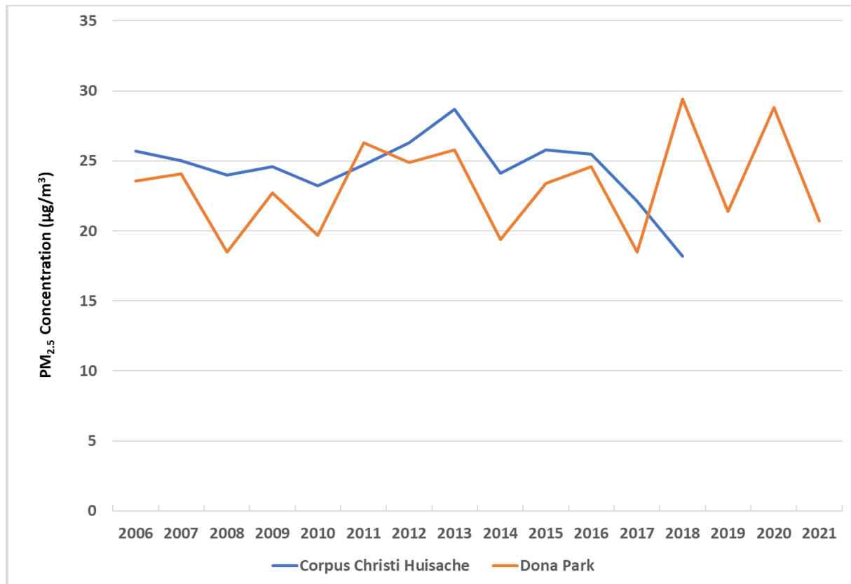
Figure 2-9: Nueces County Annual 98th Percentile of 24-hour Averages for Long-Term FRM Monitoring Sites, Including Exceptional Event Days
