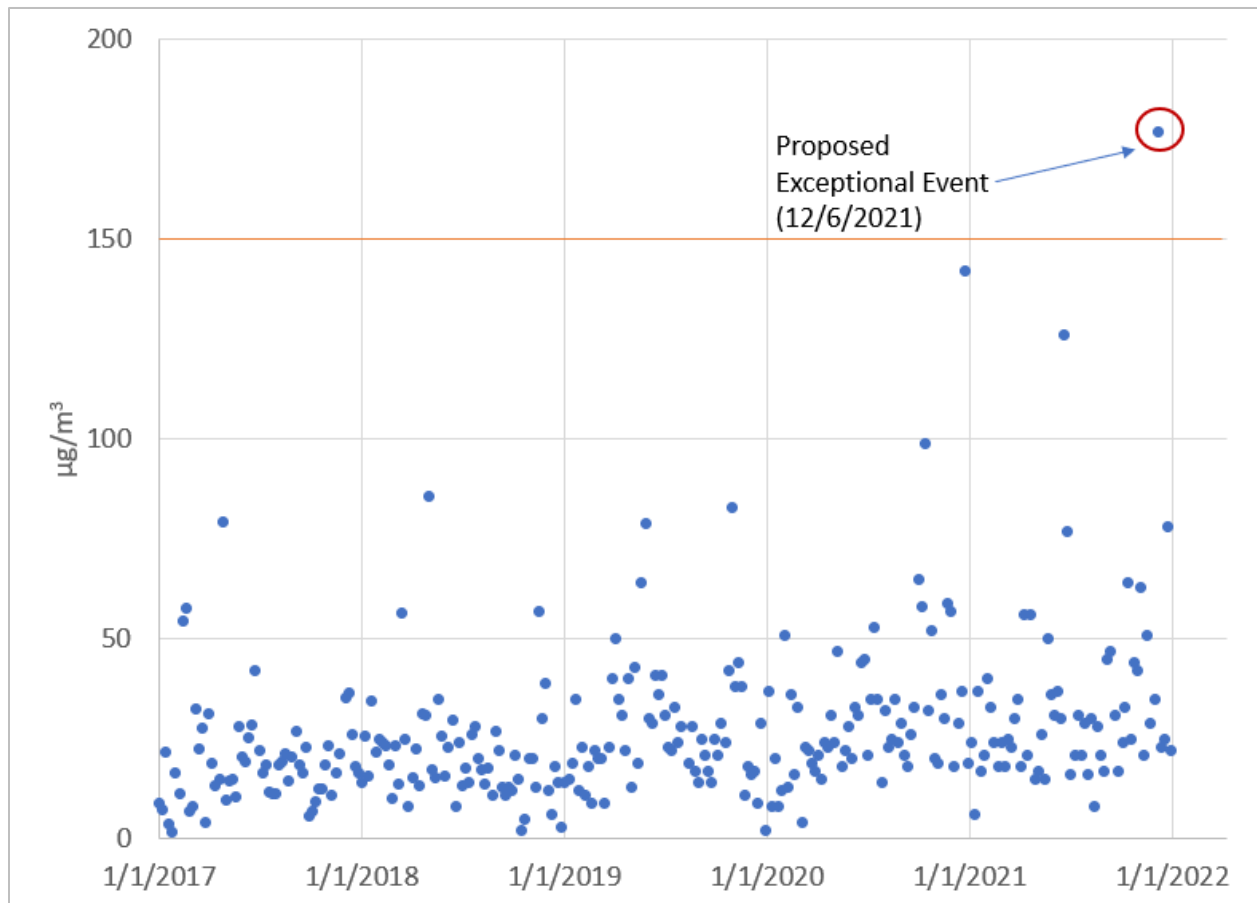
Figure 5-5: Ivanhoe (C414) FRM PM 10 Daily Measurements from 2017 through 2021
