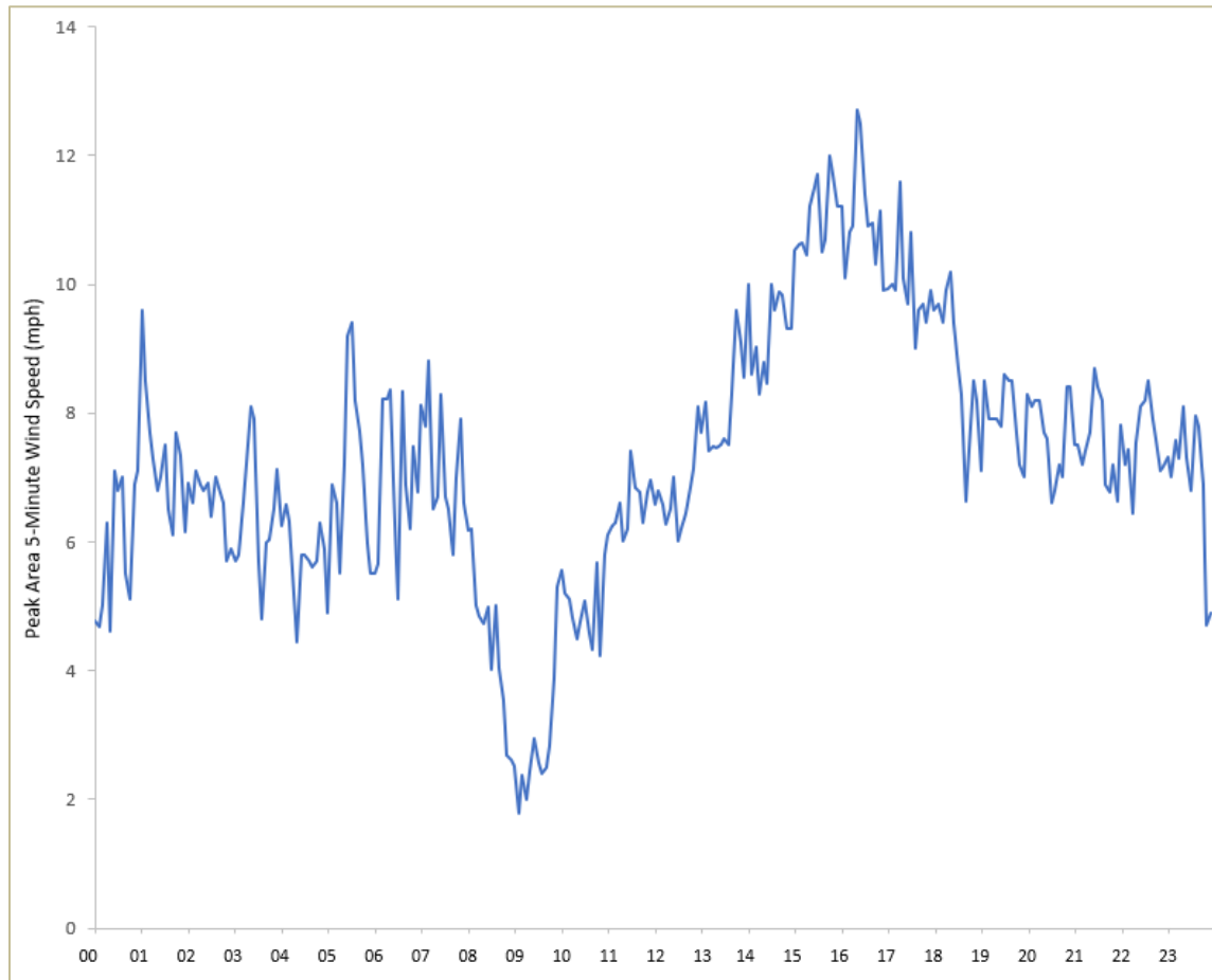
Figure B-11: Nueces County Peak Area Five-Minute Sustained Wind Speed Measurements on January 16, 2021
