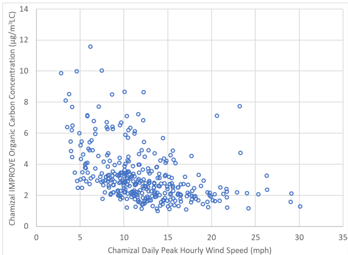
Figure C-9: El Paso Chamizal (C41) PM 2.5 IMPROVE Organic Carbon Concentration versus El Paso Chamizal (C41) Daily Peak Hourly Wind Speed for 2019 through 2021
