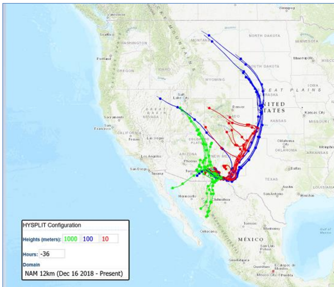
Figure D-2: HYSPLIT Backward Trajectories (June 21, 2021 from 01:00 through 04:00 MDT) at 10, 100, and 1,000 m AGL
