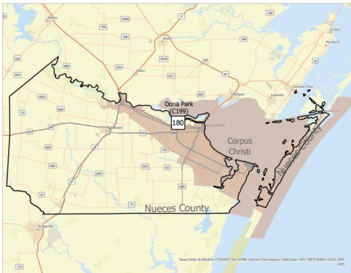
Figure B-7: Daily Average PM 10 Measurements (µg/m 3 ) in Nueces County on January 21, 2021
