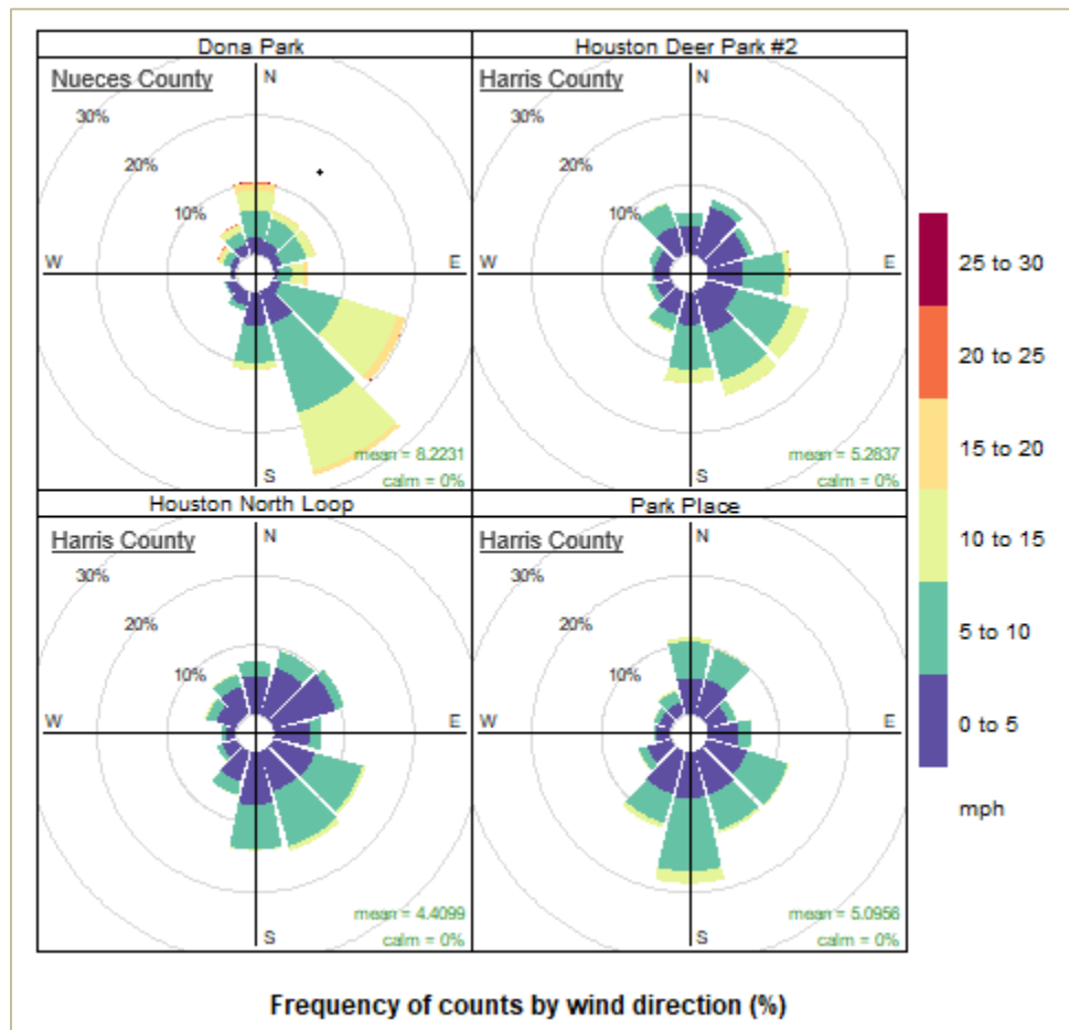
Figure 3-4: Wind Rose Plots for Harris County and Nueces County Monitors for 2019 through 2021
