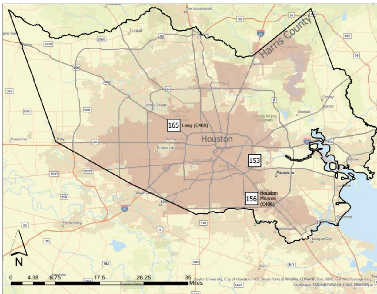
Figure B-6: Daily Average PM_{10} Measurements ( \mu g/m^3 ) in Harris County on January 16, 2021
