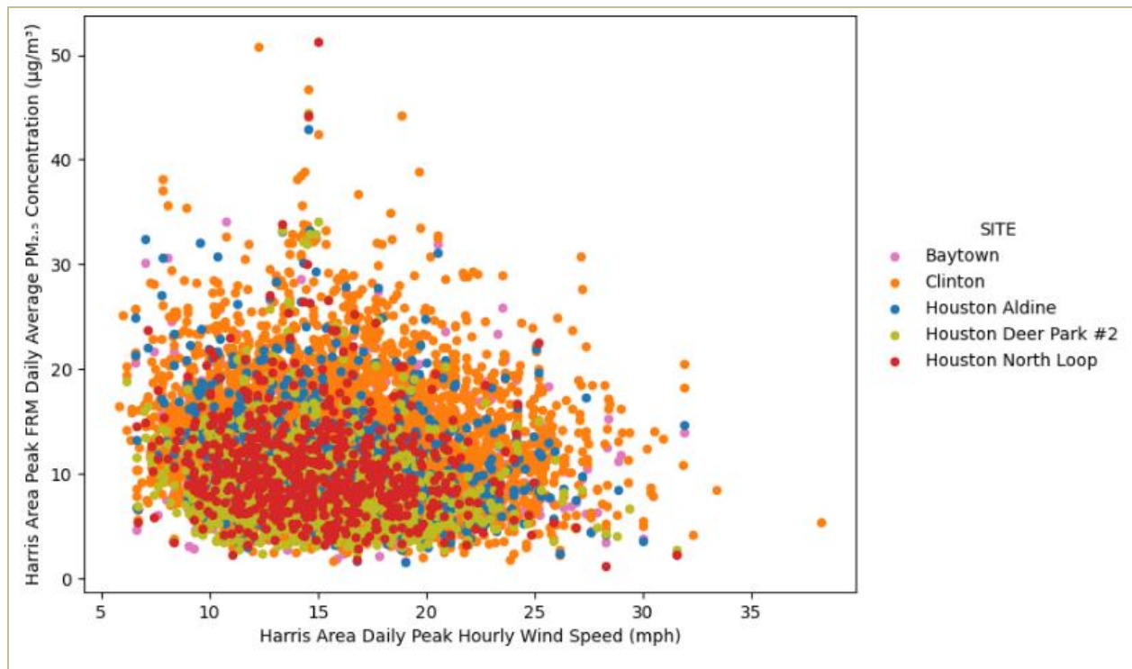
Figure 2-13: Harris County Daily Peak PM_{2.5} Average for FRM Measurements versus Harris County Daily Peak Sustained Hourly Wind Speed for 2006 through 2021
