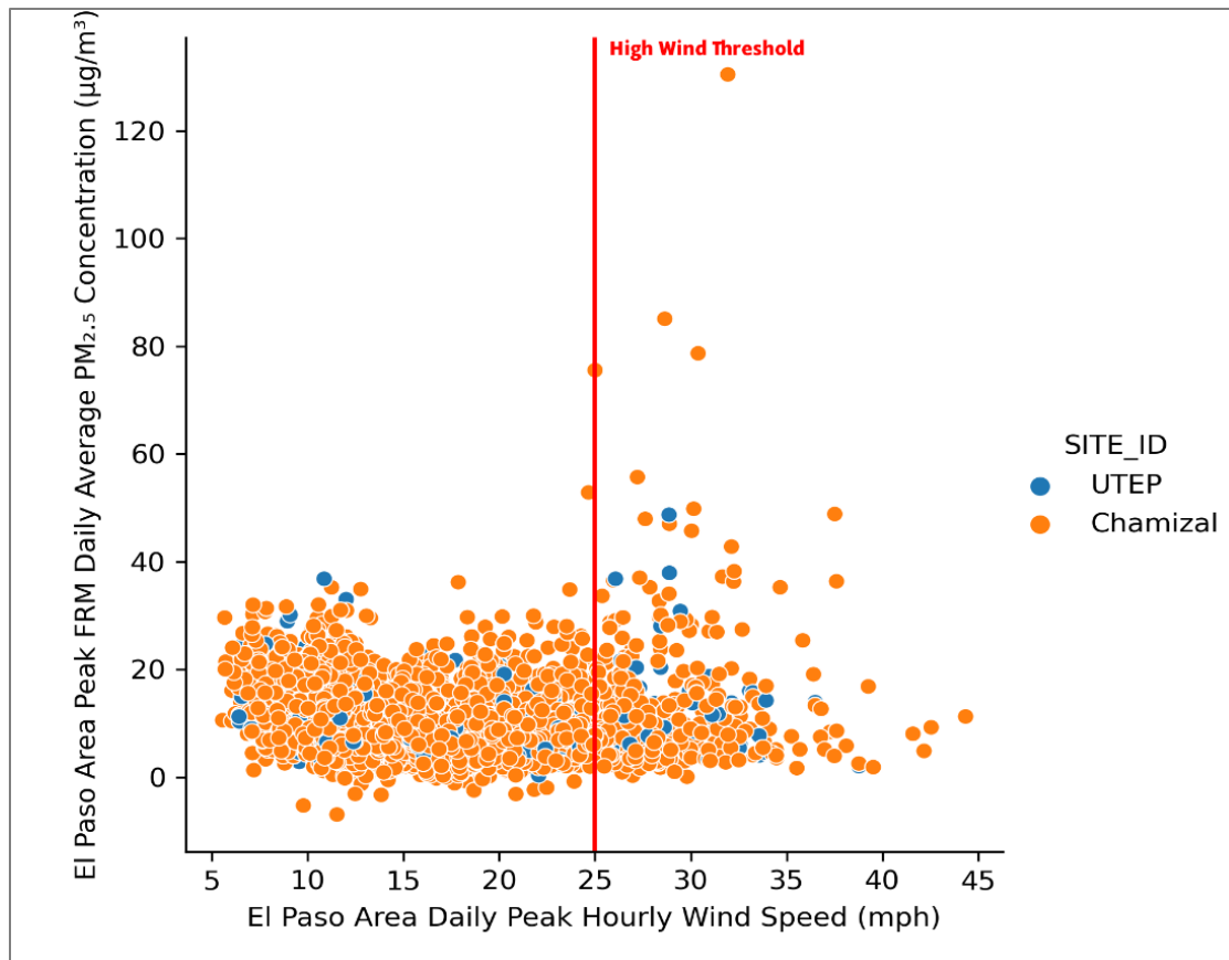
Figure 2-19: El Paso County Daily Peak PM_{2.5} Average for FRM Measurements versus El Paso County Daily Peak Sustained Hourly Wind Speed for 2006 through 2021
