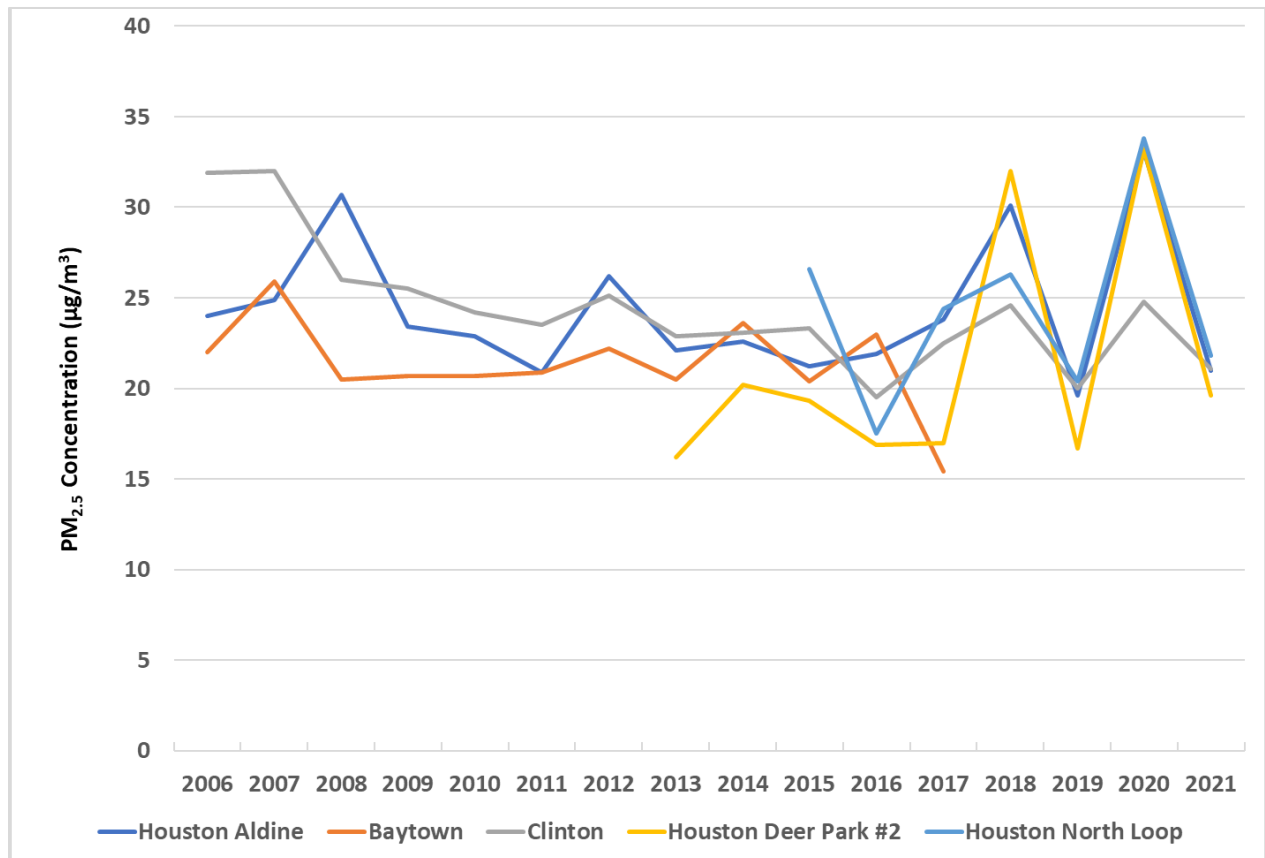
Figure 2-6: Harris County Annual 98th Percentile of 24-hour Averages for Long-Term FRM Monitoring Sites, Including Exceptional Event Days
