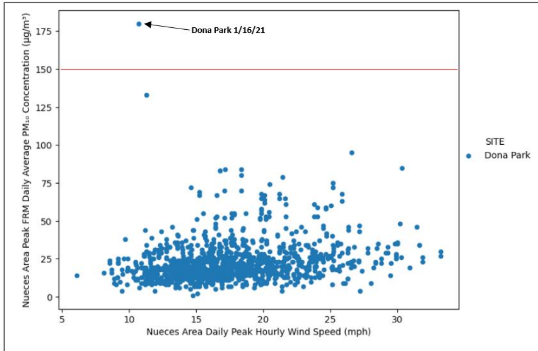
Figure 2-16: Nueces County Daily Peak PM_{10} Average for FRM Measurements versus Nueces County Daily Peak Sustained Hourly Wind Speed for 2006 through 2021
