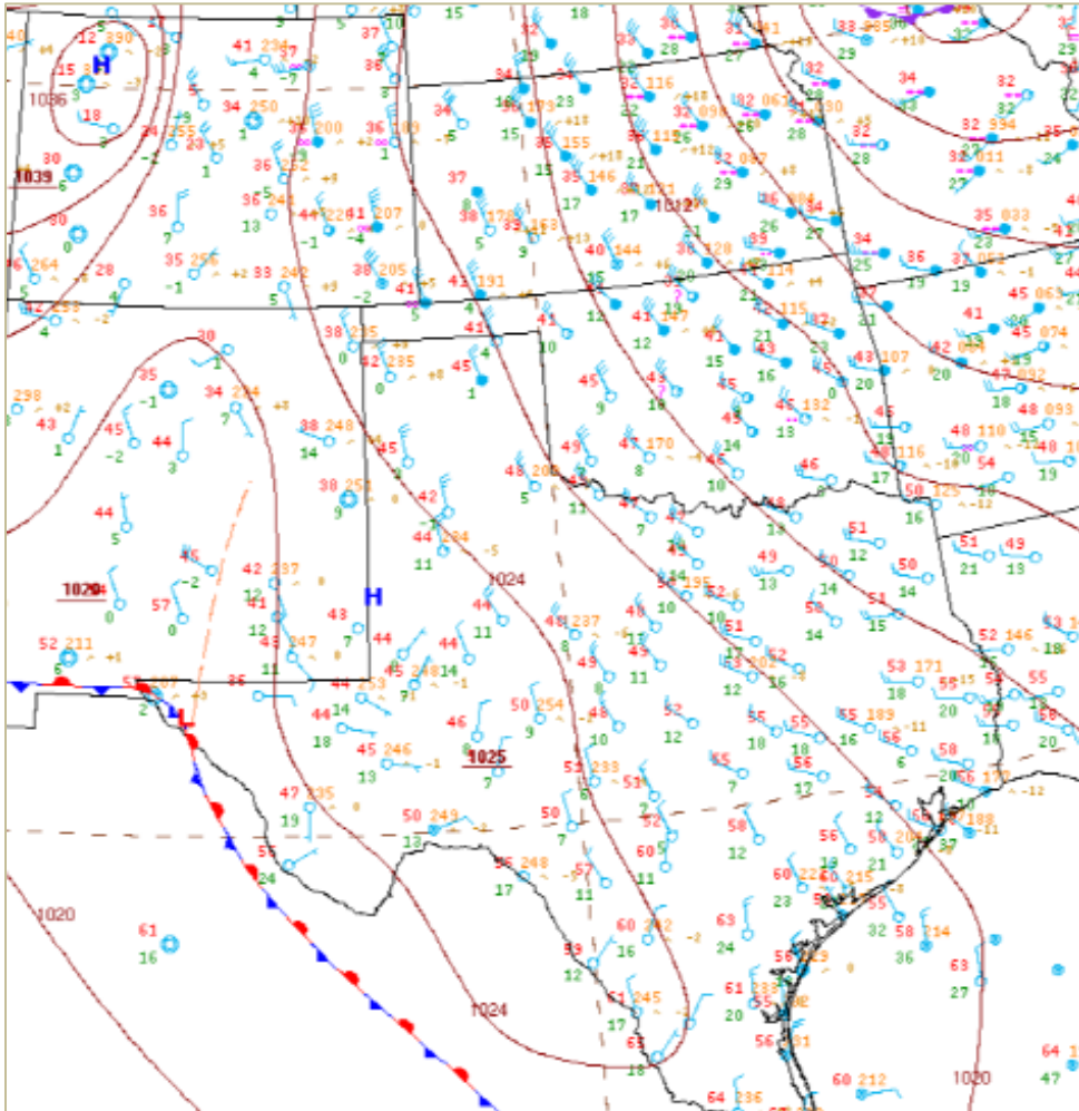
Figure B-1: Regional Weather Map for January 15, 2021
