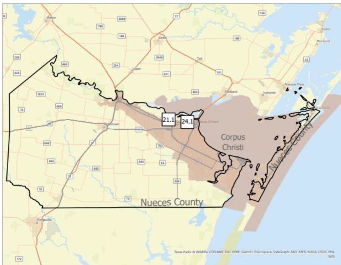
Figure B-9: Daily Average PM 2.5 Measurements (µg/m³) in Nueces County on January 21, 2021
