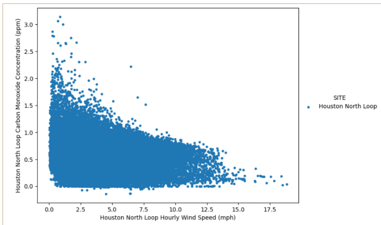
Figure 2-15: Houston North Loop (C1052) Hourly Average Carbon Monoxide Concentrations versus Houston North Loop (C1052) Hourly Wind Speeds for 2020 and 2021
