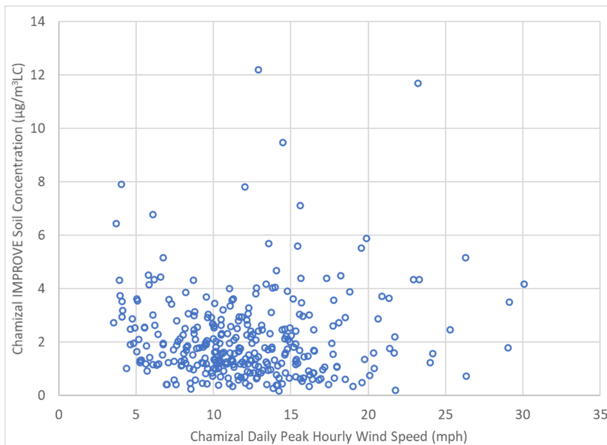
Figure C-10: El Paso Chamizal (C41) PM 2.5 IMPROVE Soil Concentration versus El Paso Chamizal (C41) Daily Peak Hourly Wind Speed for 2019 through 2021
