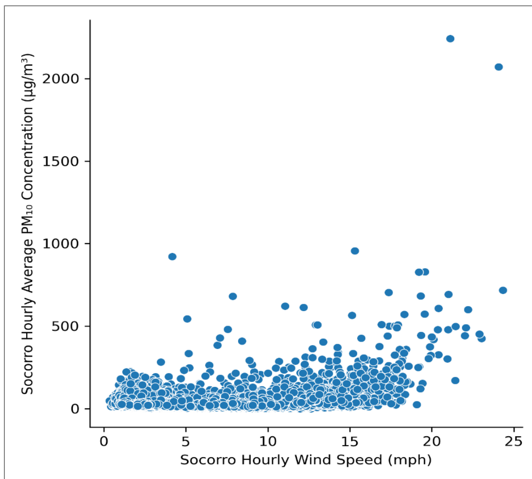
Figure 2-20: Socorro Hueco (C49) Hourly Average Continuous PM 10 Concentration versus Hourly Wind Speed for 2020 and 2021
