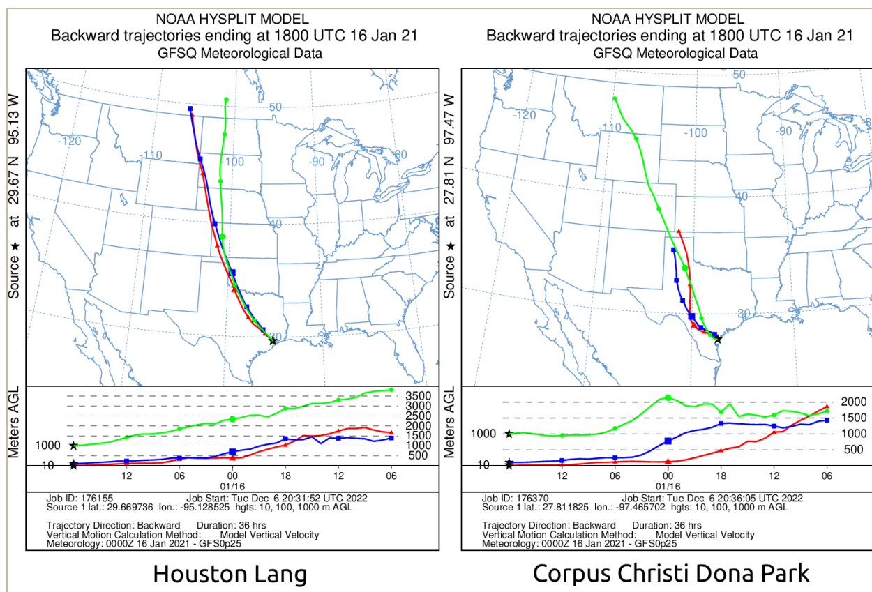
Figure B-1: HYSPLIT 36-Hour Backward Trajectories (1200 LST) at 10, 100, and 1,000 m AGL
