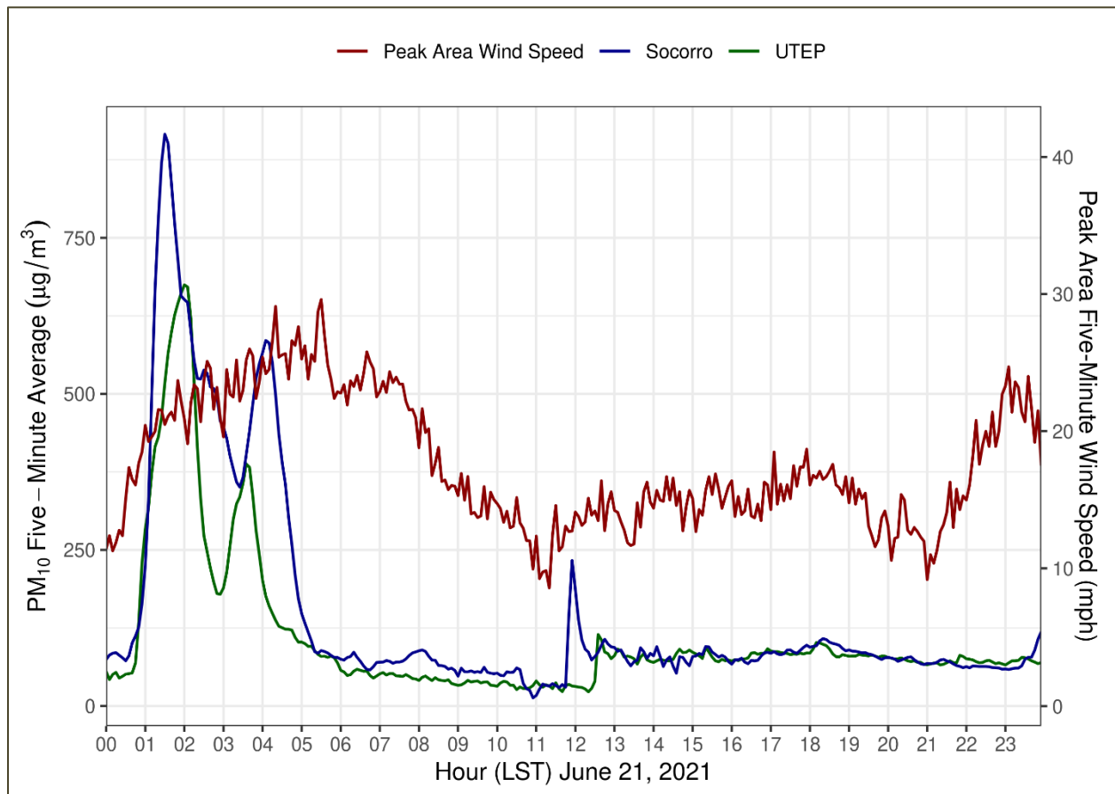
Figure C-6: Continuous Five-Minute PM 10 and Peak Area Five-Minute Sustained Wind Speed Measurements on June 21, 2021
