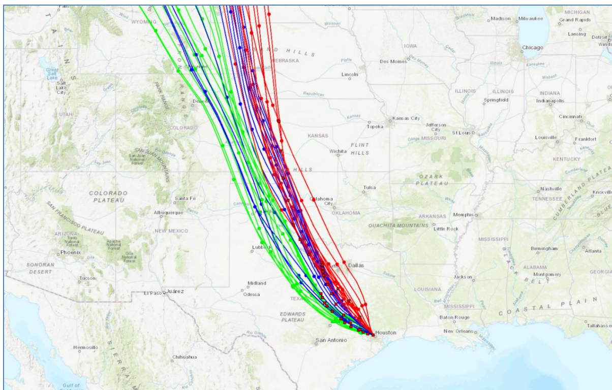
Figure B-4: HYSPLIT Backward Trajectories (Every 2 Hours on Jan. 16, 2021) at 10, 100, and 1000 m AGL at Houston Lang
