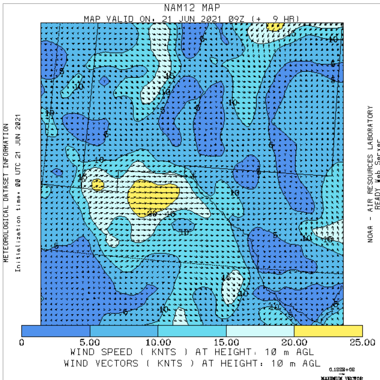
Figure C-11: NOAA ARL Model Wind Field in El Paso County at 03:00 MDT on June 21, 2021
