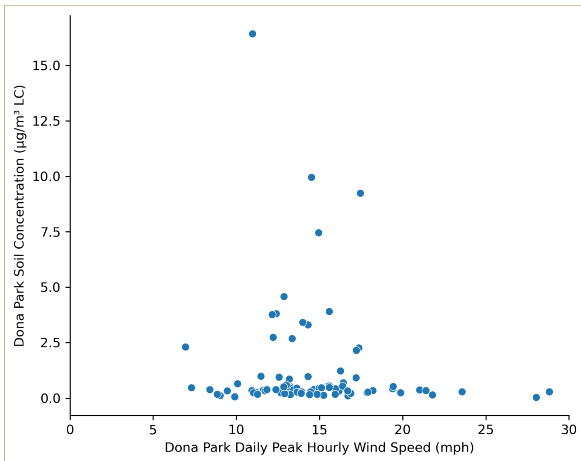
Figure B-18: Dona Park (C199) PM 2.5 IMPROVE Soil Concentration versus Dona Park (C199) Daily Peak Hourly Wind Speed for 2019 through 2021
