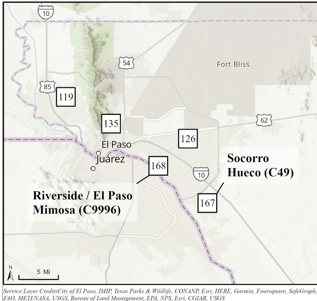
Figure C-4: Daily Average PM_{10} Measurements ( \mu g/m^3 ) on June 21, 2021
