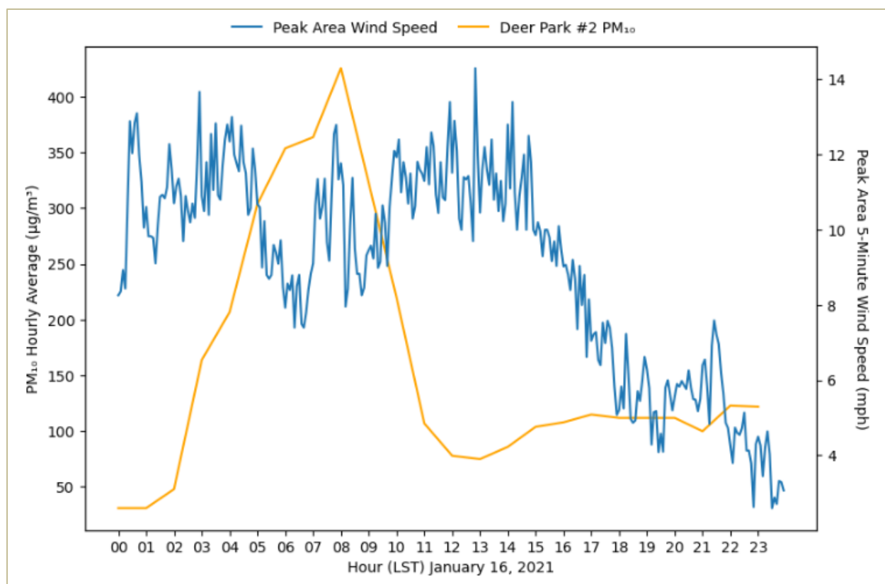
Figure B-10: Harris County Continuous Five-Minute PM_{10} and Peak Area Five-Minute Sustained Wind Speed Measurements on January 16, 2021
