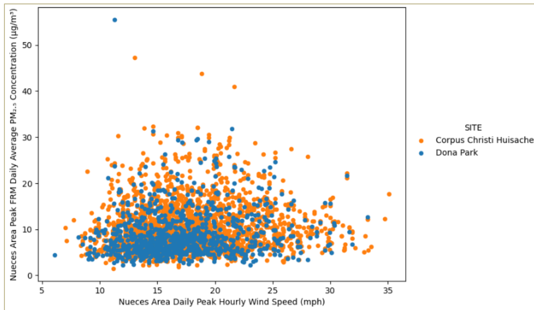
Figure 2-17: Nueces County Daily Peak PM 2.5 Average for FRM Measurements versus Nueces County Daily Peak Sustained Hourly Wind Speed for 2006 through 2021
