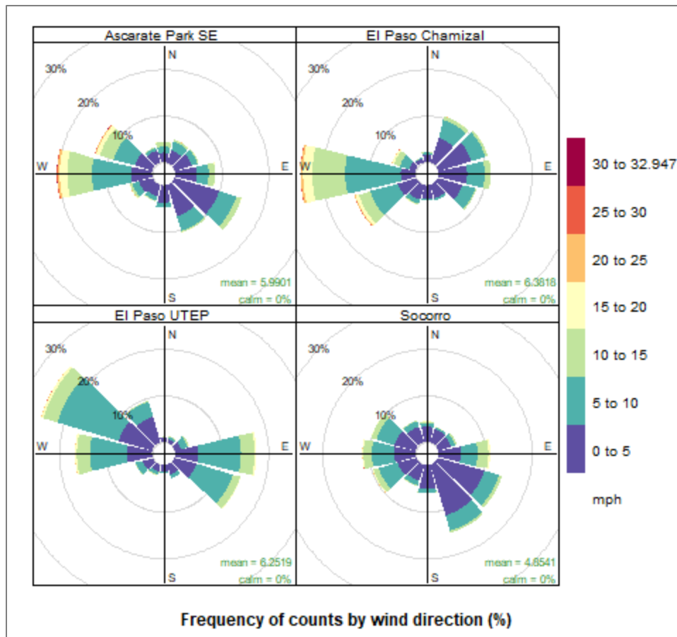
Figure 3-5: Wind Rose Plots for the El Paso UTEP (C12), Ascarate Park SE (C37), El Paso Chamizal (C41), and Socorro Hueco (C49) Monitors for 2019 through 2021
