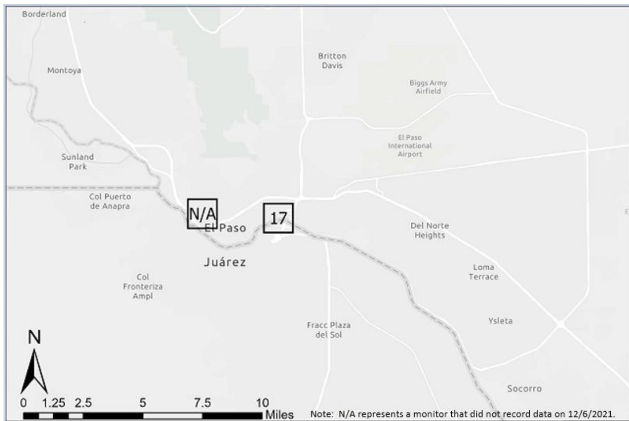
Figure D-3: Daily Average PM 2.5 Measurements (µg/m 3 ) on December 6, 2021
