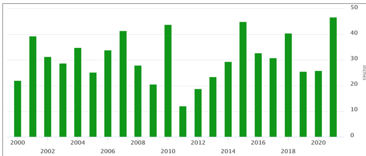
Figure 2-2: Annual Precipitation Measured at Corpus Christi International Airport (CRP) from 2000 through 2021
