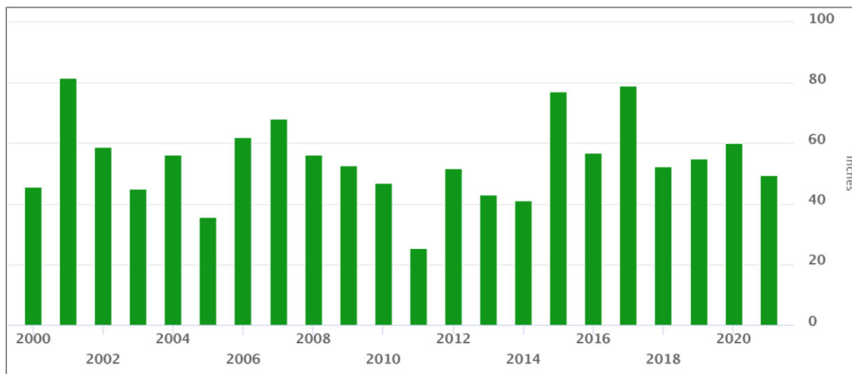
Figure 2-1: Annual Precipitation Measured at William P. Hobby Airport (HOU) from 2000 through 2021
