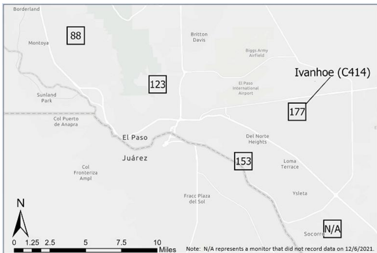
Figure D-2: Daily Average PM_{10} Measurements ( \mu g/m^3 ) on December 6, 2021
