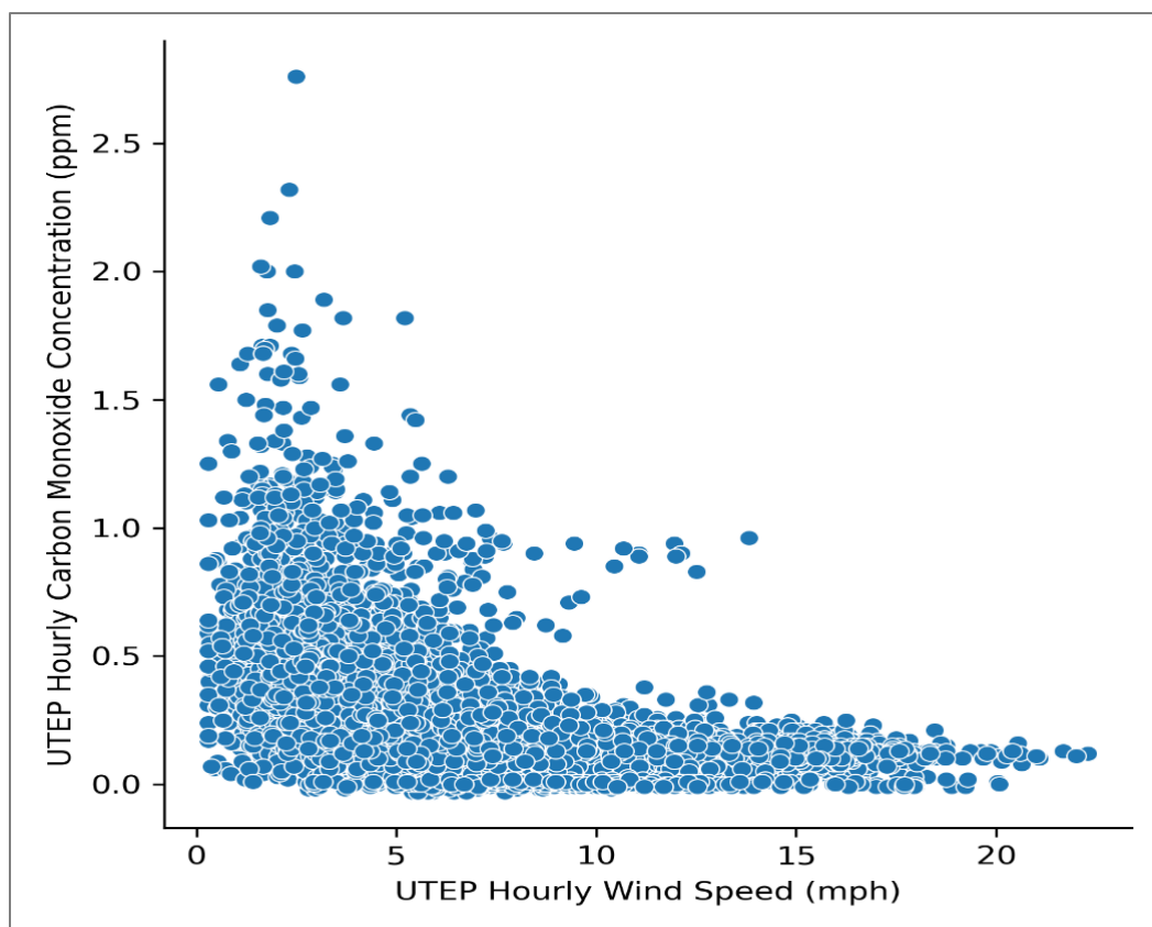
Figure 2-21: El Paso UTEP (C12) Hourly Average Carbon Monoxide Concentrations versus El Paso UTEP (C12) Hourly Wind Speeds for 2020 and 2021
