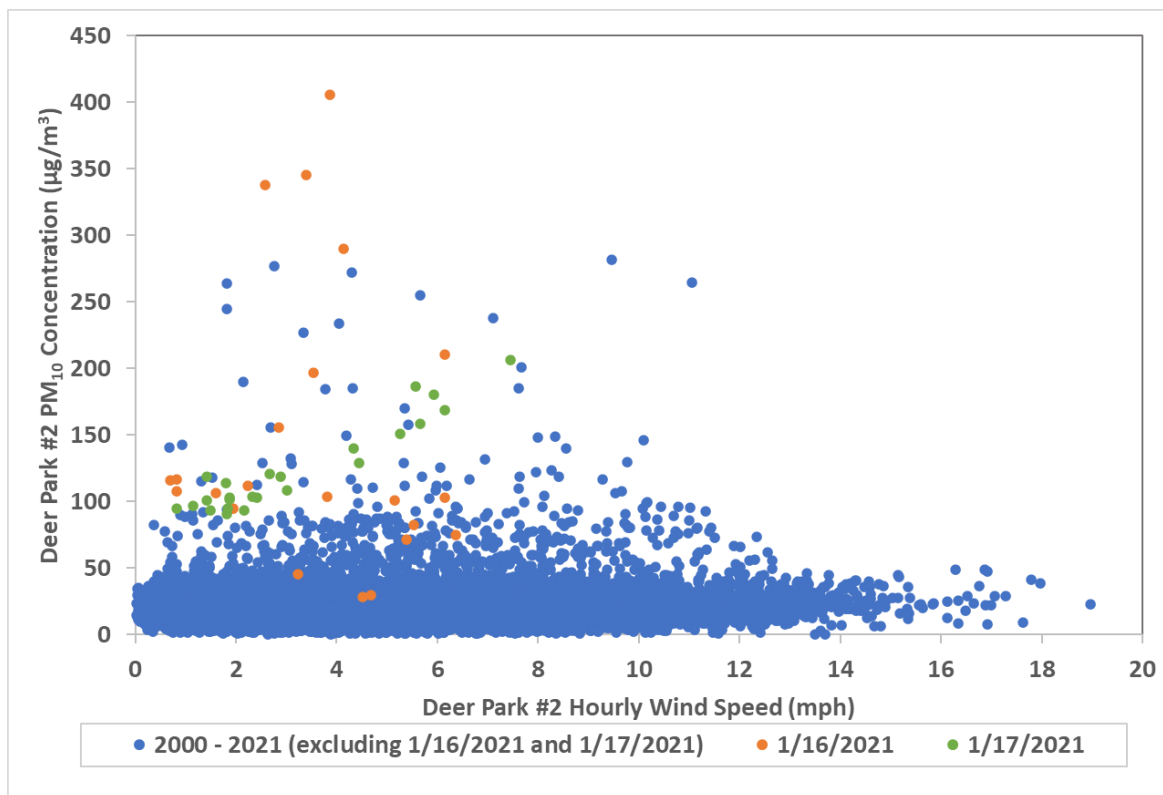
Figure 2-14: Deer Park #2 (C35) Hourly Average Continuous PM 10 Concentration versus Hourly Wind Speed for 2020 and 2021
