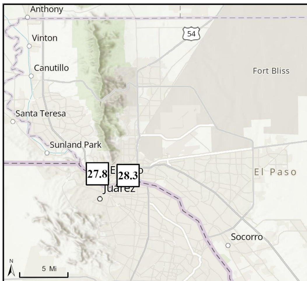
Figure C-5: Daily Average PM 2.5 Measurements (µg/m 3 ) on June 21, 2021
