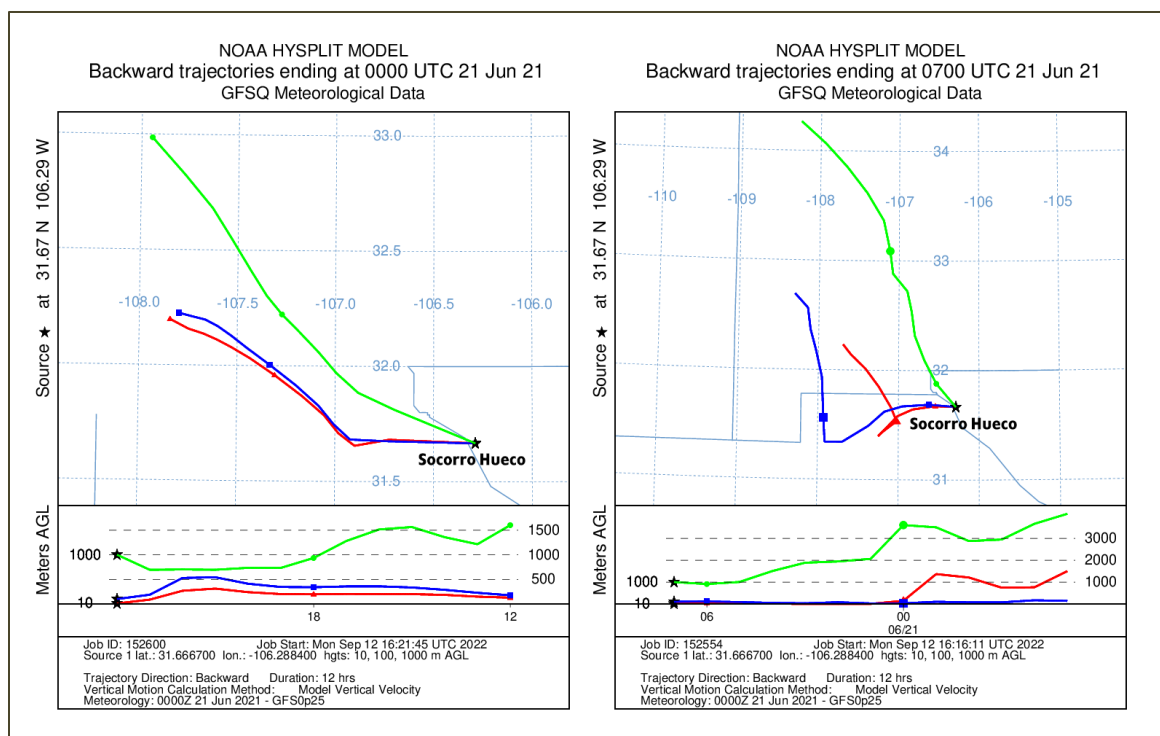
Figure C-0: HYSPLIT Backward Trajectories (June 20, 2021 at 18:00 MDT and June 21 at 0100 MDT) at 10, 100, and 1,000 m AGL
