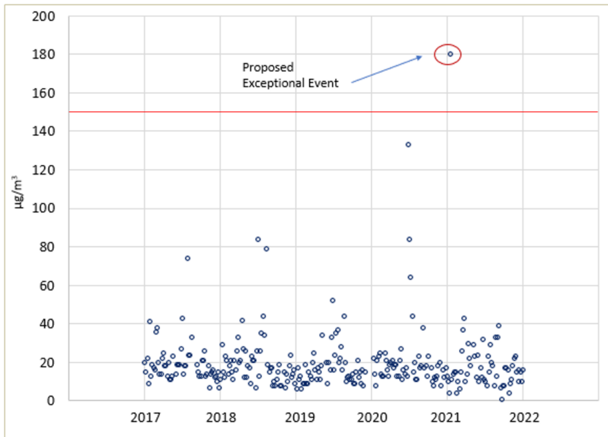
Figure 5-2: Dona Park (C199) FRM PM 10 Daily Measurements from 2017 through 2021
