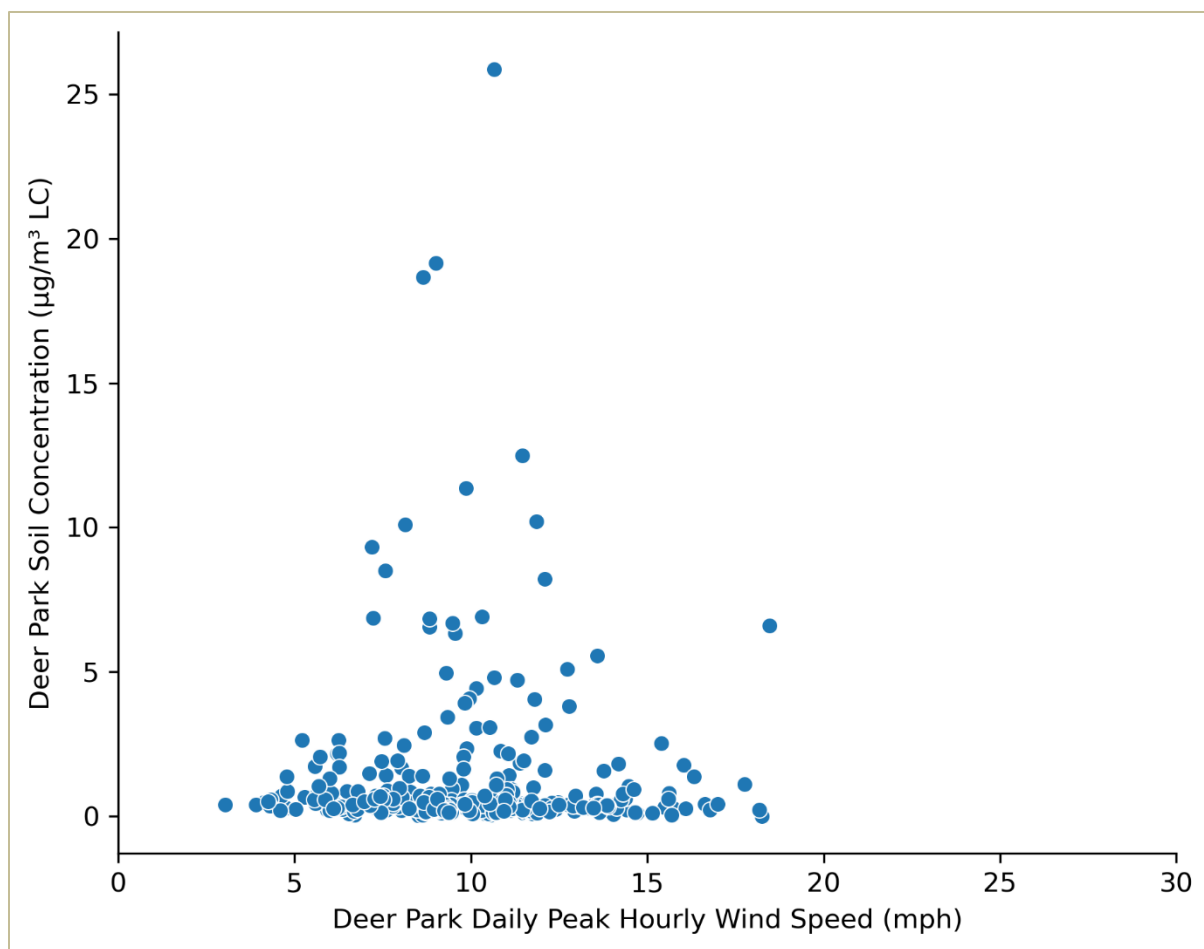
Figure B-17: Houston Deer Park #2 (C12) PM 2.5 IMPROVE Soil Concentration versus Houston Deer Park #2 (C12) Daily Peak Hourly Wind Speed for 2019 through 2021
