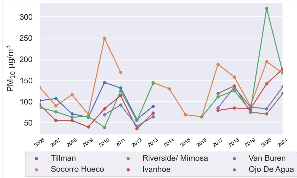
Figure 2-10: El Paso County PM 10 Annual Maximum 24-hour Averages for FRM Monitoring Sites, Including Exceptional Event Days
