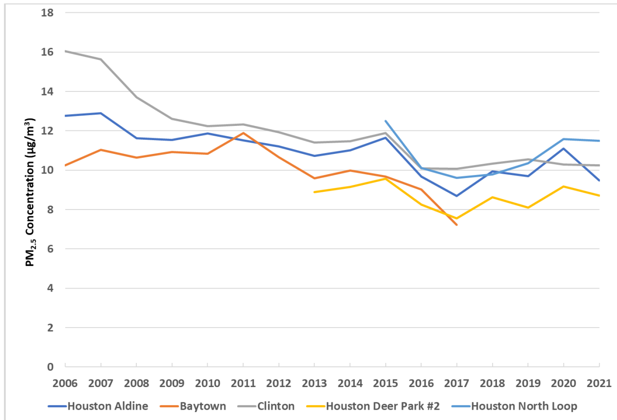
Figure 2-5: Harris County PM 2.5 Annual 24-hour Averages for Long-Term FRM Monitoring Sites, Including Exceptional Event Days
