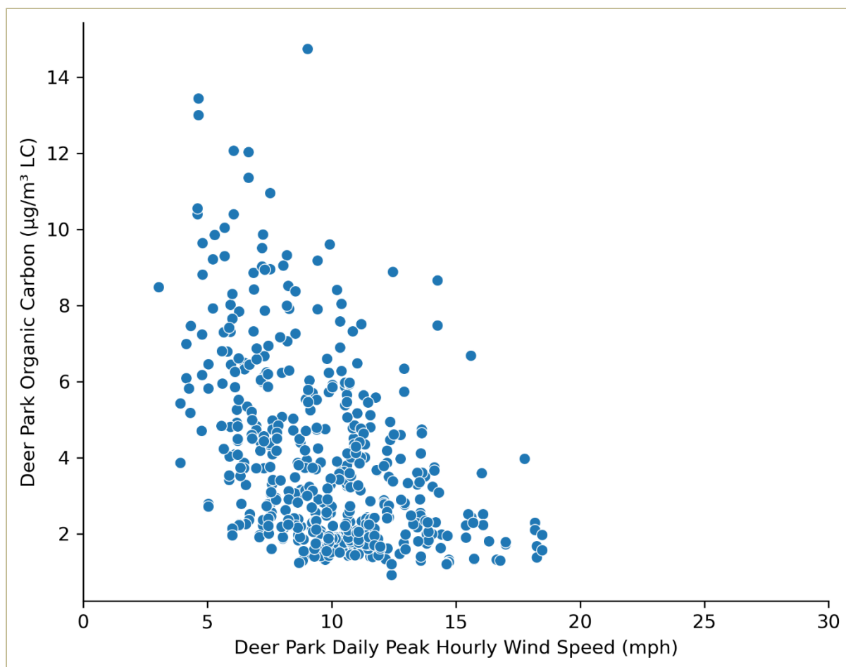
Figure B-15: Houston Deer Park #2 (C12) PM 2.5 IMPROVE Organic Carbon Concentration versus Houston Deer Park #2 (C12) Daily Peak Hourly Wind Speed for 2019 through 2021
