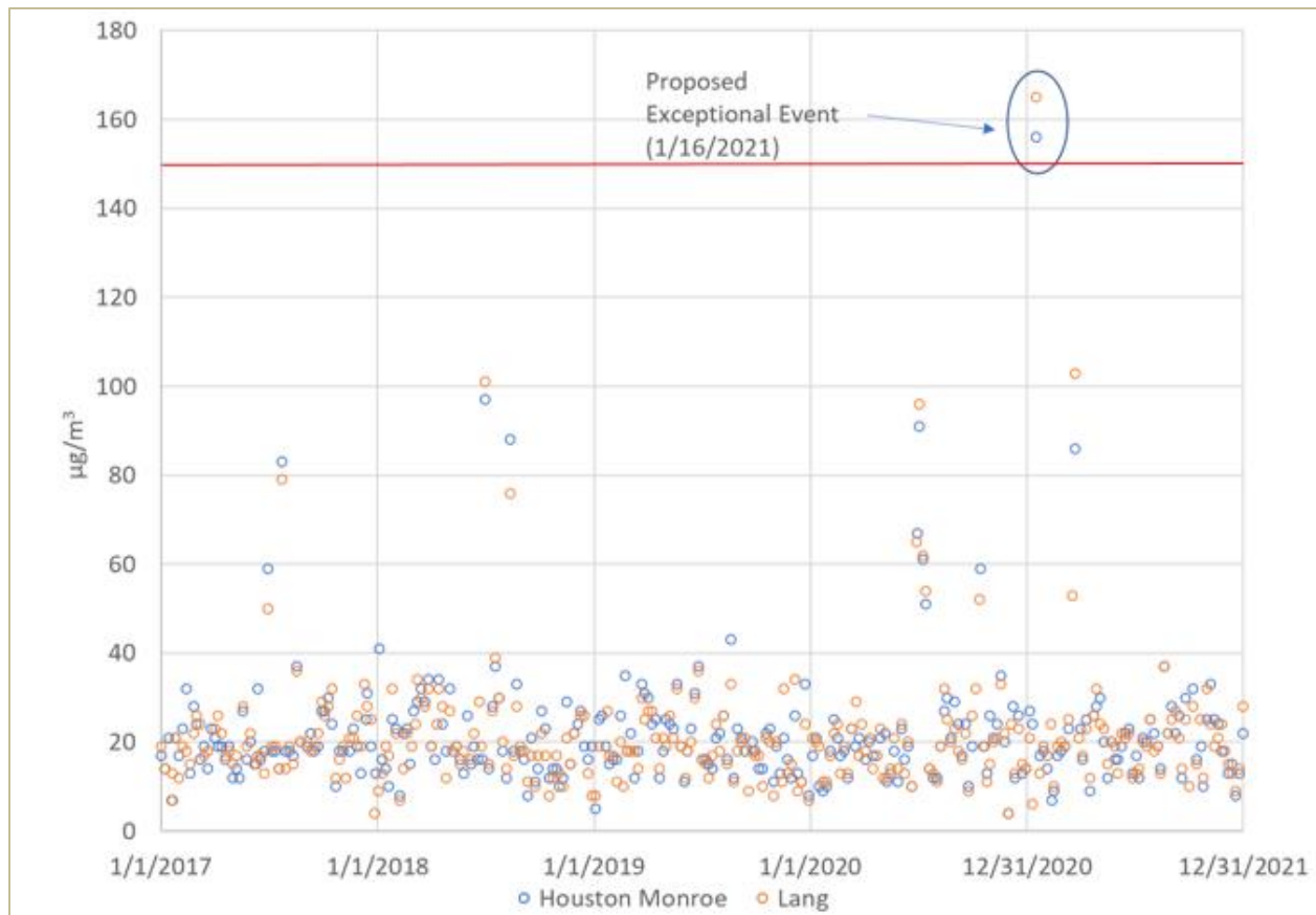
Figure 5-1: Houston Monroe (C406) and Lang (C408) FRM PM 10 Daily Measurements from 2017 through 2021
