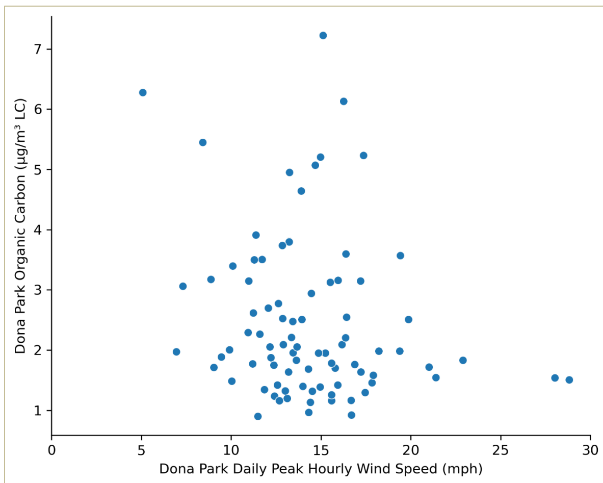
Figure B-16: Dona Park (C199) PM 2.5 IMPROVE Organic Carbon Concentration versus Dona Park (C199) Daily Peak Hourly Wind Speed for 2019 through 2021
