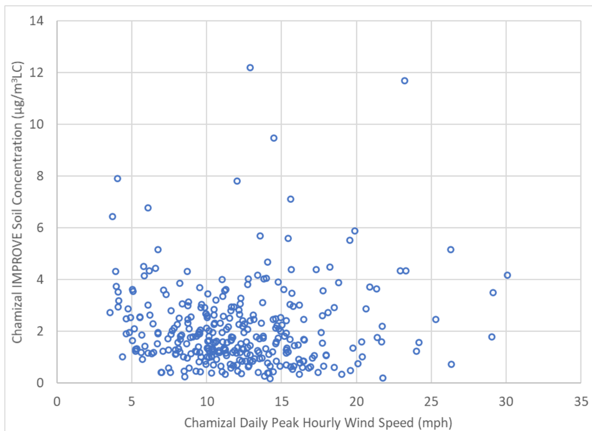
Figure: D-6:El Paso Chamizal (C41) PM 2.5 IMPROVE Soil Concentration versus El Paso Chamizal (C41) Daily Peak Hourly Wind Speed for 2019 through 2021
