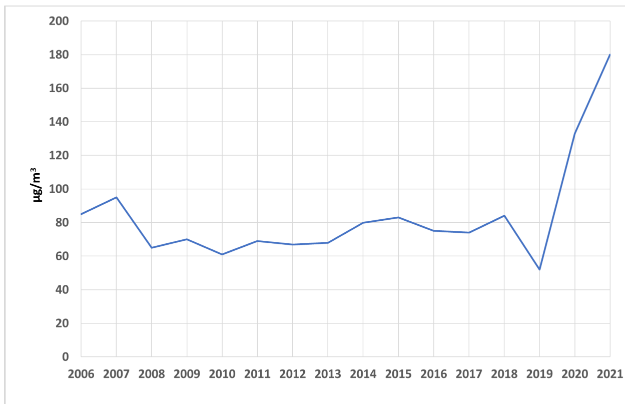
Figure 2-7: Nueces County PM 10 Annual Maximum 24-hour Averages for FRM Monitoring Sites, Including Exceptional Event Days
