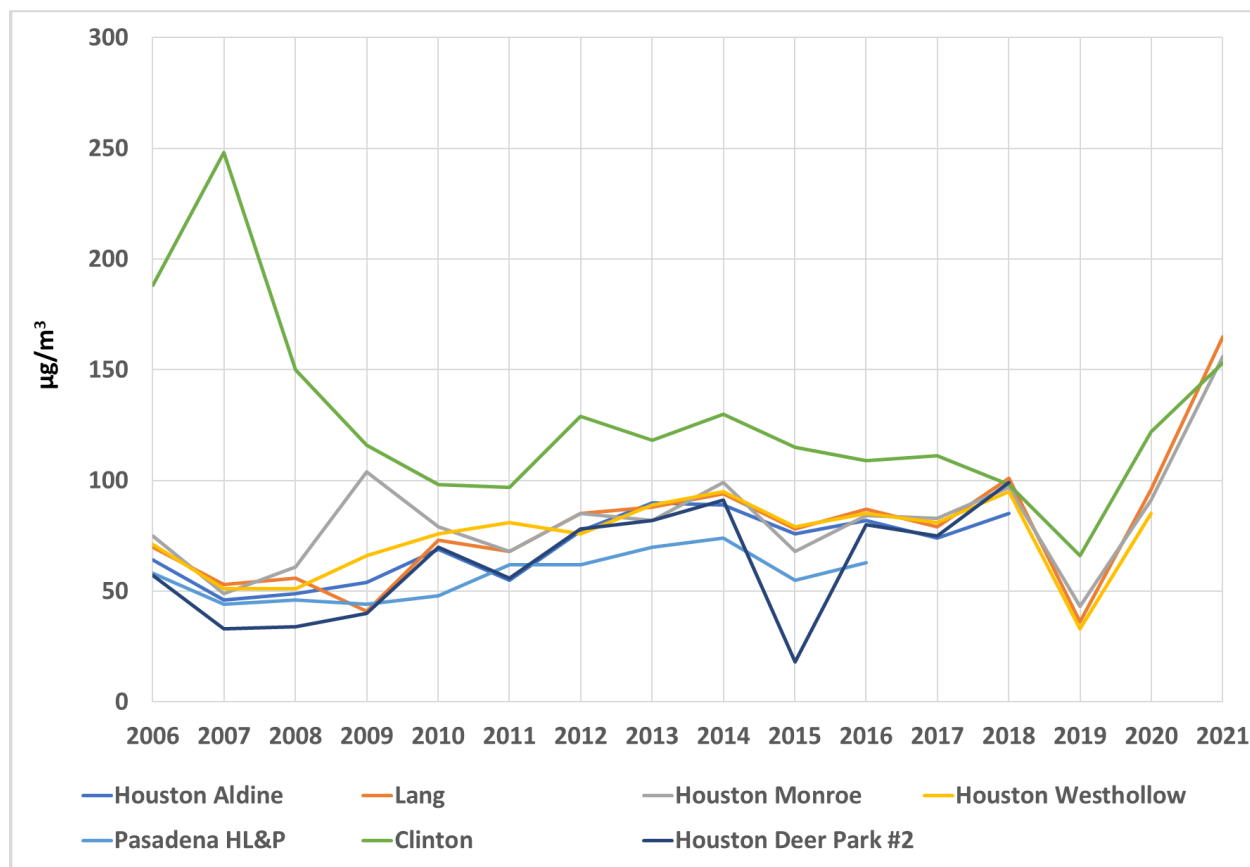
Figure 2-4: Harris County PM 10 Annual Maximum 24-hour Averages for FRM Monitoring Sites, Including Exceptional Event Days
