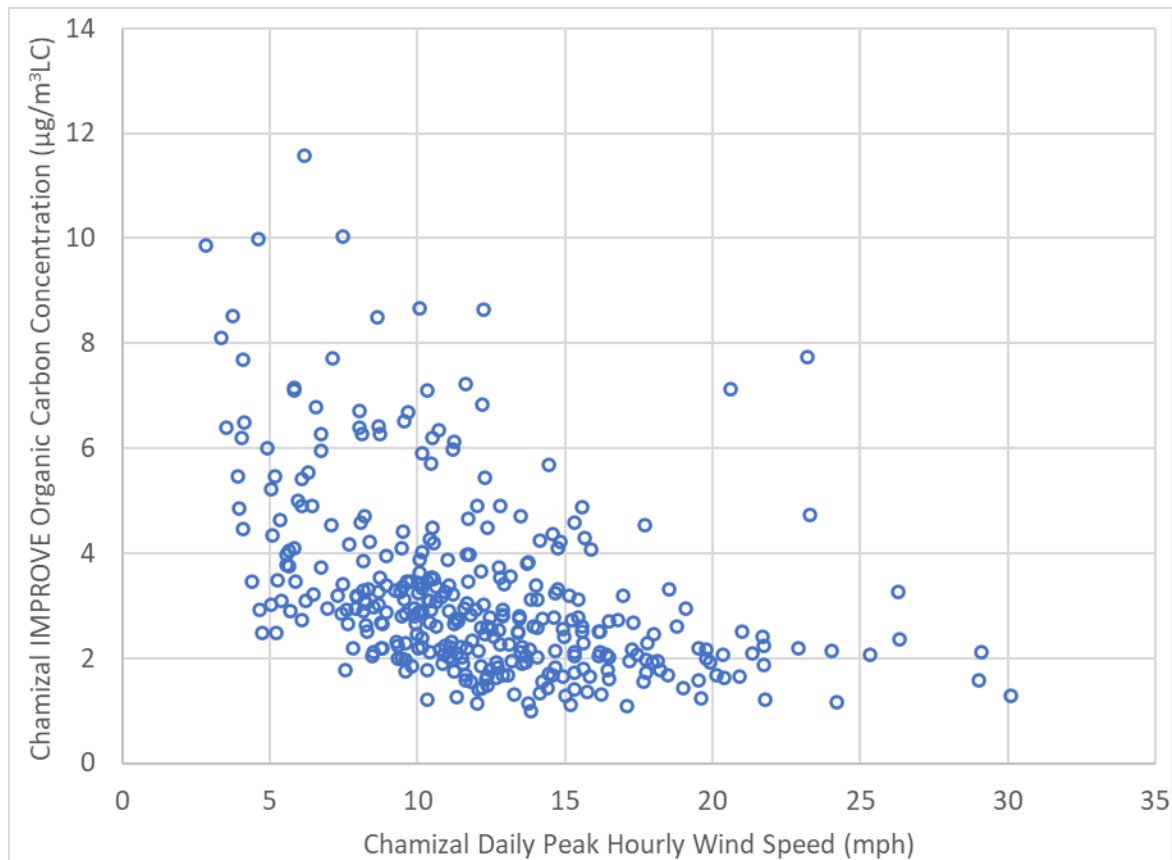
Figure D-5: El Paso Chamizal (C41) PM 2.5 IMPROVE Organic Carbon Concentration versus El Paso Chamizal (C41) Daily Peak Hourly Wind Speed for 2019 through 2021
