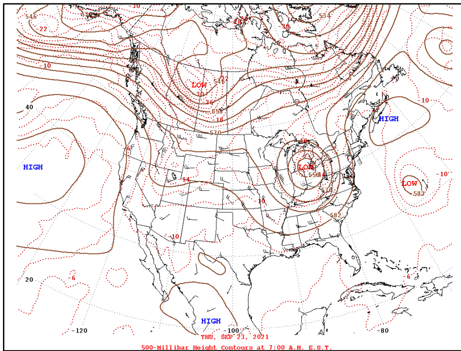
Figure 3-114: 500-mb Weather Chart for September 23, 2021
