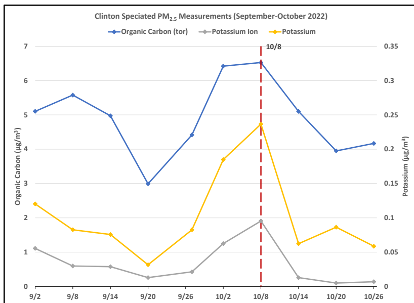
Figure 3-86: Speciated \text{PM}_{2.5} Measurements at the Clinton Monitoring Site
