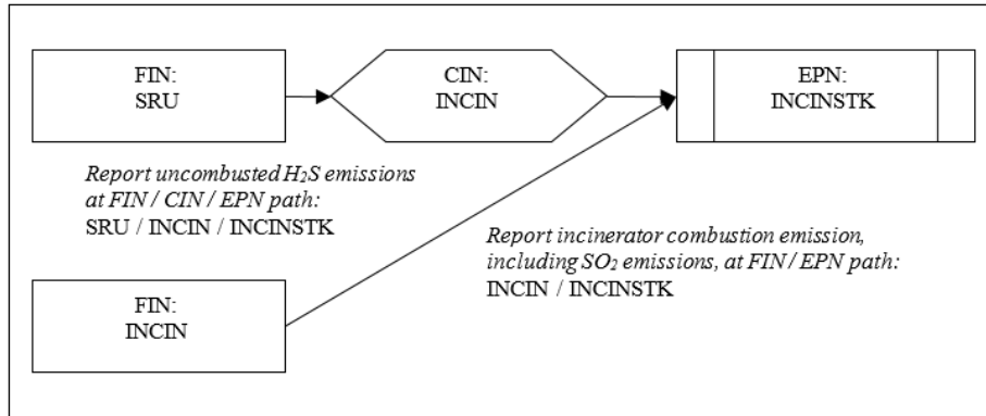
Figure 3-7. Sulfur Recovery Unit with Incinerator
