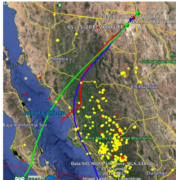
Figure 3. The profile of the sounding on 15 May 2017 ( Figure 2 ) has an ozone enhancement in the LFT with a peak at 5500 m AMSL. The enhancement may have resulted from the long-range transport of biomass burning emissions. Left: HYSPLIT back trajectories at 3000 m (red), 4250 m (blue), and 5500 m (green) AMSL overlaid on recent MODIS hot spots (red and yellow dots).
