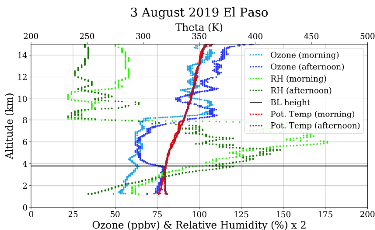
Figure 4. For El Paso, the first day during the 2019 sampling period with an MDA8 ozone concentration in exceedance of the NAAQS ozone standard was 3 August. The image shows dawn (light blue and light green) and afternoon (dark blue and dark green) ozone and relative humidity profiles. The twice-daily profiles allow for estimates of the contribution of the residual layer from the previous night to the subsequent afternoon boundary layer ozone concentrations.
