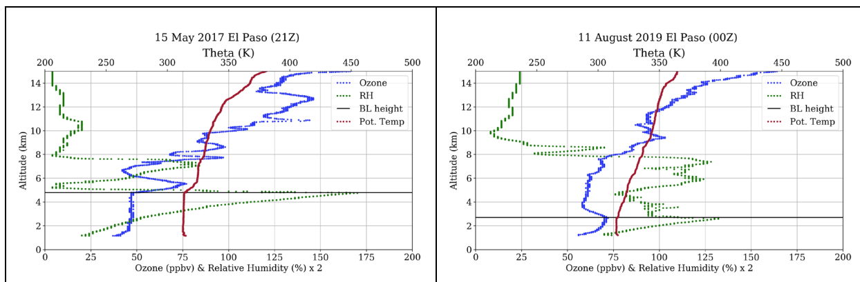
Figure 2. Left: Just above the boundary layer there is a positive gradient in the ozone concentration (it increases), which is a sign of long-range transport. Right: Just above the boundary layer there is a negative gradient in the ozone concentration (it decreases), which is more common, meaning long-range transport is less likely and that the ozone in the boundary layer is more likely the result of local photochemical production, local transport, and contributions from the nocturnal boundary layer of the previous night.
