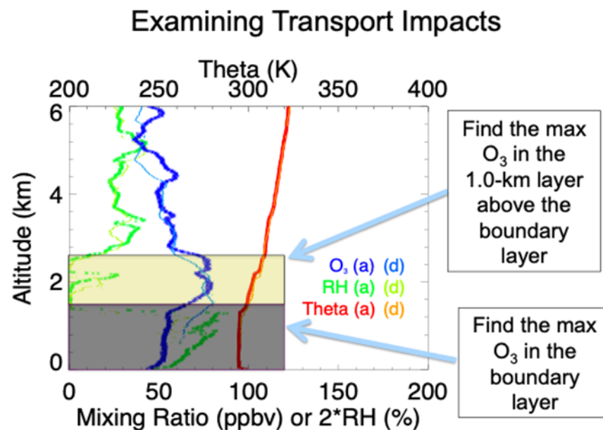
Figure 1. The figure shows an example profile used to determine O 3 in the lower free troposphere (LFT) and the mixed layer (ML). ML height determinations are made using O 3 , RH, temperature (not shown), and potential temperature ( \theta ) data. See text for details. The thick lines are data of the ascent of the ozonesonde and the thin lines show the descent. Our focus will typically be on the ascending data.
