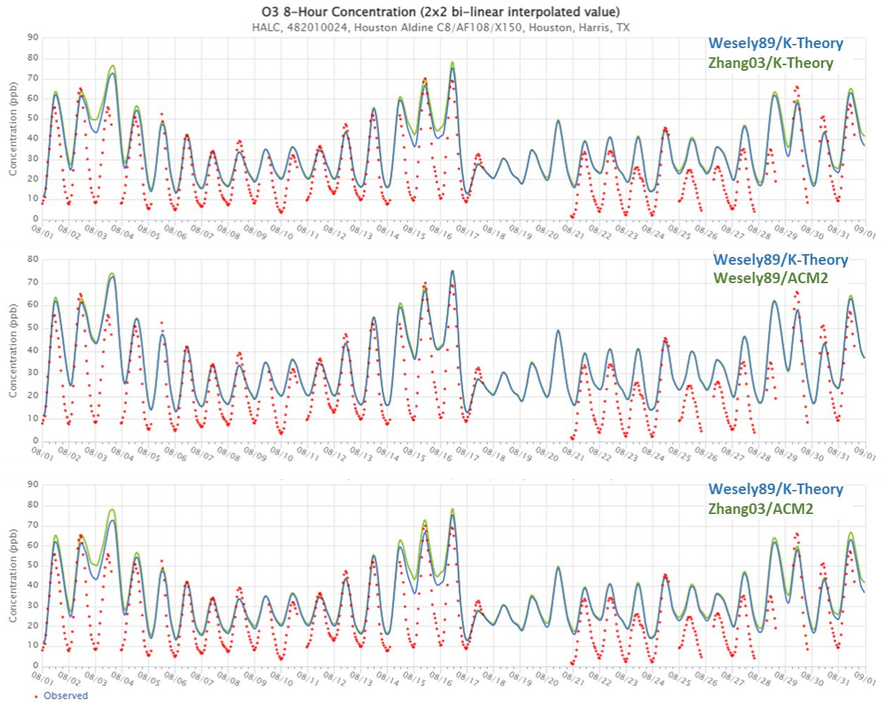
Figure 5-10: August Eight-Hour Average Ozone Comparing Wesely89/K-Theory to Zhang03/K-Theory (top), to Wesely89/ACM2 (middle), and to Zhang03/ACM2 (bottom) at the Houston Aldine Monitor
