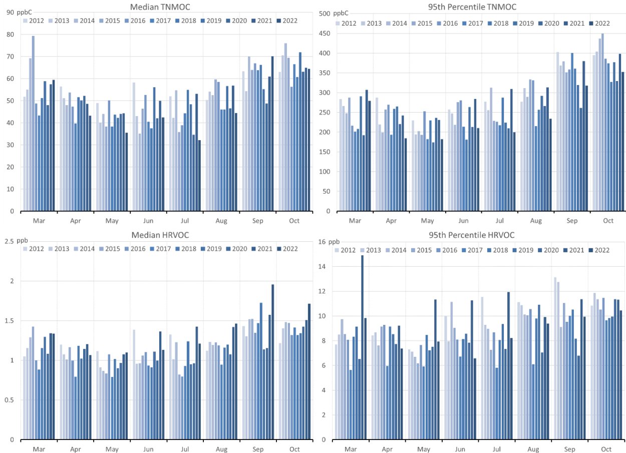
Figure 3-6: Monthly TNMOC (top) and HRVOC (bottom) Trends in the HGB Area
