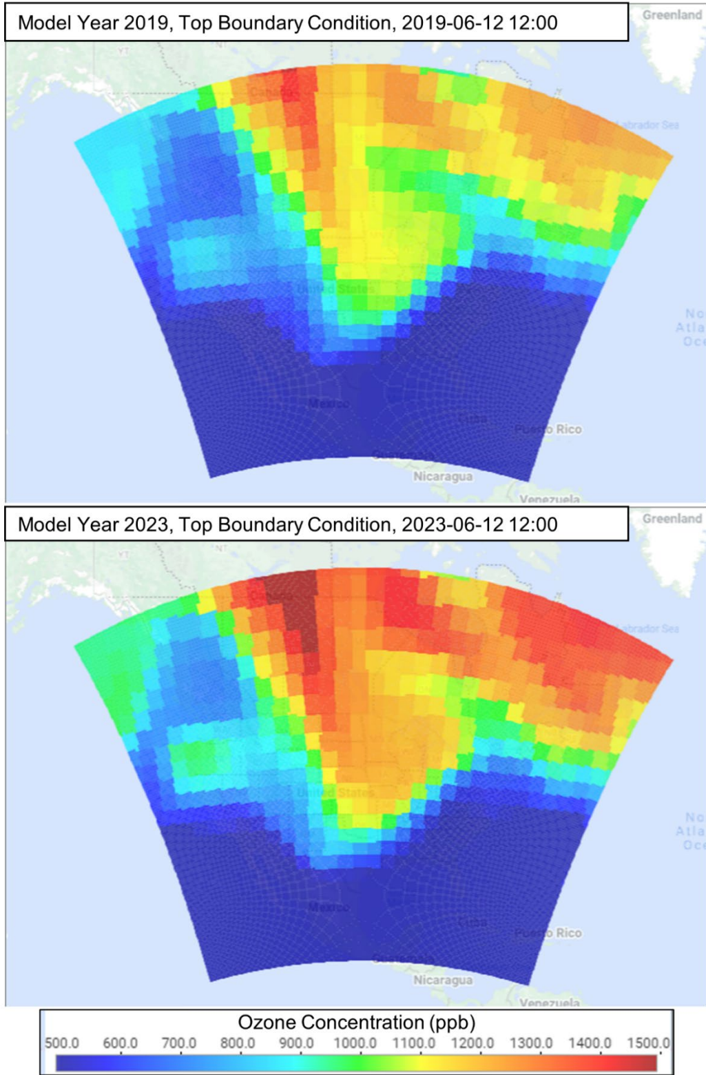
Figure 4-2: Top Boundary Condition for Ozone on June 12 in 2019 and 2023
