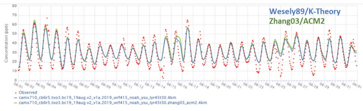
Figure 5-24: August Eight-Hour Ozone Comparing Wesely89/K-Theory to Zhang03/K-Theory (top), to Wesely89/ACM2 (middle), and to Zhang03/ACM2 (bottom) at the Camp Bullis Monitor
