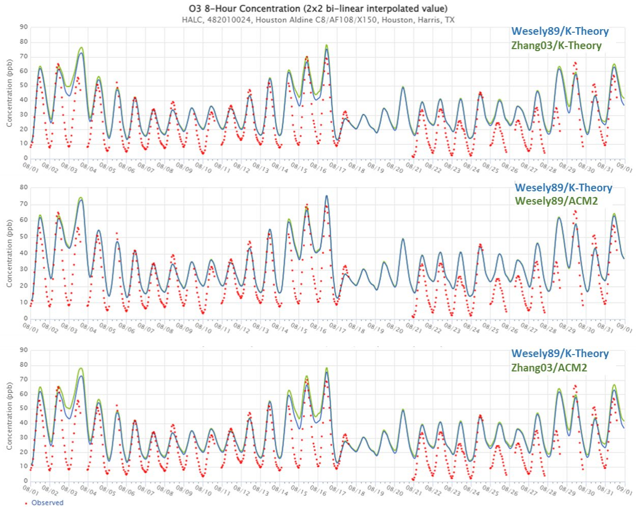
Figure 5-14: August Eight-Hour Average Ozone Comparing Wesely89/K-Theory to Zhang03/K-Theory (top), to Wesely89/ACM2 (middle), and to Zhang03/ACM2 (bottom) at the Houston Aldine Monitor
