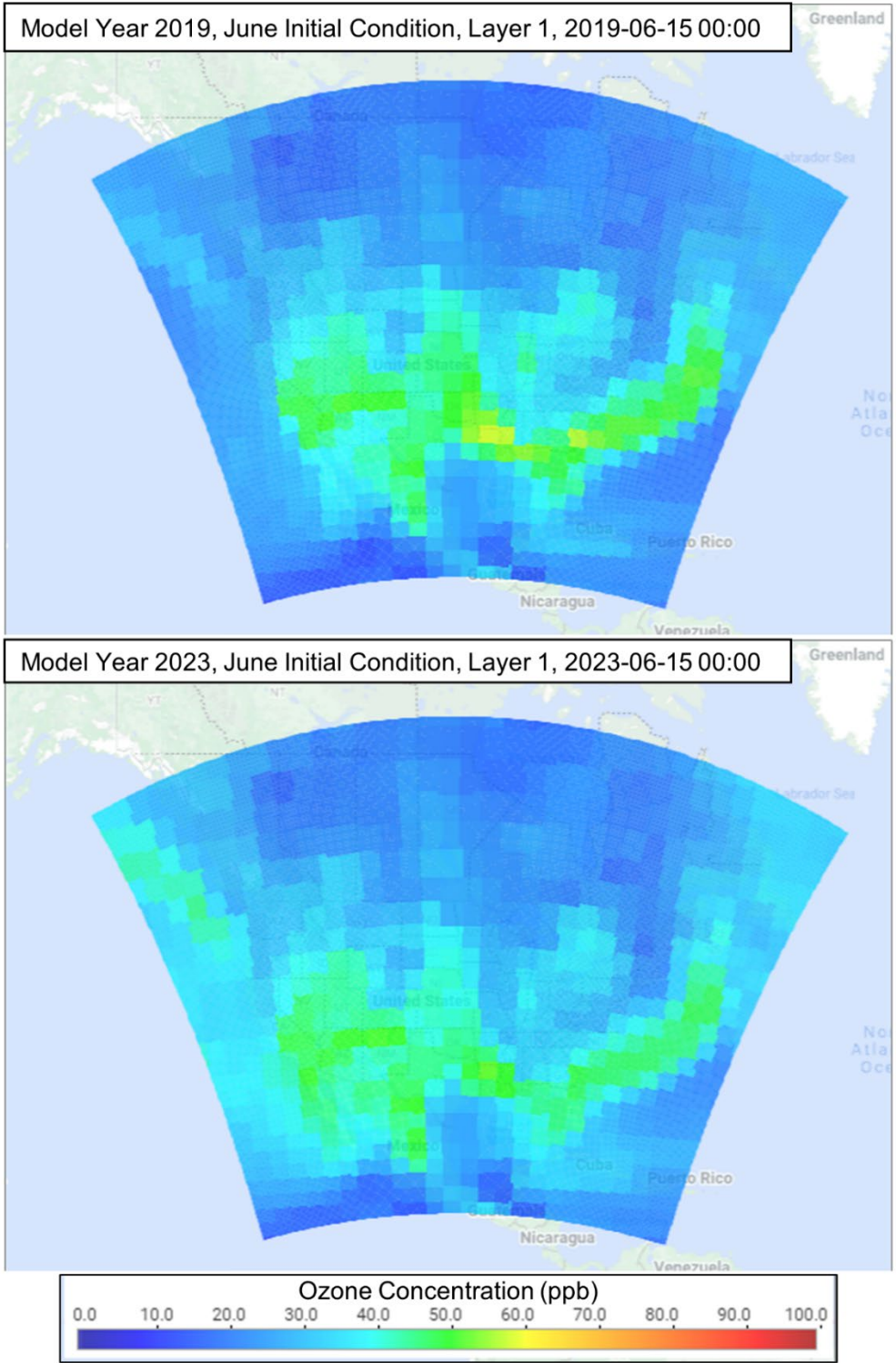
Figure 4-3: June Initial Condition for Ozone in 2019 and 2023
