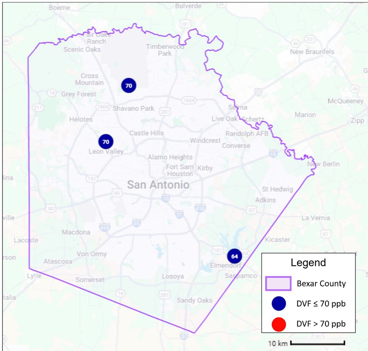
Figure 3-14: 2026 DVF in the Bexar County 2015 Ozone NAAQS Nonattainment Area
