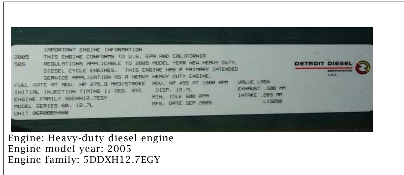
Figure 2 – Example of a Heavy-Duty Engine Emission Label
