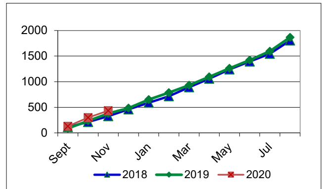
Figure 4: Assessed Penalties
