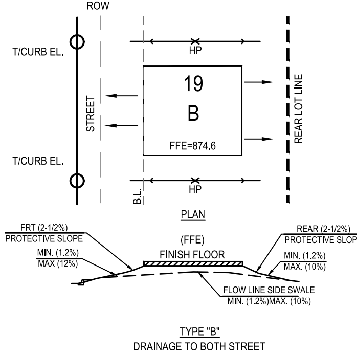
TYPE 'B' DRAINAGE TO BOTH STREET AND REAR LOT LINE
