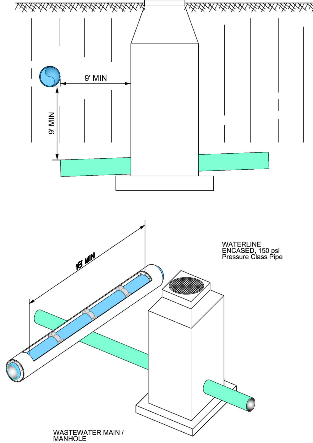
WATERLINE AND WASTEWATER MAIN OR LATERAL MANHOLE OR CLEANOUT SEPARATION CLEANOUT SEPARATION
