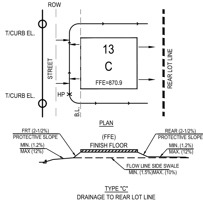
TYPE 'C' DRAINAGE TO REAR LOT LINE
