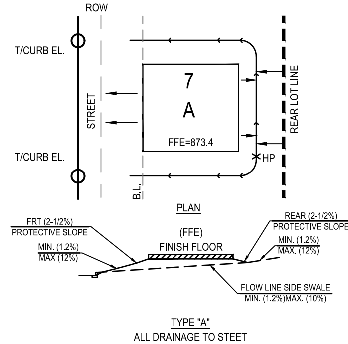
TYPE 'A' ALL DRAINAGE TO STREET
