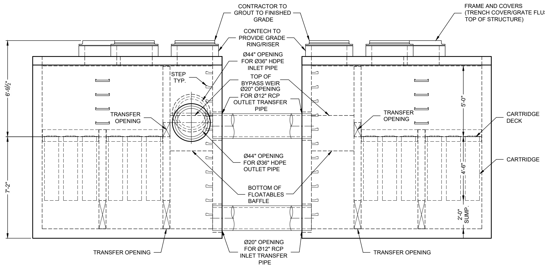
ELEVATION VIEW
