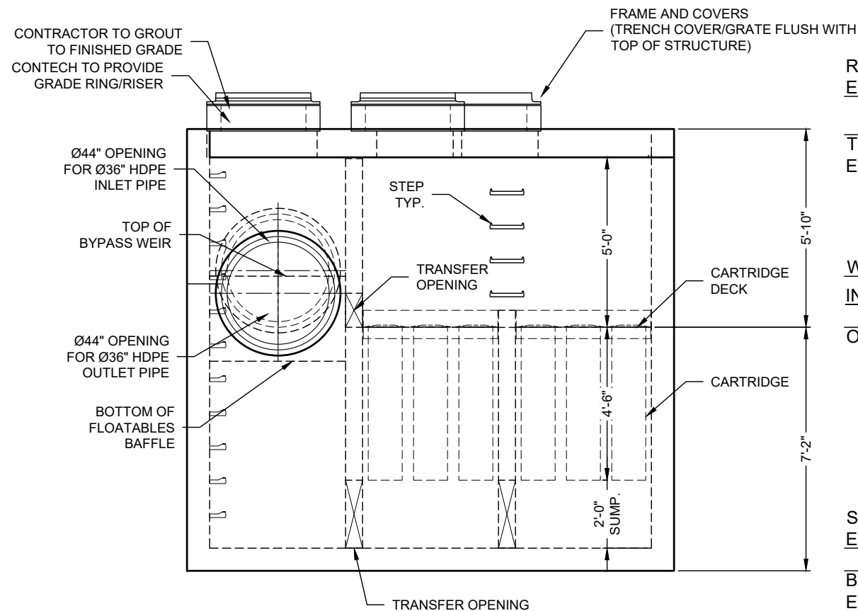
ELEVATION VIEW
