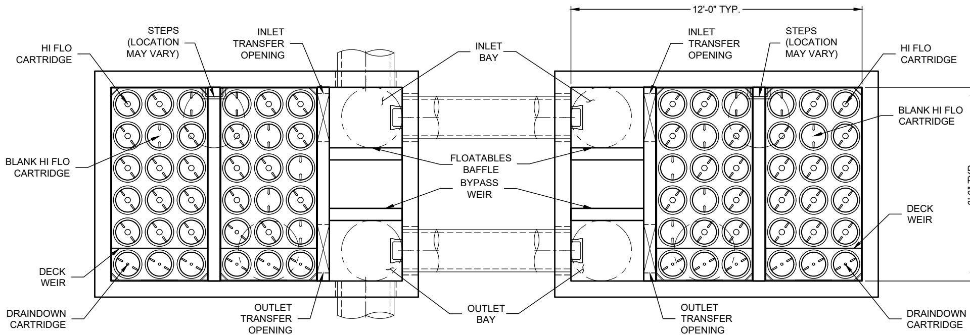
PLAN VIEW (TOP SLAB NOT SHOWN FOR CLARITY)
