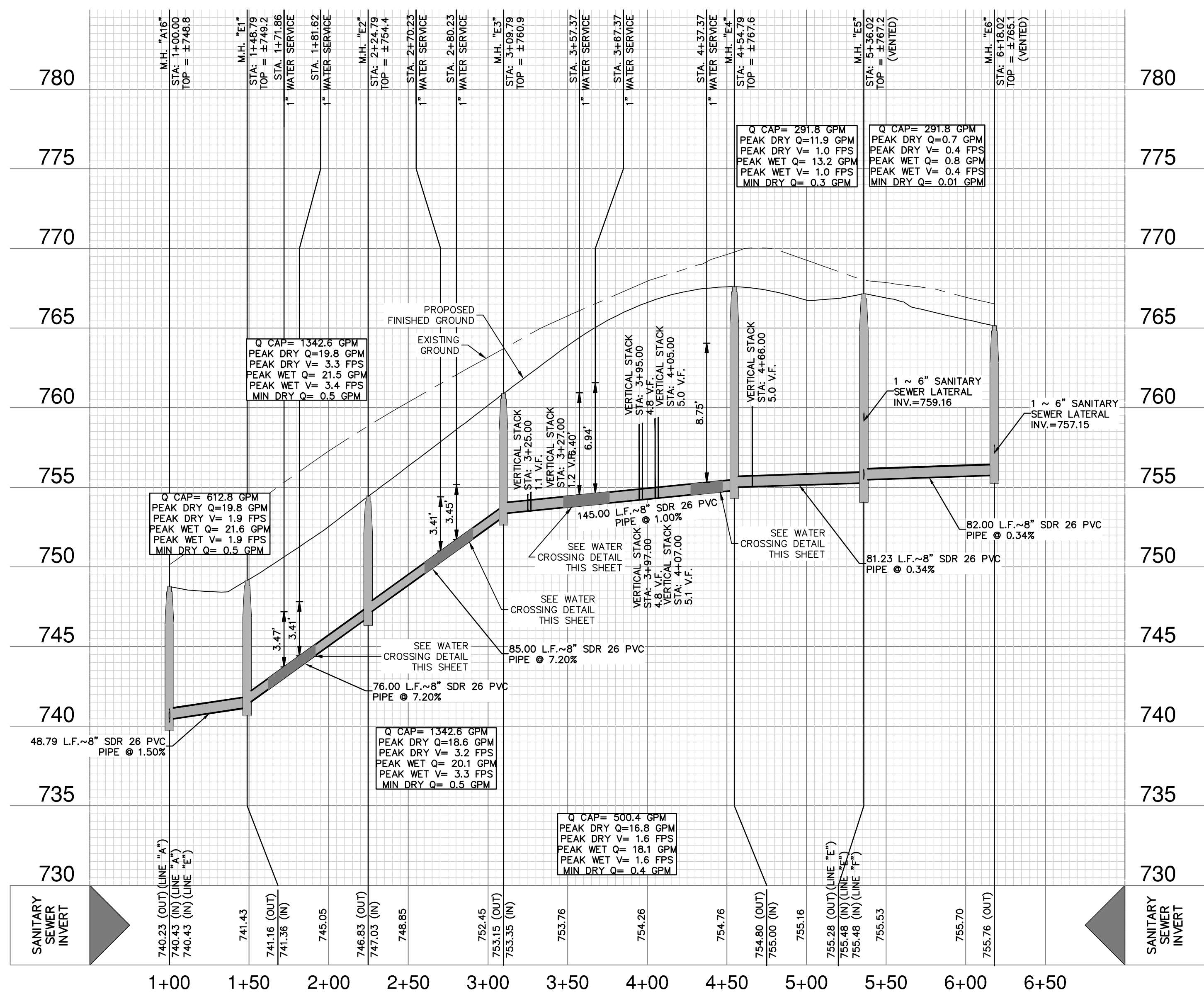
SANITARY SEWER LINE "E" STA 1+00.00 TO 6+18.02 VERTICAL SCALE: 1" = 5' HORIZONTAL SCALE: 1" = 50'
