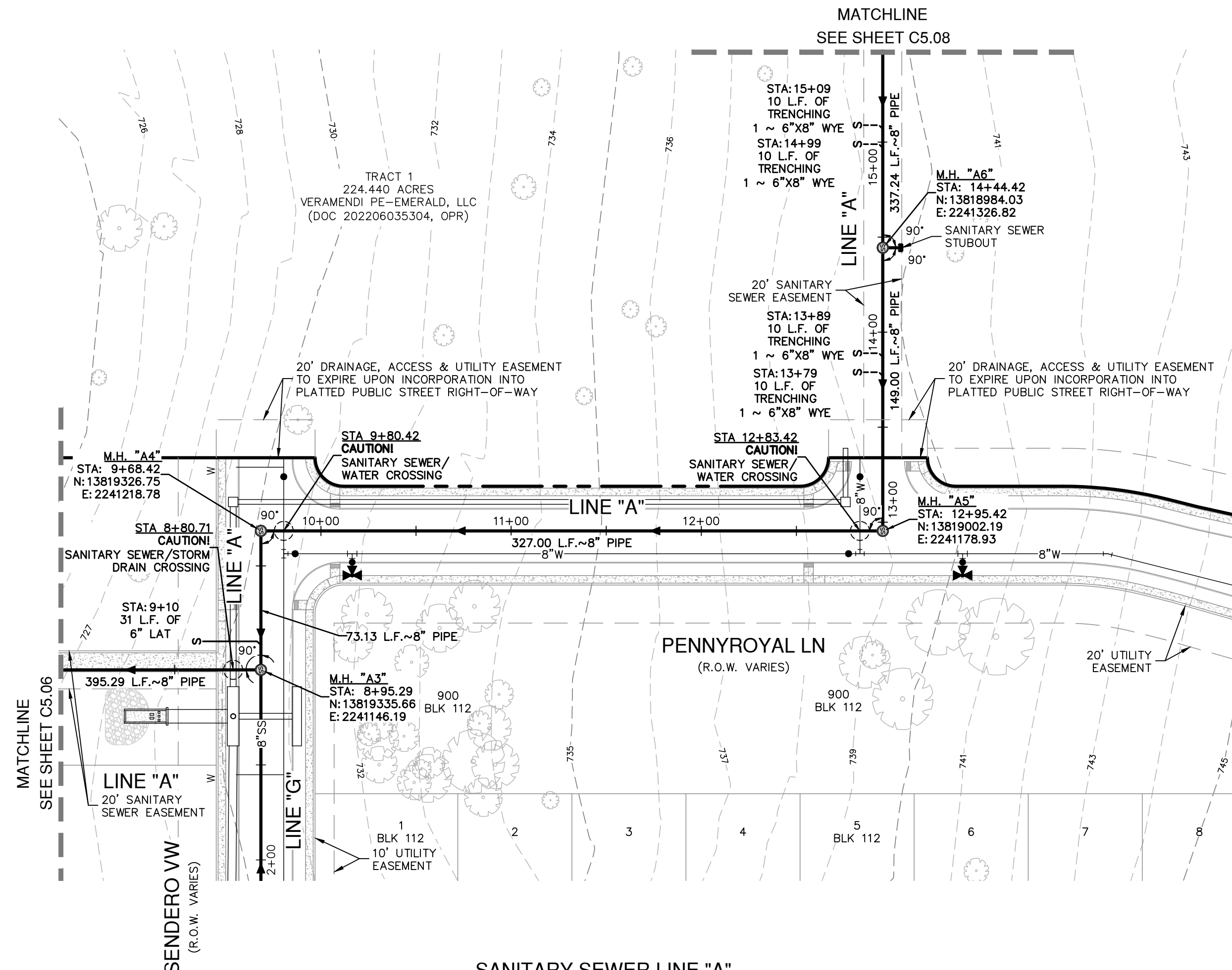
SANITARY SEWER LINE "A" STA 8+00.00 TO 16+00.00 VERTICAL SCALE: 1" = 5' HORIZONTAL SCALE: 1" = 50'
