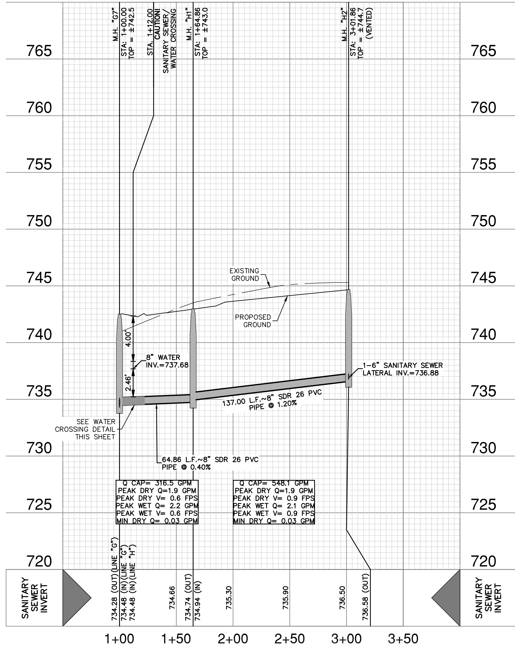
SANITARY SEWER LINE "H" STA. 1+00.00 TO 3+01.86 VERTICAL SCALE: 1" = 5' HORIZONTAL SCALE: 1" = 50'
