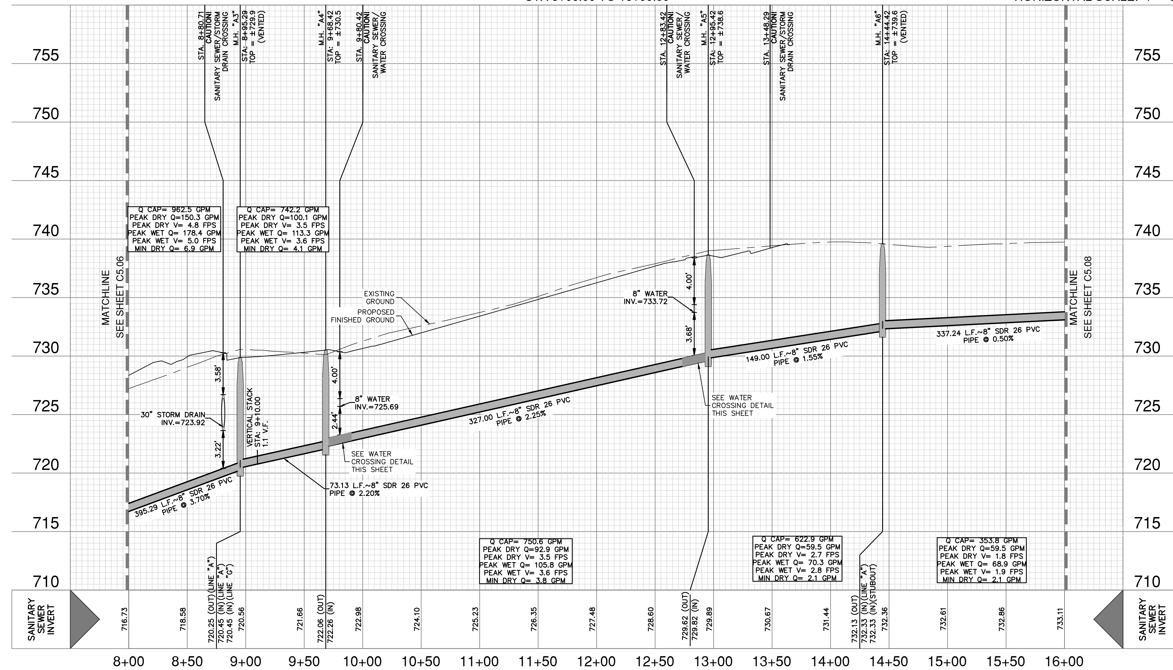
SANITARY SEWER LINE "A" STA 8+00.00 TO 16+00.00 VERTICAL SCALE: 1" = 5' HORIZONTAL SCALE: 1" = 50'
