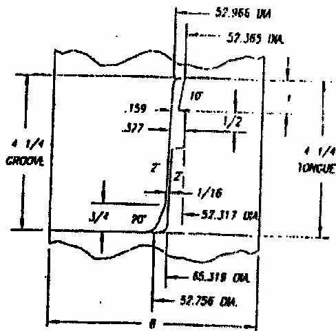
7 1/2" STEEL PIPE SCALE: 3/8"=1"
