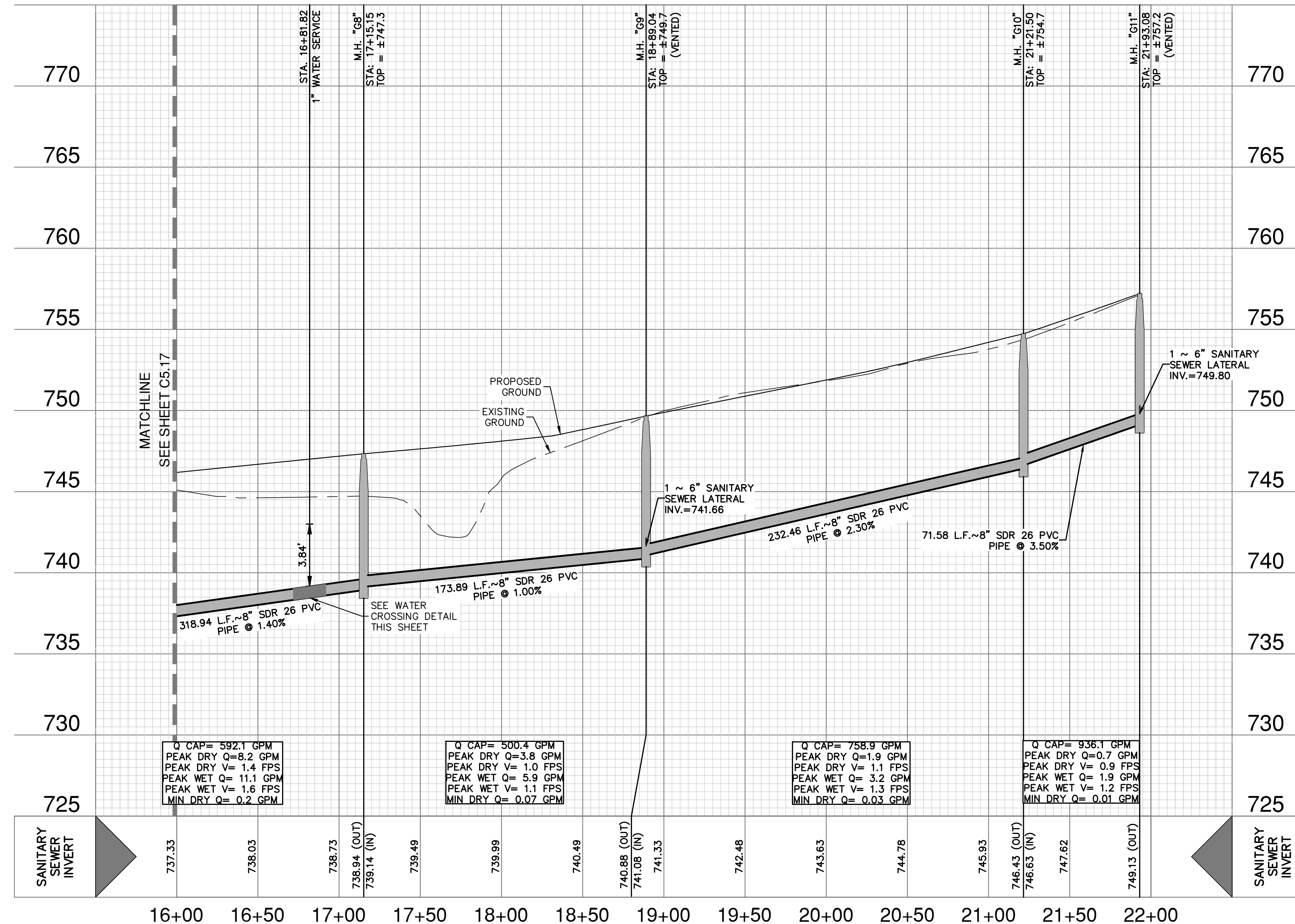
SANITARY SEWER LINE "G" STA 16+00.00 TO 21+30.25 VERTICAL SCALE: 1" = 5' HORIZONTAL SCALE: 1" = 50'
