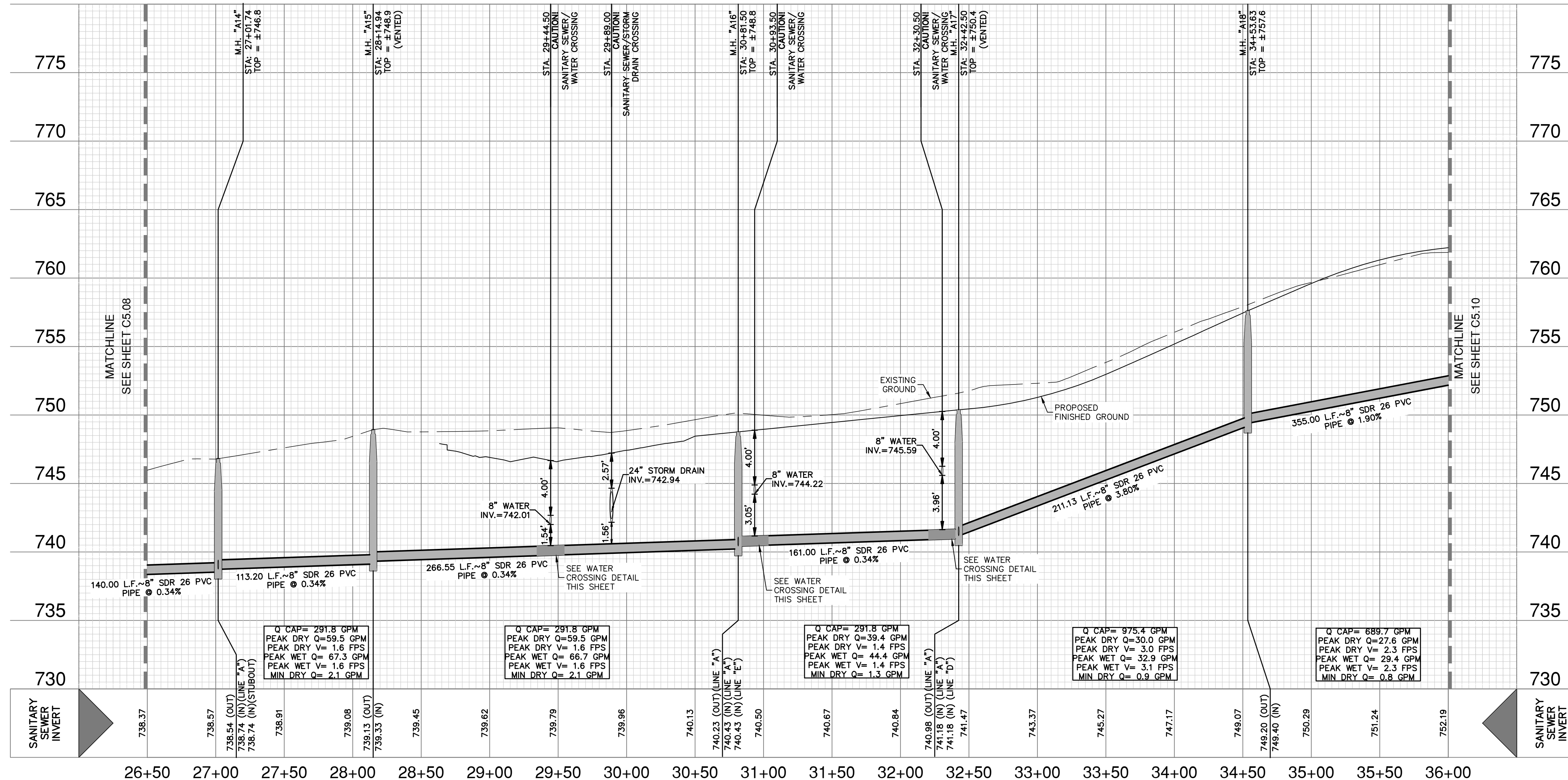
SANITARY SEWER LINE "A" STA 26+50.00 TO 36+00.00
