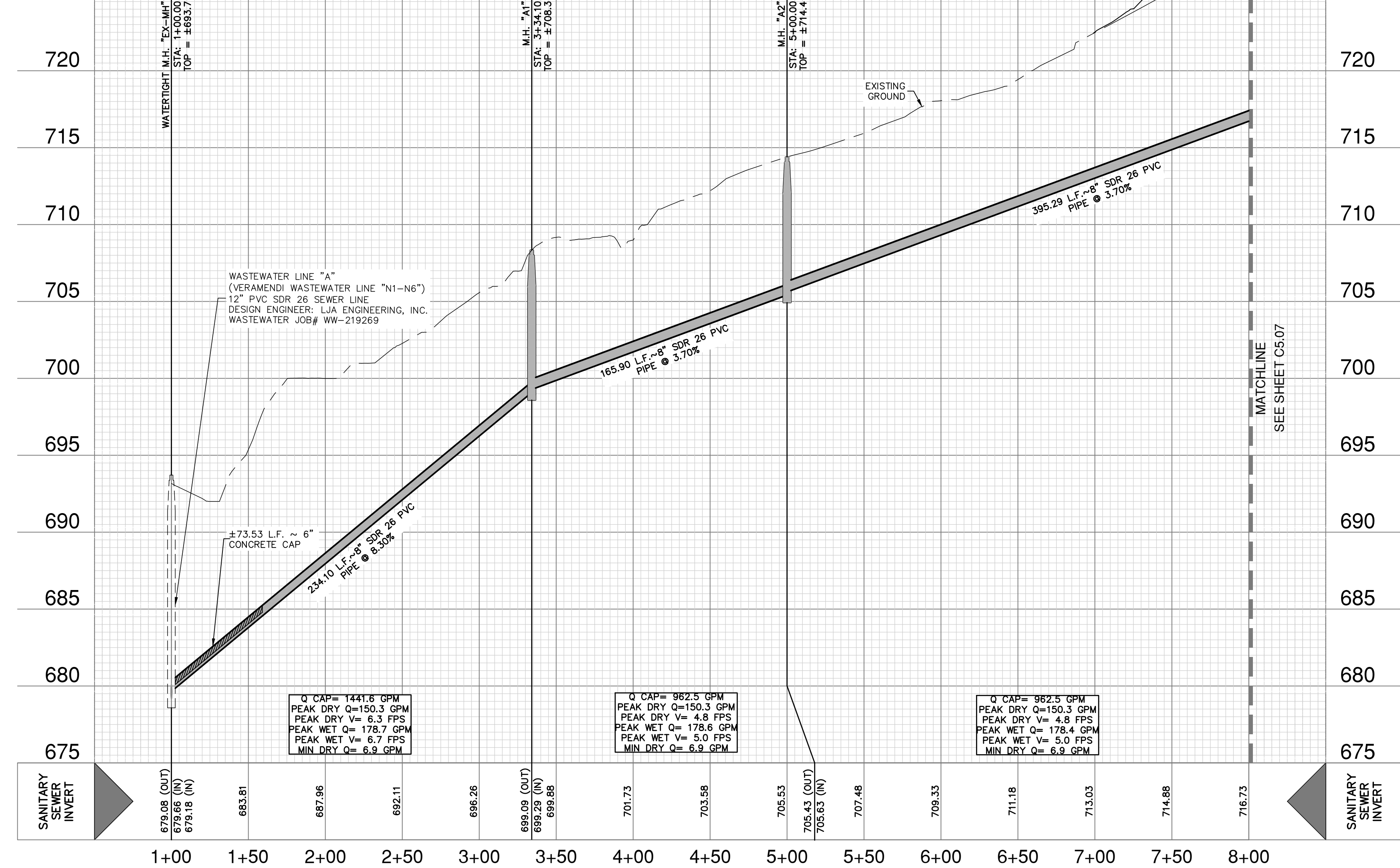
SANITARY SEWER LINE "A" STA 1+00.00 TO 8+00.00 VERTICAL SCALE: 1" = 5' HORIZONTAL SCALE: 1" = 50'
