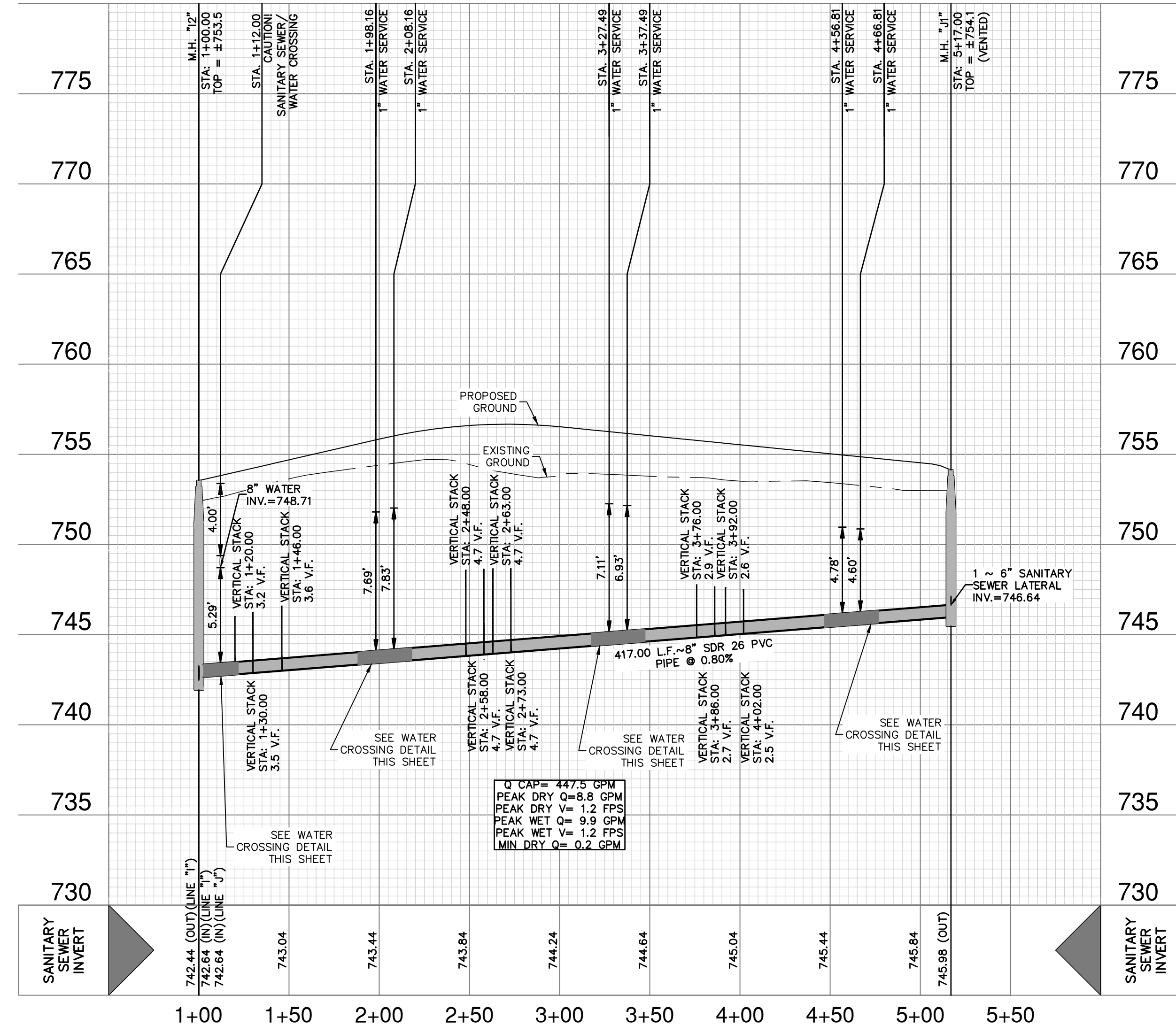
SANITARY SEWER LINE "J" STA 1+00.00 TO 5+17.00
