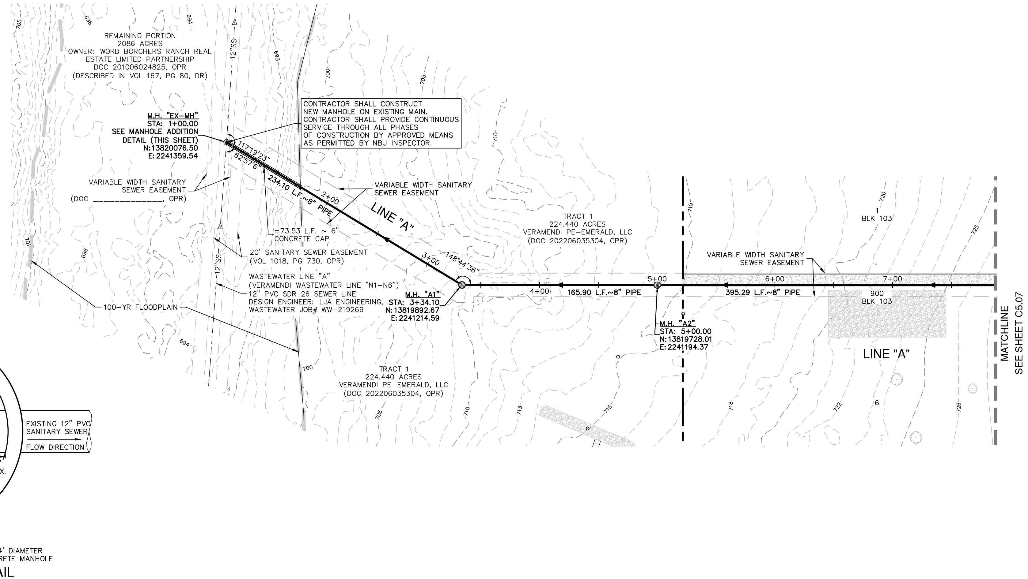
SANITARY SEWER LINE "A" STA 1+00.00 TO 8+00.00 VERTICAL SCALE: 1" = 5' HORIZONTAL SCALE: 1" = 50'
