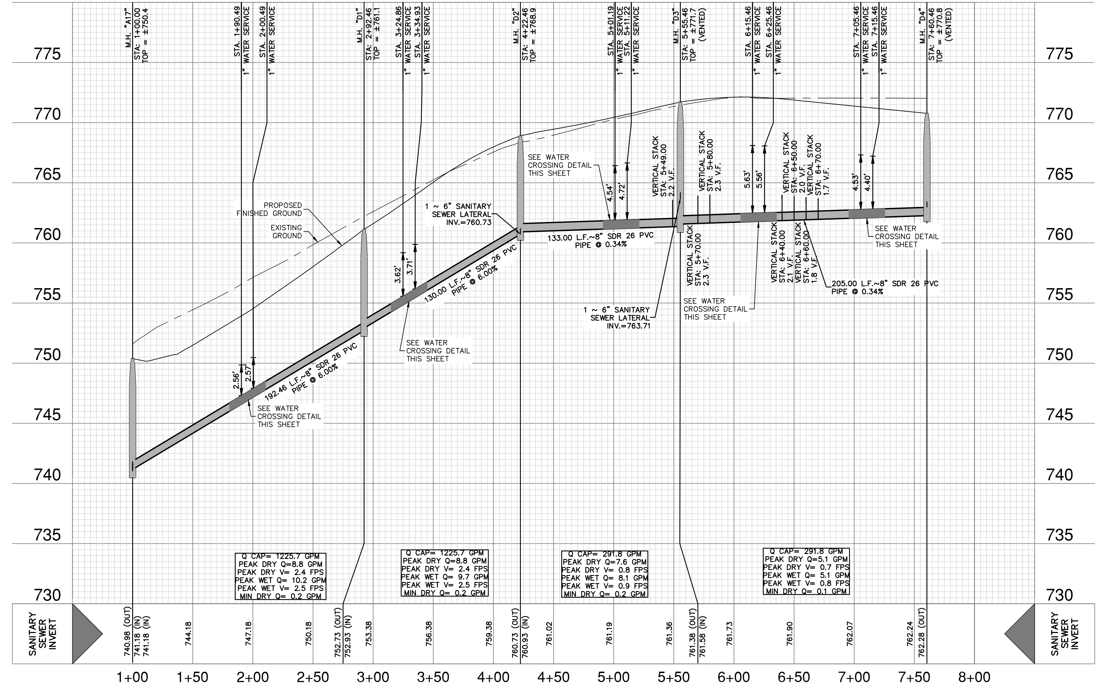
SANITARY SEWER LINE "D" STA 1+00.00 TO 7+60.46 VERTICAL SCALE: 1" = 5' HORIZONTAL SCALE: 1" = 50'
