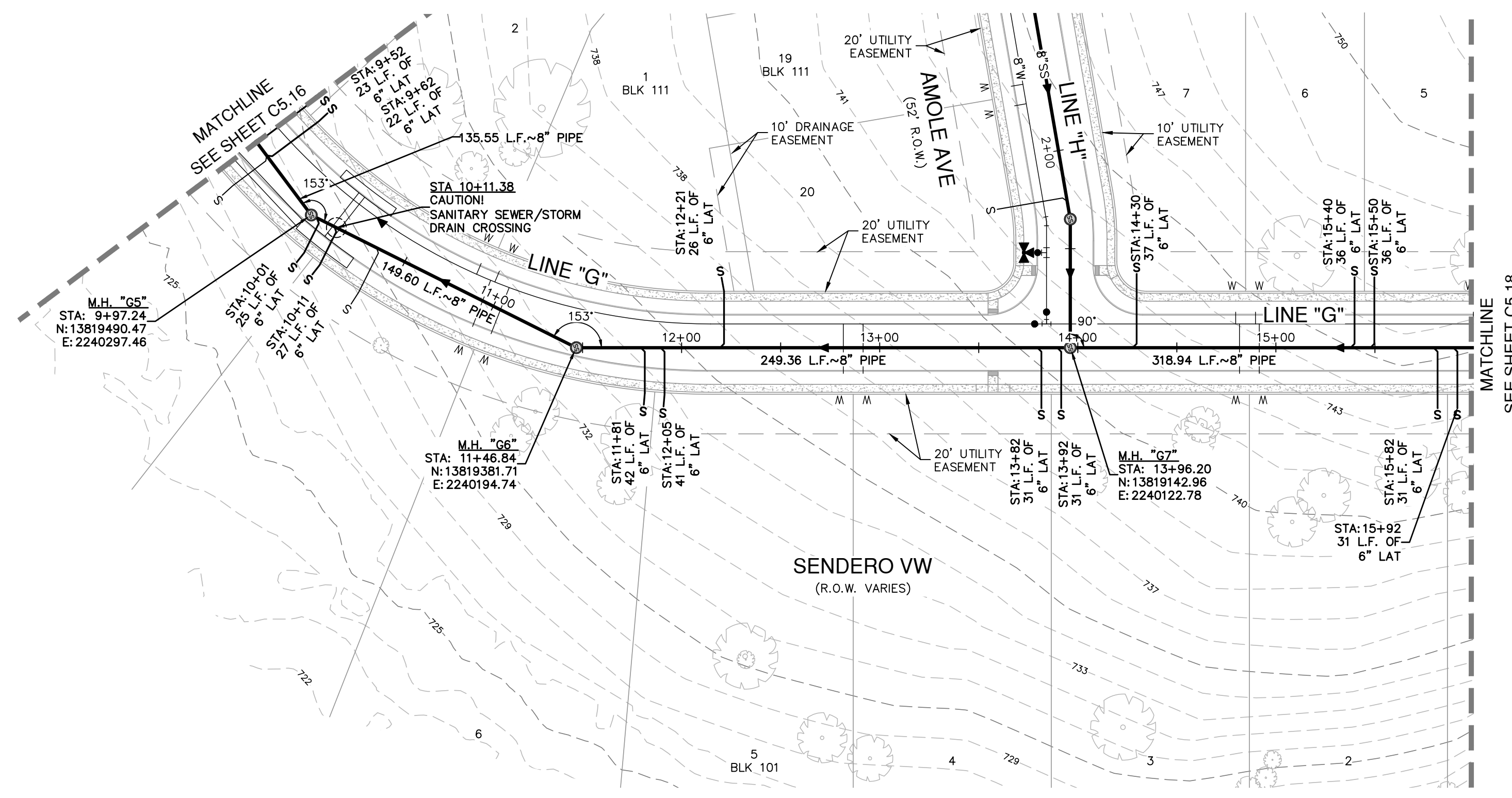
SANITARY SEWER LINE "G" STA 9+50.00 TO 16+00.00 VERTICAL SCALE: 1" = 5' HORIZONTAL SCALE: 1" = 50'
