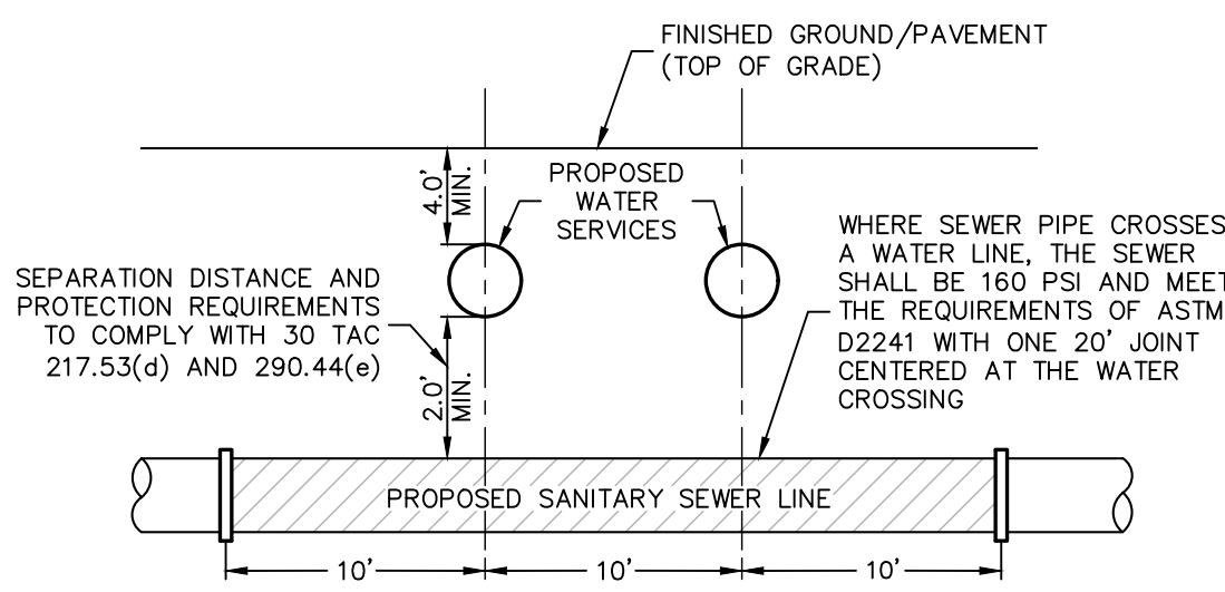
TYPICAL SANITARY SEWER/DOUBLE WATER SERVICE CROSSING DETAIL NOT TO SCALE
