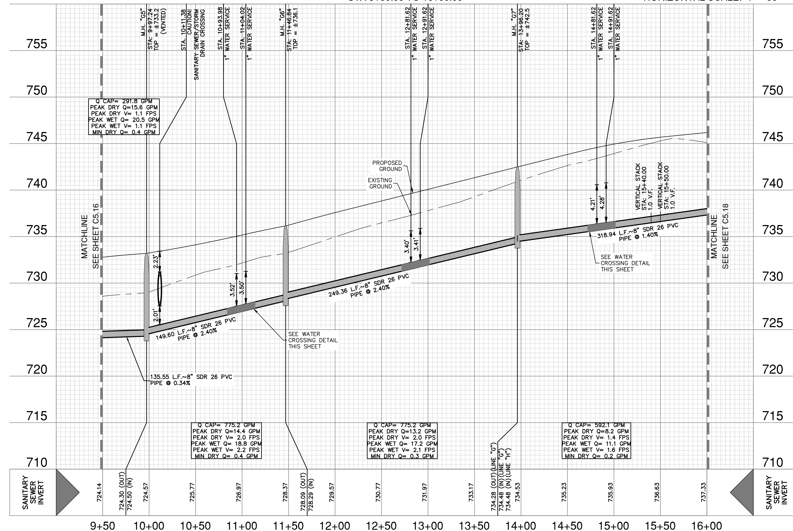
SANITARY SEWER LINE "G" STA 9+50.00 TO 16+00.00 VERTICAL SCALE: 1" = 5' HORIZONTAL SCALE: 1" = 50'
