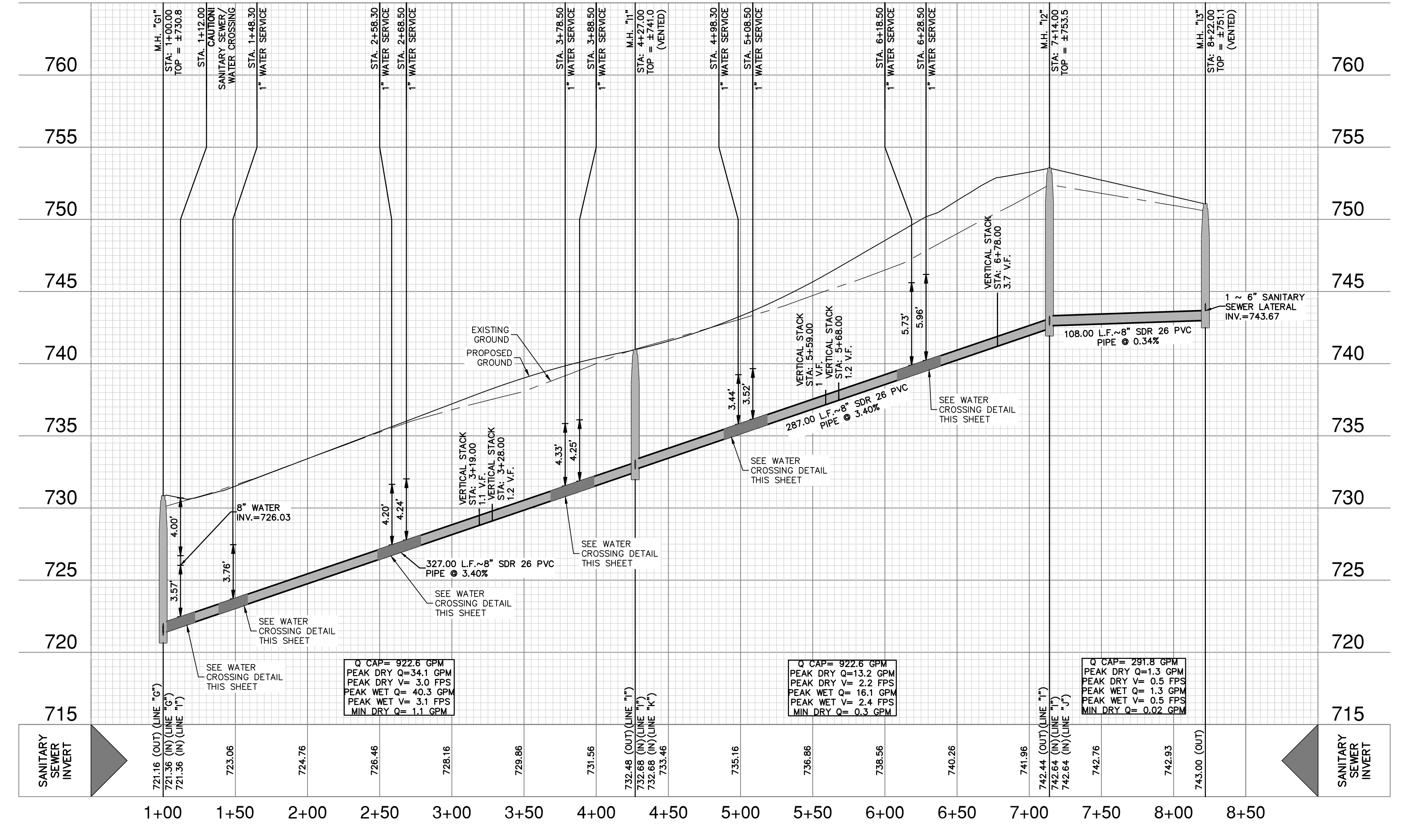
SANITARY SEWER LINE "I" STA 1+00.00 TO 8+22.00
