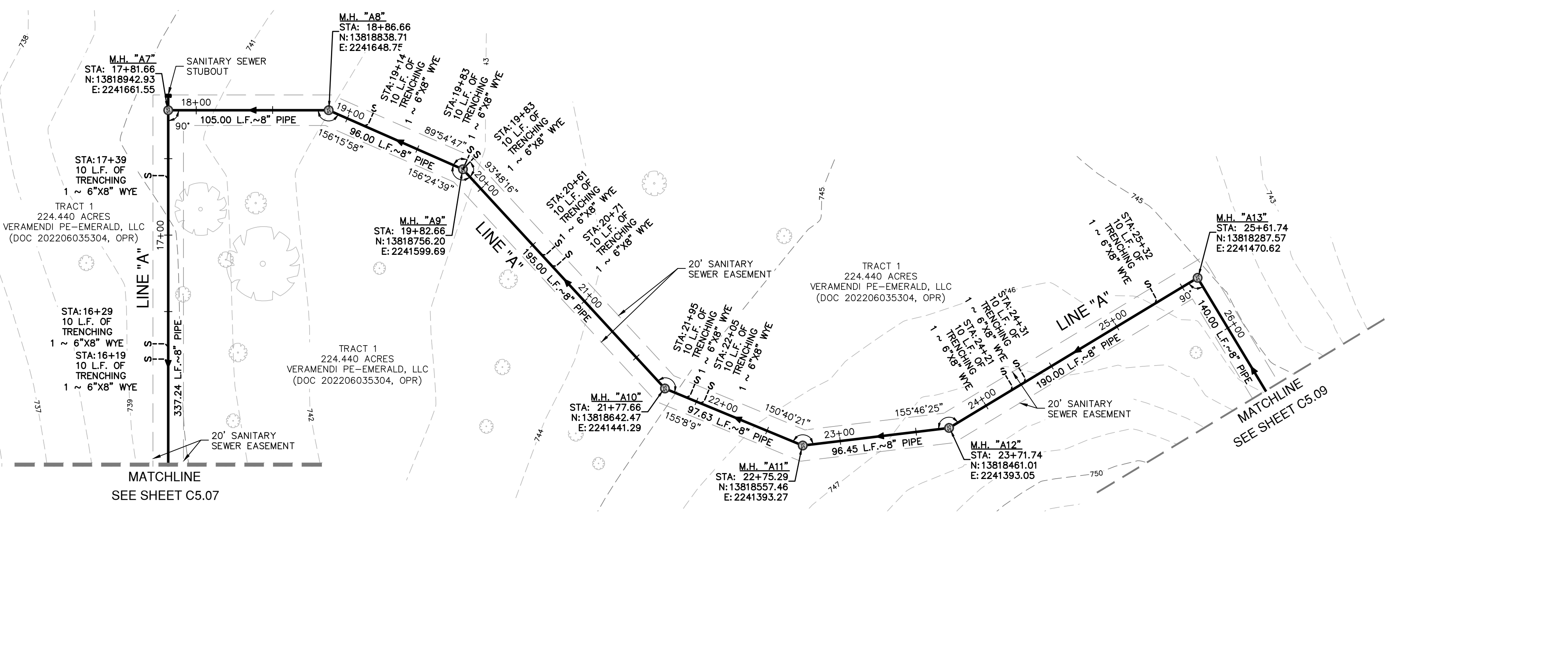
SANITARY SEWER LINE "A" STA 16+00.00 TO 27+00.00 VERTICAL SCALE: 1" = 5' HORIZONTAL SCALE: 1" = 50'
