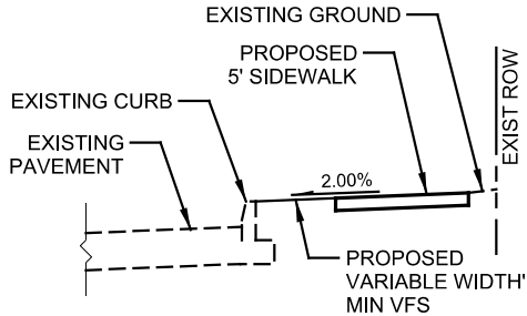
PROPOSED TYPICAL SECTION 5' DIVORCED SIDEWALK HARDY OAK BLVD SIDEWALK NOT TO SCALE
