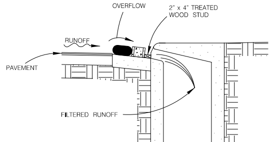
SECTION G-G
