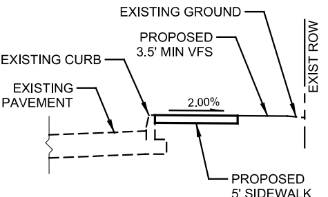
PROPOSED TYPICAL SECTION 5' MARRIED SIDEWALK HARDY OAK BLVD SIDEWALK NOT TO SCALE
