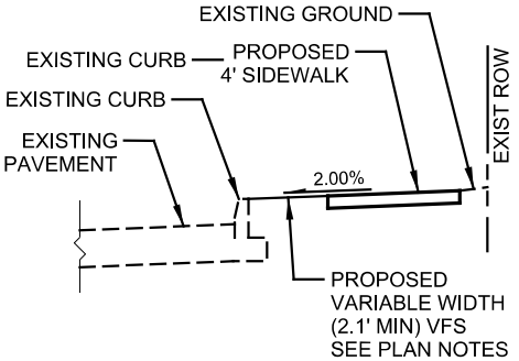
PROPOSED TYPICAL SECTION 4' DIVORCED SIDEWALK SPRING TERRACE DR SIDEWALK NOT TO SCALE
