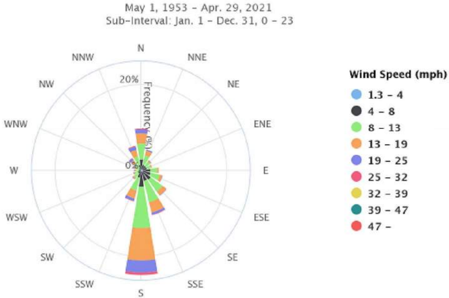
DALLAS FT WORTH AP (TX) Wind Rose
