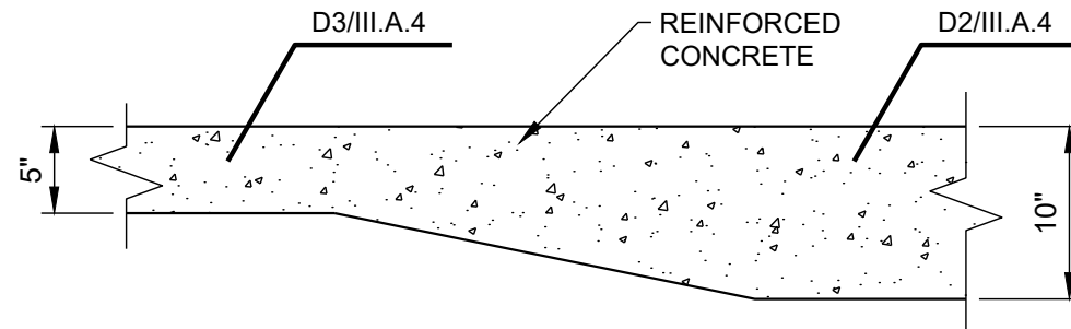
D6 PAVEMENT TRANSITION NOT TO SCALE
