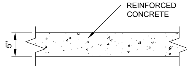
D3 PAVEMENT B NOT TO SCALE
