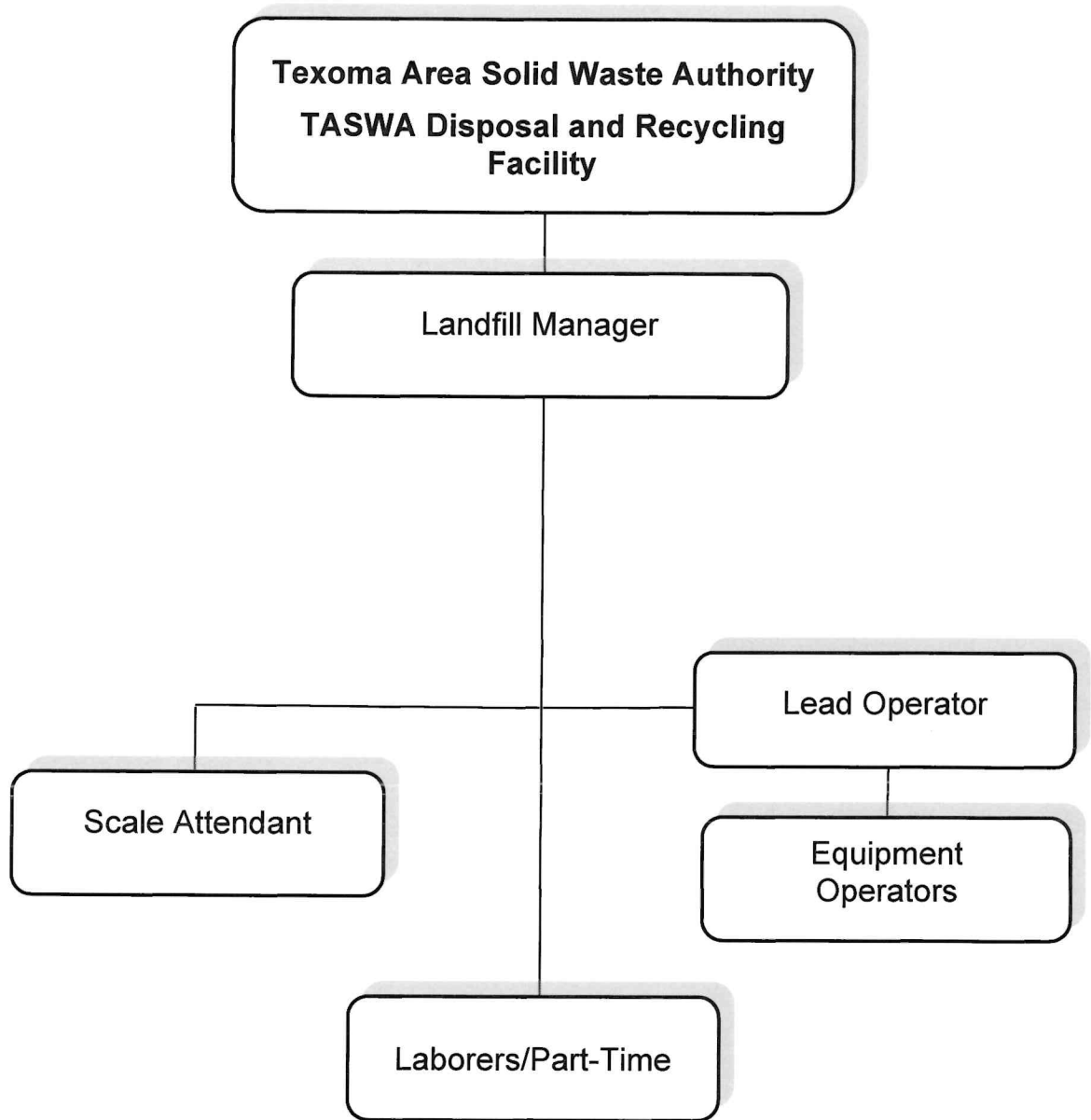
Figure 3.1 Organizational Chart
