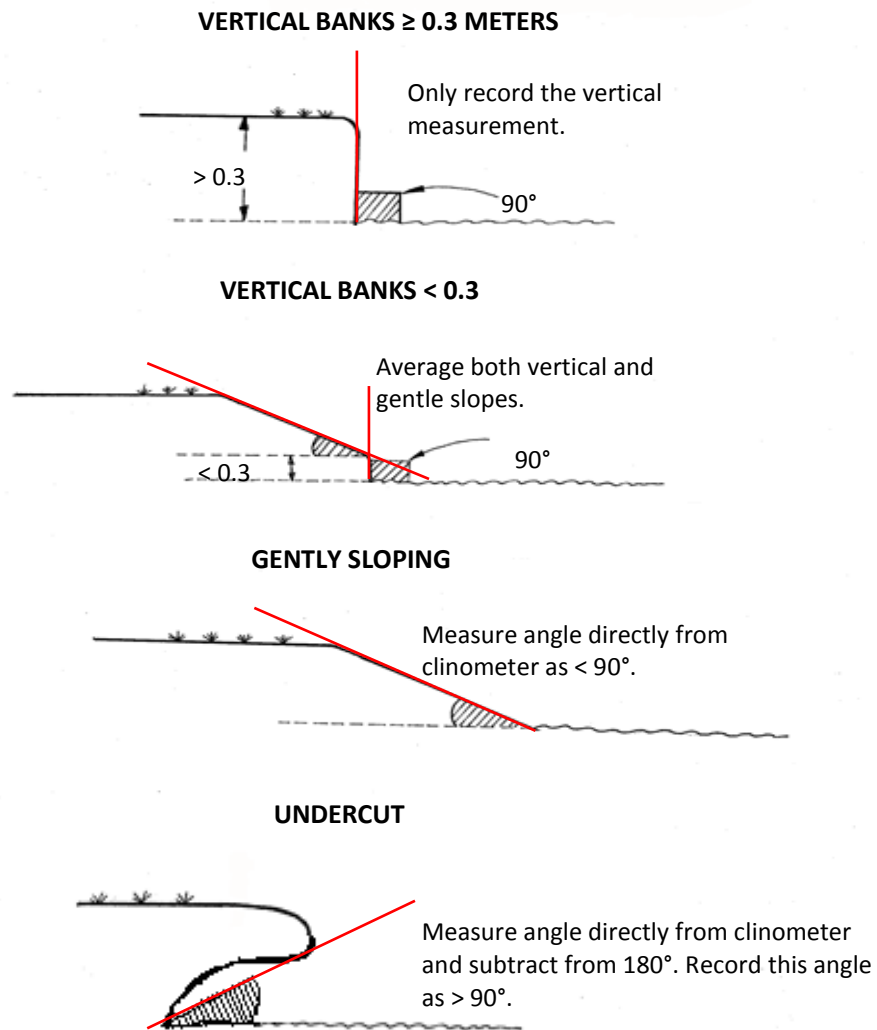
Figure 9.6. Bank-angle measurements.
