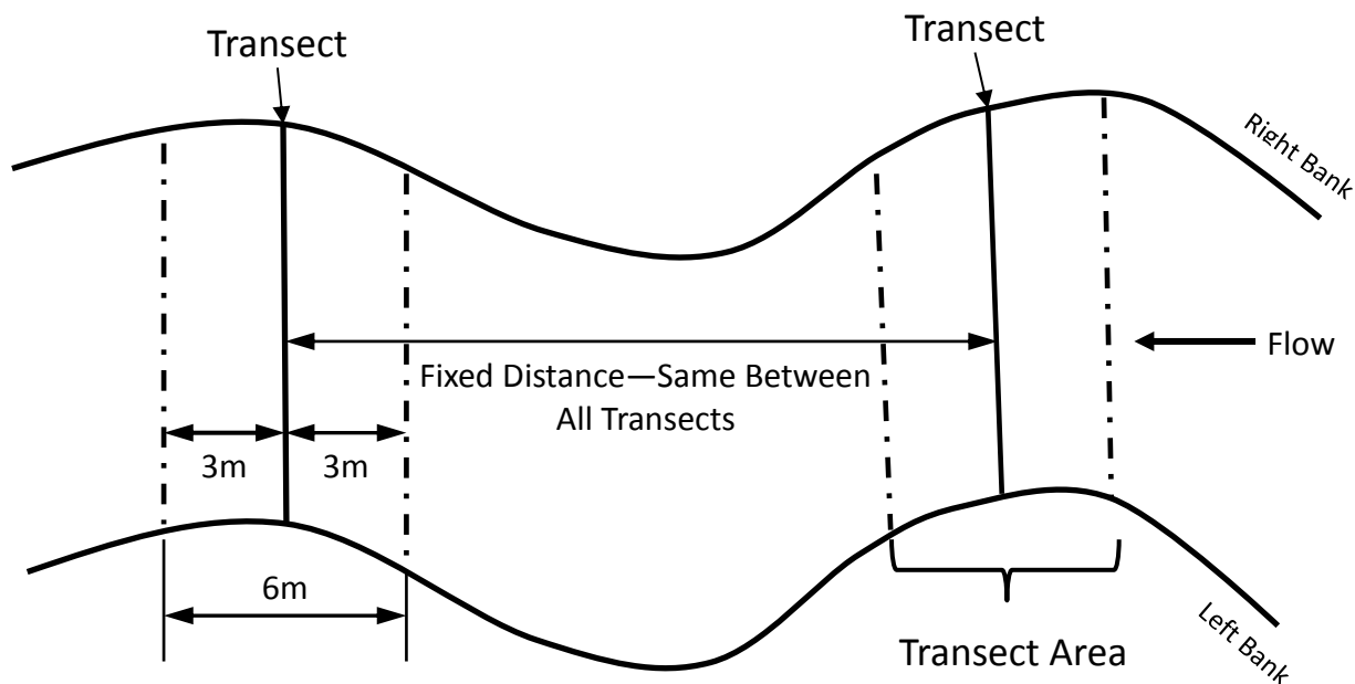
Figure 9.3. Transect area.
