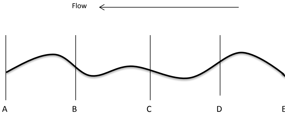
Figure 9.1. Transect placement for reach lengths of 150 to 300 m.
