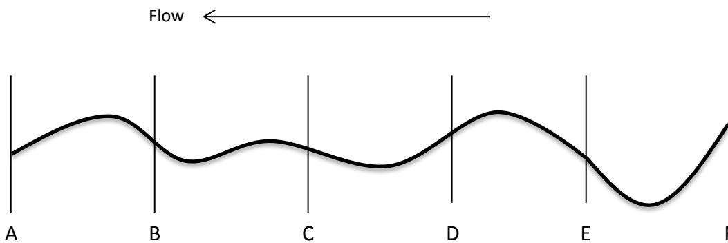
Figure 9.2. Transect placement for reach lengths of 301 to 500 m.
