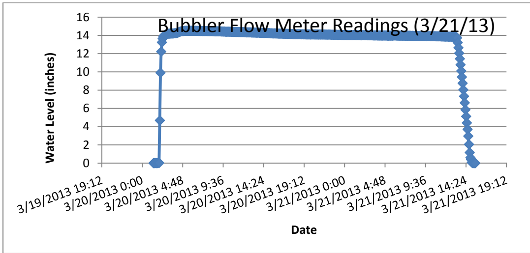
Figure 11. Pon Court Basin Bubbler Flow Meter Water Level after March 20, 2013 Storm Event.
