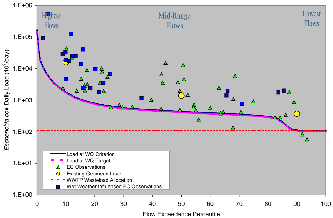
Figure 11. Load Duration Curve for Sims Bayou Above Tidal (1007D_03)
