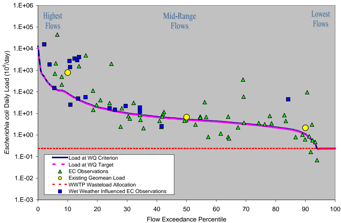
Figure 12. Load Duration Curve for Unnamed Non-Tidal Tributary of Sims Bayou (1007N_01)
