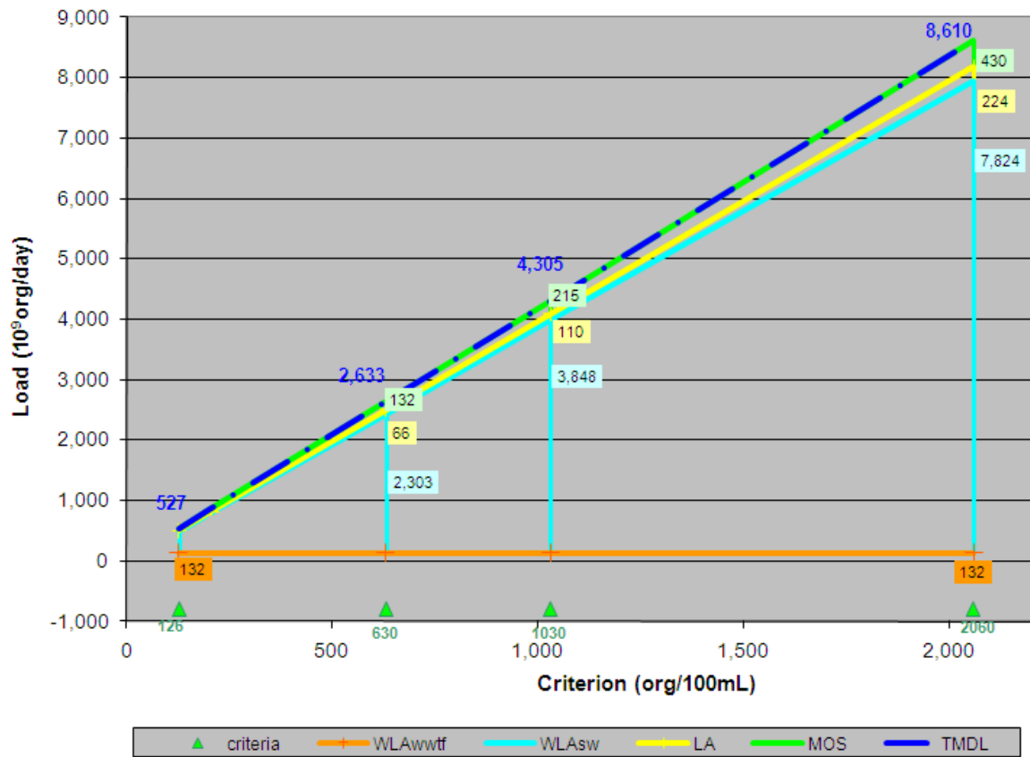
Figure A-2. Allocation Loads for AU 1007D_02 as a function of WQ Criteria
