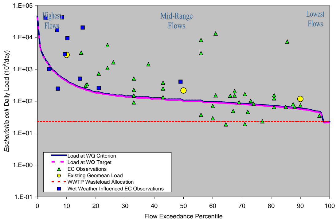
Figure 9. Load Duration Curve for E. coli in Sims Bayou Above Tidal (1007D_01)
