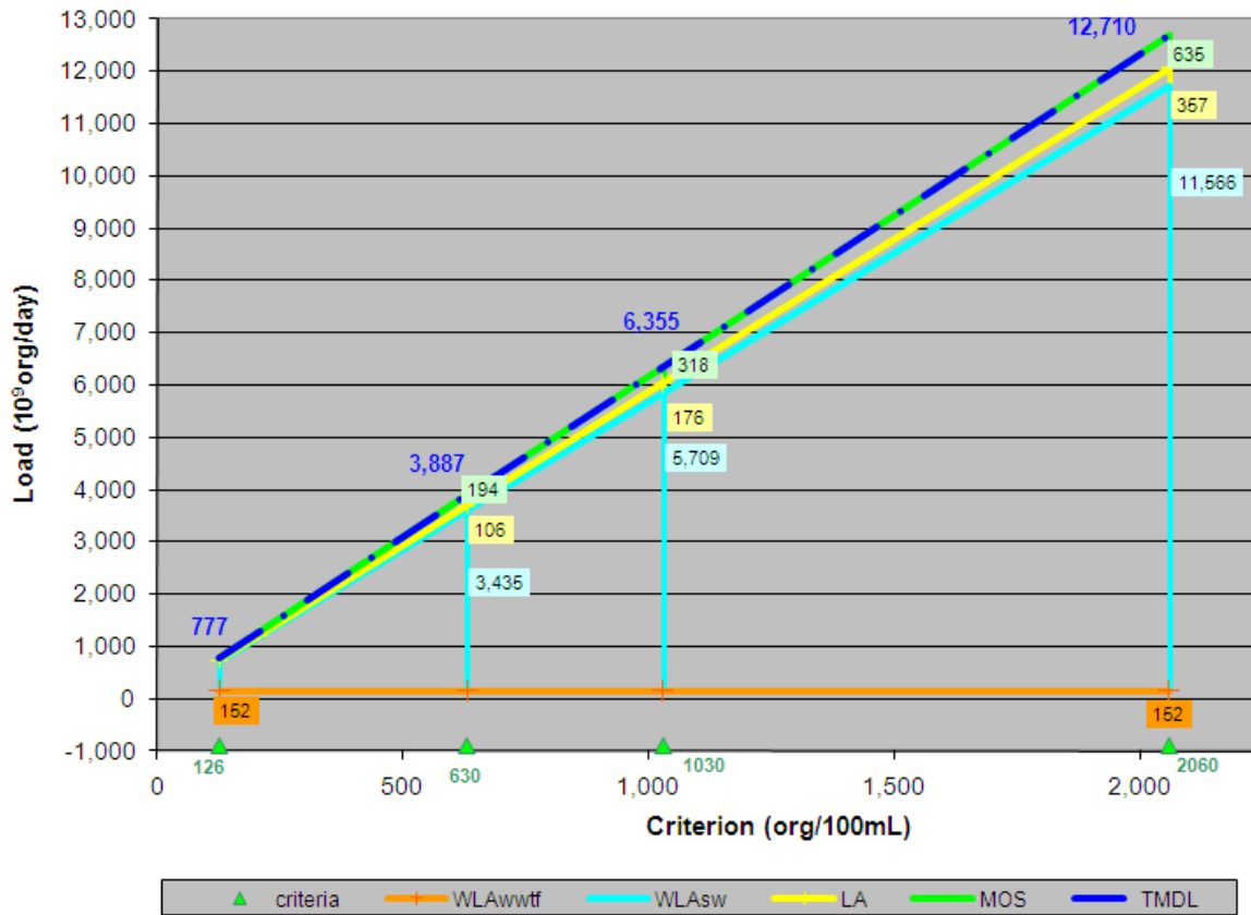
Figure A-3. Allocation Loads for AU 1007D_03 as a function of WQ Criteria
