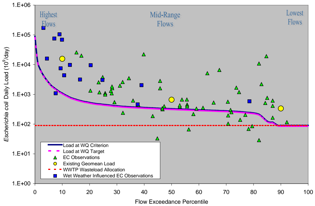
Figure 10. Load Duration Curve for Sims Bayou Above Tidal (1007D_02)
