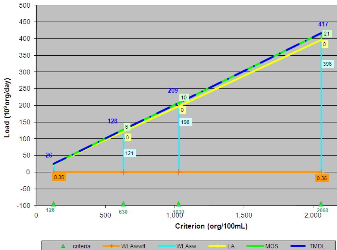
Figure A-4. Allocation Loads for AU 1007N_01 as a function of WQ Criteria
