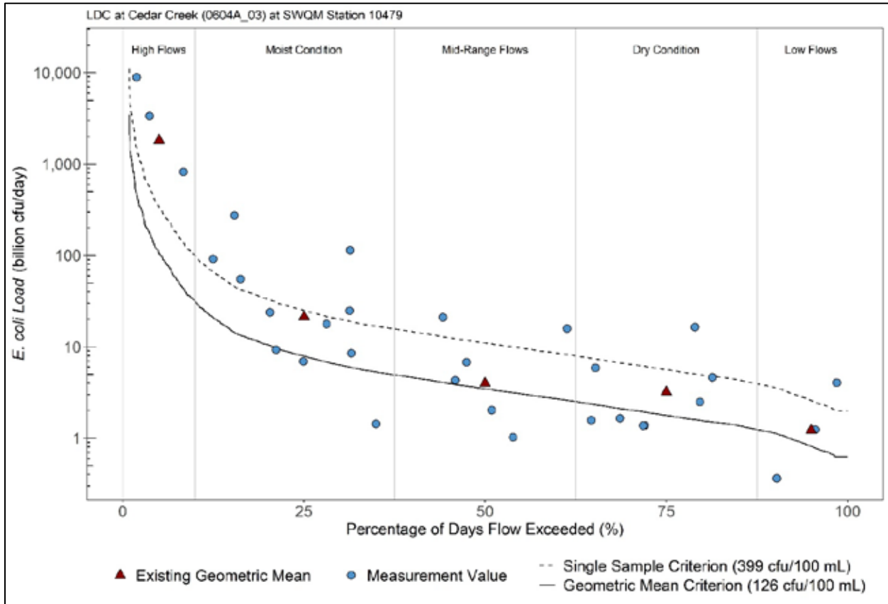
Figure 9. LDC for AU 0604A_03 at SWQM station 10479
