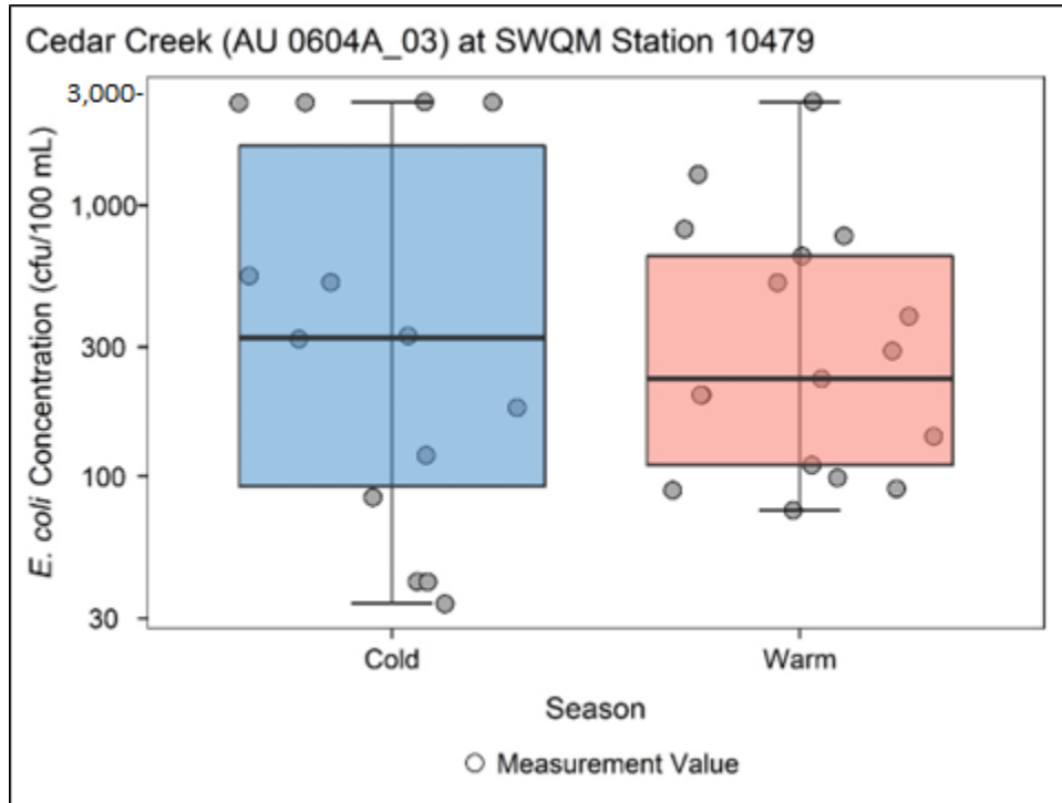
Figure 10. Distribution of E. coli concentrations by season in the AU 0604A_03 watershed
