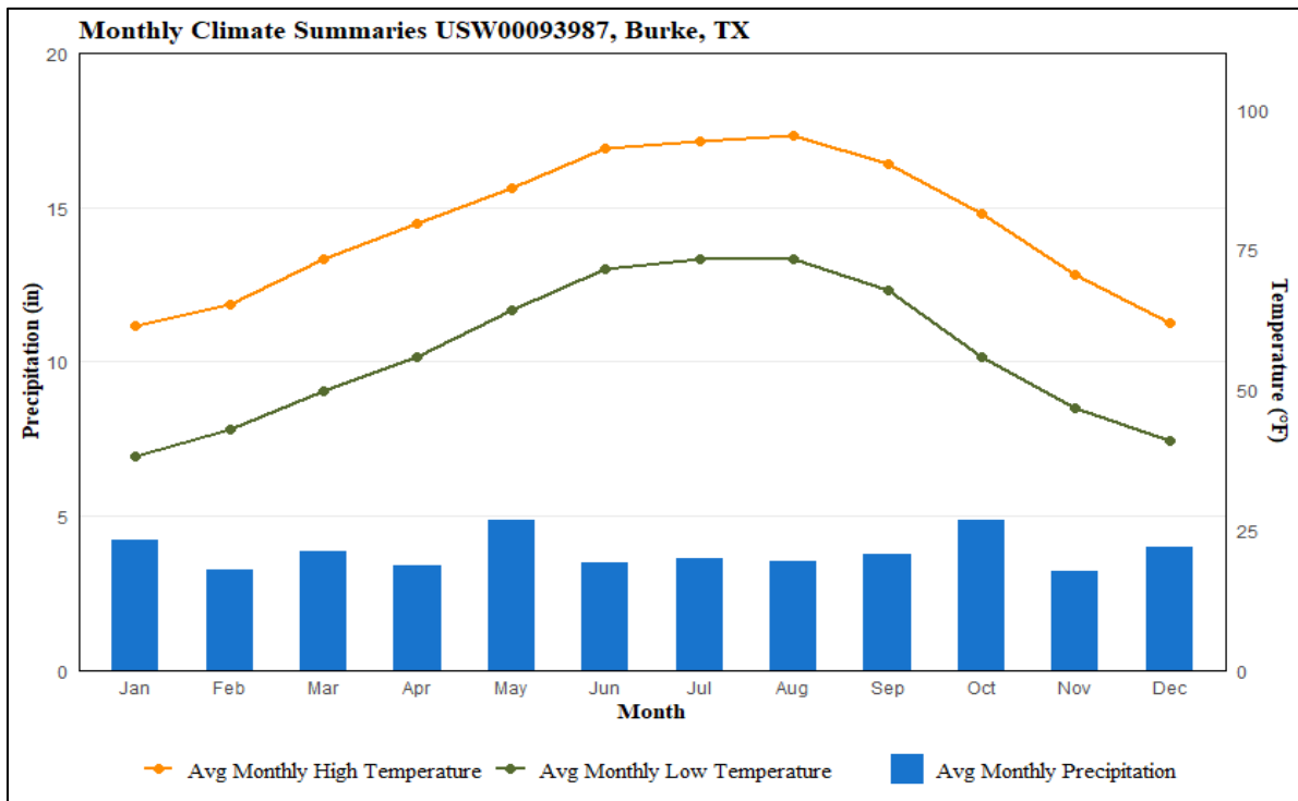
Figure 2. Average monthly temperature and precipitation (2005-2018) at Angelina County Airport
