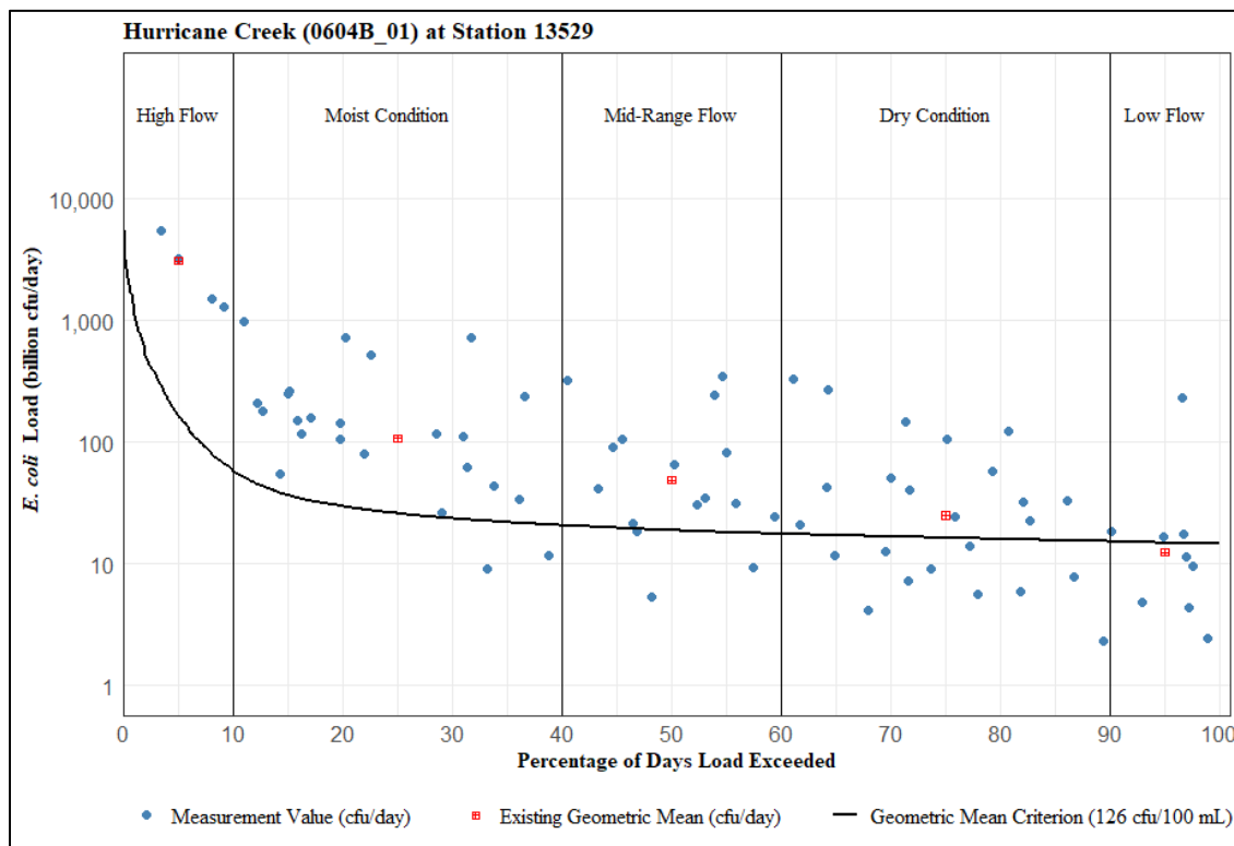
Figure 16. LDC for Hurricane Creek AU 0604B_01 at SWQM station 13529
