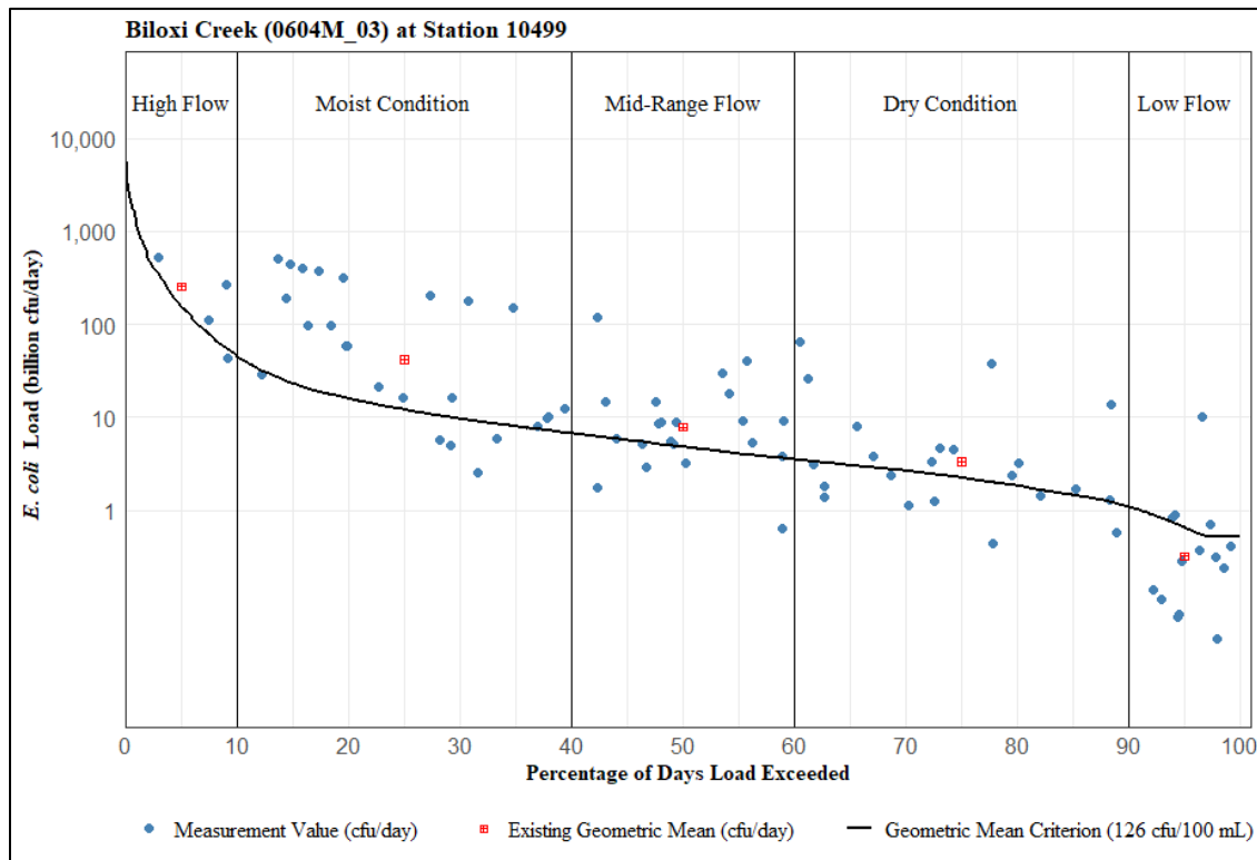
Figure 18. LDC for Biloxi Creek AU 0604M_03 at SWQM station 10499
