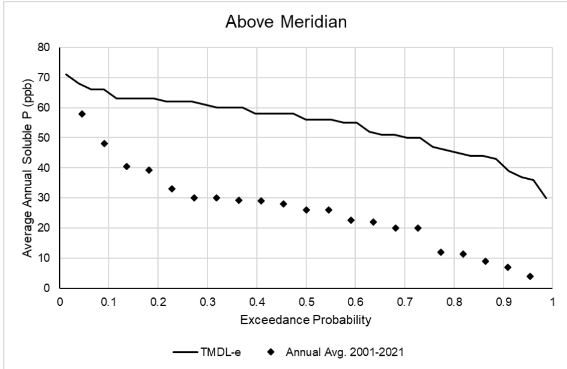
Figure 14 TMDL goal probability curve for index site above Meridian (18003 [BO083]) compared to monitored data curve
