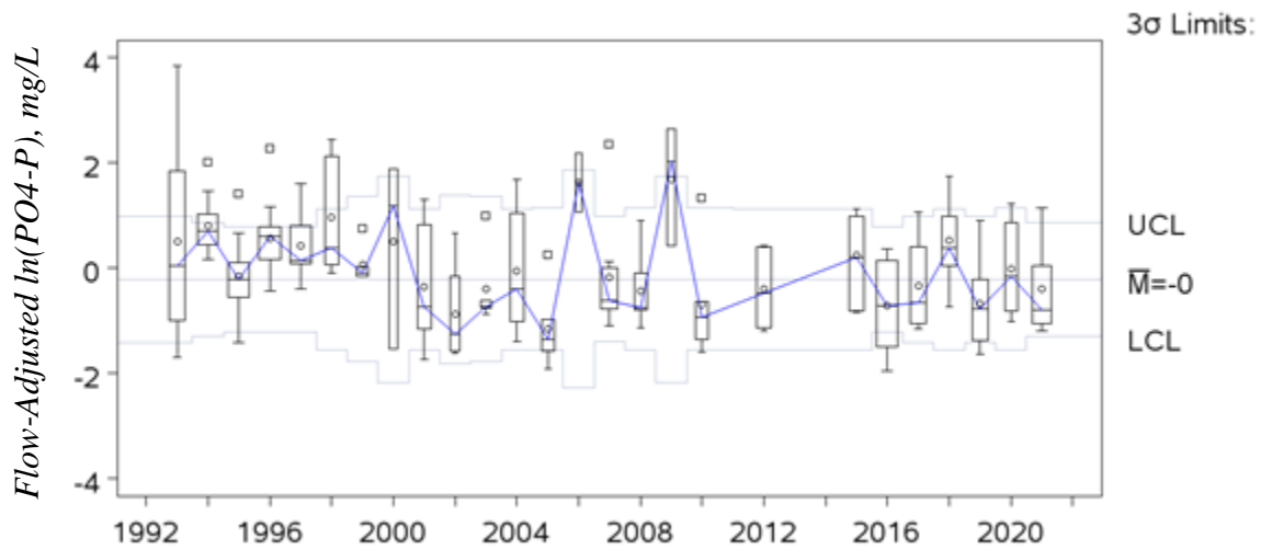
Figure 20 Annual box-and-whisker plots of monthly volume-weighted PO 4 -P grab data for station 13486 (GC100)
