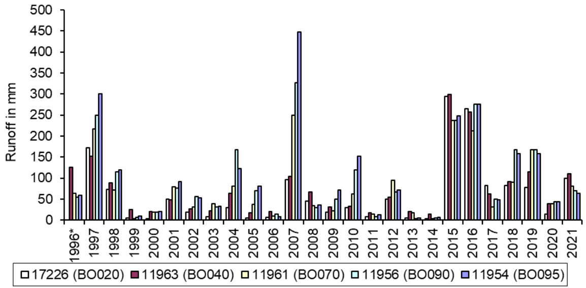
Figure 26 Annual runoff in millimeters for gauged stations along the North Bosque River
