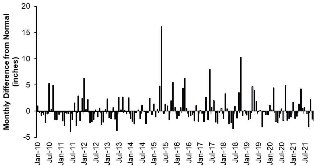
Figure 25 Monthly difference from normal precipitation from January 2010 through December 2021 for Stephenville, Texas
