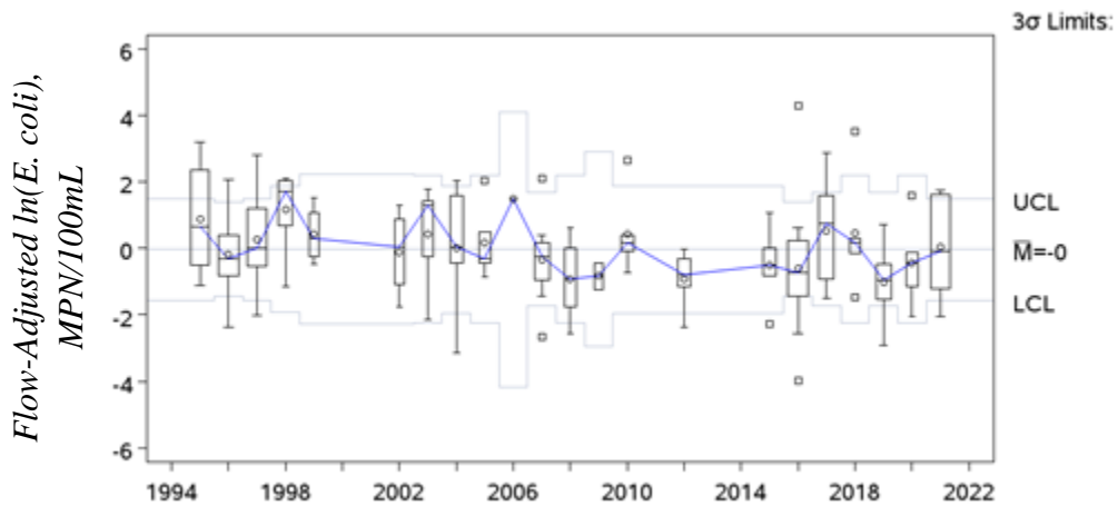
Figure B-6 Annual box-and-whisker plots of monthly flow-weighted and flow-adjusted E. coli data for station 13486 (GC100)
