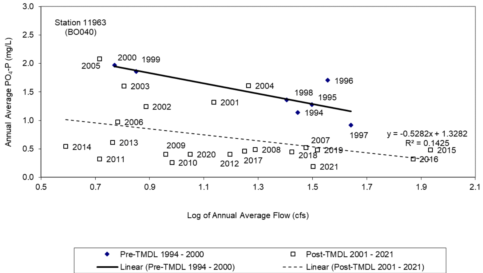
Figure 5 Relationship of the natural log of flow to annual average PO 4 -P concentration of routine grab samples for station 11963 (BO040)
