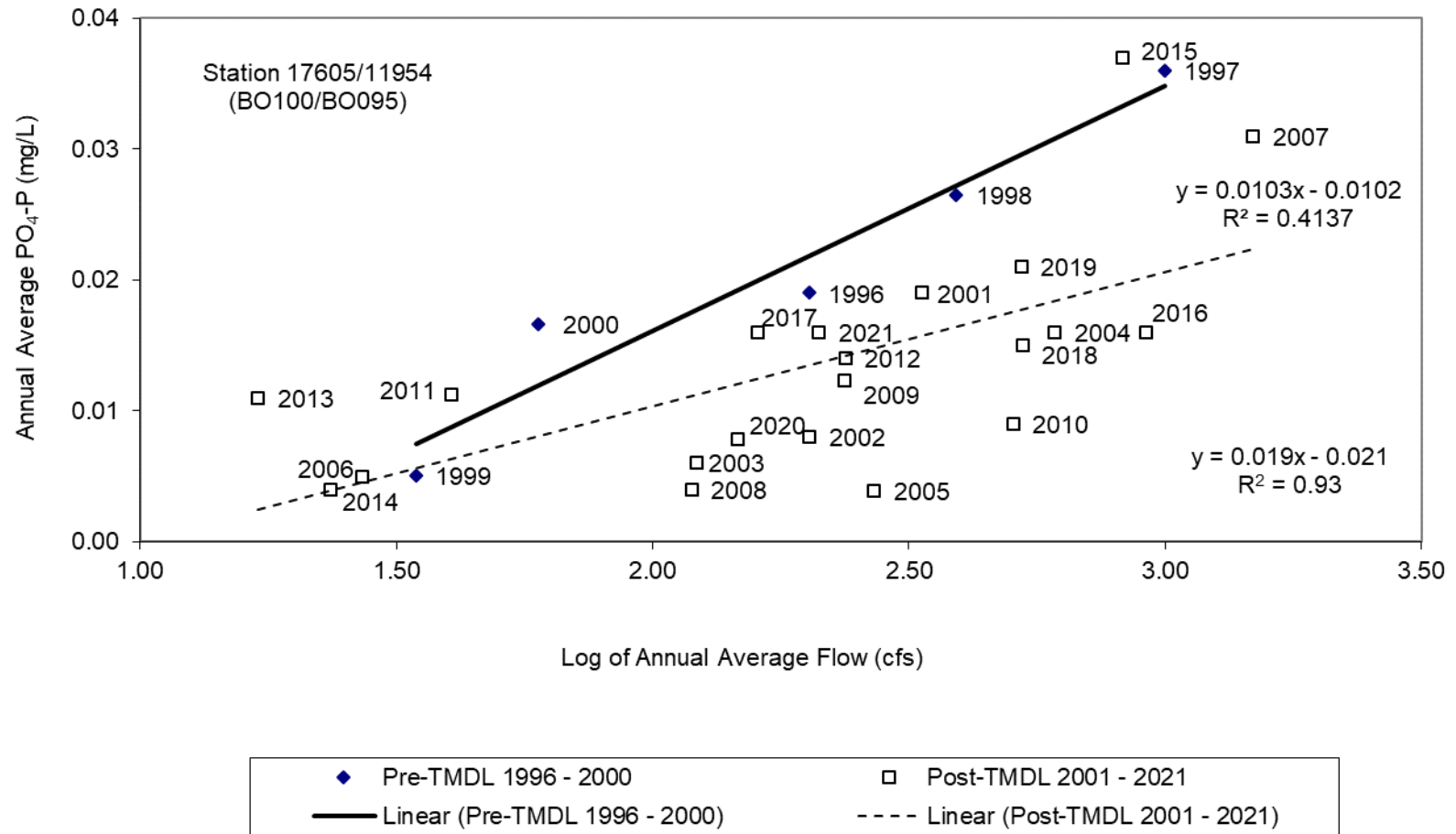
Figure 9 Relationship of the natural log of flow to annual average PO 4 -P concentration of routine grab samples for station 17605/11954 (BO100/BO095)
