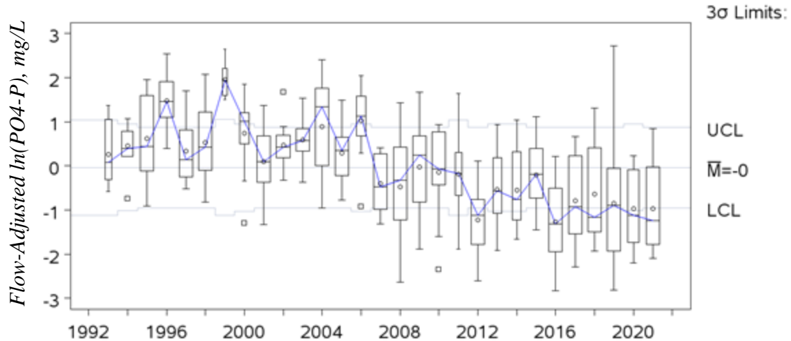
Figure 19 Annual box-and-whisker plots of monthly volume-weighted \text{PO}_4\text{-P} grab data for station 11961 (BO070)
