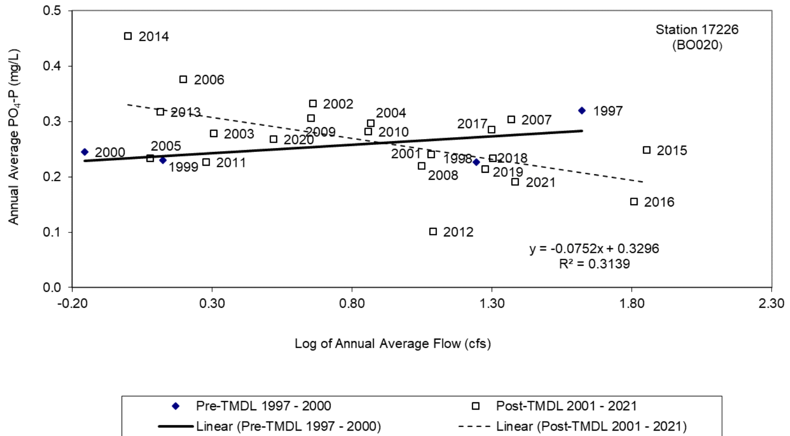
Figure 4 Relationship of the natural log of flow to annual average PO 4 -P concentration of routine grab samples for station 17226 (BO020)
