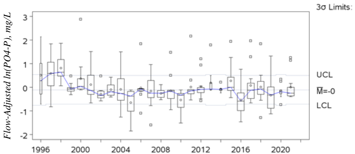
Figure 22 Annual box-and-whisker plots of monthly volume-weighted PO 4 -P data for station 11954 (BO095)
