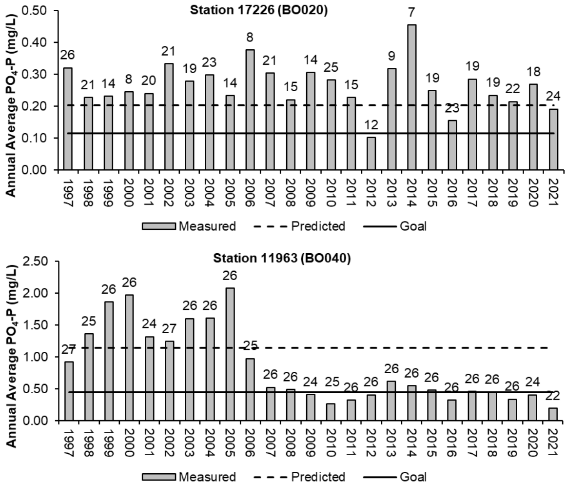
Figure 10 Annual average PO 4 -P from routine grab data for stations 17226 (BO020) and 11963 (BO040) compared to the long-term predicted concentration without TMDL implementation and the TMDL goal
