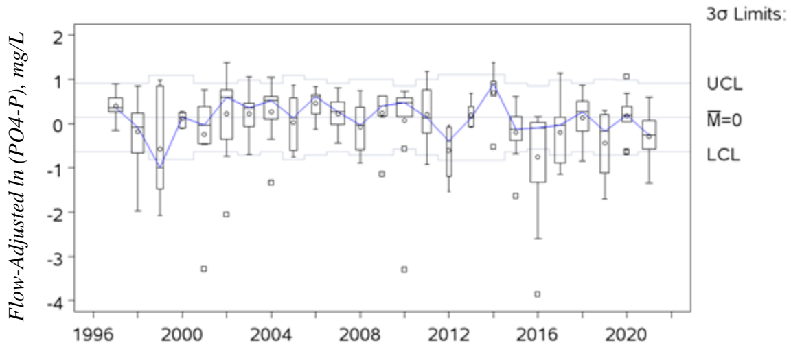
Figure 17 Annual box-and-whisker plots of monthly volume-weighted \text{PO}_4\text{-P} grab data for station 17226 (BO020)
