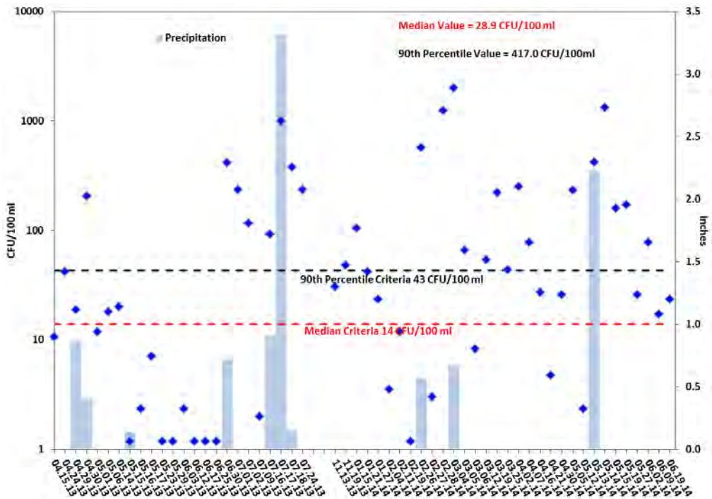
Figure 4.3. All fecal coliform concentrations at Station 13440 with precipitation amounts, median and 90 th percentile criteria, and actual calculated median and 90 th percentile values.
