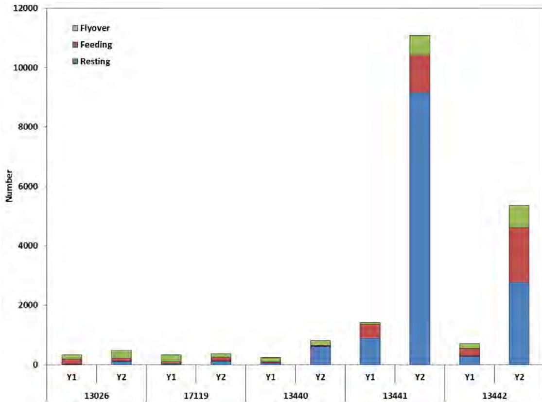
Figure 4.6. Total numbers of birds at each sampling location by activity observed for Year-one and Year-two.
