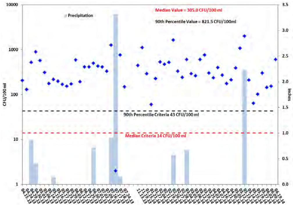
Figure 4.4. All fecal coliform concentrations at Station 13441 with precipitation amounts, median and 90 th percentile criteria, and actual calculated median and 90 th percentile values.
