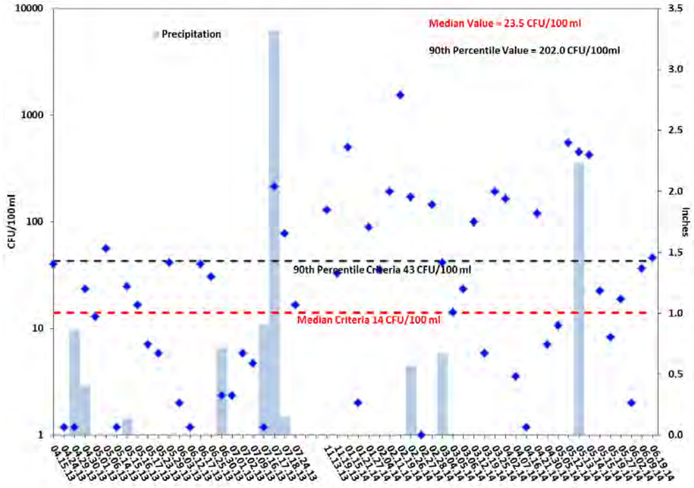
Figure 4.5. All fecal coliform concentrations at Station 13442 with precipitation amounts, median and 90 th percentile criteria, and actual calculated median and 90 th percentile values.
