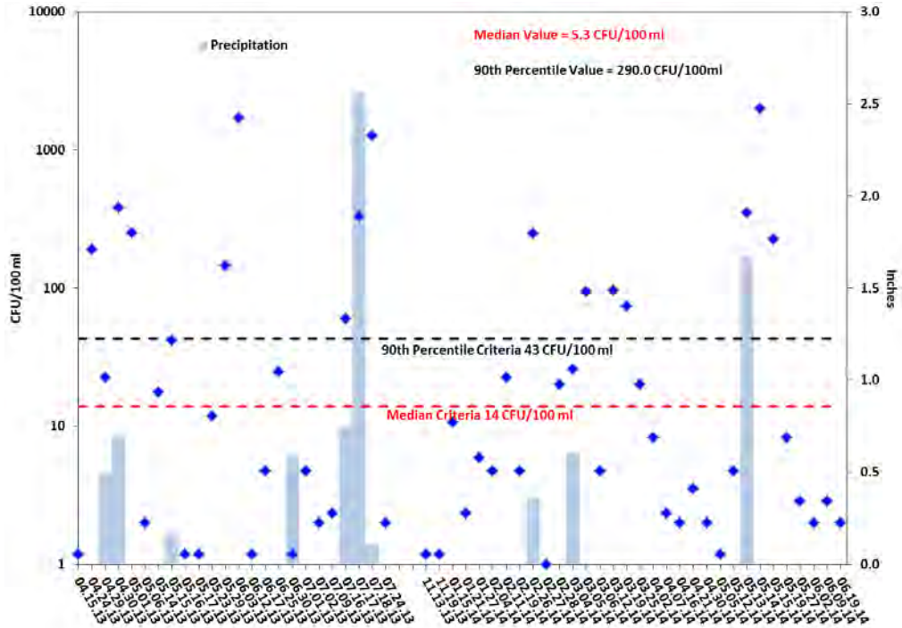
Figure 4.1. All fecal coliform concentrations at Station 13026 with precipitation amounts, median and 90 th percentile criteria, and actual calculated median and 90 th percentile values.
