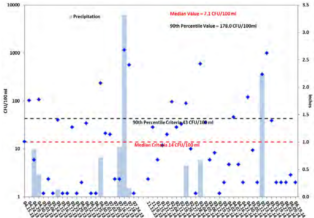
Figure 4.2. All fecal coliform concentrations at Station 17719 with precipitation amounts, median and 90 th percentile criteria, and actual calculated median and 90 th percentile values.
